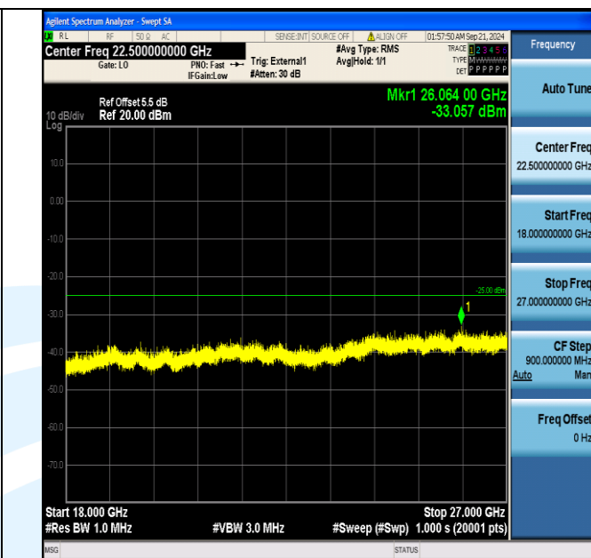
Band38_10MHz_QPSK_37800_1RB#0_18000~27000_18000~27000
