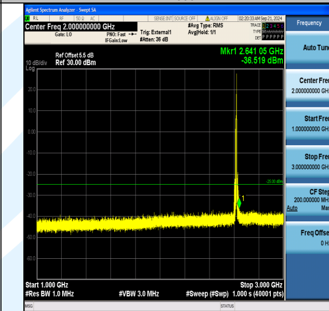
Band38_10MHz_QPSK_38200_1RB#49_1000~3000_1000~3000
