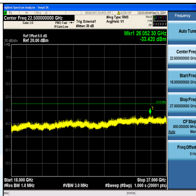
Band38_10MHz_QPSK_37800_1RB#49_18000~27000_18000~27000
