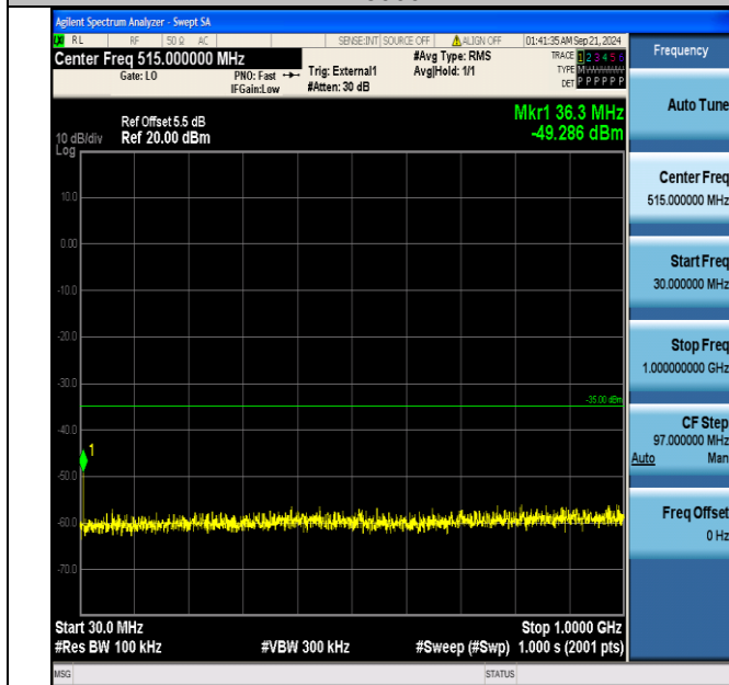
Band38_5MHz_16QAM_38000_1RB#24_30~1000_30~1000
