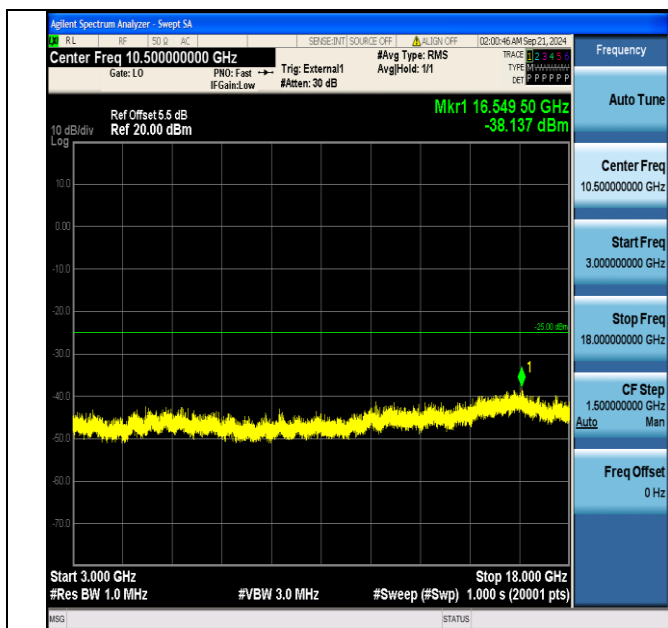
Band38_10MHz_QPSK_37800_1RB#49_3000~18000_3000~18000
