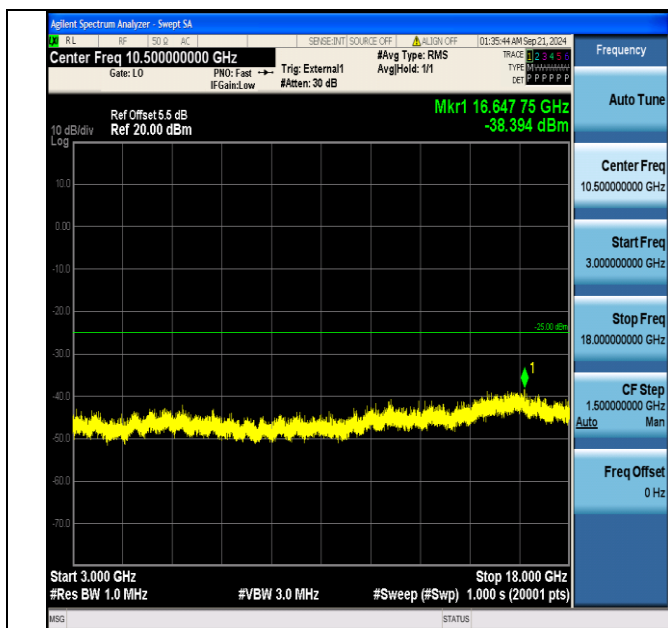
Band38_5MHz_16QAM_37775_25RB#0_3000~18000_3000~18000
