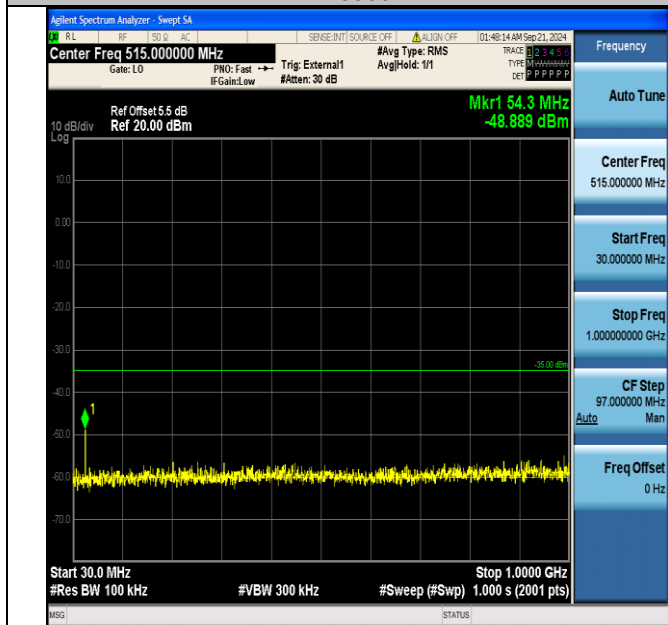
Band38_5MHz_16QAM_38225_1RB#0_30~1000_30~1000
