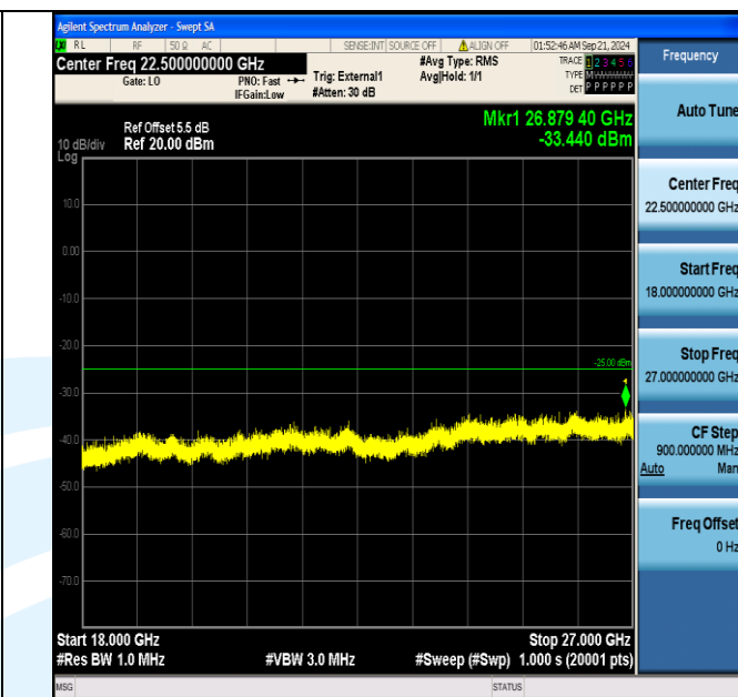
Band38_5MHz_16QAM_38225_1RB#24_18000~27000_18000~27000
