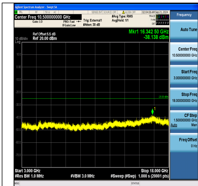
Band38_10MHz_QPSK_37800_50RB#0_3000~18000_3000~18000
