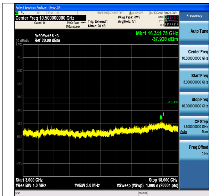
Band38_5MHz_16QAM_38225_1RB#24_3000~18000_3000~18000
