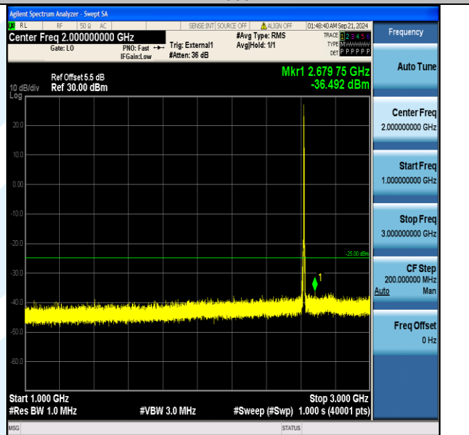
Band38_5MHz_16QAM_38225_1RB#0_1000~3000_1000~3000
