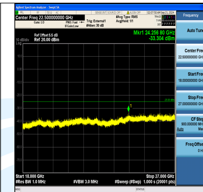
Band38_10MHz_QPSK_38000_1RB#0_18000~27000_18000~27000
