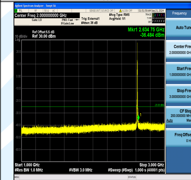
Band38_5MHz_16QAM_38225_1RB#24_1000~3000_1000~3000
