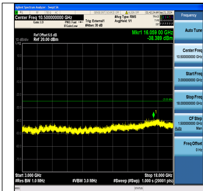
Band38_5MHz_16QAM_38000_1RB#24_3000~18000_3000~18000
