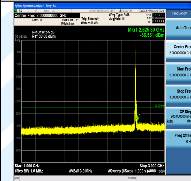
Band38_10MHz_QPSK_38000_1RB#49_1000~3000_1000~3000
