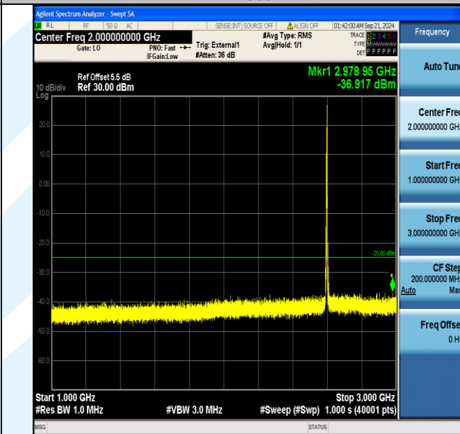
Band38_5MHz_16QAM_38000_1RB#24_1000~3000_1000~3000
