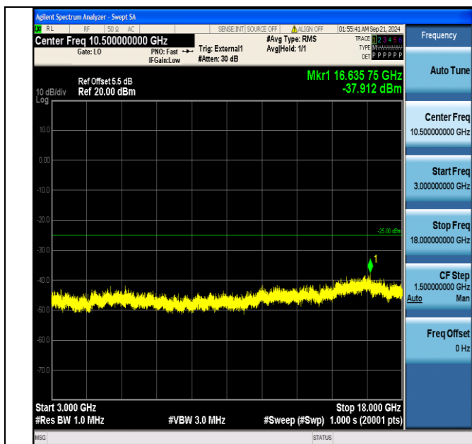
Band38_5MHz_16QAM_38225_25RB#0_3000~18000_3000~18000
