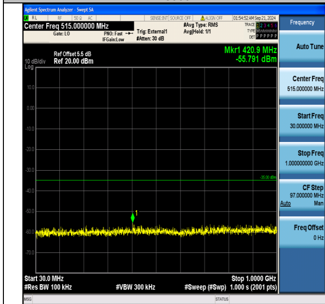
Band38_5MHz_16QAM_38225_25RB#0_30~1000_30~1000
