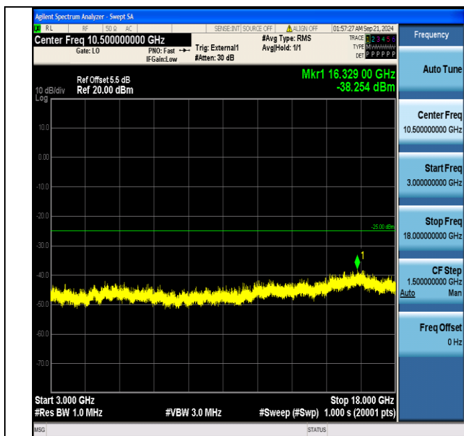
Band38_10MHz_QPSK_37800_1RB#0_3000~18000_3000~18000
