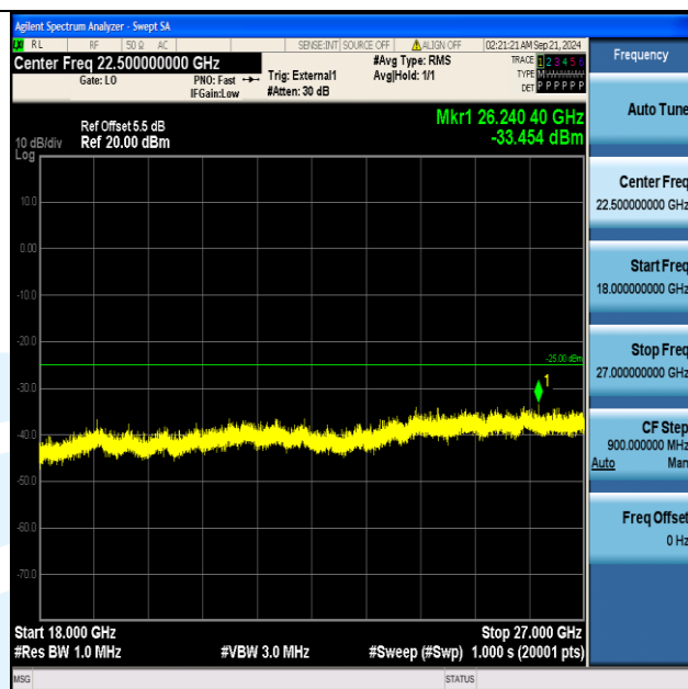
Band38_10MHz_QPSK_38200_1RB#49_18000~27000_18000~27000
