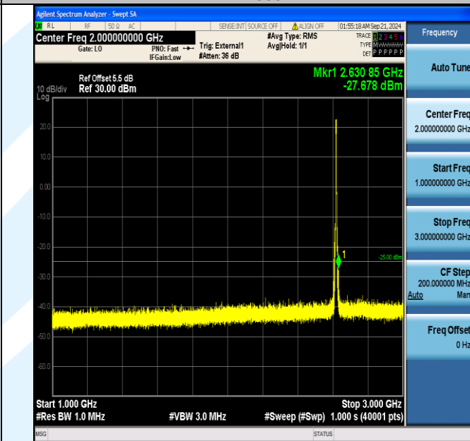
Band38_5MHz_16QAM_38225_25RB#0_1000~3000_1000~3000
