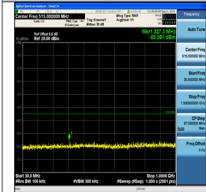
Band38_10MHz_QPSK_37800_1RB#49_30~1000_30~1000
