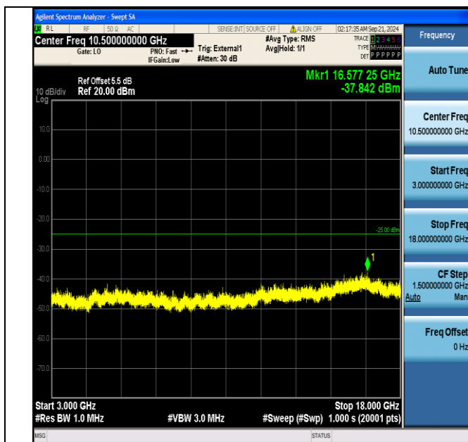
Band38_10MHz_QPSK_38200_1RB#0_3000~18000_3000~18000
