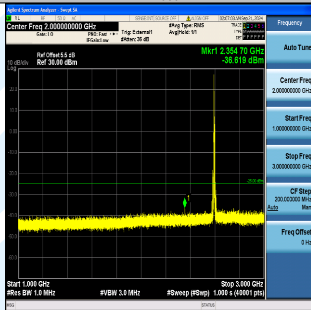
Band38_10MHz_QPSK_38000_1RB#0_1000~3000_1000~3000
