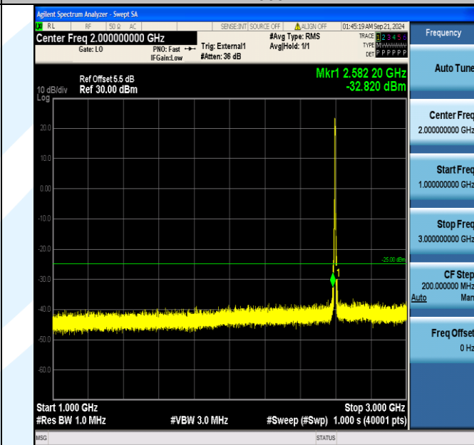
Band38_5MHz_16QAM_38000_25RB#0_1000~3000_1000~3000
