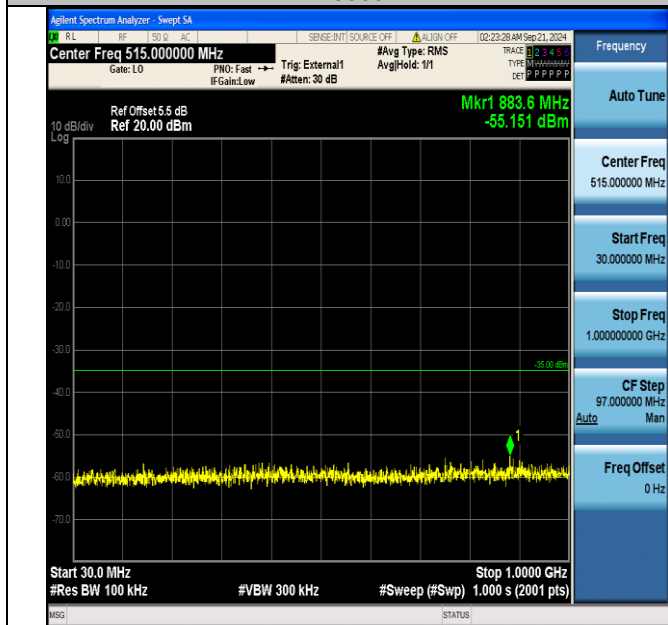
Band38_10MHz_QPSK_38200_50RB#0_30~1000_30~1000
