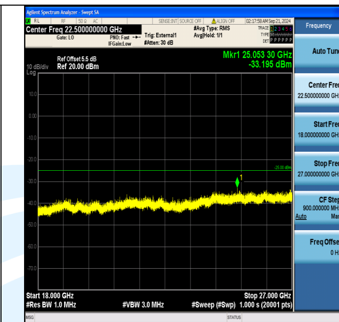
Band38_10MHz_QPSK_38200_1RB#0_18000~27000_18000~27000
