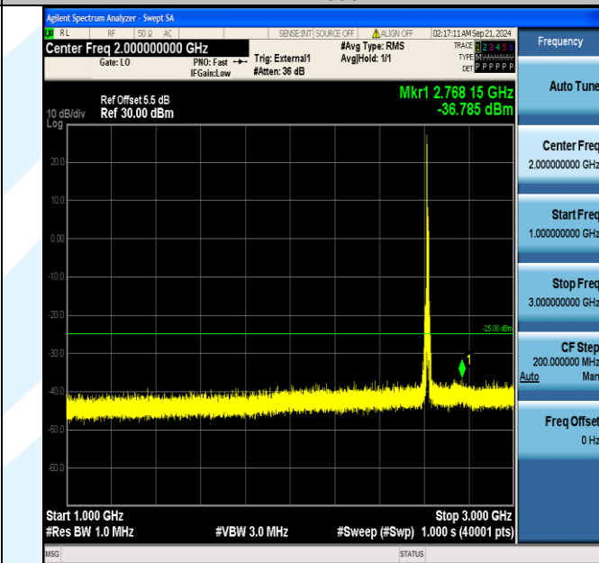
Band38_10MHz_QPSK_38200_1RB#0_1000~3000_1000~3000 0
