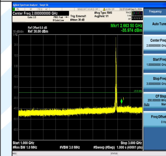
Band38_10MHz_QPSK_37800_1RB#0_1000~3000_1000~3000
