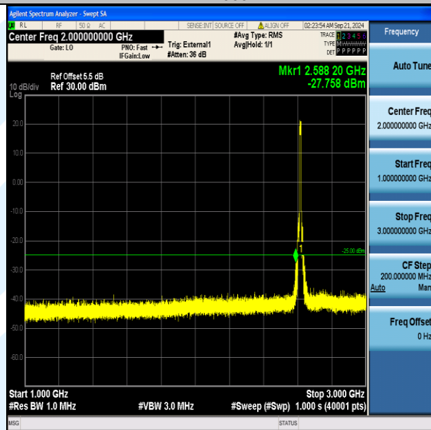
Band38_10MHz_QPSK_38200_50RB#0_1000~3000_1000~3000
