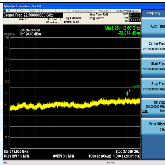
Band38_10MHz_QPSK_37800_50RB#0_18000~27000_18000~27000
