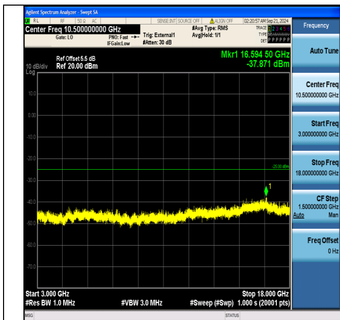
Band38_10MHz_QPSK_38200_1RB#49_3000~18000_3000~18000
