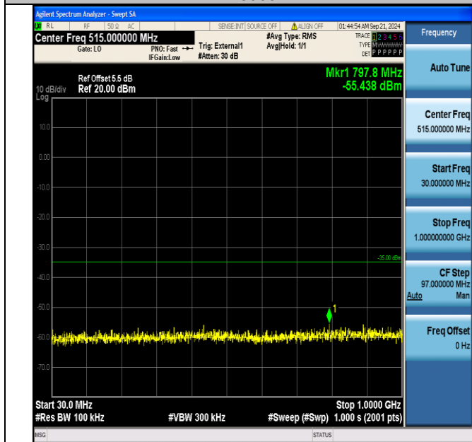
Band38_5MHz_16QAM_38000_25RB#0_30~1000_30~1000
