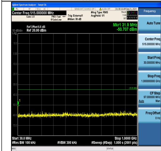
Band38_5MHz_16QAM_38000_1RB#0_30~1000_30~1000
