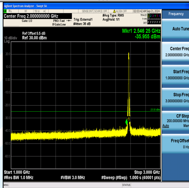
Band38_10MHz_QPSK_37800_50RB#0_1000~3000_1000~3000
