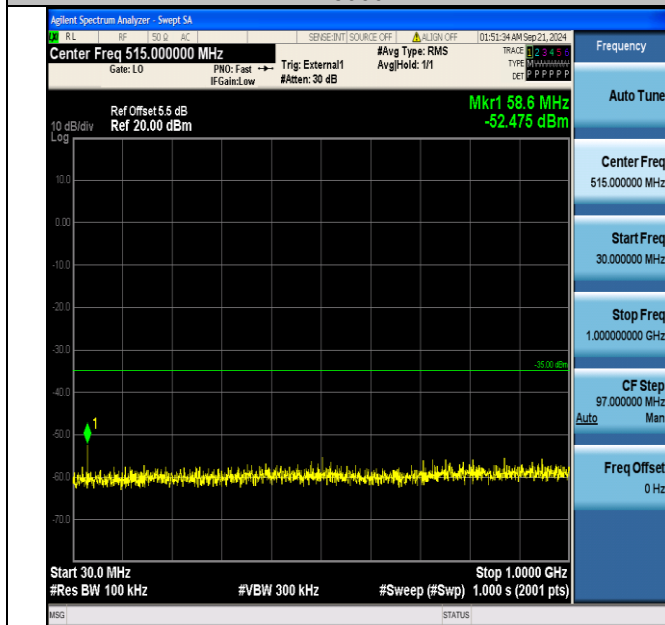
Band38_5MHz_16QAM_38225_1RB#24_30~1000_30~1000
