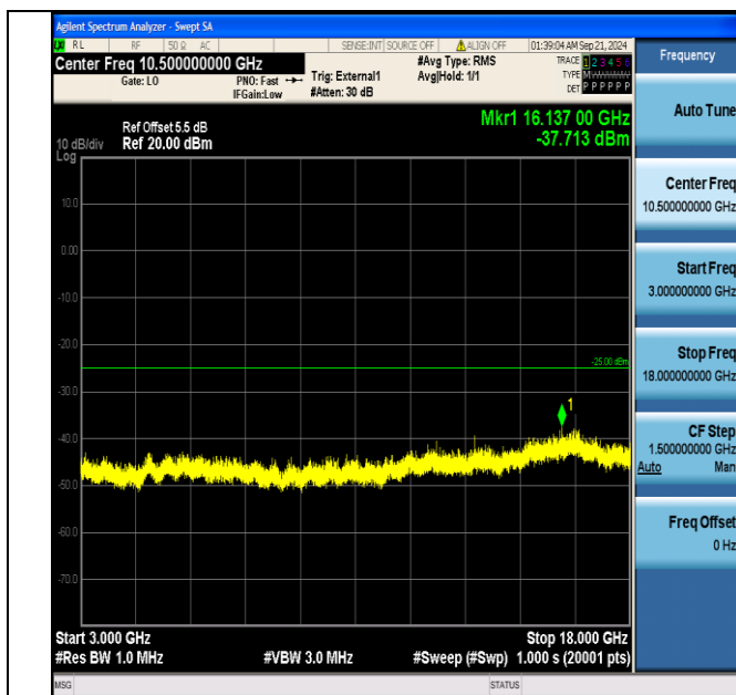
Band38_5MHz_16QAM_38000_1RB#0_3000~18000_3000~18000
