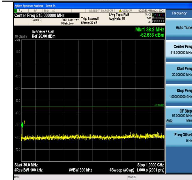
Band38_10MHz_QPSK_38000_1RB#49_30~1000_30~1000
