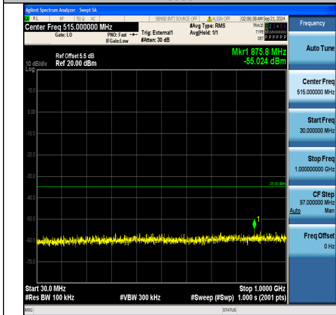
Band38_10MHz_QPSK_38000_1RB#0_30~1000_30~1000
