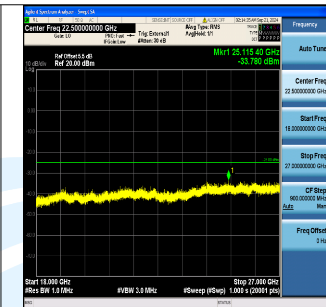
Band38_10MHz_QPSK_38000_50RB#0_18000~27000_18000~27000
