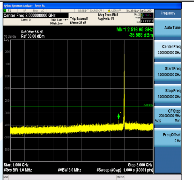
Band38_5MHz_16QAM_38000_1RB#0_1000~3000_1000~3000
