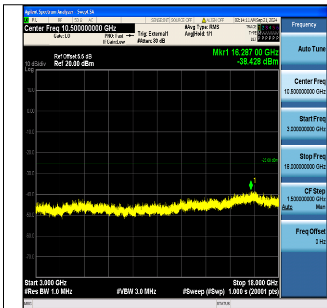
Band38_10MHz_QPSK_38000_50RB#0_3000~18000_3000~18000
