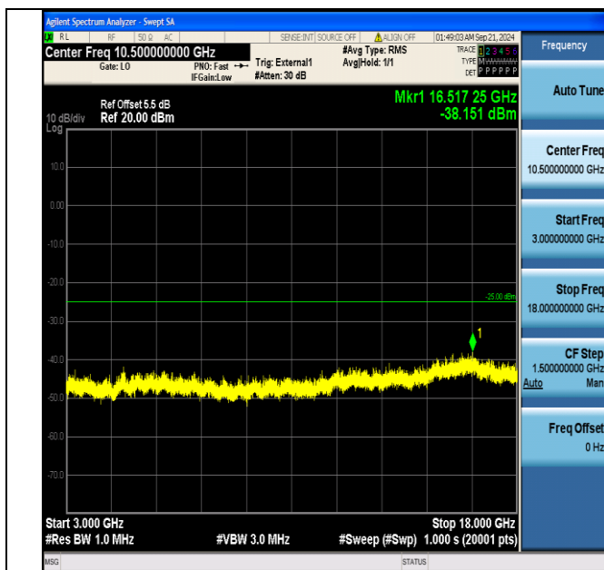
Band38_5MHz_16QAM_38225_1RB#0_3000~18000_3000~18000
