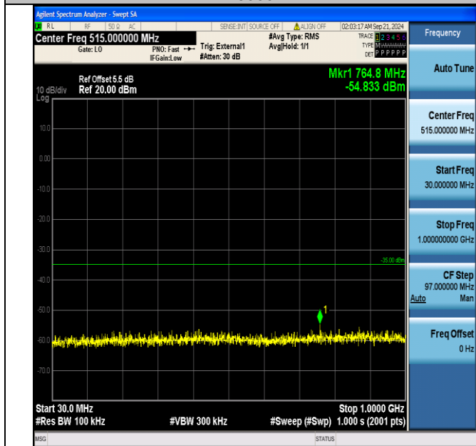
Band38_10MHz_QPSK_37800_50RB#0_30~1000_30~1000
