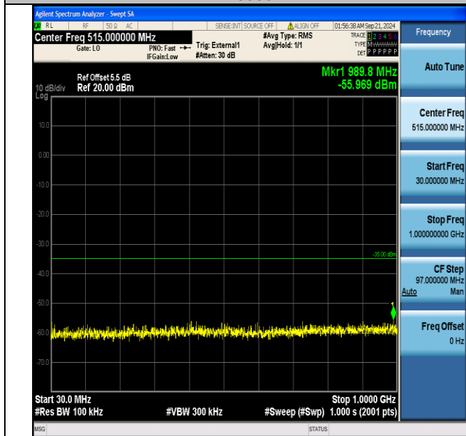
Band38_10MHz_QPSK_37800_1RB#0_30~1000_30~1000
