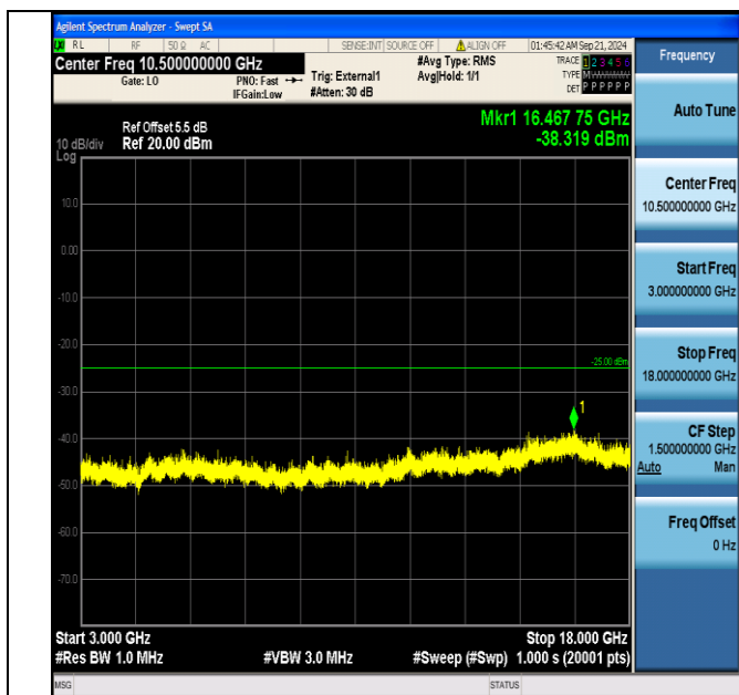
Band38_5MHz_16QAM_38000_25RB#0_3000~18000_3000~18000
