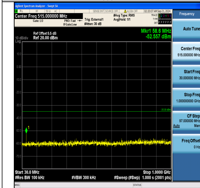
Band38_10MHz_QPSK_38200_1RB#49_30~1000_30~1000
