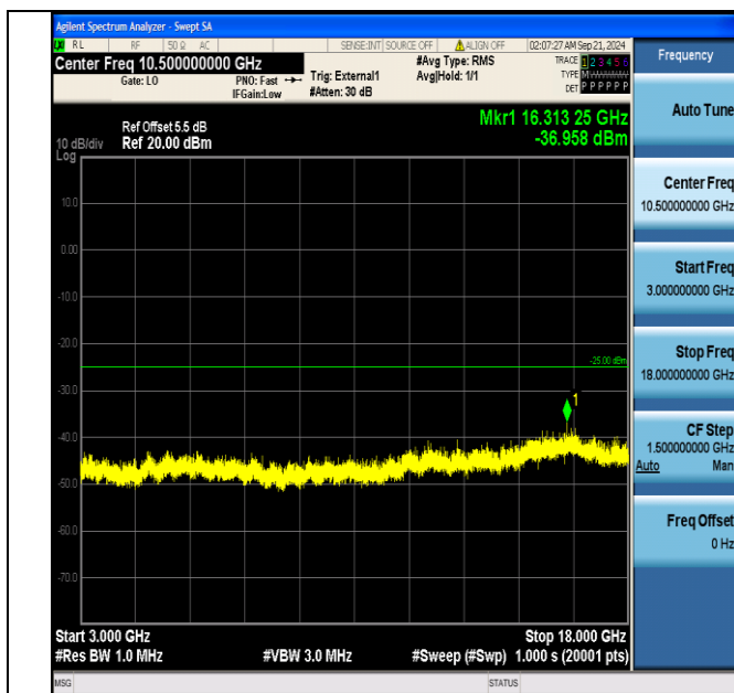
Band38_10MHz_QPSK_38000_1RB#0_3000~18000_3000~18000
