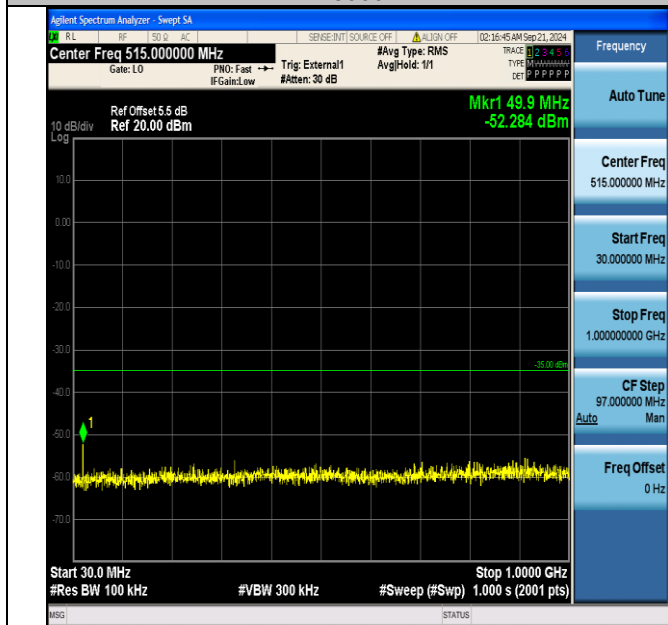
Band38_10MHz_QPSK_38200_1RB#0_30~1000_30~1000
