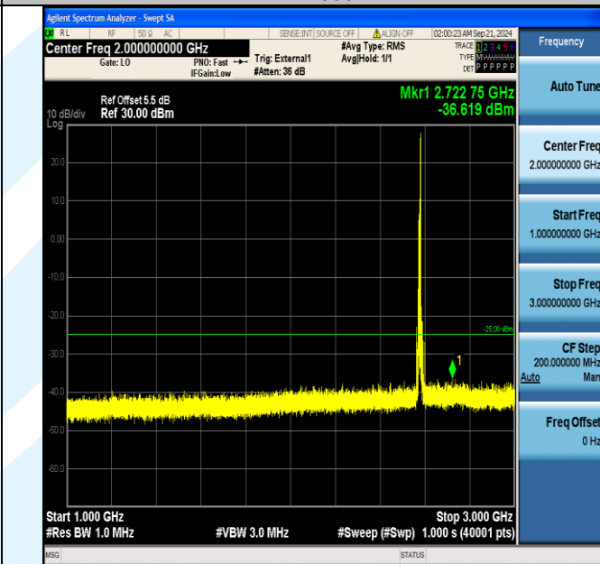
Band38_10MHz_QPSK_37800_1RB#49_1000~3000_1000~3000
