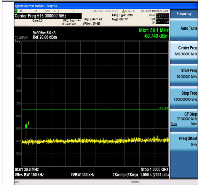
Band38_5MHz_QPSK_38225_1RB#24_30~1000_30~1000
