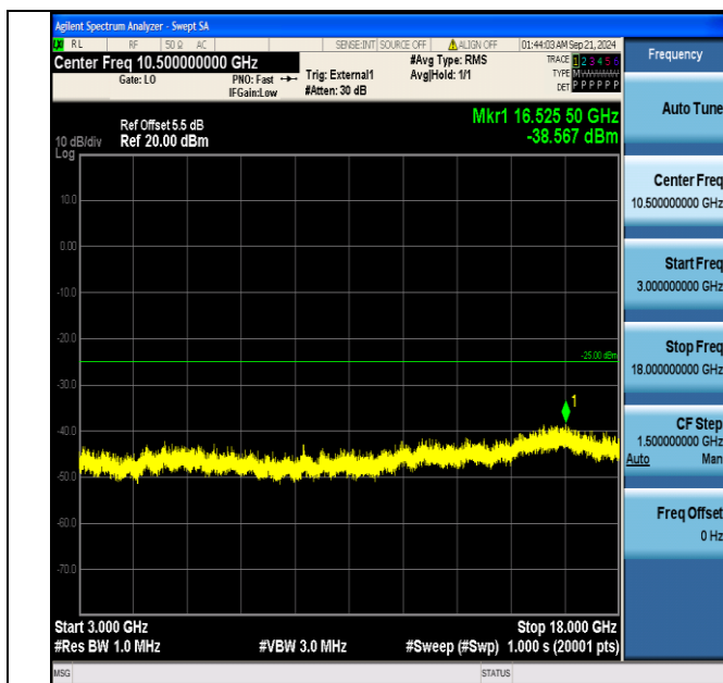
Band38_5MHz_QPSK_38000_25RB#0_3000~18000_3000~18000
