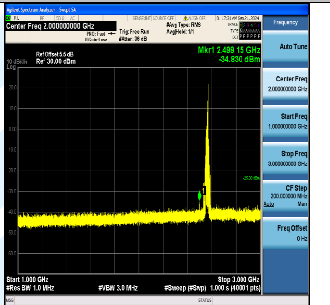
Band7_20MHz_16QAM_21350_1RB#99_1000~3000_1000~3000
