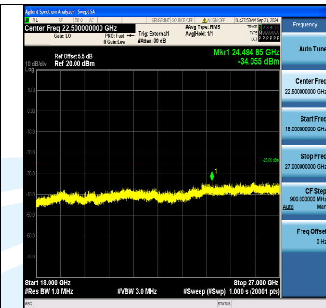
Band38_5MHz_QPSK_37775_1RB#0_18000~27000_18000~27000
