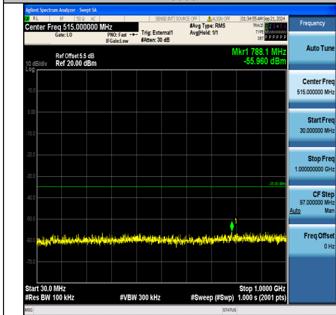
Band38_5MHz_16QAM_37775_25RB#0_30~1000_30~1000
