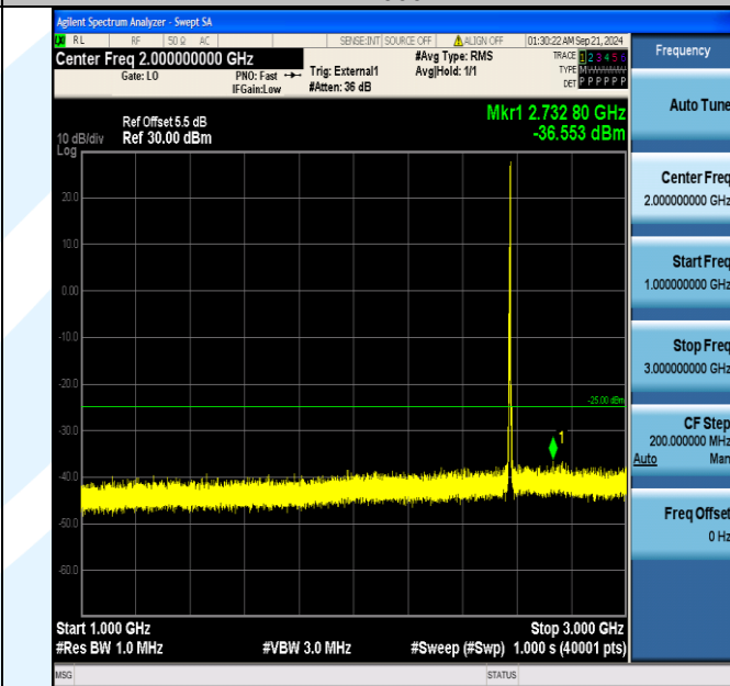
Band38_5MHz_QPSK_37775_1RB#24_1000~3000_1000~3000
