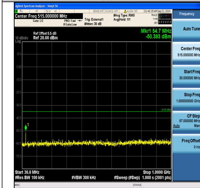
Band38_5MHz_QPSK_38225_1RB#0_30~1000_30~1000
