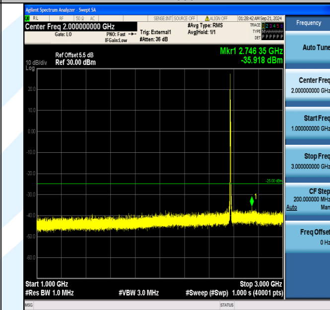
Band38_5MHz_16QAM_37775_1RB#0_1000~3000_1000~3000
