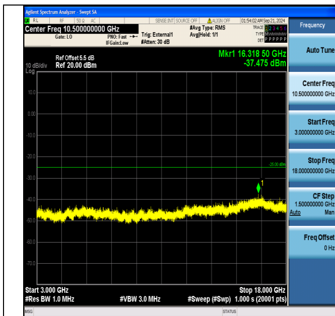
Band38_5MHz_QPSK_38225_25RB#0_3000~18000_3000~18000
