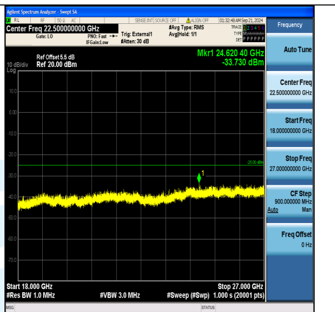
Band38_5MHz_16QAM_37775_1RB#24_18000~27000_18000~27000
