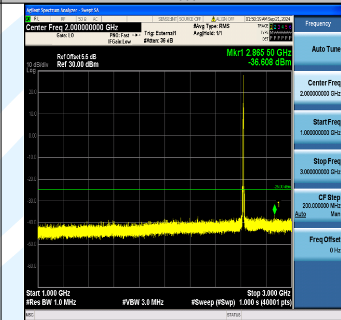
Band38_5MHz_QPSK_38225_1RB#24_1000~3000_1000~3000
