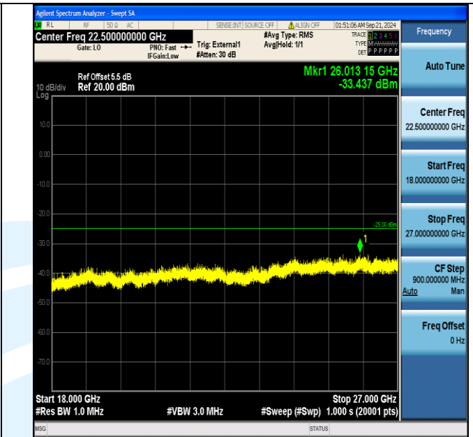
Band38_5MHz_QPSK_38225_1RB#24_18000~27000_18000~27000
