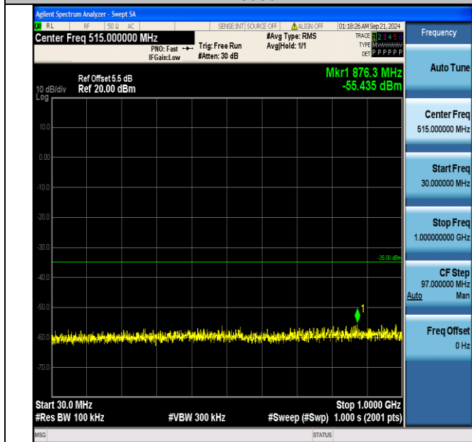
Band7_20MHz_16QAM_21350_100RB#0_30~1000_30~1000
