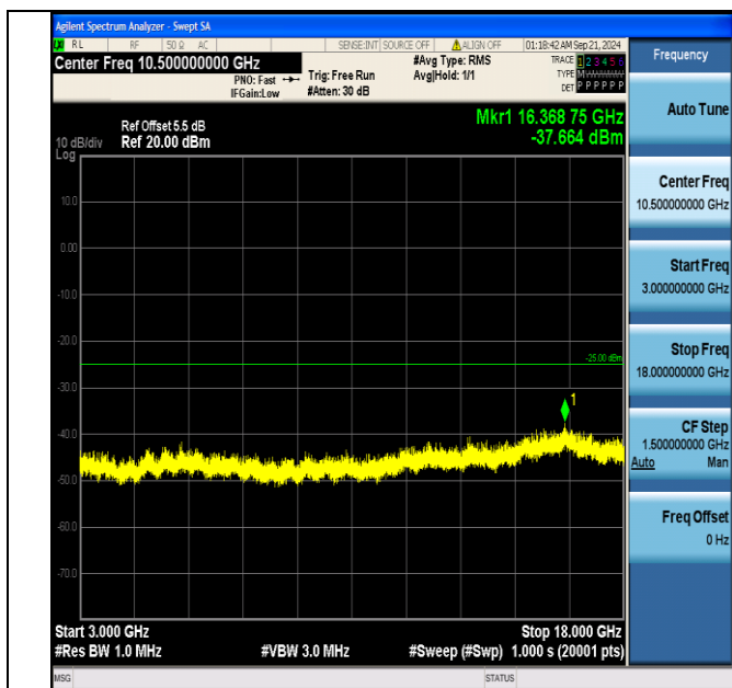
Band7_20MHz_16QAM_21350_100RB#0_3000~18000_3000~18000
