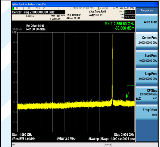
Band38_5MHz_QPSK_38225_25RB#0_1000~3000_1000~3000
