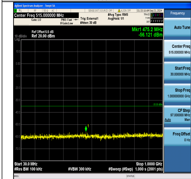
Band38_5MHz_QPSK_37775_25RB#0_30~1000_30~1000
