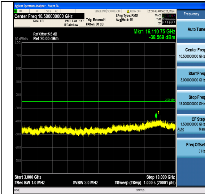
Band38_5MHz_QPSK_38225_1RB#24_3000~18000_3000~18000
