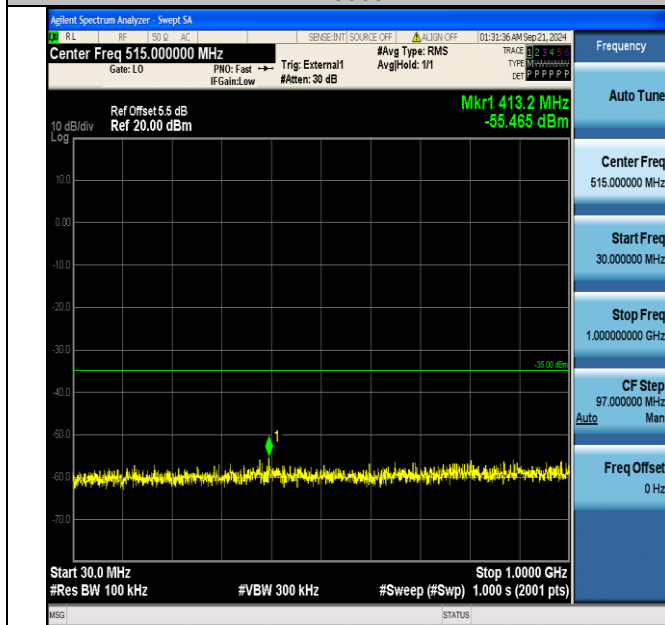
Band38_5MHz_16QAM_37775_1RB#24_30~1000_30~1000
