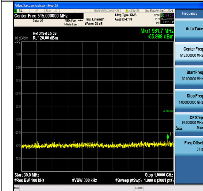
Band38_5MHz_QPSK_38225_25RB#0_30~1000_30~1000
