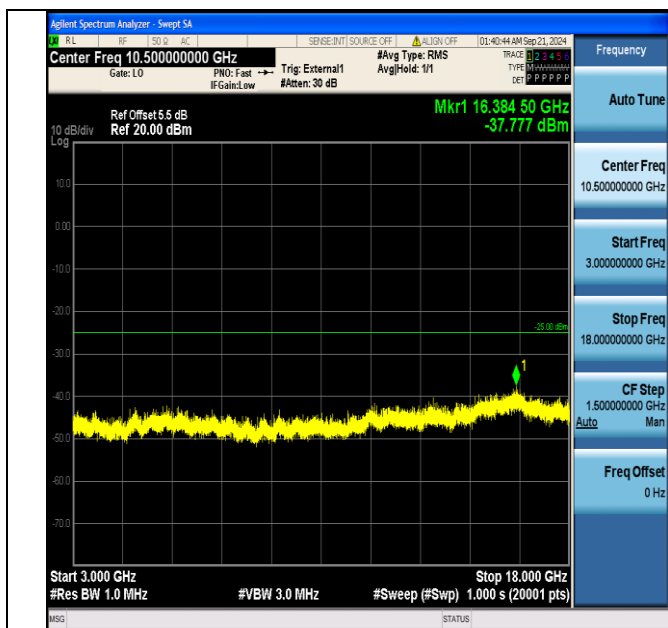
Band38_5MHz_QPSK_38000_1RB#24_3000~18000_3000~18000
