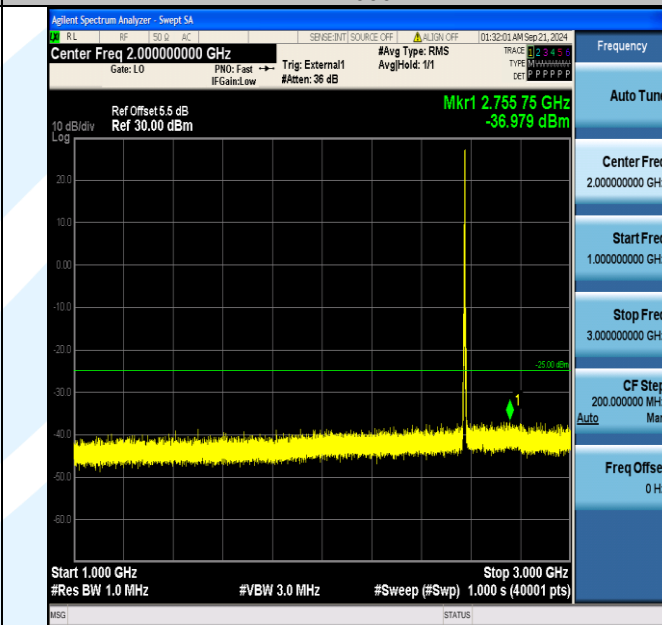
Band38_5MHz_16QAM_37775_1RB#24_1000~3000_1000~3000
