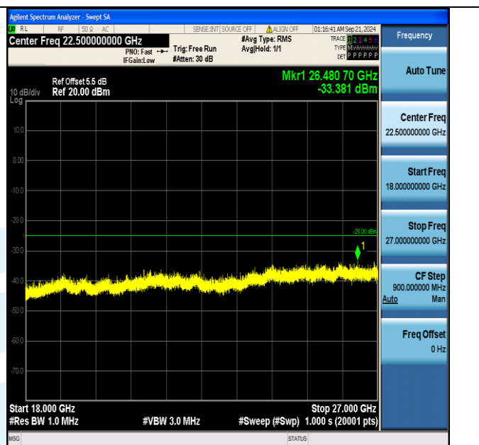
Band7_20MHz_16QAM_21350_1RB#0_18000~27000_18000~27000
