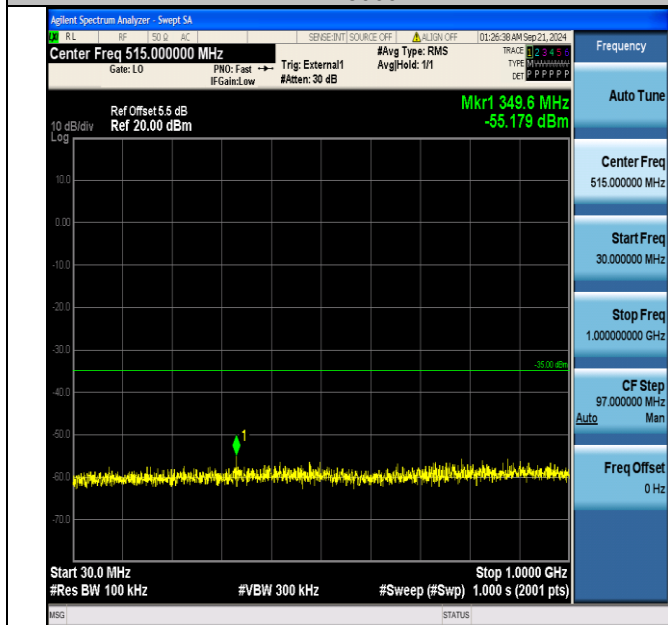
Band38_5MHz_QPSK_37775_1RB#0_30~1000_30~1000
