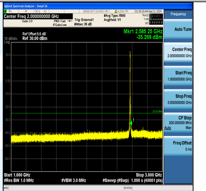
Band38_5MHz_16QAM_37775_25RB#0_1000~3000_1000~3000
