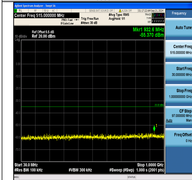
Band7_20MHz_16QAM_21350_1RB#99_30~1000_30~1000
