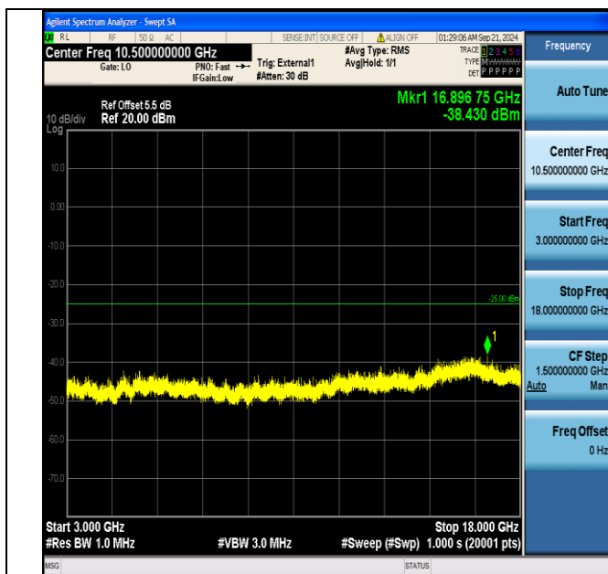
Band38_5MHz_16QAM_37775_1RB#0_3000~18000_3000~18000
