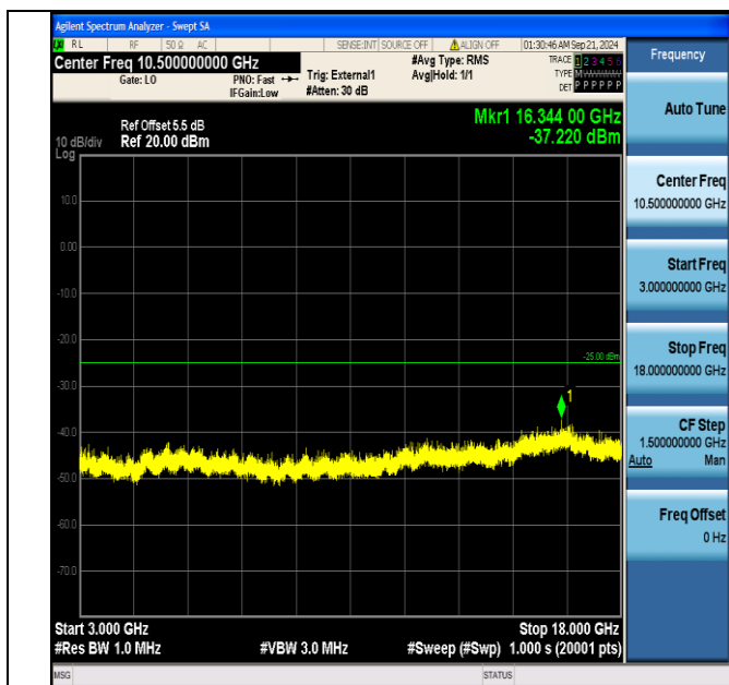
Band38_5MHz_QPSK_37775_1RB#24_3000~18000_3000~18000
