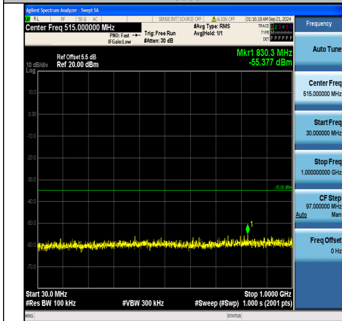
Band7_20MHz_16QAM_21350_1RB#0_30~1000_30~1000
