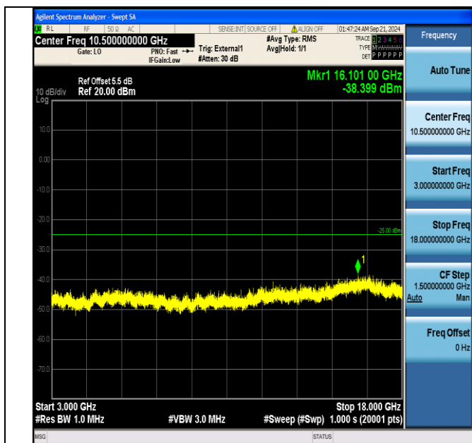
Band38_5MHz_QPSK_38225_1RB#0_3000~18000_3000~18000
