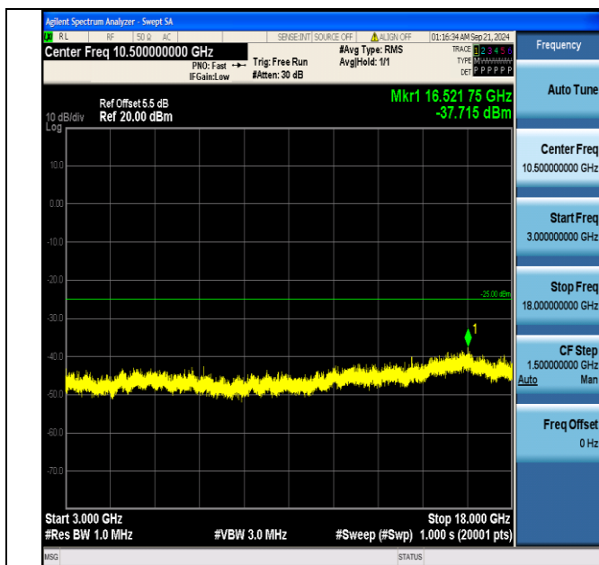
Band7_20MHz_16QAM_21350_1RB#0_3000~18000_3000~18000
