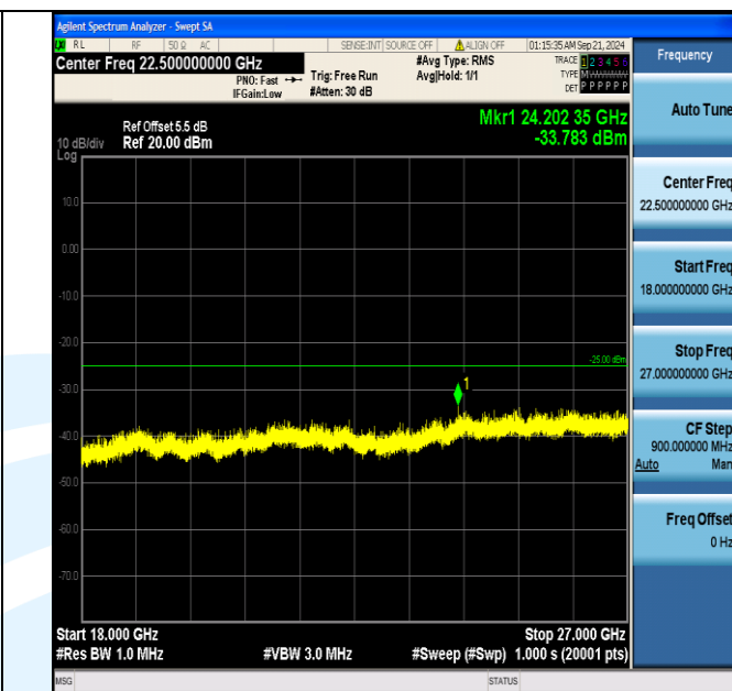
Band7_20MHz_16QAM_21100_100RB#0_18000~27000_18000~27000
