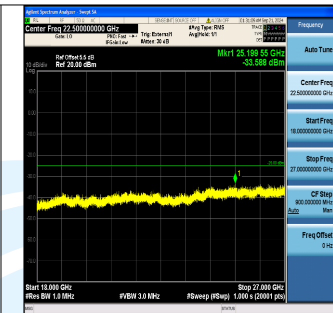
Band38_5MHz_QPSK_37775_1RB#24_18000~27000_18000~27000
