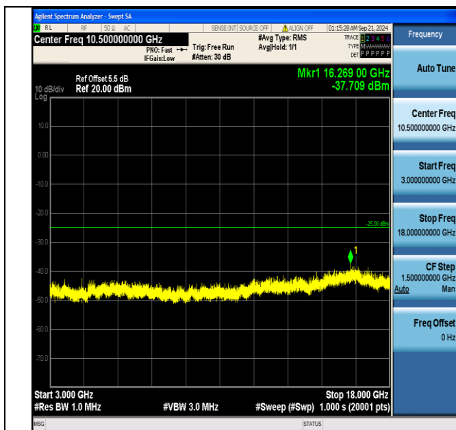
Band7_20MHz_16QAM_21100_100RB#0_3000~18000_3000~18000
