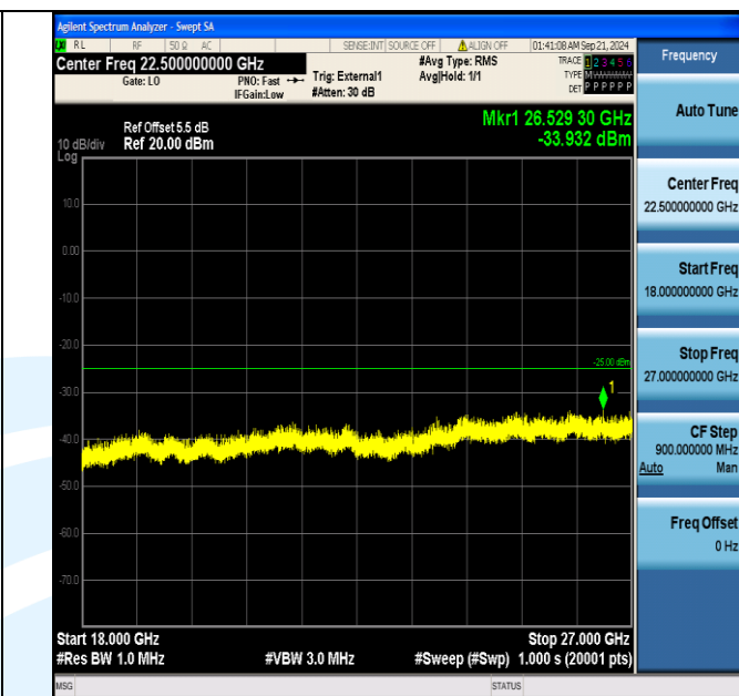
Band38_5MHz_QPSK_38000_1RB#24_18000~27000_18000~27000
