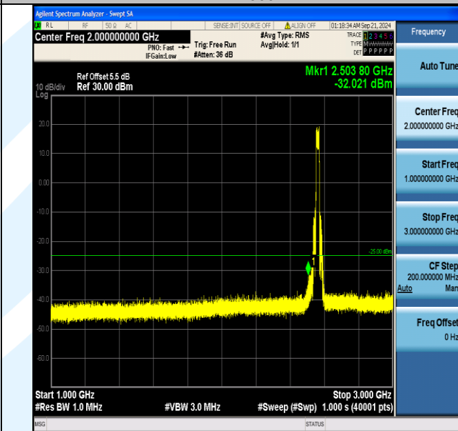
Band7_20MHz_16QAM_21350_100RB#0_1000~3000_1000~3000
