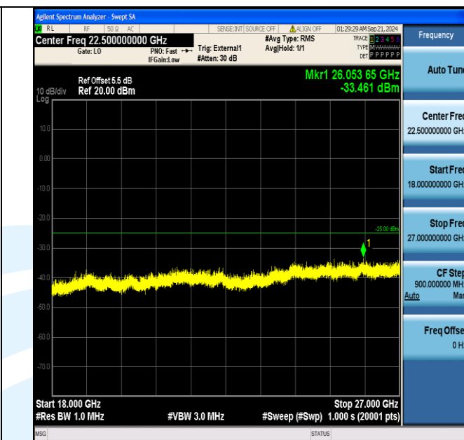
Band38_5MHz_16QAM_37775_1RB#0_18000~27000_18000~27000
