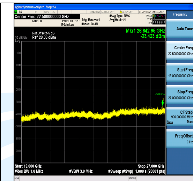
Band38_5MHz_QPSK_38000_1RB#0_18000~27000_18000~27000
