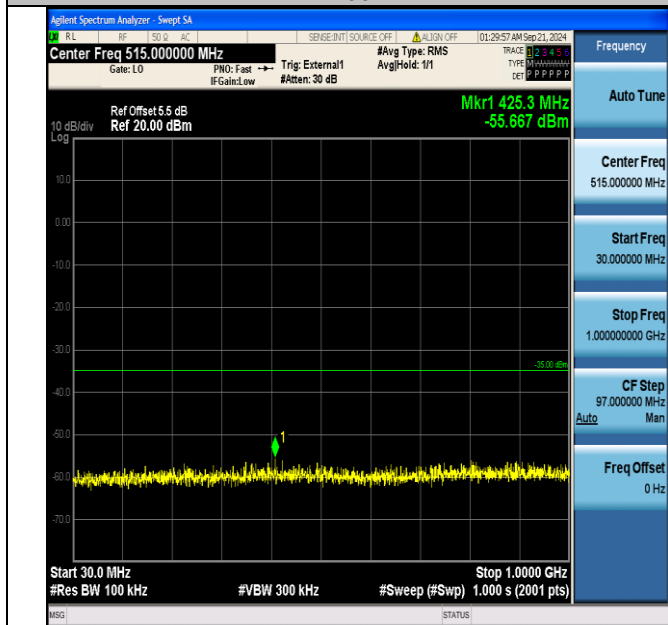
Band38_5MHz_QPSK_37775_1RB#24_30~1000_30~1000
