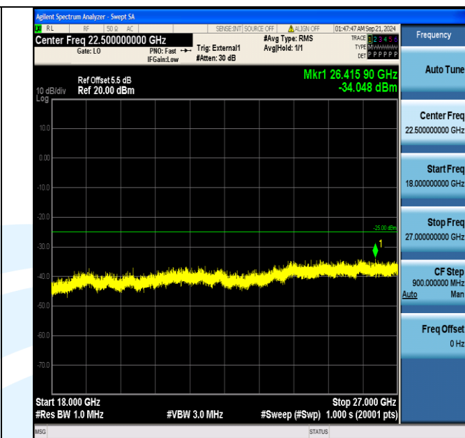
Band38_5MHz_QPSK_38225_1RB#0_18000~27000_18000~27000
