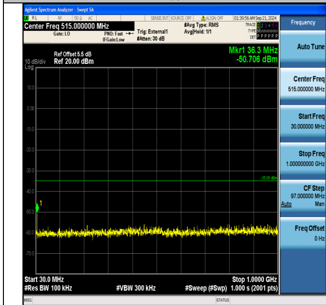
Band38_5MHz_QPSK_38000_1RB#24_30~1000_30~1000
