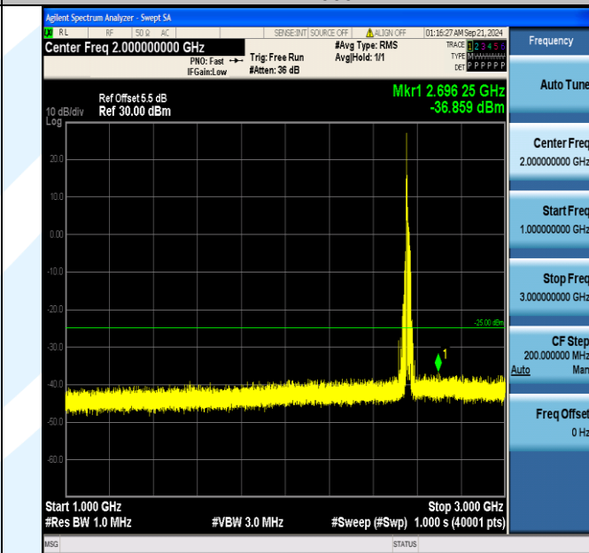
Band7_20MHz_16QAM_21350_1RB#0_1000~3000_1000~3000 0
