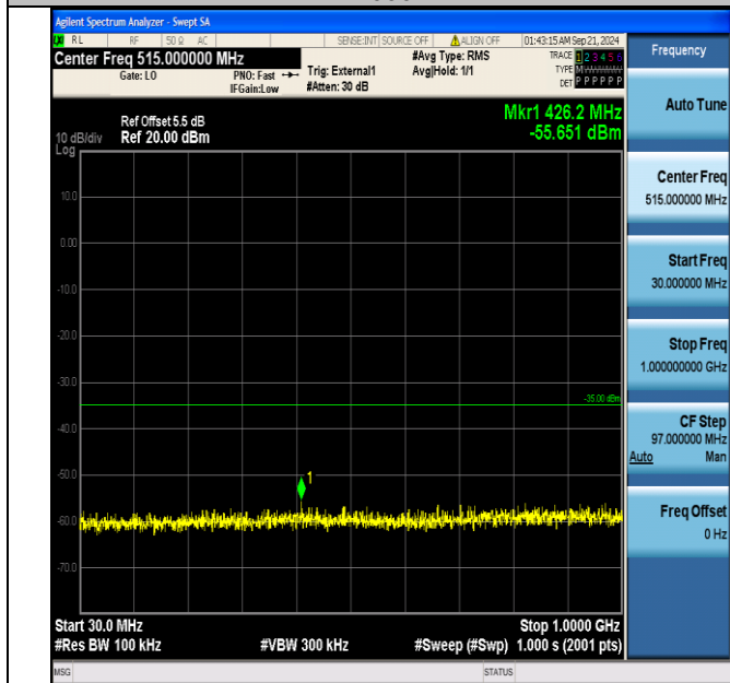
Band38_5MHz_QPSK_38000_25RB#0_30~1000_30~1000
