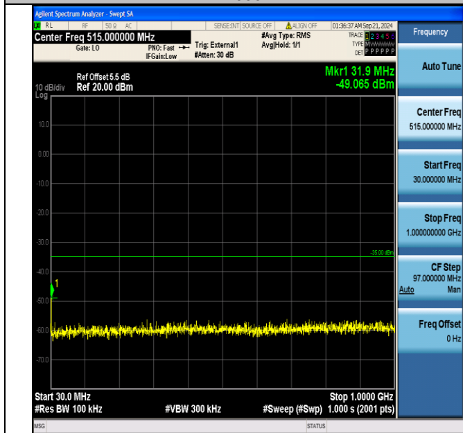
Band38_5MHz_QPSK_38000_1RB#0_30~1000_30~1000
