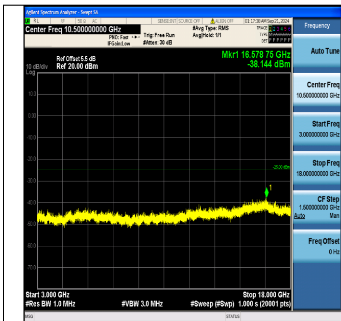
Band7_20MHz_16QAM_21350_1RB#99_3000~18000_3000~18000
