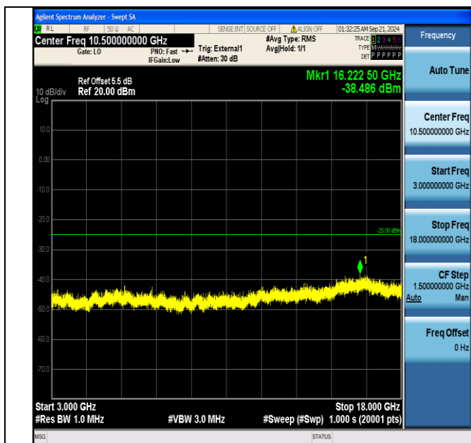
Band38_5MHz_16QAM_37775_1RB#24_3000~18000_3000~18000
