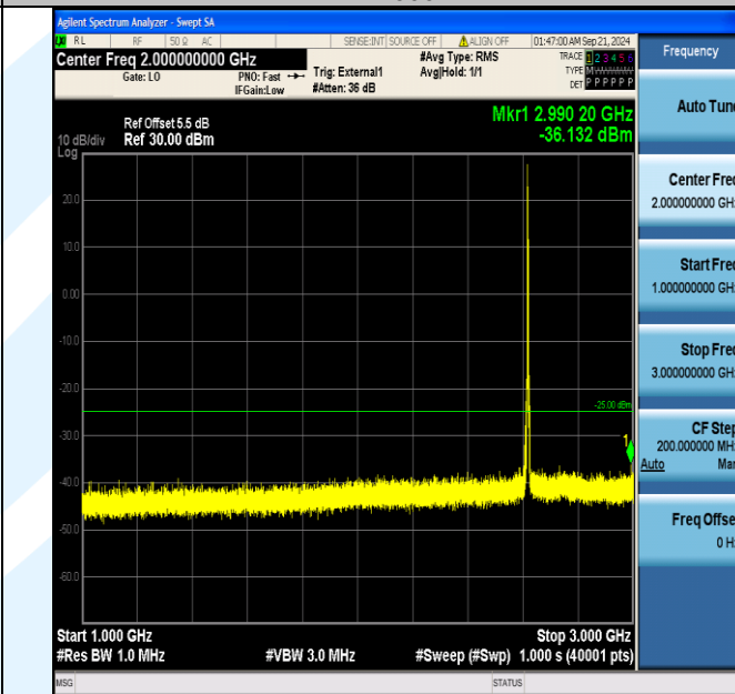
Band38_5MHz_QPSK_38225_1RB#0_1000~3000_1000~3000
