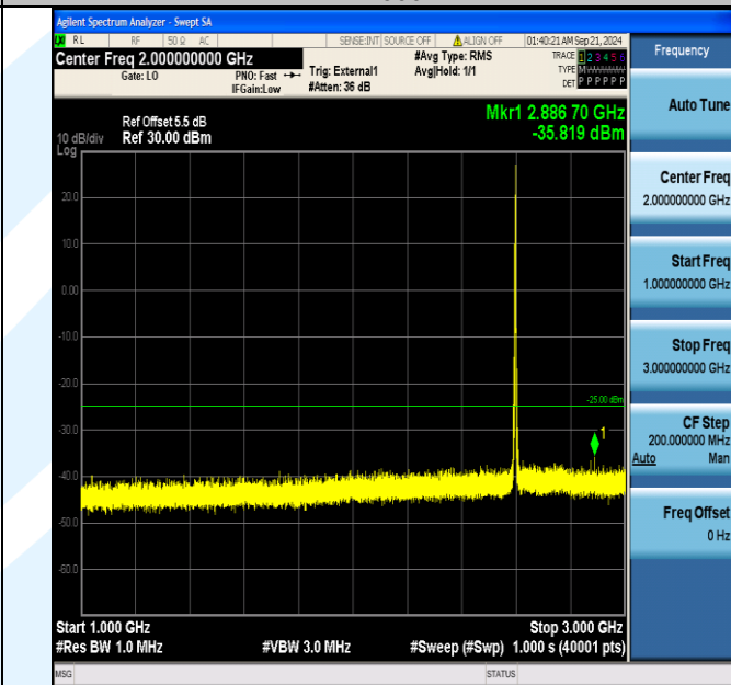
Band38_5MHz_QPSK_38000_1RB#24_1000~3000_1000~3000
