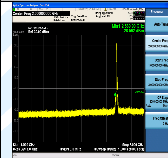
Band7_10MHz_16QAM_21400_50RB#0_1000~3000_1000~3000
