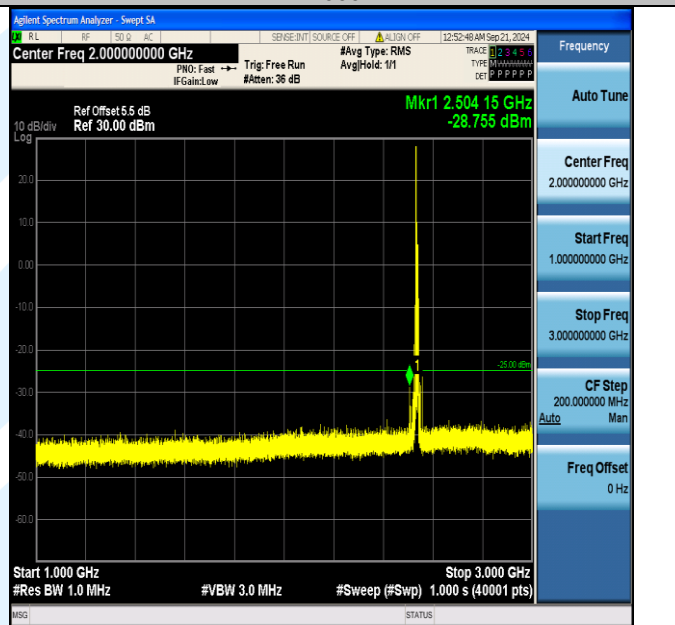
Band7_10MHz_16QAM_21100_1RB#0_1000~3000_1000~3000
