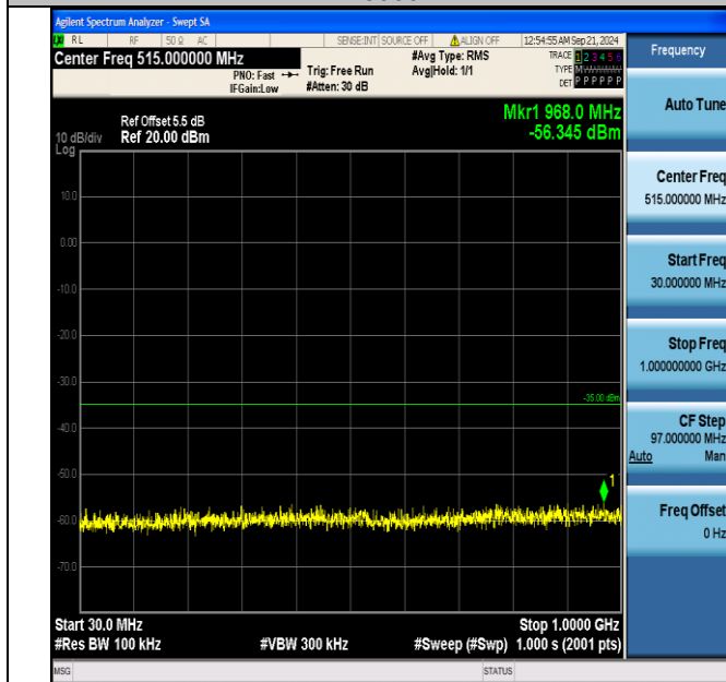
Band7_10MHz_16QAM_21100_50RB#0_30~1000_30~1000
