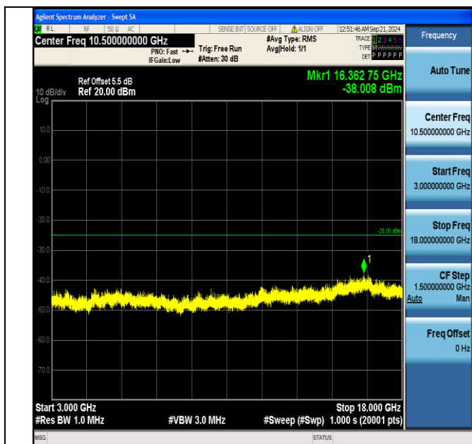
Band7_10MHz_16QAM_20800_50RB#0_3000~18000_3000~18000
