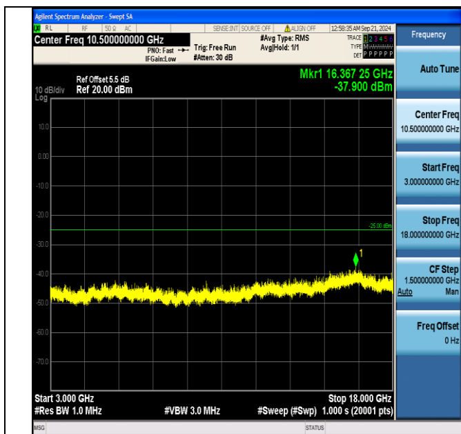
Band7_10MHz_16QAM_21400_50RB#0_3000~18000_3000~18000
