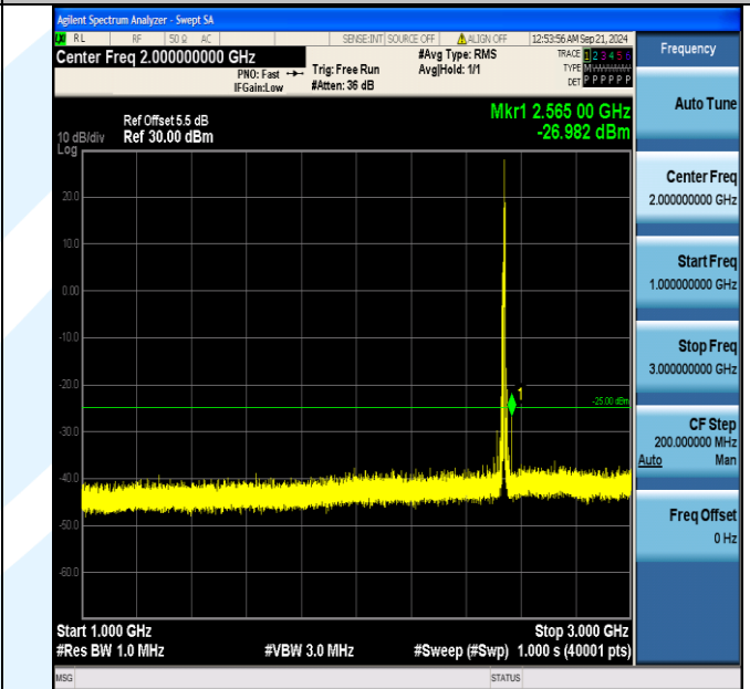
Band7_10MHz_16QAM_21100_1RB#49_1000~3000_1000~3000
