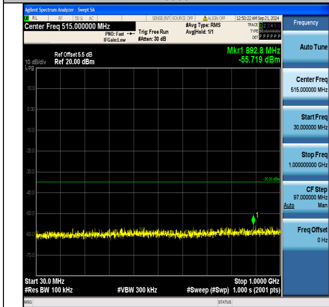
Band7_10MHz_16QAM_20800_1RB#49_30~1000_30~1000
