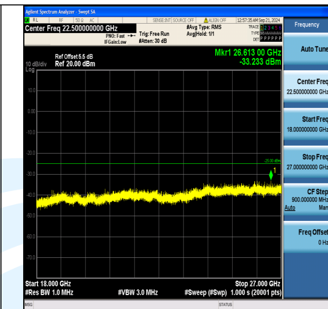
Band7_10MHz_16QAM_21400_1RB#49_18000~27000_18000~27000
