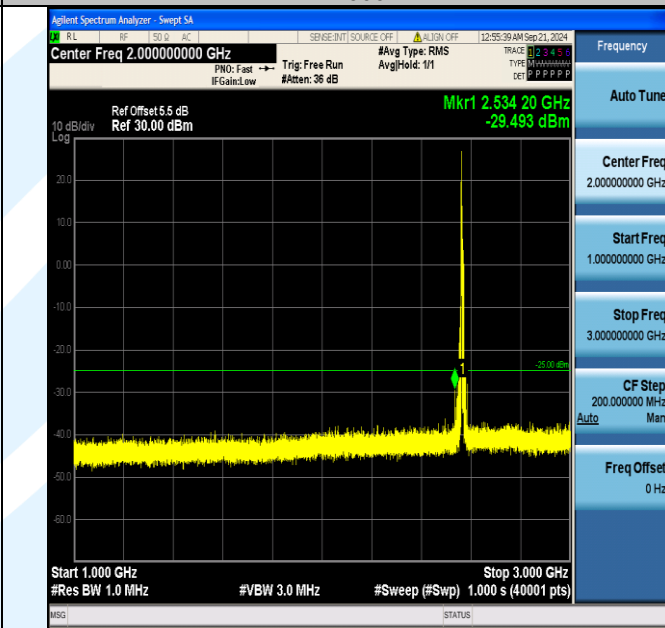
Band7_10MHz_QPSK_21400_1RB#0_1000~3000_1000~3000
