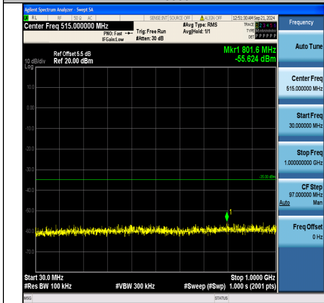
Band7_10MHz_16QAM_20800_50RB#0_30~1000_30~1000
