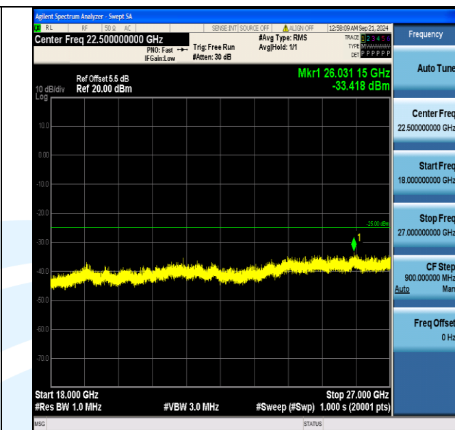
Band7_10MHz_QPSK_21400_50RB#0_18000~27000_18000~27000
