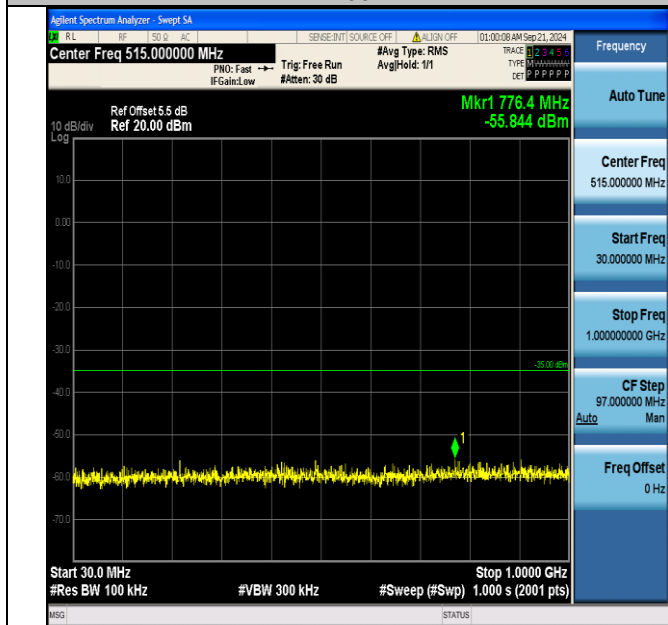
Band7_15MHz_QPSK_20825_1RB#74_30~1000_30~1000
