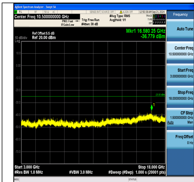
Band7_10MHz_16QAM_20800_1RB#49_3000~18000_3000~18000
