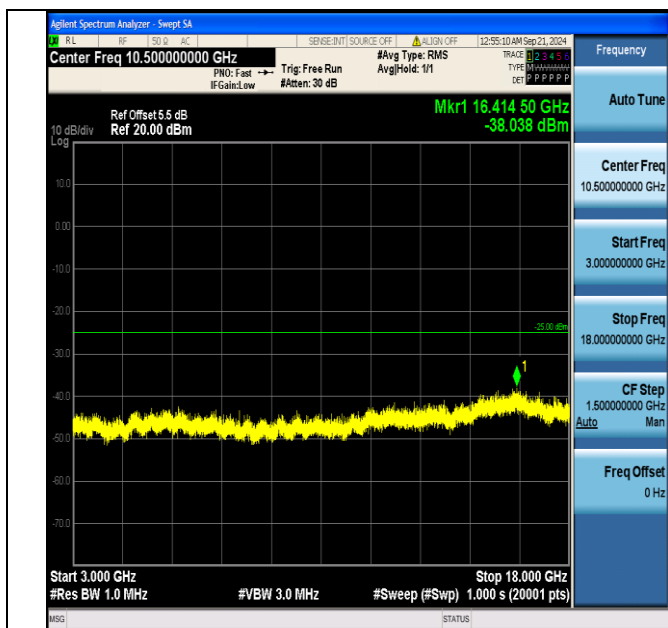
Band7_10MHz_16QAM_21100_50RB#0_3000~18000_3000~18000
