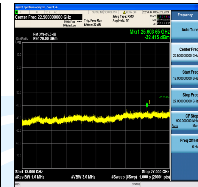
Band7_10MHz_QPSK_21100_50RB#0_18000~27000_18000~27000
