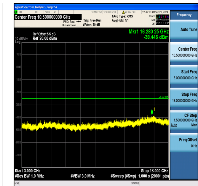
Band7_10MHz_16QAM_20800_1RB#0_3000~18000_3000~18000
