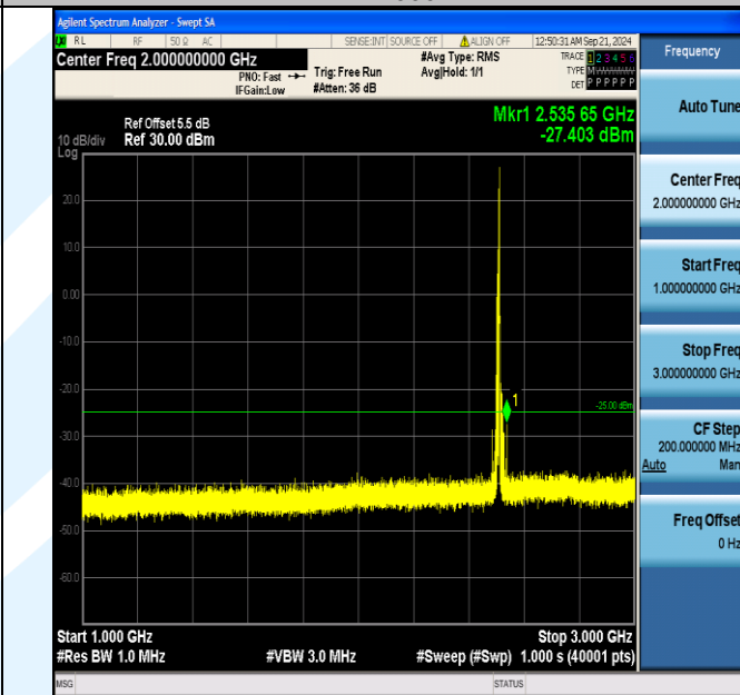
Band7_10MHz_16QAM_20800_1RB#49_1000~3000_1000~3000
