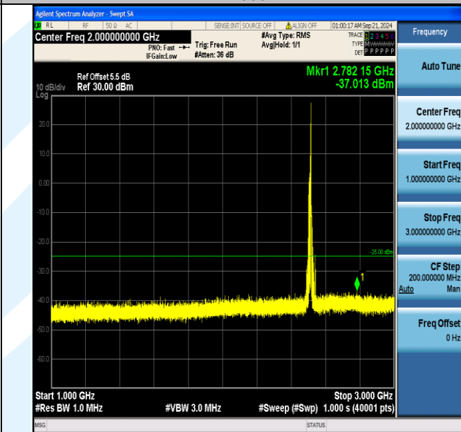
Band7_15MHz_QPSK_20825_1RB#74_1000~3000_1000~3000
