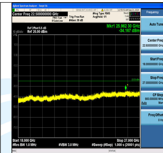
Band7_10MHz_QPSK_21400_1RB#0_18000~27000_18000~27000
