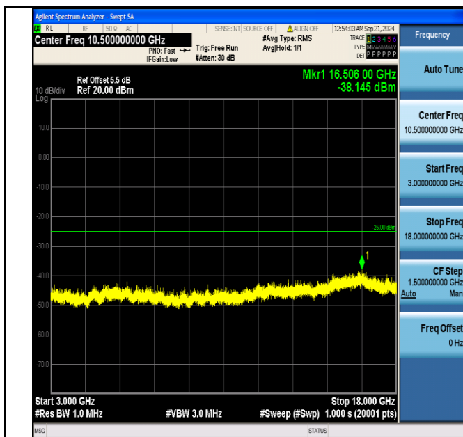
Band7_10MHz_16QAM_21100_1RB#49_3000~18000_3000~18000
