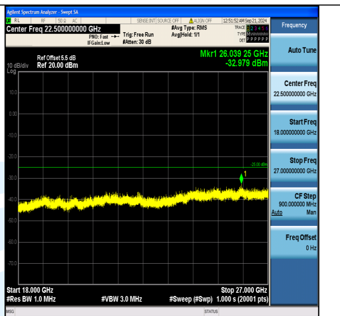
Band7_10MHz_16QAM_20800_50RB#0_18000~27000_18000~27000
