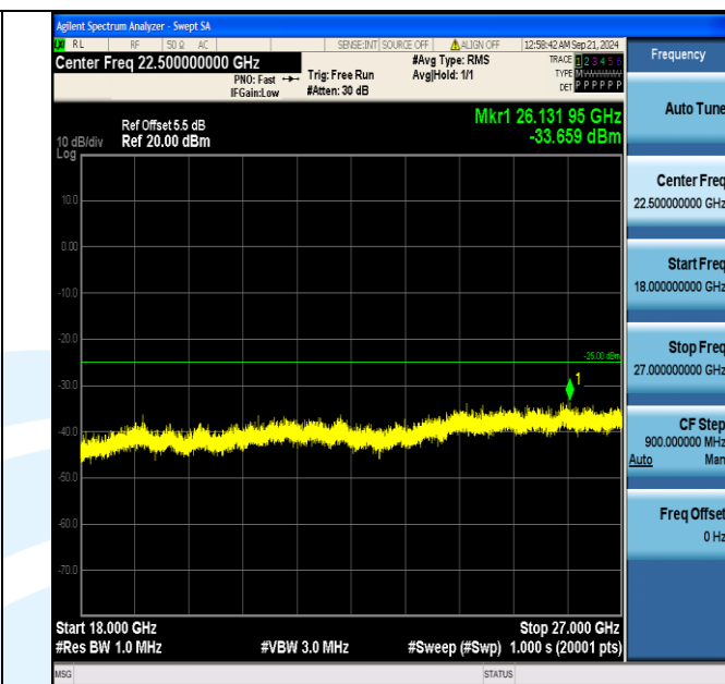
Band7_10MHz_16QAM_21400_50RB#0_18000~27000_18000~27000
