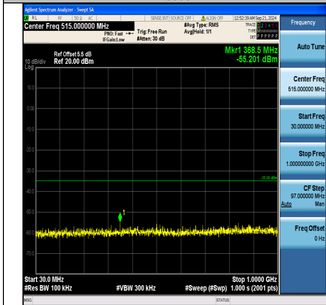
Band7_10MHz_16QAM_21100_1RB#0_30~1000_30~1000
