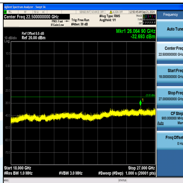
Band7_10MHz_16QAM_20800_1RB#49_18000~27000_18000~27000
