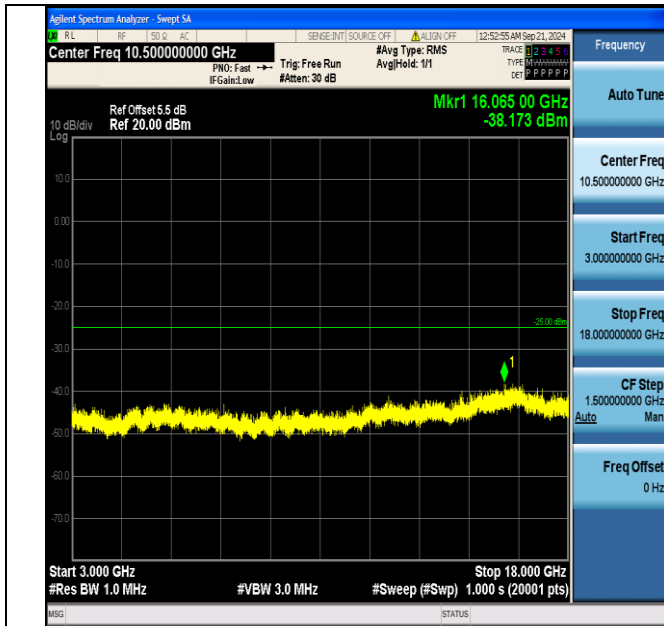
Band7_10MHz_16QAM_21100_1RB#0_3000~18000_3000~18000
