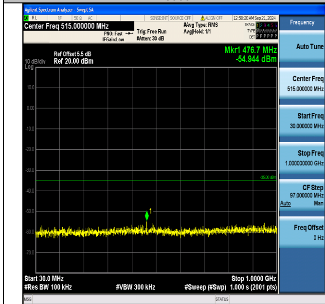
Band7_10MHz_16QAM_21400_50RB#0_30~1000_30~1000
