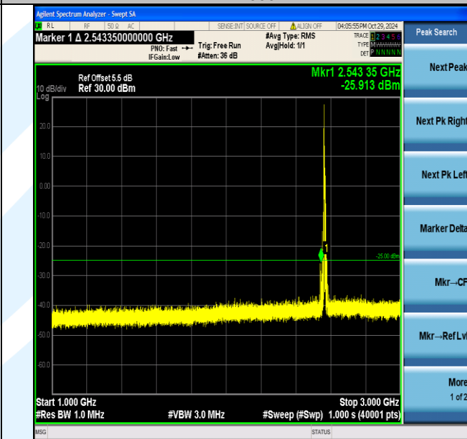
Band7_10MHz_16QAM_21400_1RB#0_1000~3000_1000~3000
