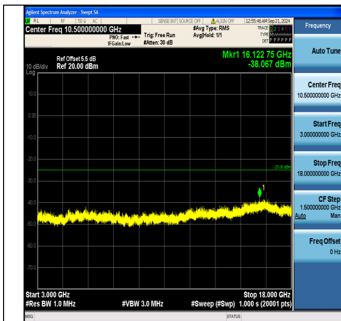
Band7_10MHz_QPSK_21400_1RB#0_3000~18000_3000~18000
