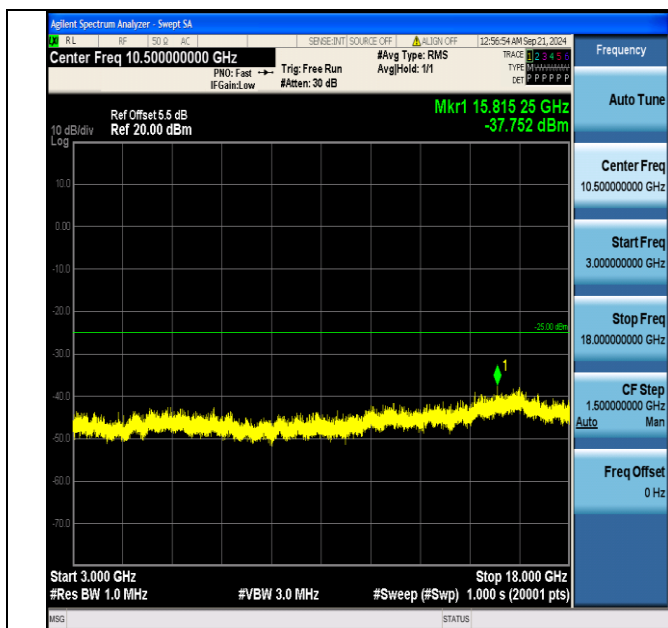
Band7_10MHz_QPSK_21400_1RB#49_3000~18000_3000~18000
