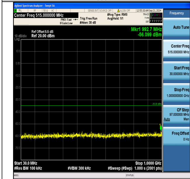
Band7_10MHz_QPSK_21400_1RB#0_30~1000_30~1000
