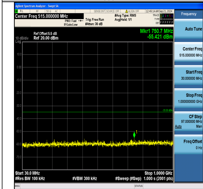
Band7_10MHz_16QAM_20800_1RB#0_30~1000_30~1000
