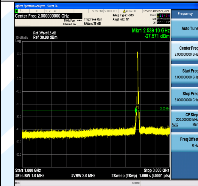
Band7_10MHz_QPSK_21400_50RB#0_1000~3000_1000~3000
