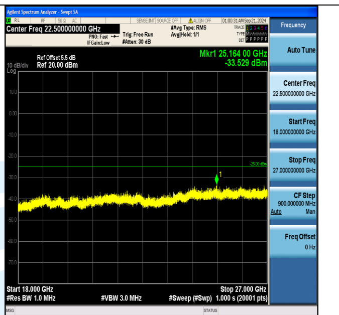
Band7_15MHz_QPSK_20825_1RB#74_18000~27000_18000~27000
