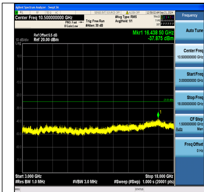
Band7_10MHz_QPSK_21400_50RB#0_3000~18000_3000~18000
