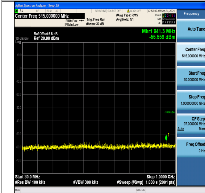
Band7_10MHz_16QAM_21100_1RB#49_30~1000_30~1000
