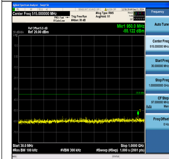
Band7_10MHz_QPSK_21400_1RB#49_30~1000_30~1000
