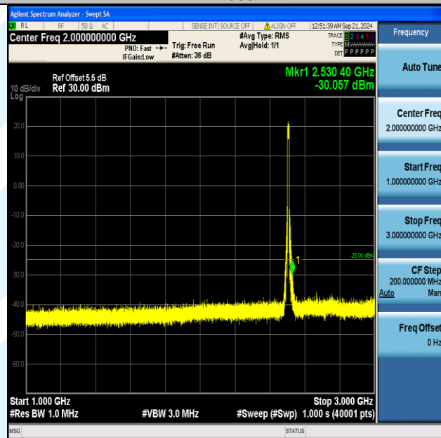
Band7_10MHz_16QAM_20800_50RB#0_1000~3000_1000~3000
