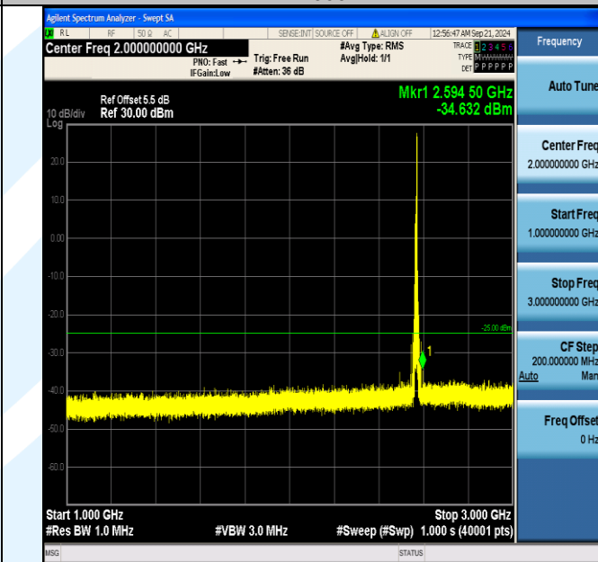
Band7_10MHz_QPSK_21400_1RB#49_1000~3000_1000~3000
