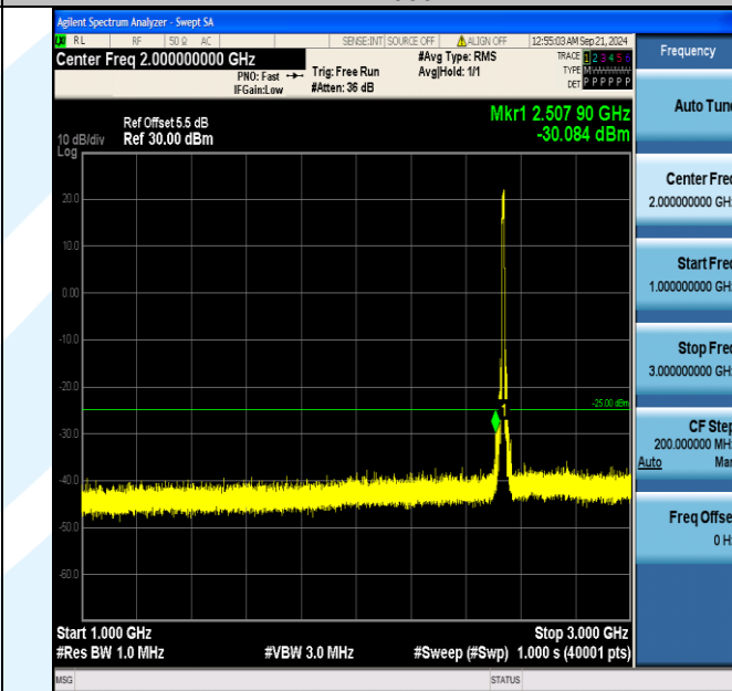
Band7_10MHz_16QAM_21100_50RB#0_1000~3000_1000~3000
