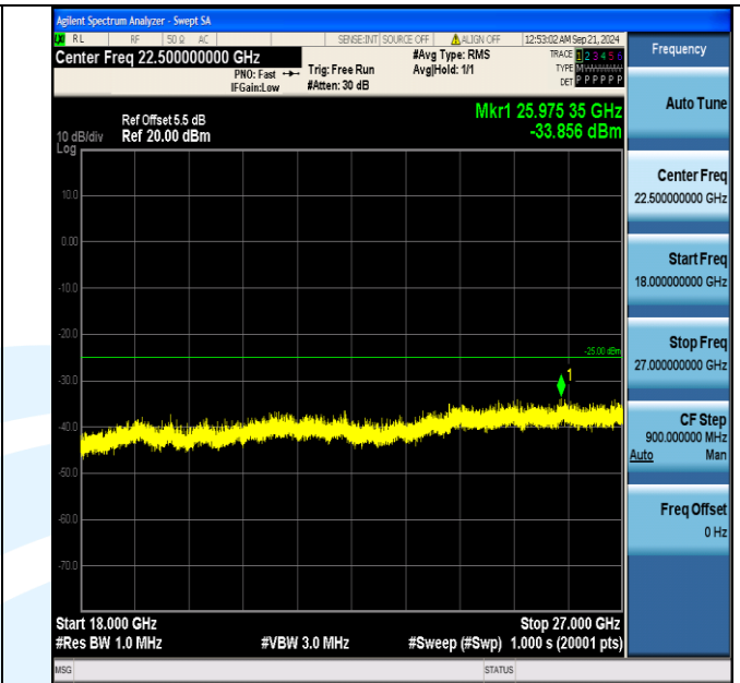
Band7_10MHz_16QAM_21100_1RB#0_18000~27000_18000~27000
