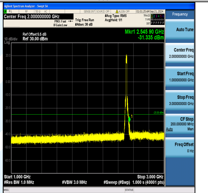
Band7_15MHz_QPSK_20825_75RB#0_1000~3000_1000~3000
