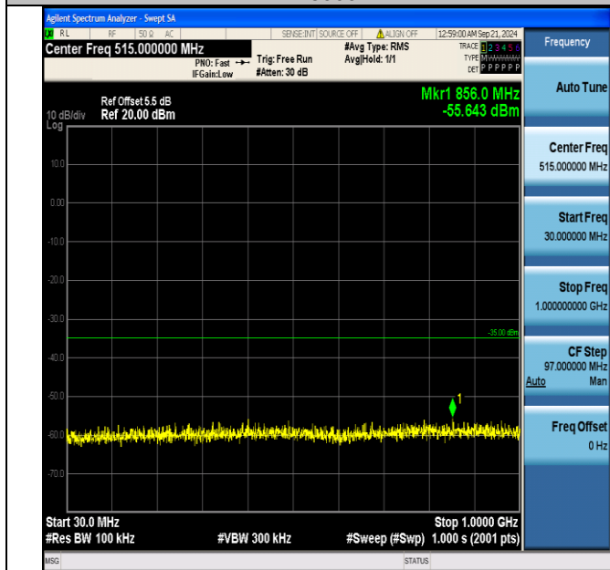
Band7_15MHz_QPSK_20825_1RB#0_30~1000_30~1000
