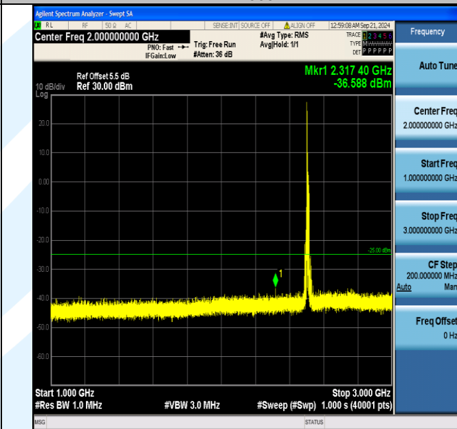
Band7_15MHz_QPSK_20825_1RB#0_1000~3000_1000~3000
