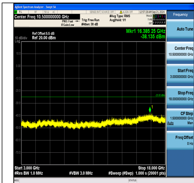
Band7_10MHz_16QAM_21400_1RB#49_3000~18000_3000~18000
