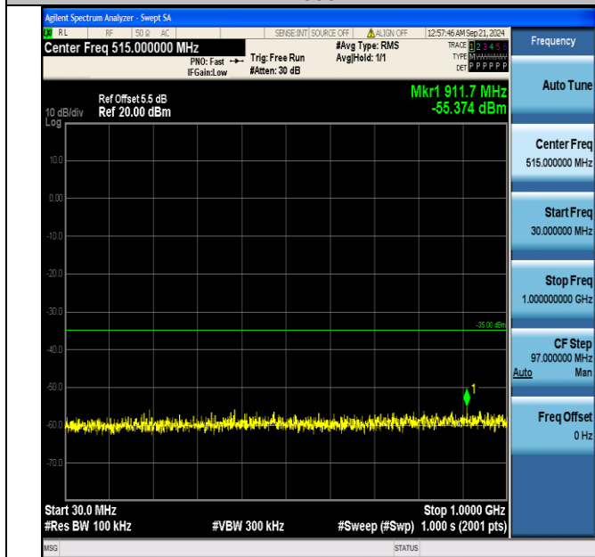
Band7_10MHz_QPSK_21400_50RB#0_30~1000_30~1000
