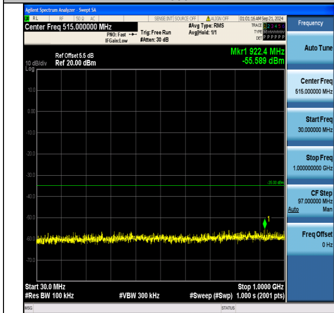
Band7_15MHz_QPSK_20825_75RB#0_30~1000_30~1000
