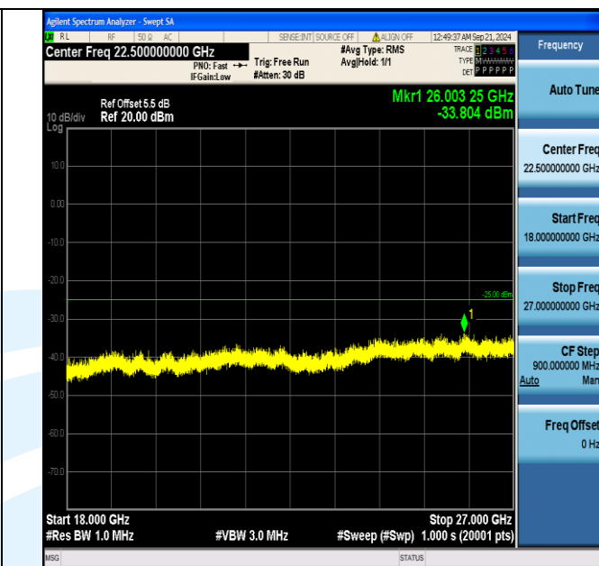
Band7_10MHz_16QAM_20800_1RB#0_18000~27000_18000~27000
