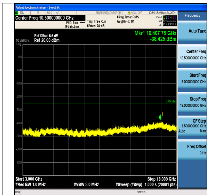
Band7_15MHz_QPSK_20825_1RB#0_3000~18000_3000~18000
