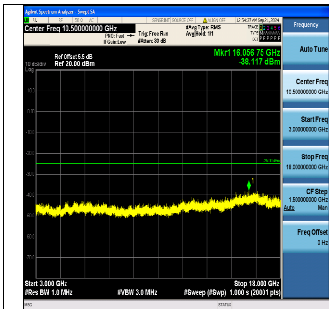
Band7_10MHz_QPSK_21100_50RB#0_3000~18000_3000~18000
