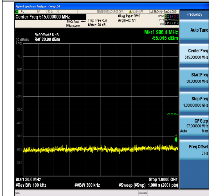
Band7_10MHz_16QAM_21400_1RB#0_30~1000_30~1000
