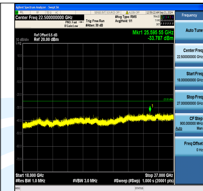
Band7_15MHz_QPSK_20825_1RB#0_18000~27000_18000~27000
