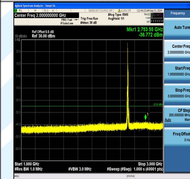
Band7_10MHz_16QAM_20800_1RB#0_1000~3000_1000~3000
