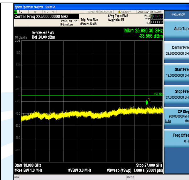
Band7_10MHz_16QAM_21100_1RB#49_18000~27000_18000~27000
