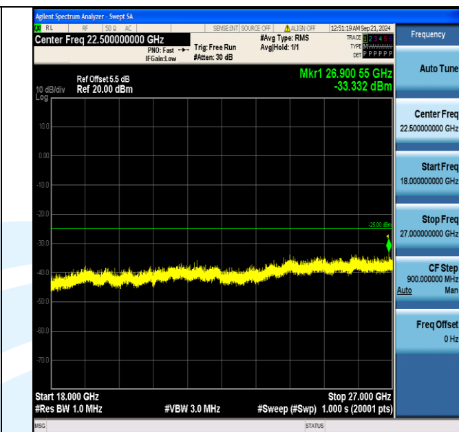
Band7_10MHz_QPSK_20800_50RB#0_18000~27000_18000~27000
