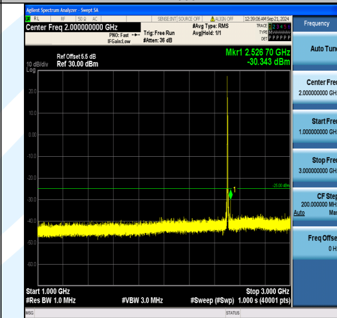
Band7_5MHz_16QAM_20775_1RB#0_1000~3000_1000~3000
