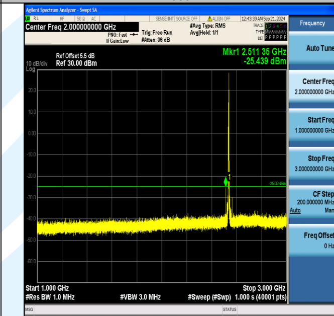
Band7_5MHz_16QAM_21100_1RB#24_1000~3000_1000~3000
