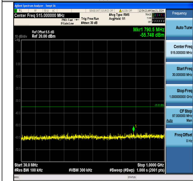
Band7_10MHz_QPSK_21100_50RB#0_30~1000_30~1000
