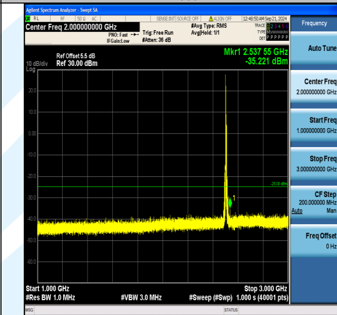
Band7_10MHz_QPSK_20800_1RB#0_1000~3000_1000~3000
