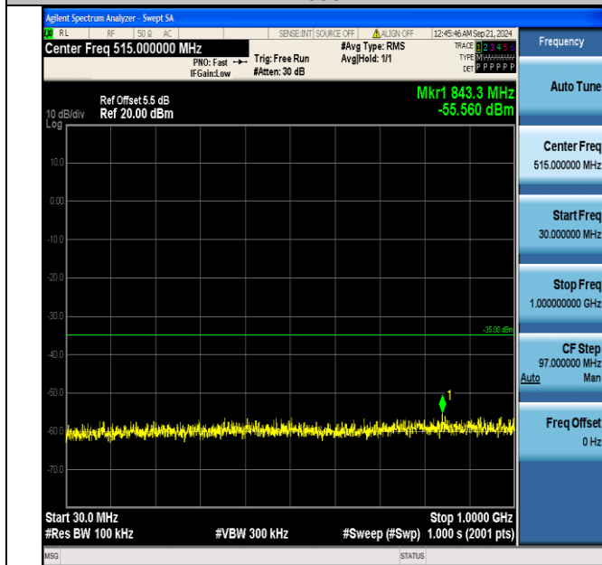
Band7_5MHz_16QAM_21425_1RB#0_30~1000_30~1000
