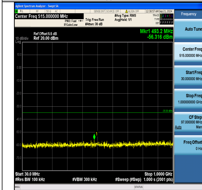
Band7_5MHz_16QAM_20775_1RB#0_30~1000_30~1000
