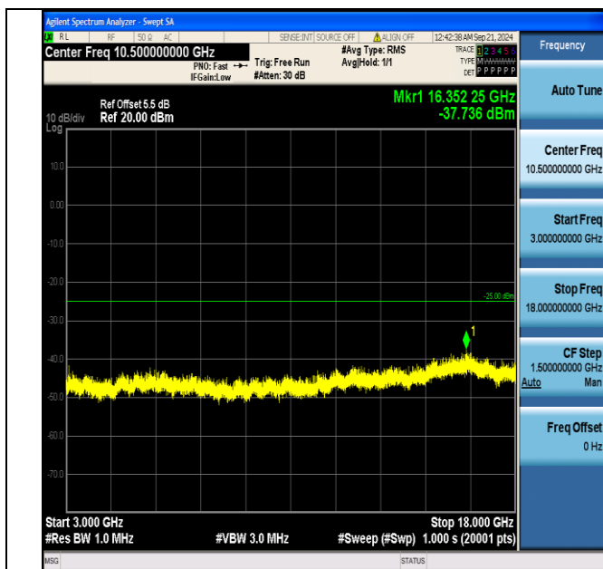
Band7_5MHz_16QAM_21100_1RB#0_3000~18000_3000~18000
