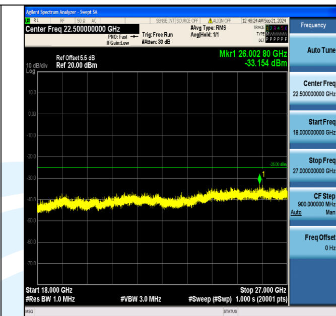
Band7_5MHz_16QAM_21425_25RB#0_18000~27000_18000~27000
