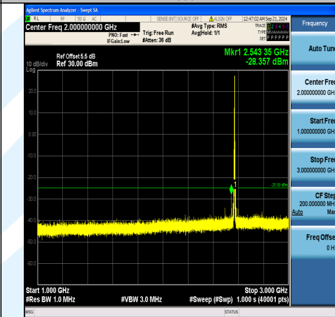
Band7_5MHz_16QAM_21425_1RB#24_1000~3000_1000~3000
