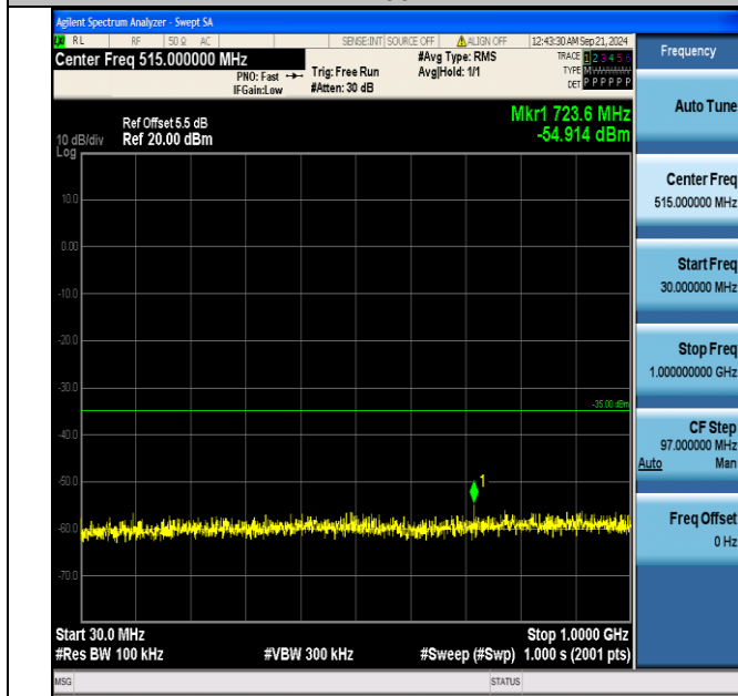
Band7_5MHz_16QAM_21100_1RB#24_30~1000_30~1000
