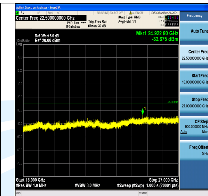
Band7_10MHz_QPSK_21100_1RB#49_18000~27000_18000~27000
