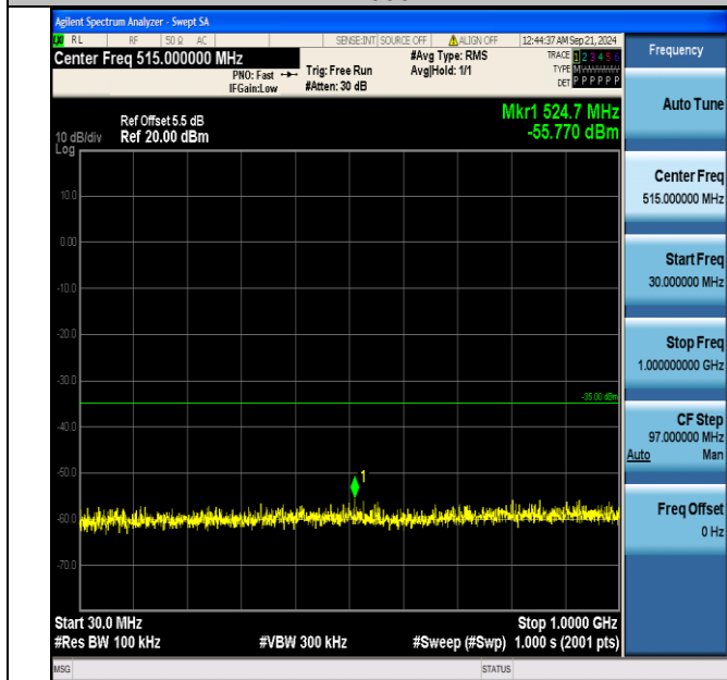
Band7_5MHz_16QAM_21100_25RB#0_30~1000_30~1000
