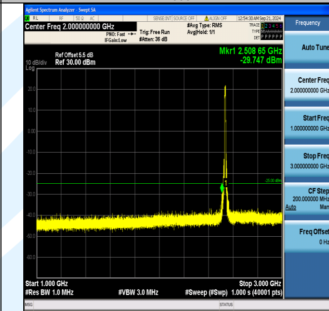
Band7_10MHz_QPSK_21100_50RB#0_1000~3000_1000~3000
