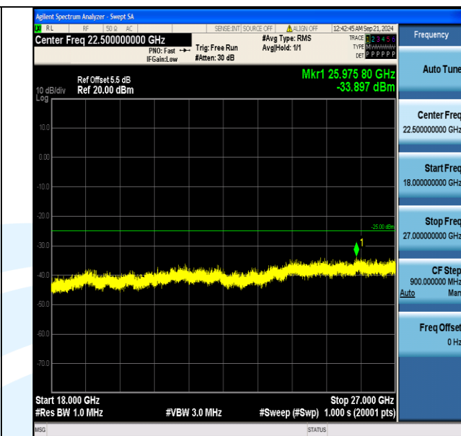
Band7_5MHz_16QAM_21100_1RB#0_18000~27000_18000~27000
