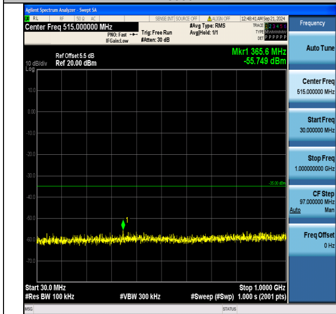
Band7_10MHz_QPSK_20800_1RB#0_30~1000_30~1000
