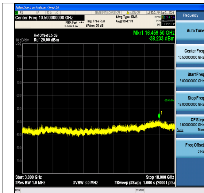
Band7_10MHz_QPSK_21100_1RB#0_3000~18000_3000~18000
