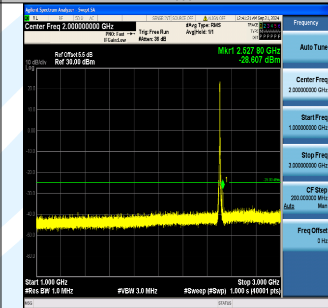
Band7_5MHz_16QAM_20775_25RB#0_1000~3000_1000~3000
