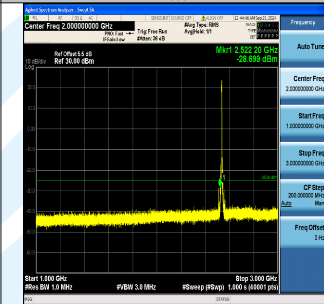
Band7_5MHz_16QAM_21100_25RB#0_1000~3000_1000~3000
