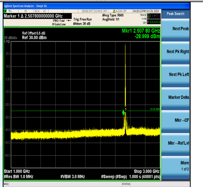
Band7_5MHz_16QAM_21100_1RB#0_1000~3000_1000~3000
