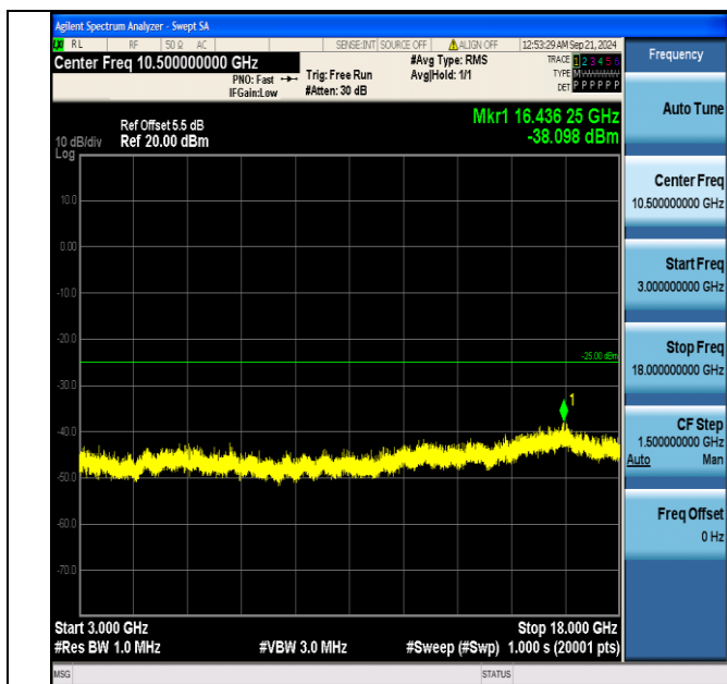
Band7_10MHz_QPSK_21100_1RB#49_3000~18000_3000~18000
