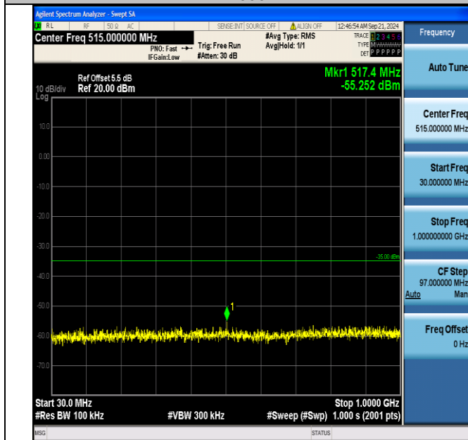
Band7_5MHz_16QAM_21425_1RB#24_30~1000_30~1000
