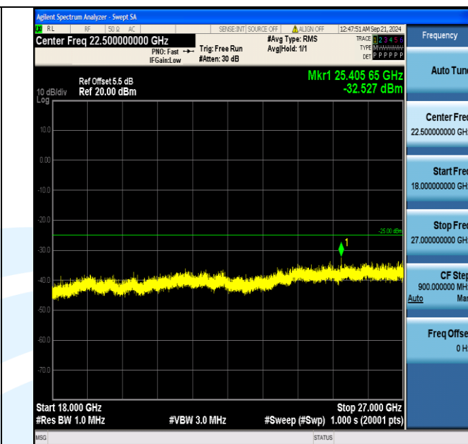
Band7_5MHz_QPSK_21425_25RB#0_18000~27000_18000~27000
