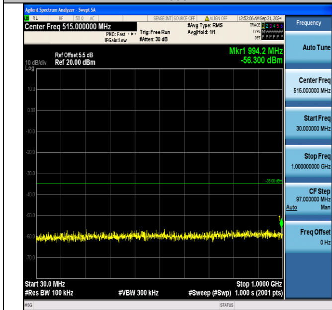
Band7_10MHz_QPSK_21100_1RB#0_30~1000_30~1000
