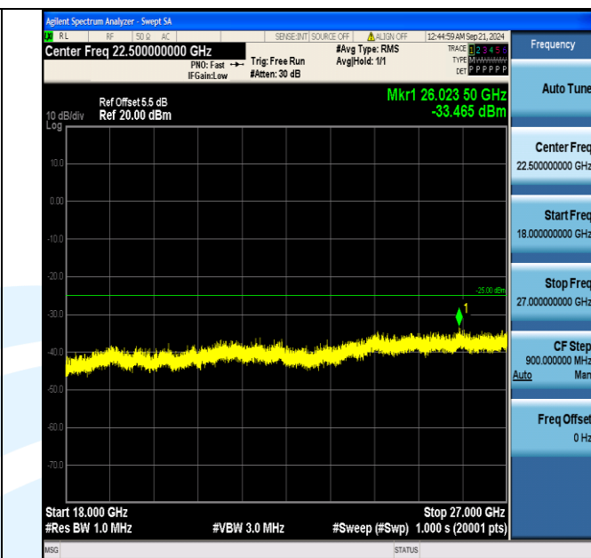
Band7_5MHz_16QAM_21100_25RB#0_18000~27000_18000~27000
