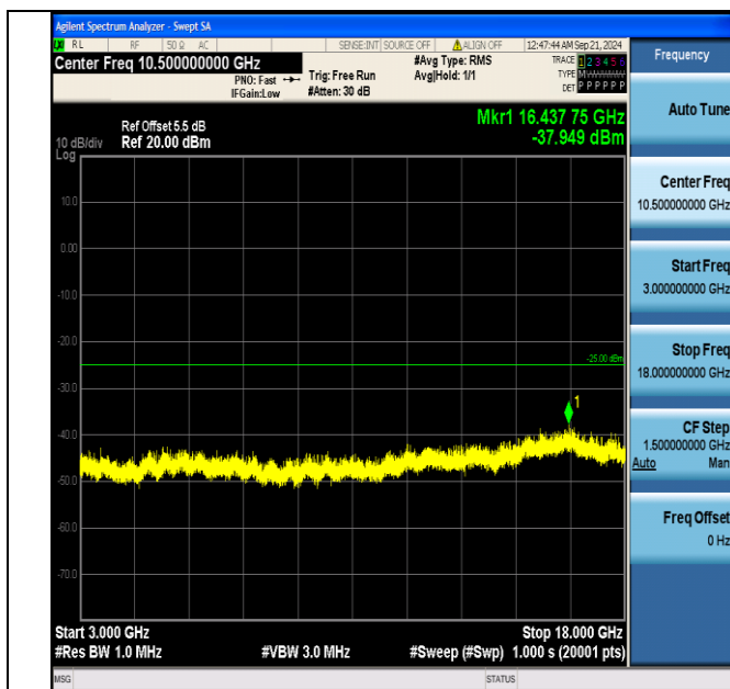
Band7_5MHz_QPSK_21425_25RB#0_3000~18000_3000~18000
