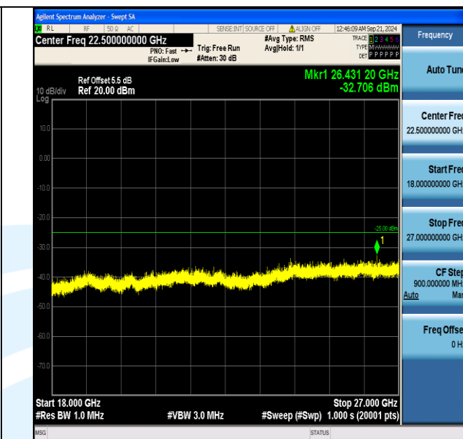
Band7_5MHz_16QAM_21425_1RB#0_18000~27000_18000~27000
