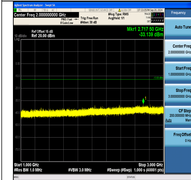
Band5_10MHz_16QAM_20450_50RB#0_1000~3000_1000~3000
