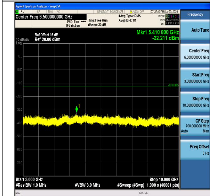
Band5_10MHz_16QAM_20600_1RB#49_3000~10000_3000~10000
