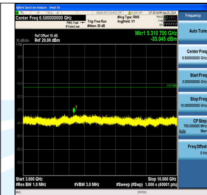
Band5_10MHz_16QAM_20600_50RB#0_3000~10000_3000~10000
