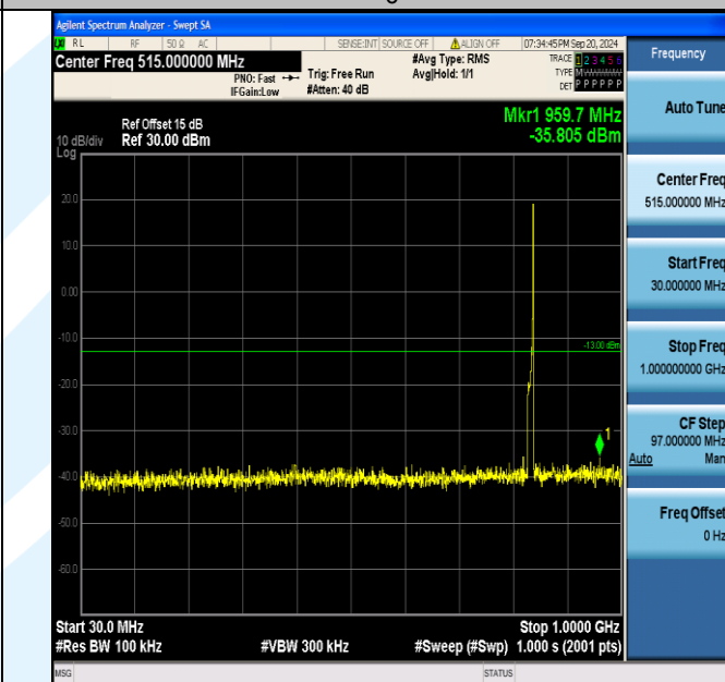
Band5_10MHz_16QAM_20525_1RB#49_30~1000_30~1000
