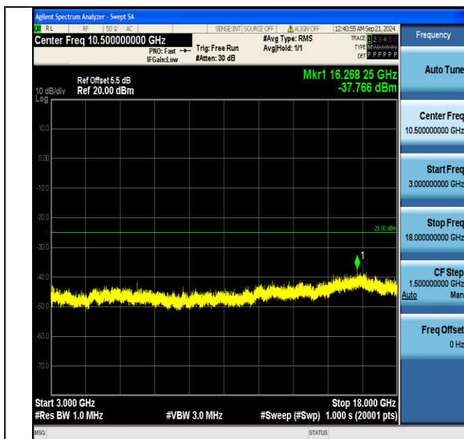
Band7_5MHz_QPSK_20775_25RB#0_3000~18000_3000~18000
