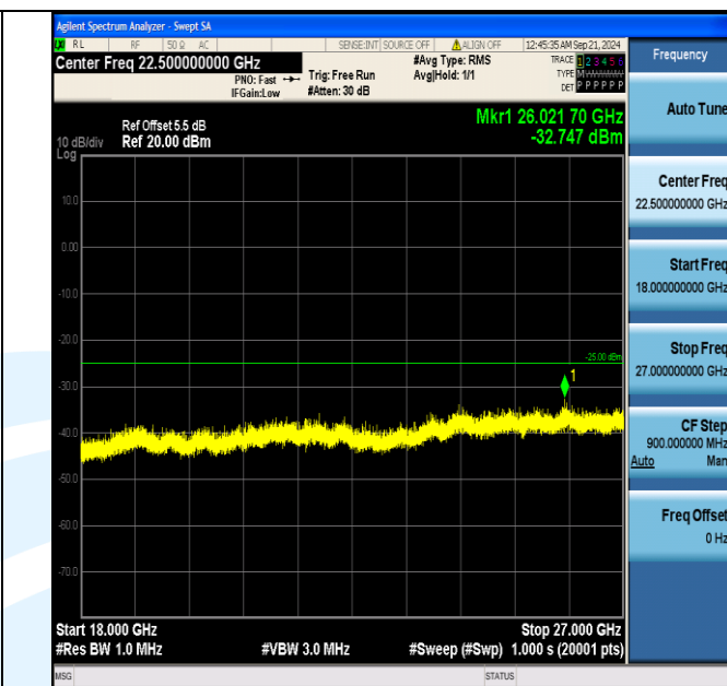
Band7_5MHz_QPSK_21425_1RB#0_18000~27000_18000~27000
