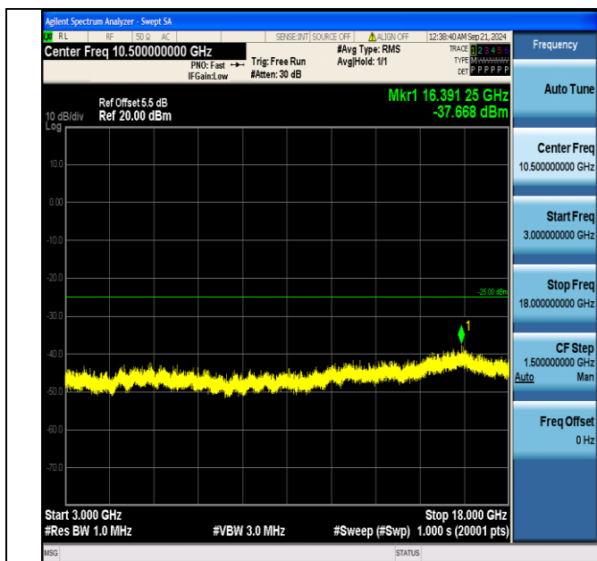
Band7_5MHz_QPSK_20775_1RB#0_3000~18000_3000~18000
