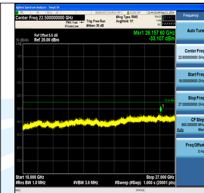
Band7_5MHz_QPSK_21100_25RB#0_18000~27000_18000~27000
