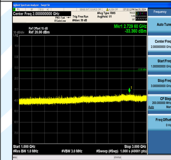
Band5_10MHz_16QAM_20450_1RB#49_1000~3000_1000~3000
