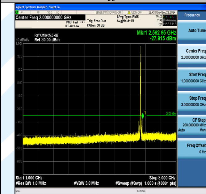
Band7_5MHz_QPSK_21100_1RB#24_1000~3000_1000~3000
