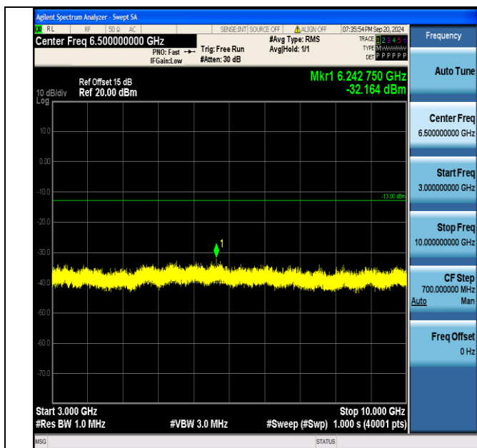
Band5_10MHz_16QAM_20525_50RB#0_3000~10000_3000~10000
