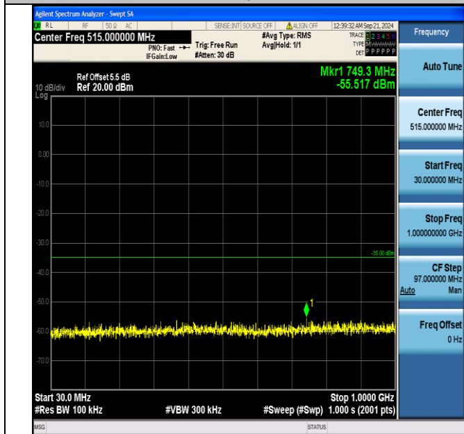
Band7_5MHz_QPSK_20775_1RB#24_30~1000_30~1000
