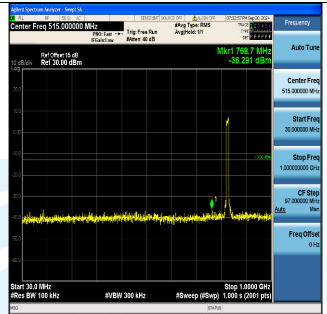
Band5_10MHz_16QAM_20450_50RB#0_30~1000_30~1000
