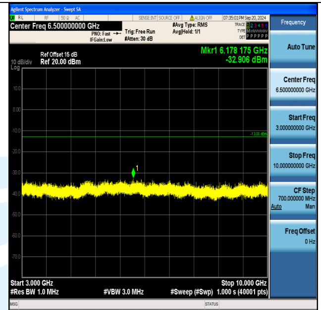
Band5_10MHz_16QAM_20525_1RB#49_3000~10000_3000~10000
