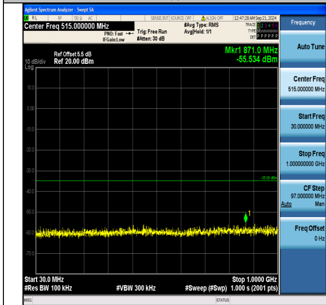
Band7_5MHz_QPSK_21425_25RB#0_30~1000_30~1000
