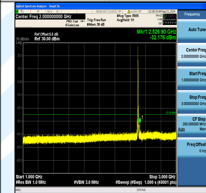
Band7_5MHz_QPSK_20775_1RB#0_1000~3000_1000~3000
