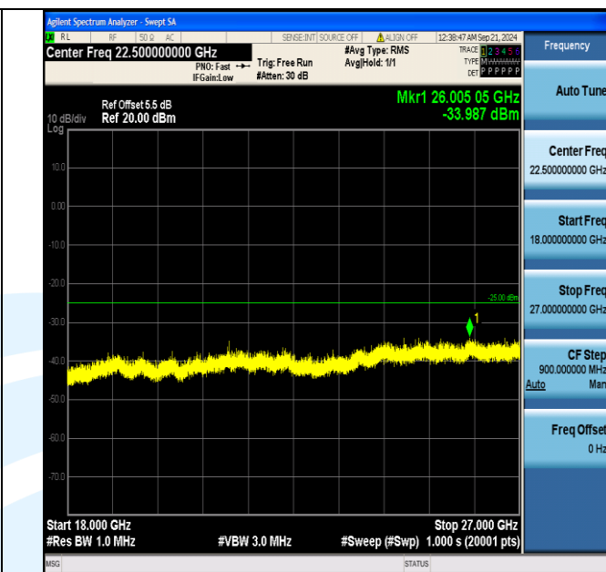
Band7_5MHz_QPSK_20775_1RB#0_18000~27000_18000~27000
