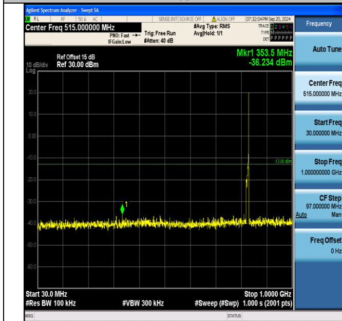
Band5_10MHz_16QAM_20450_1RB#49_30~1000_30~1000
