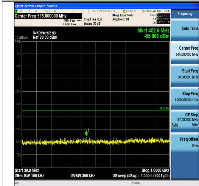
Band7_5MHz_QPSK_20775_25RB#0_30~1000_30~1000
