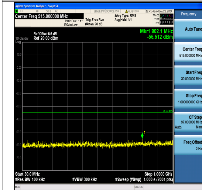
Band7_5MHz_QPSK_21100_1RB#0_30~1000_30~1000
