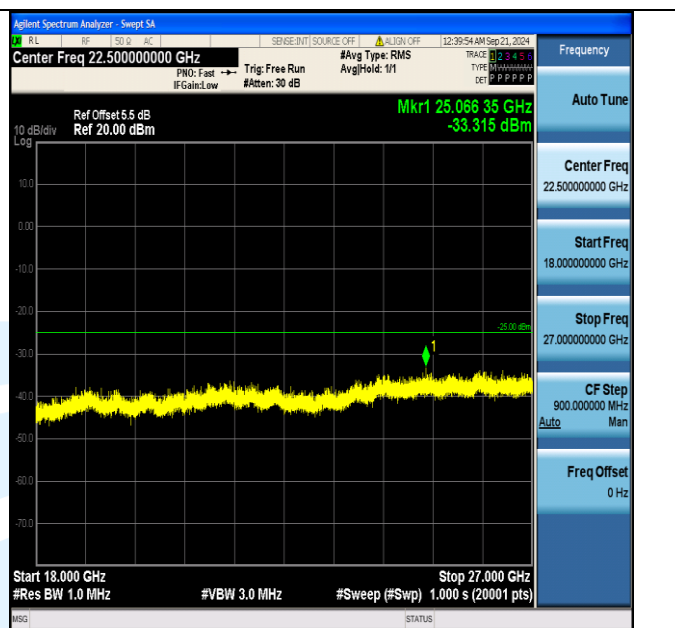
Band7_5MHz_QPSK_20775_1RB#24_18000~27000_18000~27000
