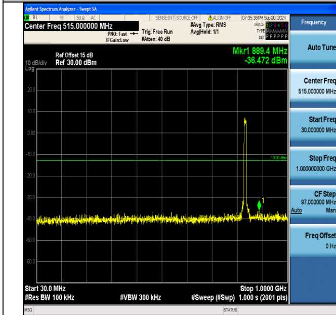
Band5_10MHz_16QAM_20525_50RB#0_30~1000_30~1000
