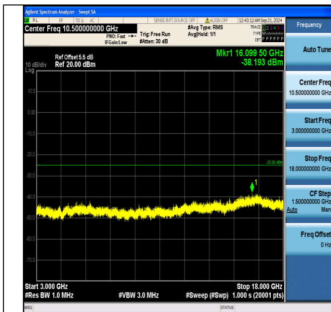
Band7_5MHz_QPSK_21100_1RB#24_3000~18000_3000~18000
