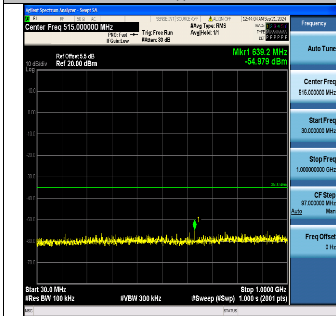
Band7_5MHz_QPSK_21100_25RB#0_30~1000_30~1000
