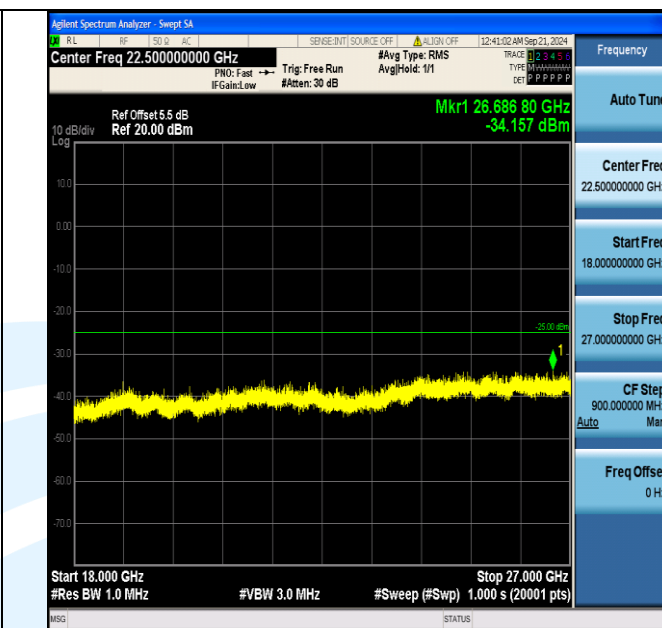
Band7_5MHz_QPSK_20775_25RB#0_18000~27000_18000~27000
