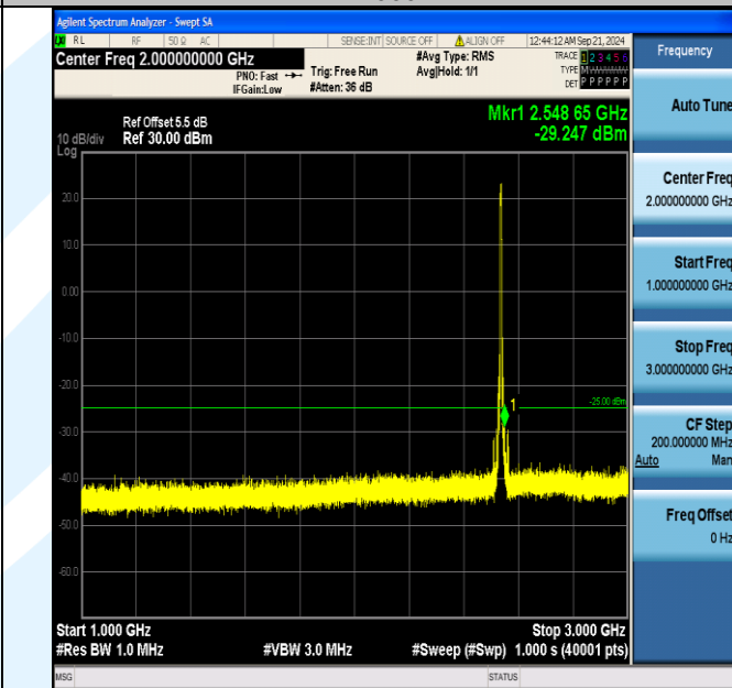
Band7_5MHz_QPSK_21100_25RB#0_1000~3000_1000~3000
