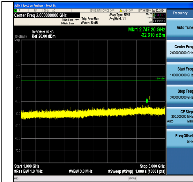
Band5_10MHz_16QAM_20525_1RB#49_1000~3000_1000~3000
