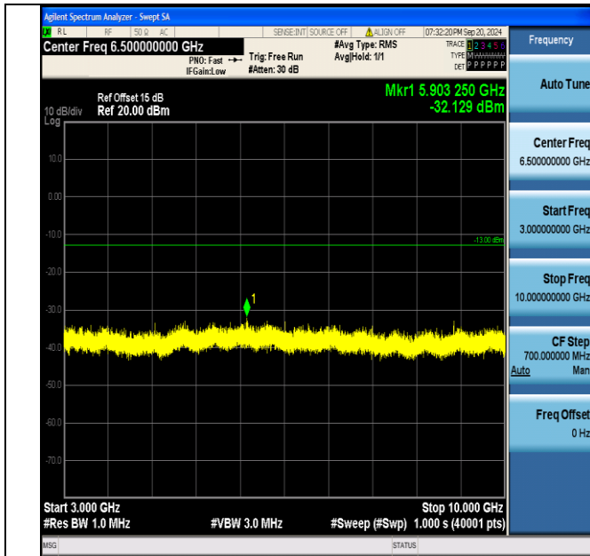
Band5_10MHz_16QAM_20450_1RB#49_3000~10000_3000~10000
