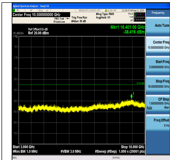
Band7_5MHz_QPSK_20775_1RB#24_3000~18000_3000~18000
