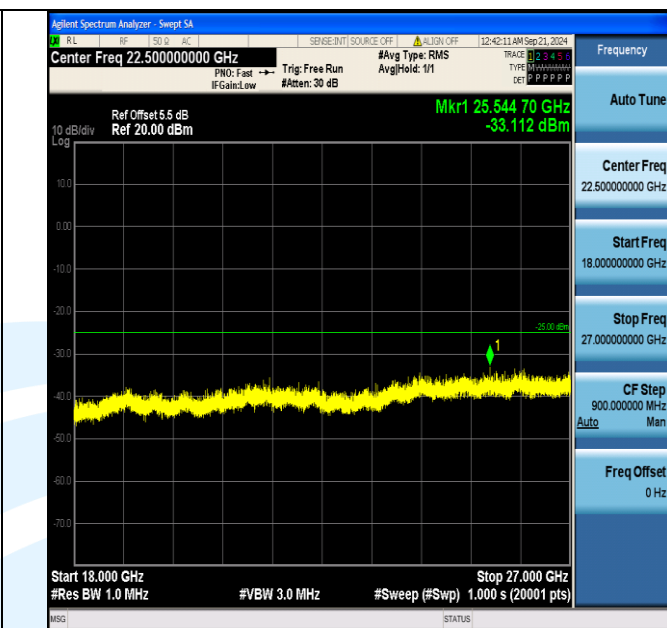
Band7_5MHz_QPSK_21100_1RB#0_18000~27000_18000~27000
