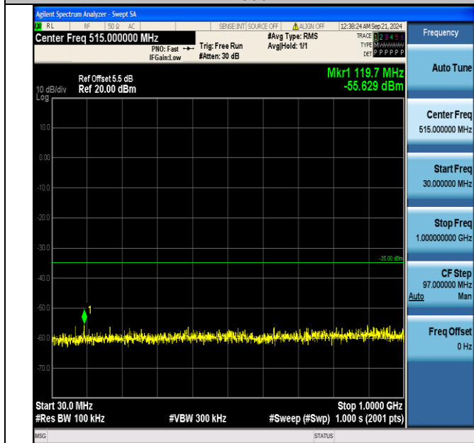
Band7_5MHz_QPSK_20775_1RB#0_30~1000_30~1000
