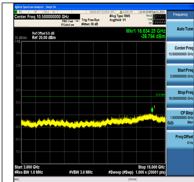
Band7_5MHz_QPSK_21100_25RB#0_3000~18000_3000~18000
