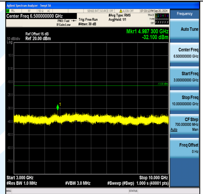
Band5_10MHz_16QAM_20450_50RB#0_3000~10000_3000~10000
