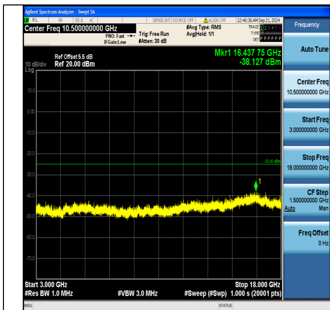
Band7_5MHz_QPSK_21425_1RB#24_3000~18000_3000~18000
