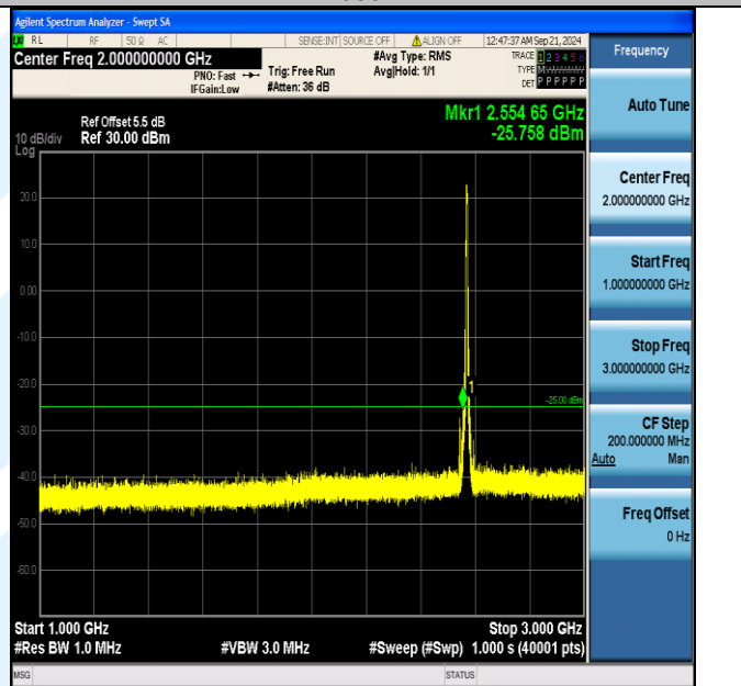
Band7_5MHz_QPSK_21425_25RB#0_1000~3000_1000~3000
