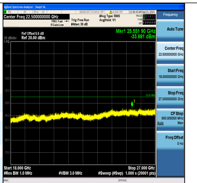
Band7_5MHz_QPSK_21425_1RB#24_18000~27000_18000~27000
