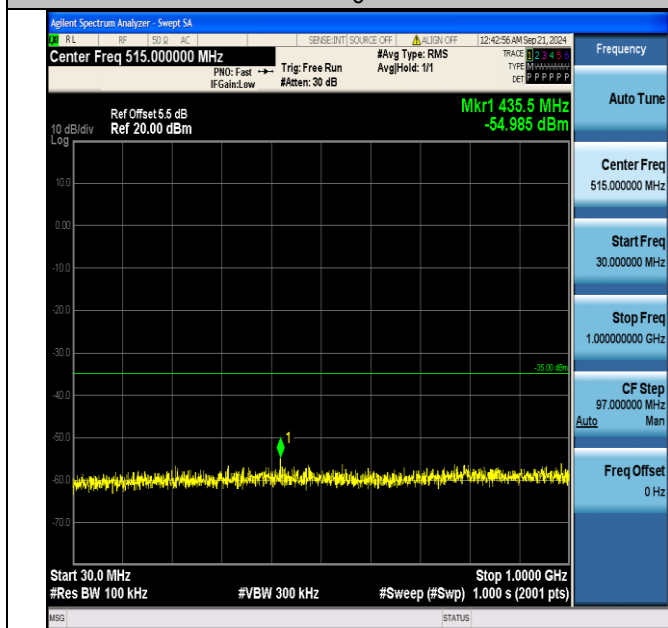
Band7_5MHz_QPSK_21100_1RB#24_30~1000_30~1000
