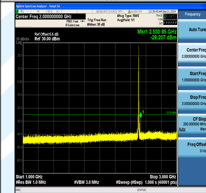
Band7_5MHz_QPSK_20775_1RB#24_1000~3000_1000~3000
