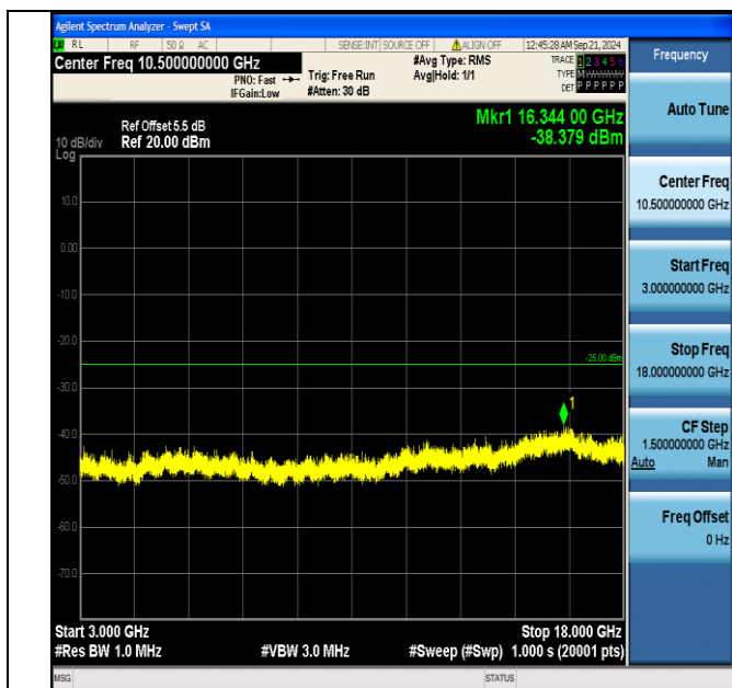
Band7_5MHz_QPSK_21425_1RB#0_3000~18000_3000~18000
