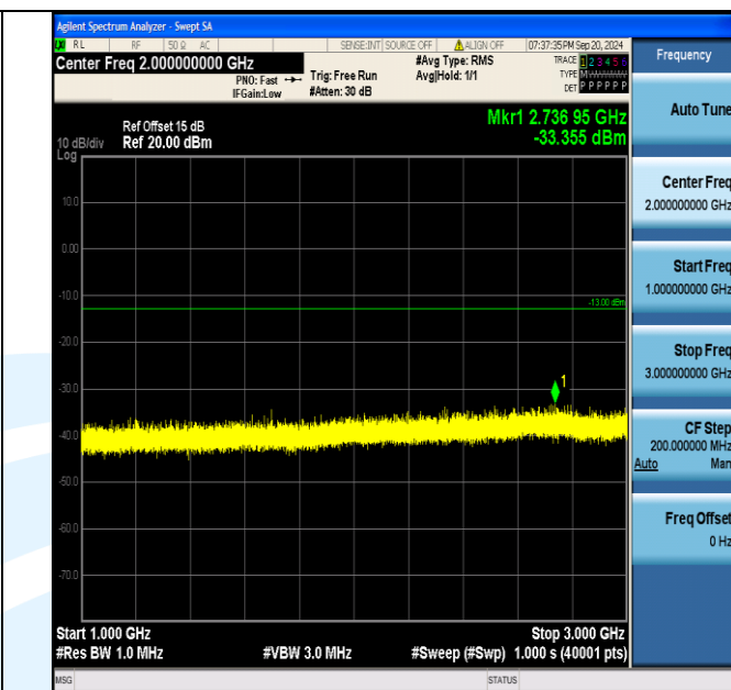
Band5_10MHz_16QAM_20600_1RB#49_1000~3000_1000~3000
