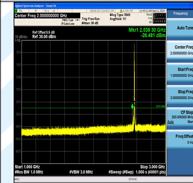
Band7_5MHz_QPSK_21425_1RB#0_1000~3000_1000~3000
