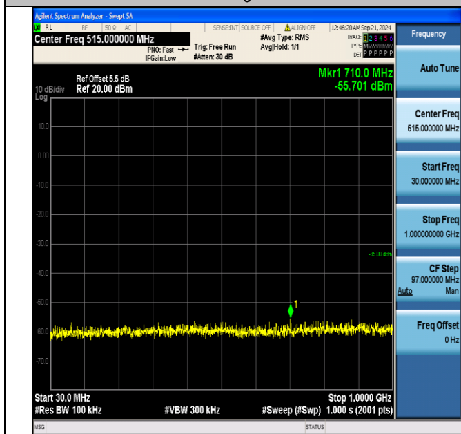
Band7_5MHz_QPSK_21425_1RB#24_30~1000_30~1000
