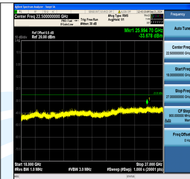
Band7_5MHz_QPSK_21100_1RB#24_18000~27000_18000~27000
