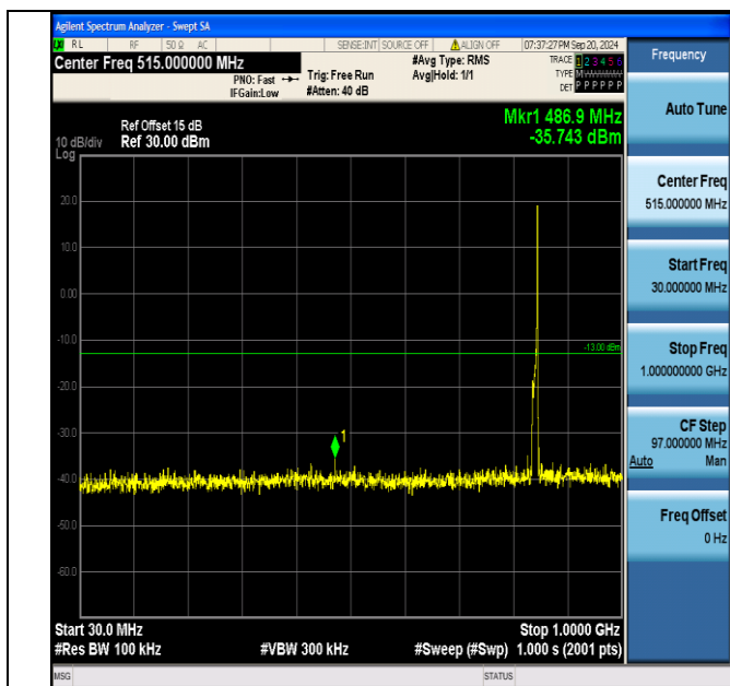
Band5_10MHz_16QAM_20600_1RB#49_30~1000_30~1000
