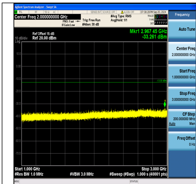
Band5_10MHz_16QAM_20600_50RB#0_1000~3000_1000~3000
