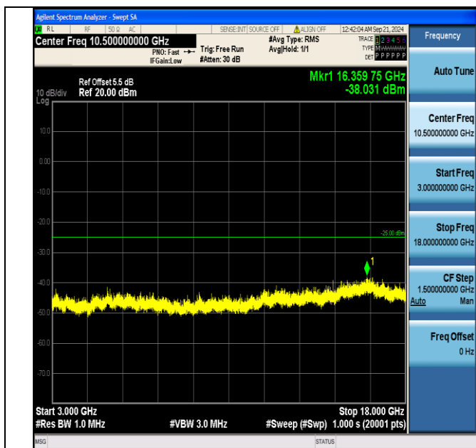
Band7_5MHz_QPSK_21100_1RB#0_3000~18000_3000~18000
