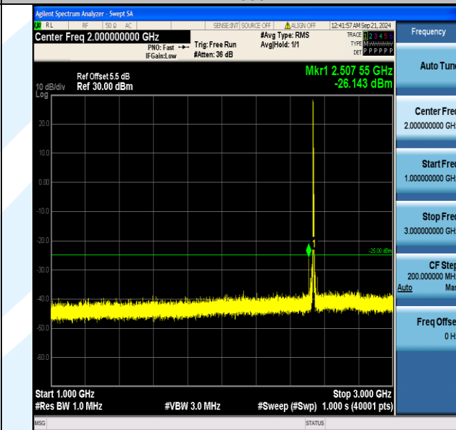
Band7_5MHz_QPSK_21100_1RB#0_1000~3000_1000~3000
