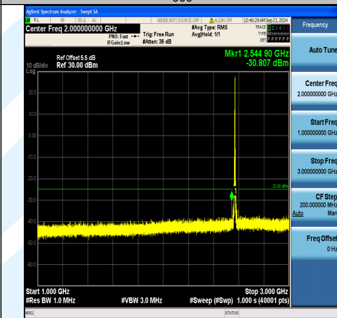
Band7_5MHz_QPSK_21425_1RB#24_1000~3000_1000~3000
