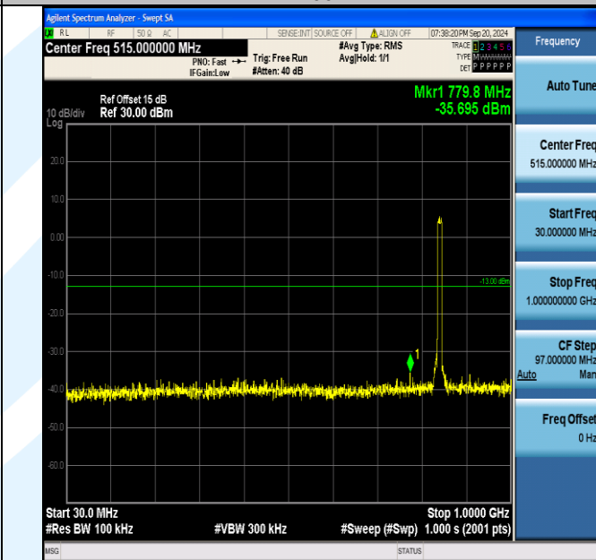
Band5_10MHz_16QAM_20600_50RB#0_30~1000_30~1000
