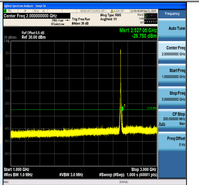
Band7_5MHz_QPSK_20775_25RB#0_1000~3000_1000~3000
