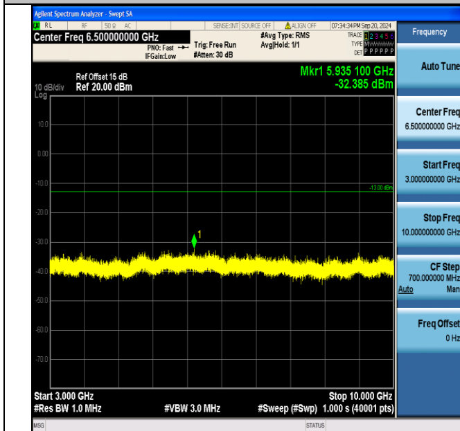
Band5_10MHz_QPSK_20525_1RB#49_3000~10000_3000~10000
