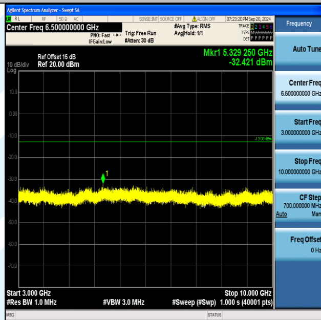
Band5_5MHz_16QAM_20425_1RB#0_3000~10000_3000~10000
