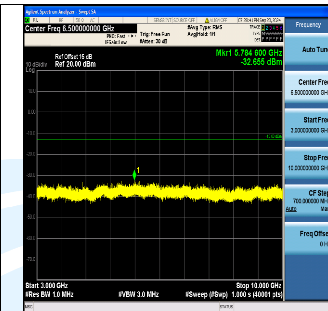
Band5_5MHz_16QAM_20625_1RB#0_3000~10000_3000~10000
