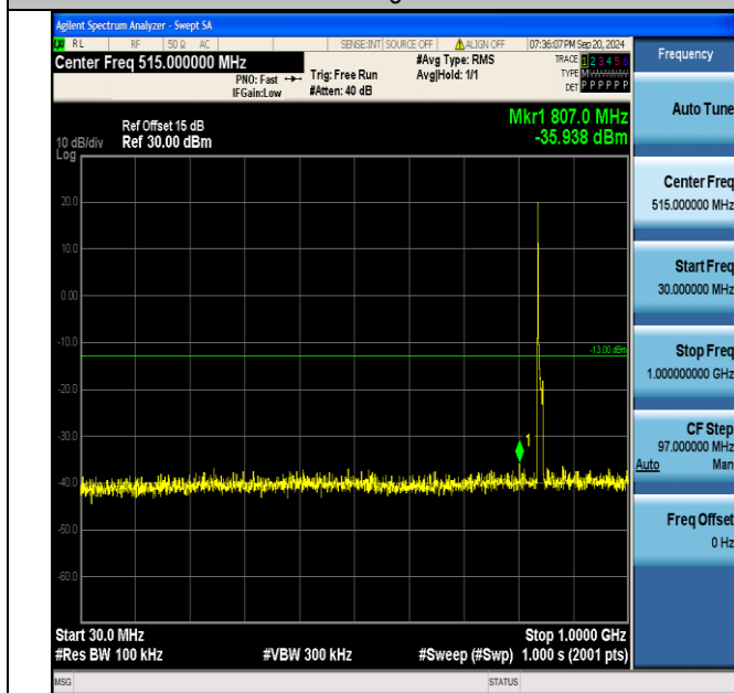
Band5_10MHz_QPSK_20600_1RB#0_30~1000_30~1000
