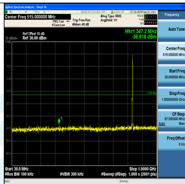
Band5_5MHz_16QAM_20525_1RB#24_30~1000_30~1000
