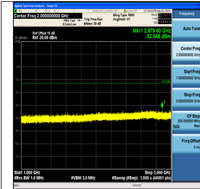
Band5_5MHz_QPSK_20625_1RB#24_1000~3000_1000~3000
