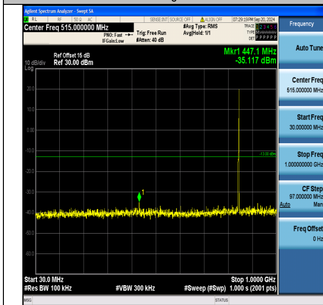
Band5_5MHz_16QAM_20625_1RB#24_30~1000_30~1000
