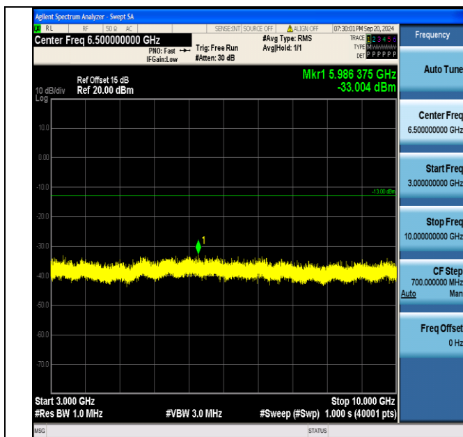
Band5_5MHz_QPSK_20625_25RB#0_3000~10000_3000~10000
