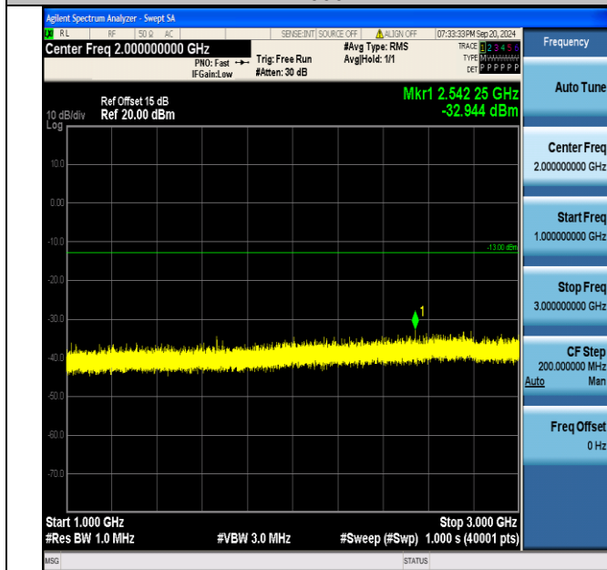
Band5_10MHz_QPSK_20525_1RB#0_1000~3000_1000~3000
