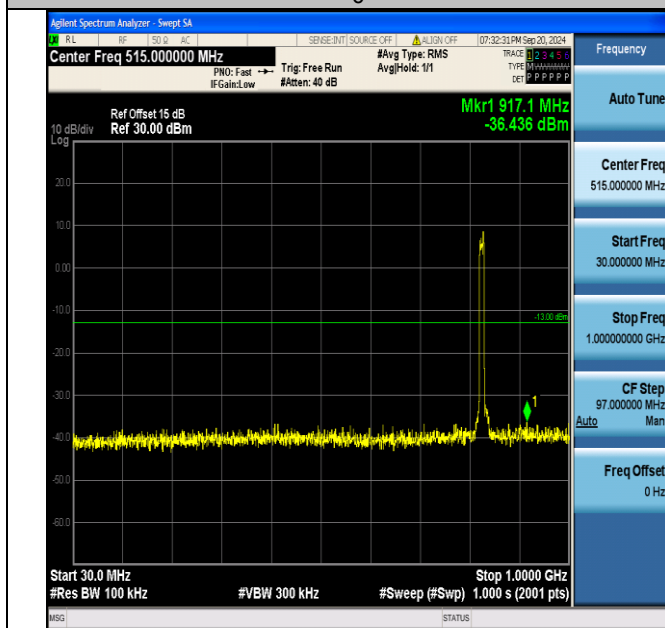
Band5_10MHz_QPSK_20450_50RB#0_30~1000_30~1000
