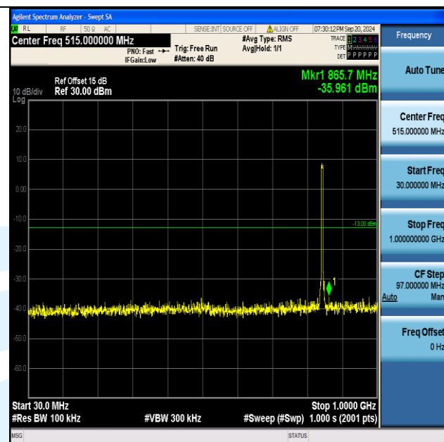
Band5_5MHz_16QAM_20625_25RB#0_30~1000_30~1000
