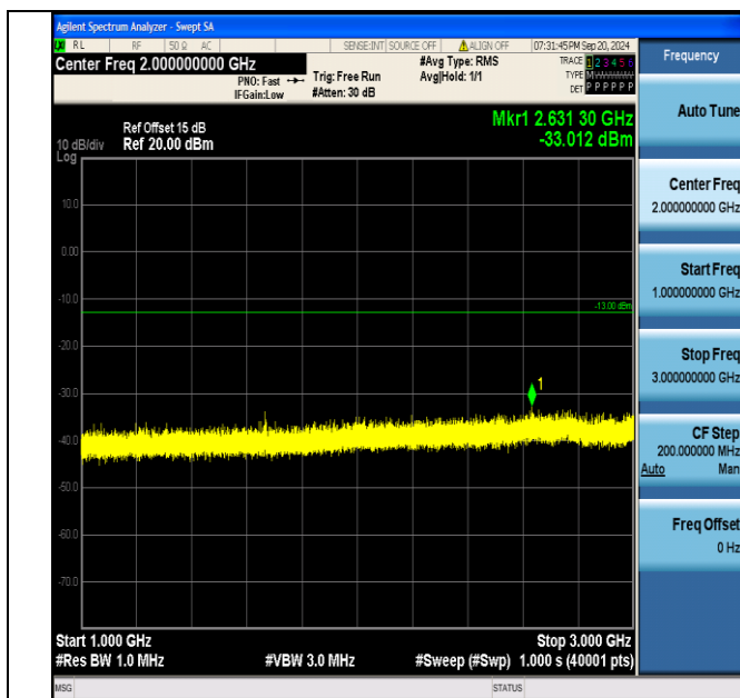
Band5_10MHz_QPSK_20450_1RB#49_1000~3000_1000~3000
