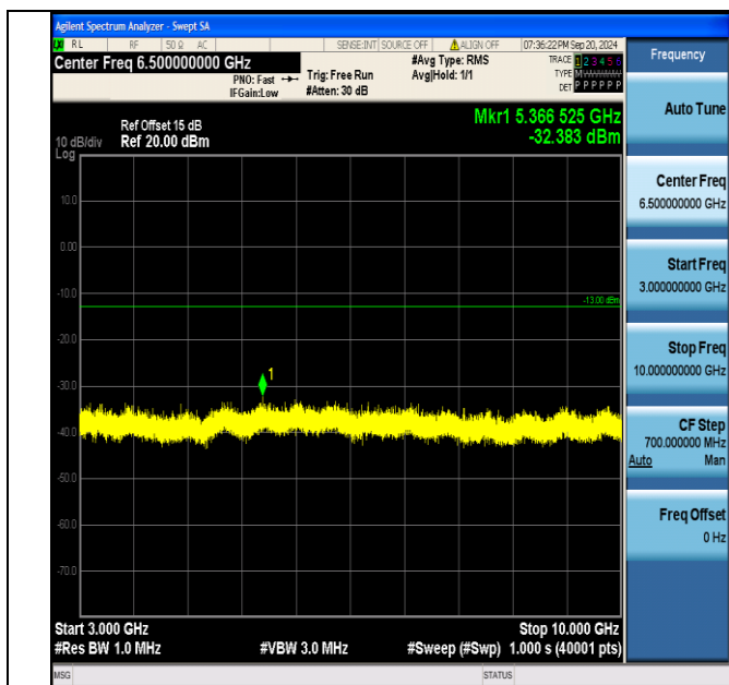
Band5_10MHz_QPSK_20600_1RB#0_3000~10000_3000~10000
