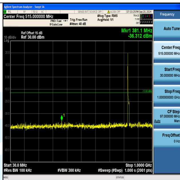
Band5_10MHz_QPSK_20525_1RB#0_30~1000_30~1000
