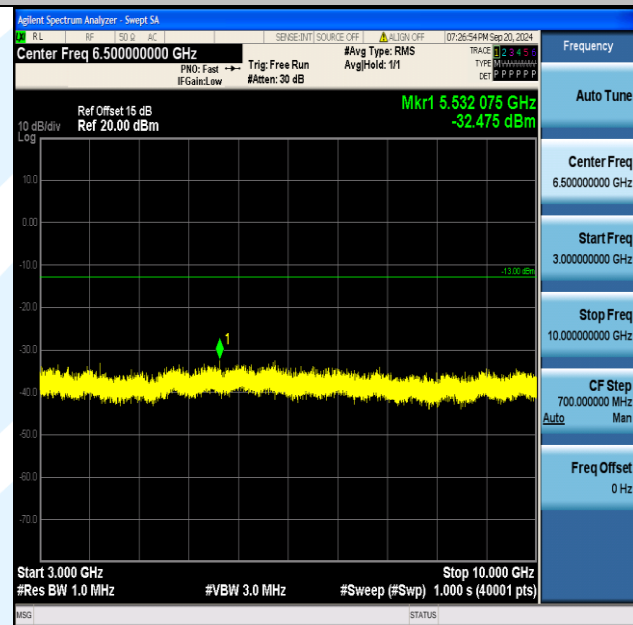
Band5_5MHz_16QAM_20525_1RB#24_3000~10000_3000~10000
