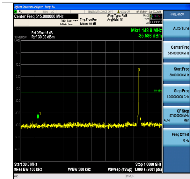
Band5_10MHz_QPSK_20600_50RB#0_30~1000_30~1000
