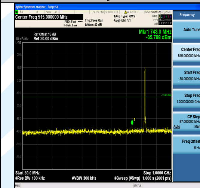
Band5_5MHz_16QAM_20425_25RB#0_30~1000_30~1000
