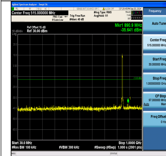
Band5_5MHz_QPSK_20625_25RB#0_30~1000_30~1000
