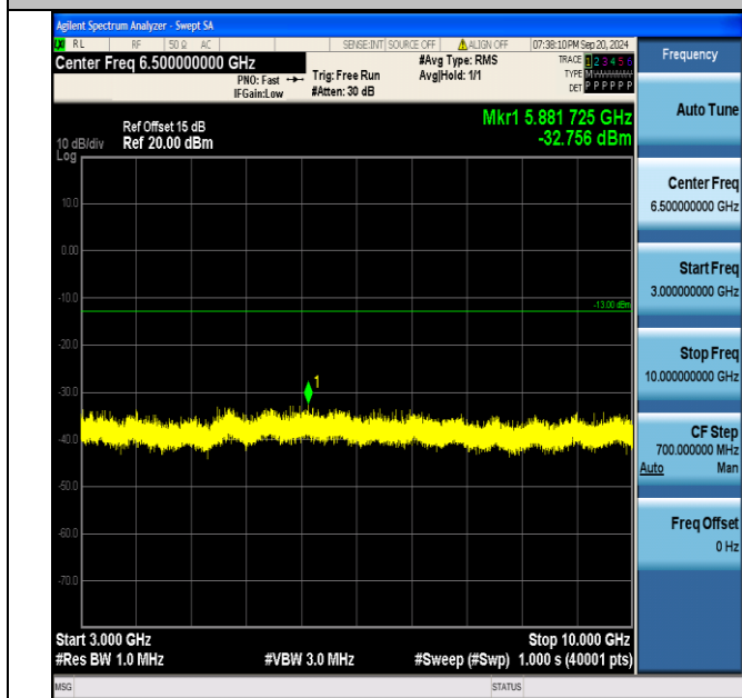
Band5_10MHz_QPSK_20600_50RB#0_3000~10000_3000~10000
