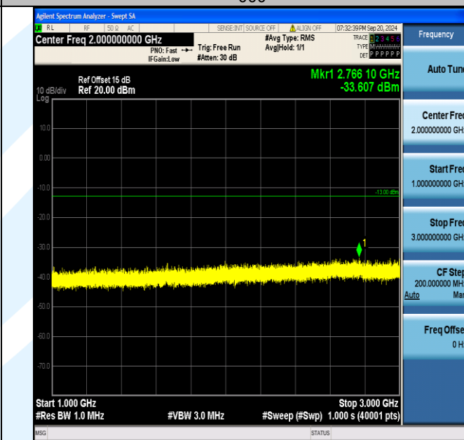
Band5_10MHz_QPSK_20450_50RB#0_1000~3000_1000~3000
