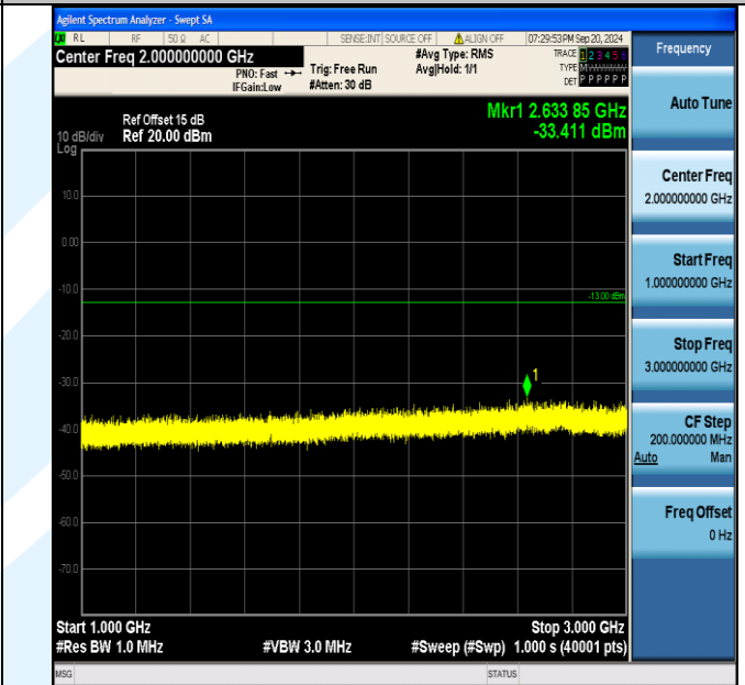
Band5_5MHz_QPSK_20625_25RB#0_1000~3000_1000~3000
