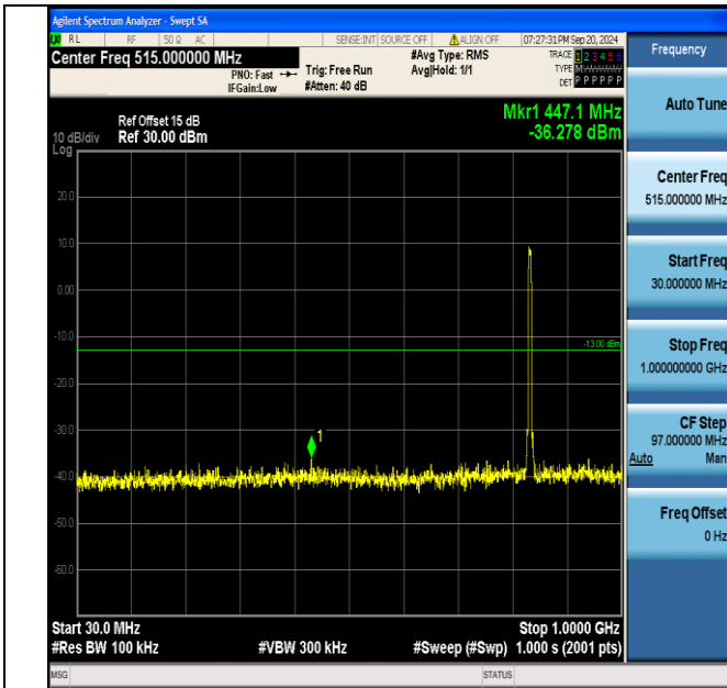
Band5_5MHz_16QAM_20525_25RB#0_30~1000_30~1000
