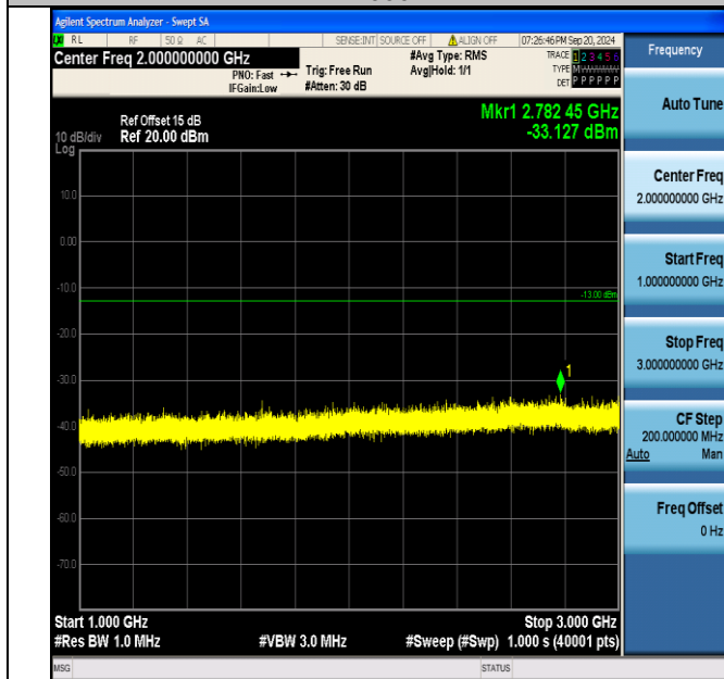
Band5_5MHz_16QAM_20525_1RB#24_1000~3000_1000~3000
