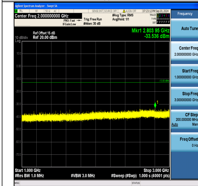
Band5_5MHz_16QAM_20425_1RB#0_1000~3000_1000~3000
