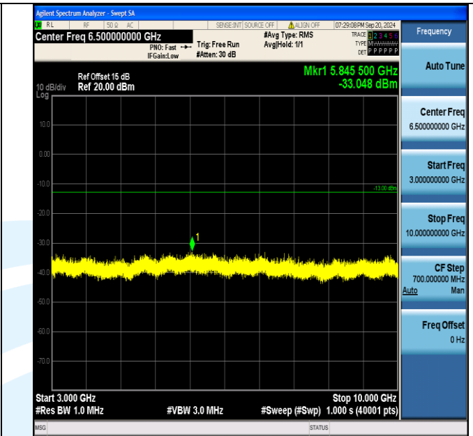
Band5_5MHz_QPSK_20625_1RB#24_3000~10000_3000~10000
