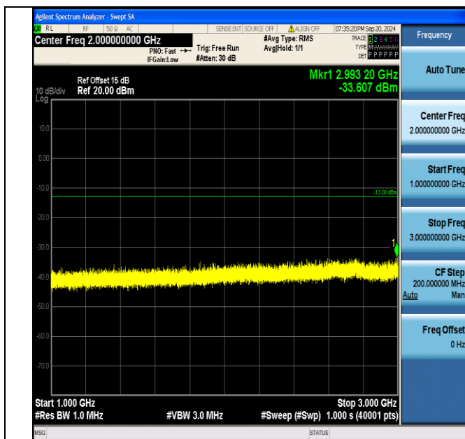
Band5_10MHz_QPSK_20525_50RB#0_1000~3000_1000~3000
