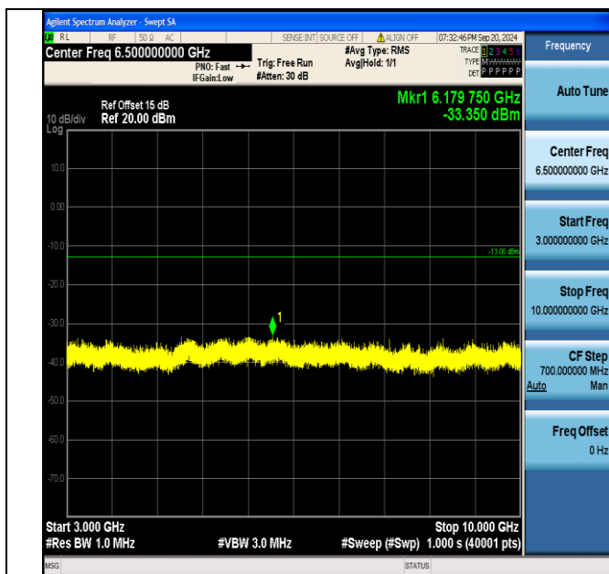
Band5_10MHz_QPSK_20450_50RB#0_3000~10000_3000~10000
