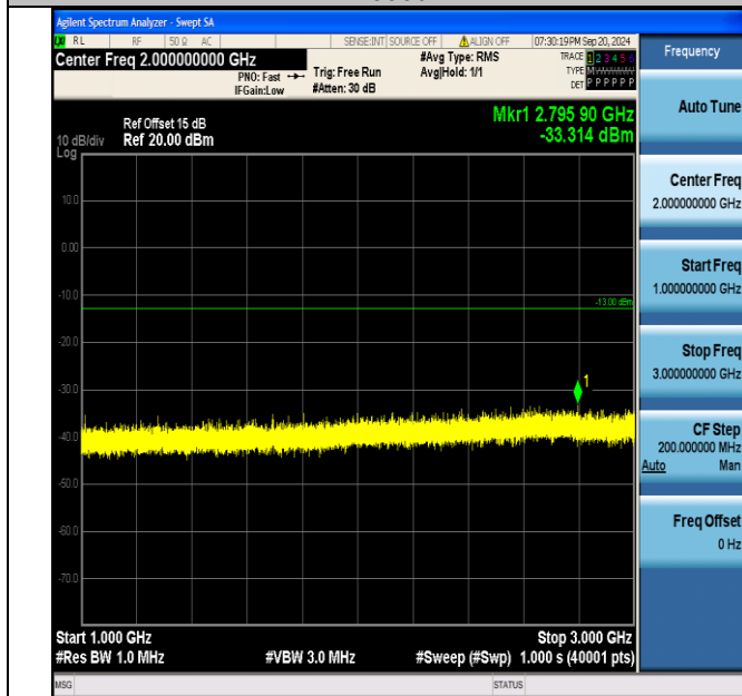
Band5_5MHz_16QAM_20625_25RB#0_1000~3000_1000~3000
