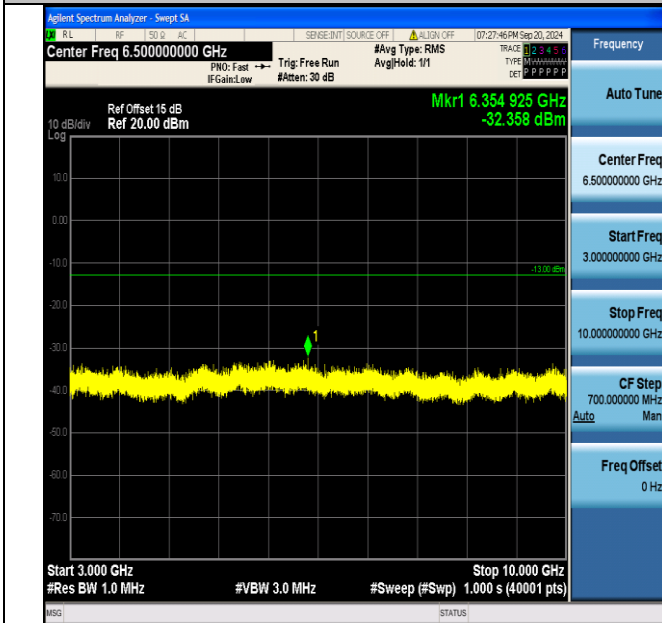
Band5_5MHz_16QAM_20525_25RB#0_3000~10000_3000~10000
