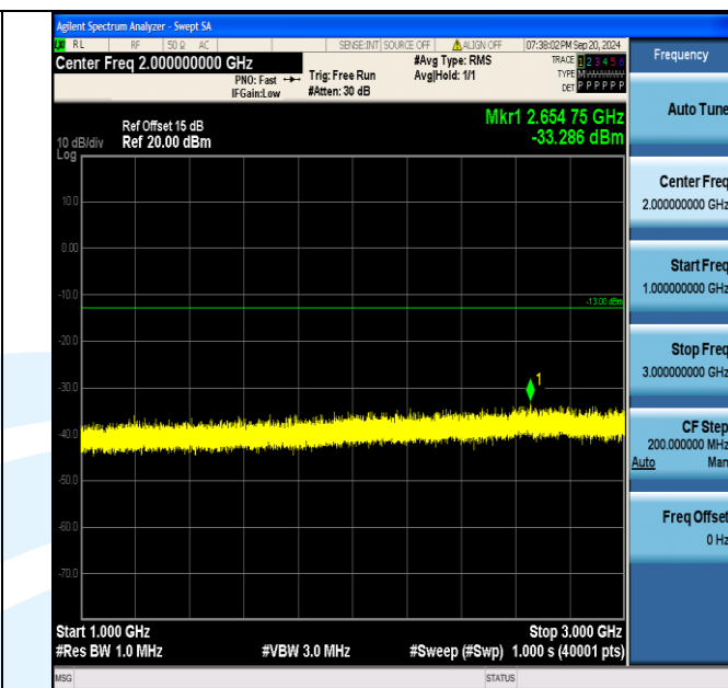
Band5_10MHz_QPSK_20600_50RB#0_1000~3000_1000~3000
