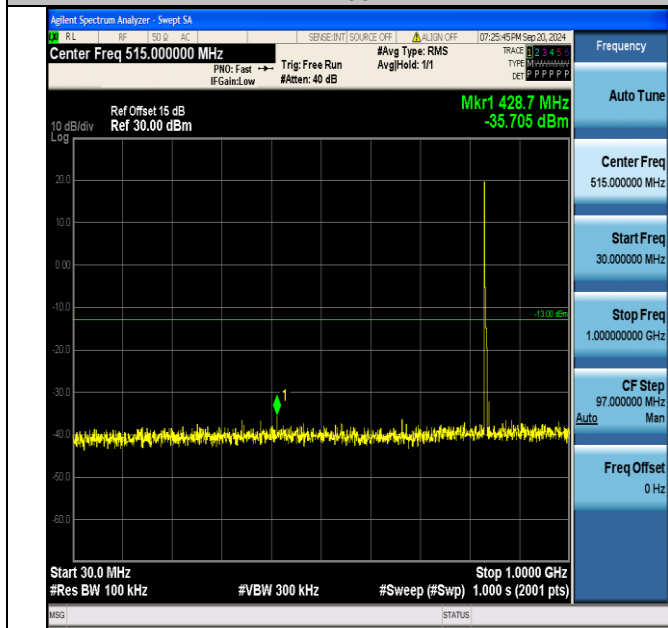
Band5_5MHz_16QAM_20525_1RB#0_30~1000_30~1000
