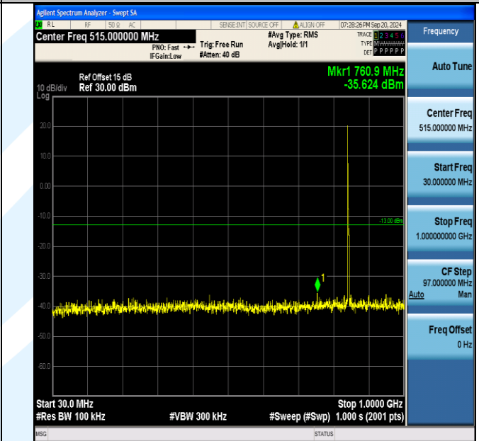
Band5_5MHz_16QAM_20625_1RB#0_30~1000_30~1000
