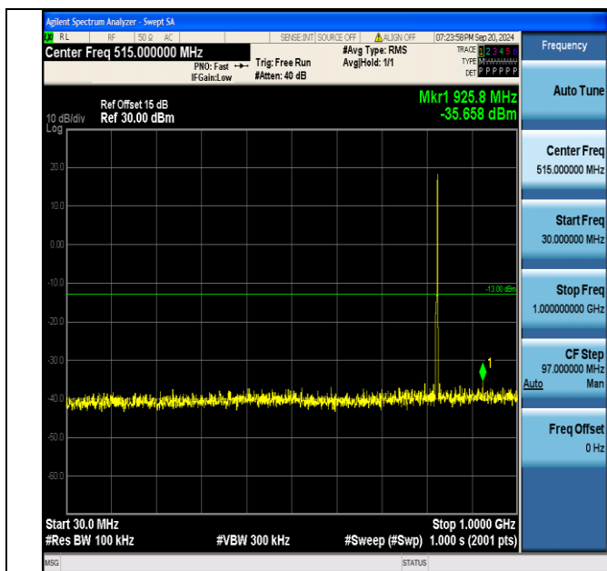
Band5_5MHz_16QAM_20425_1RB#24_30~1000_30~1000
