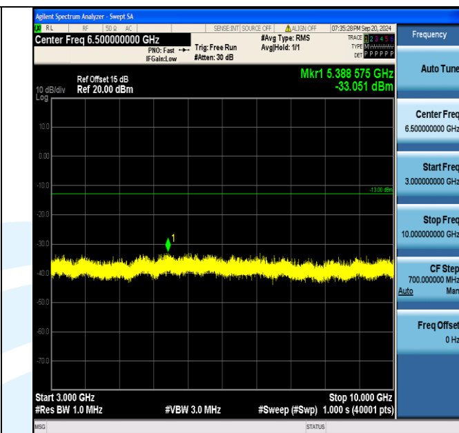
Band5_10MHz_QPSK_20525_50RB#0_3000~10000_3000~10000
