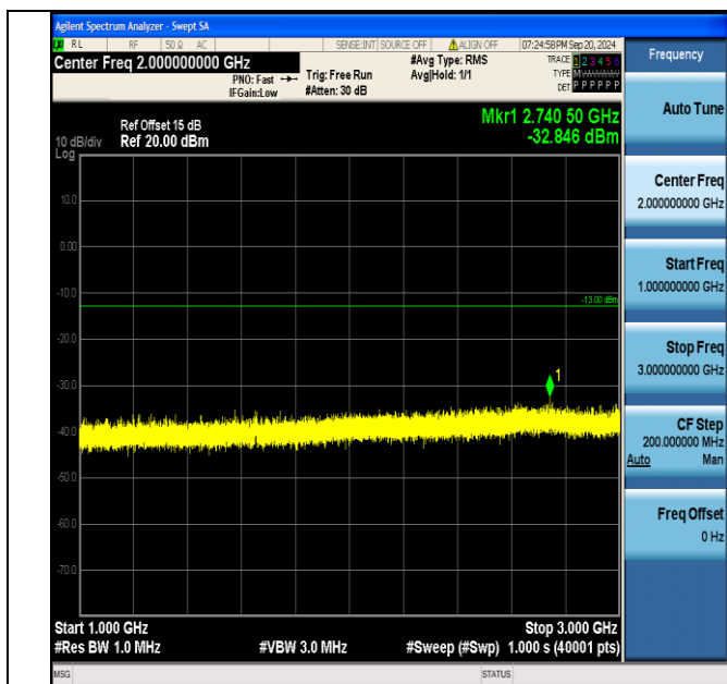
Band5_5MHz_16QAM_20425_25RB#0_1000~3000_1000~3000
