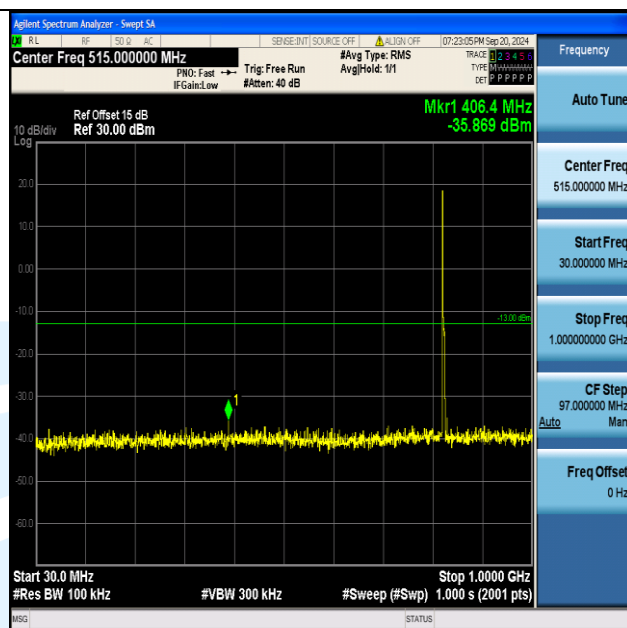
Band5_5MHz_16QAM_20425_1RB#0_30~1000_30~1000
