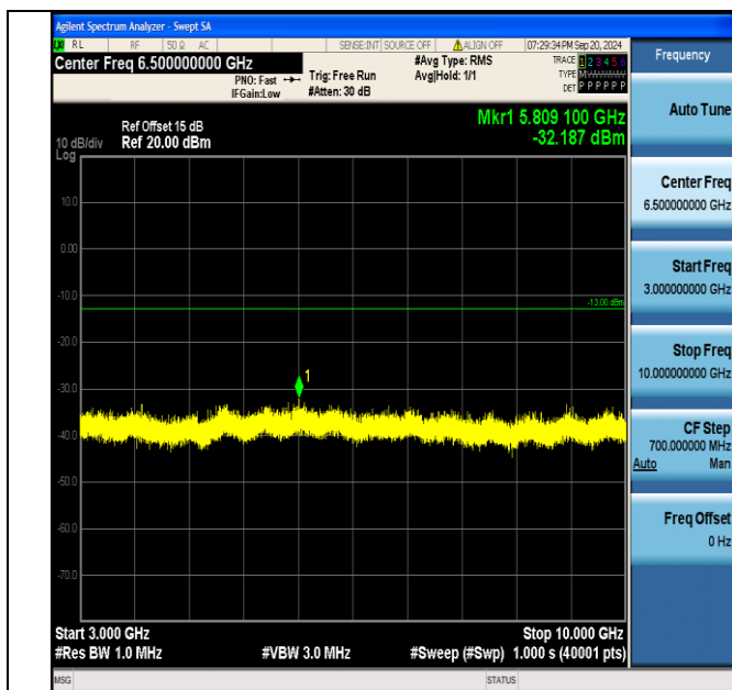
Band5_5MHz_16QAM_20625_1RB#24_3000~10000_3000~10000
