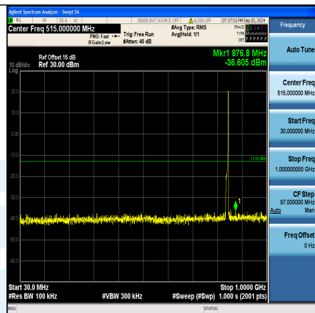
Band5_10MHz_QPSK_20600_1RB#49_30~1000_30~1000
