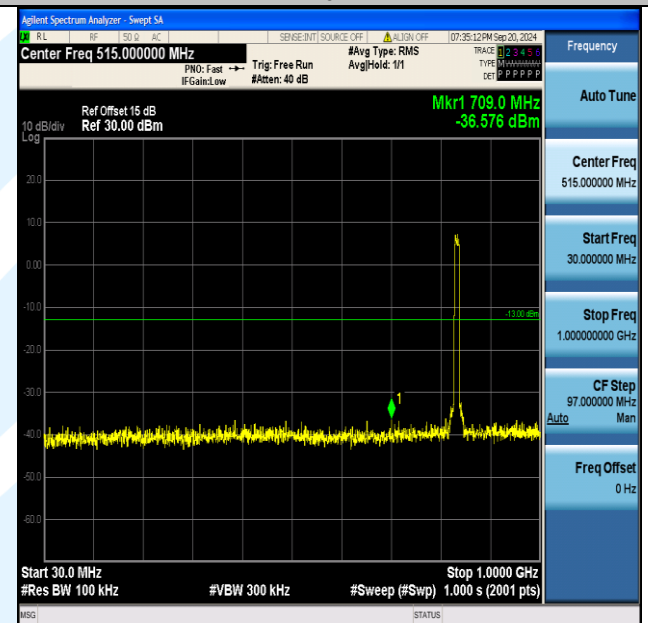
Band5_10MHz_QPSK_20525_50RB#0_30~1000_30~1000
