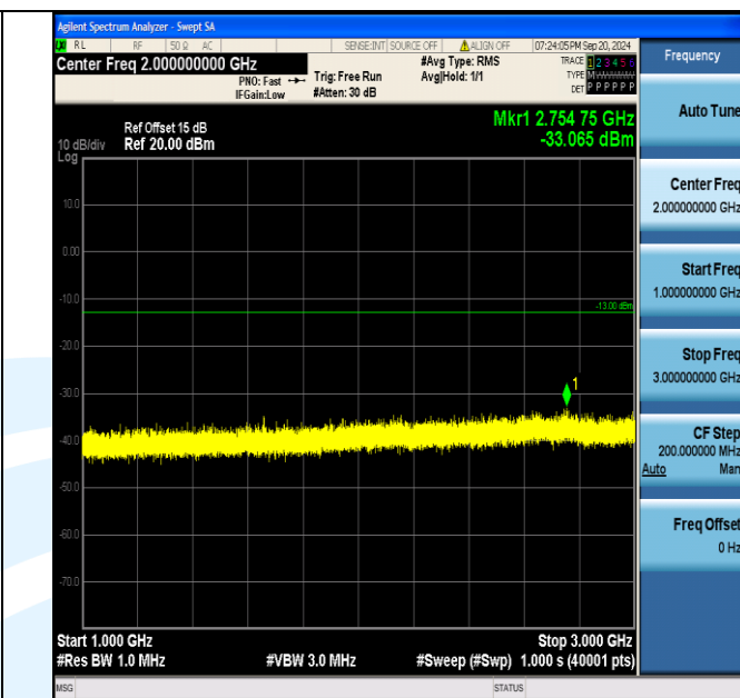
Band5_5MHz_16QAM_20425_1RB#24_1000~3000_1000~3000
