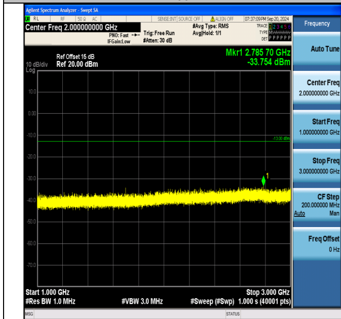
Band5_10MHz_QPSK_20600_1RB#49_1000~3000_1000~3000
