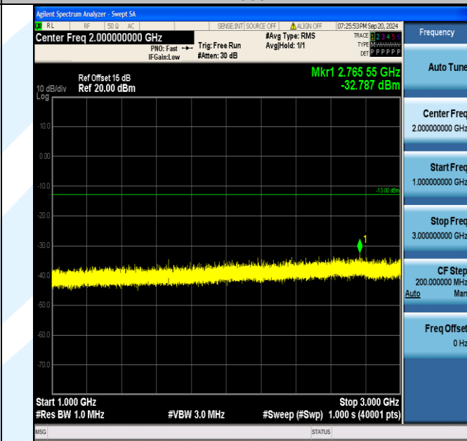
Band5_5MHz_16QAM_20525_1RB#0_1000~3000_1000~3000
