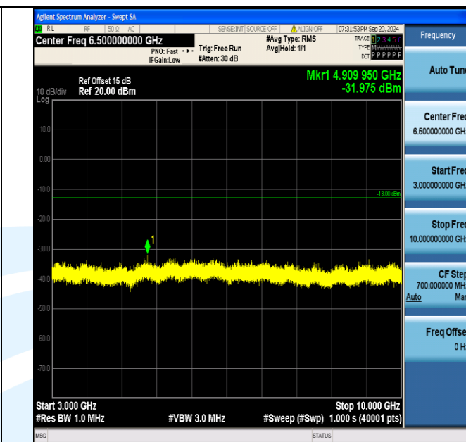
Band5_10MHz_QPSK_20450_1RB#49_3000~10000_3000~10000
