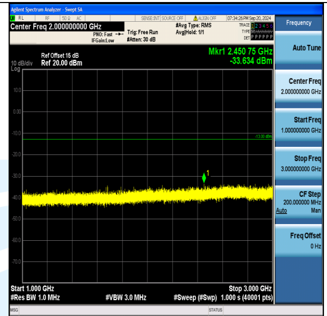
Band5_10MHz_QPSK_20525_1RB#49_1000~3000_1000~3000
