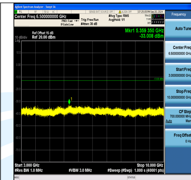
Band5_5MHz_16QAM_20425_25RB#0_3000~10000_3000~10000
