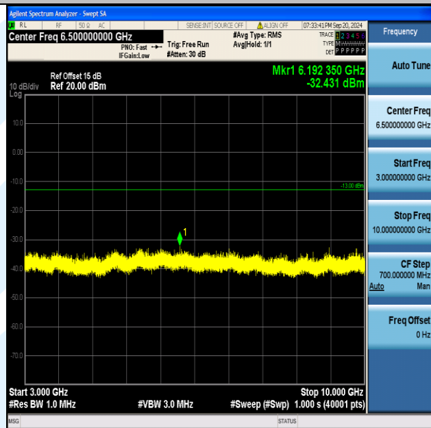
Band5_10MHz_QPSK_20525_1RB#0_3000~10000_3000~10000
