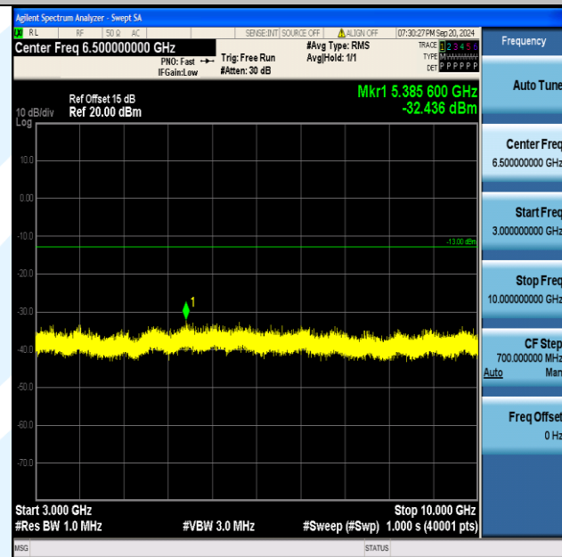
Band5_5MHz_16QAM_20625_25RB#0_3000~10000_3000~10000
