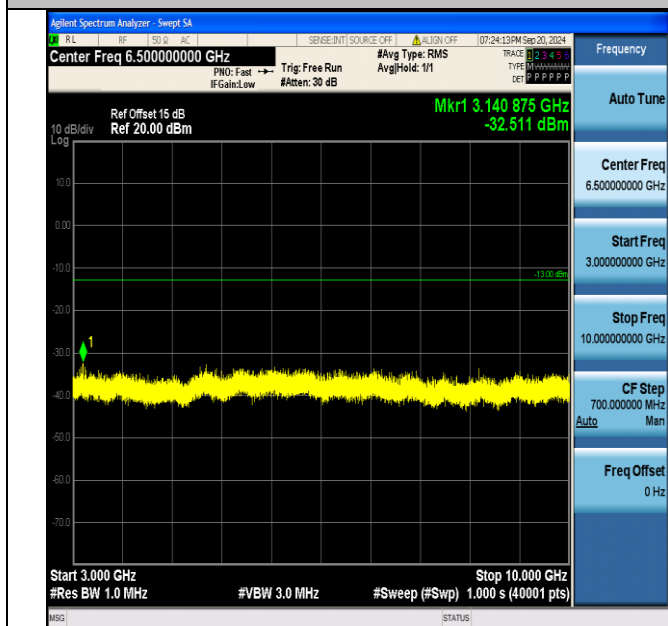
Band5_5MHz_16QAM_20425_1RB#24_3000~10000_3000~10000
