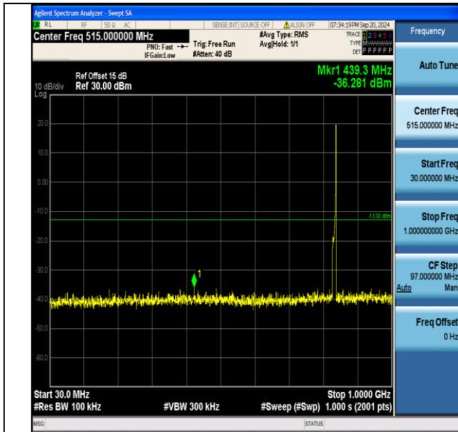
Band5_10MHz_QPSK_20525_1RB#49_30~1000_30~1000
