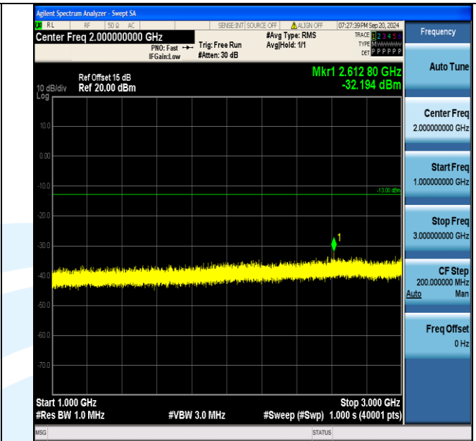
Band5_5MHz_16QAM_20525_25RB#0_1000~3000_1000~3000
