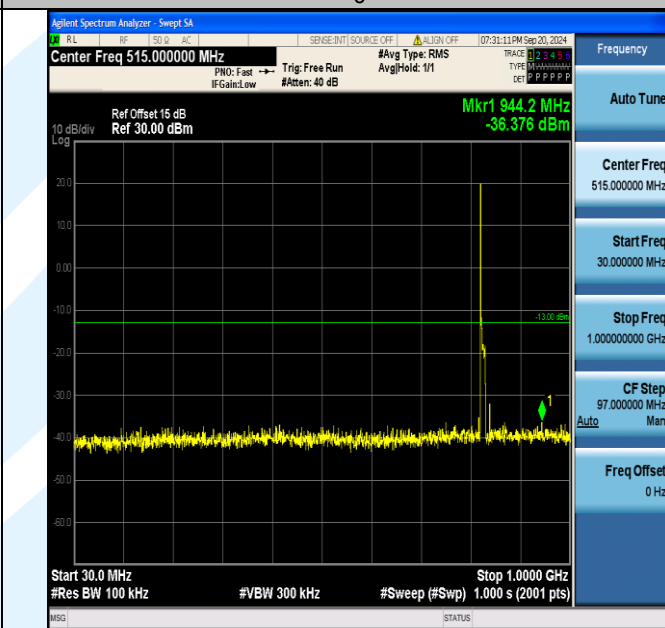
Band5_10MHz_16QAM_20450_1RB#0_30~1000_30~1000
