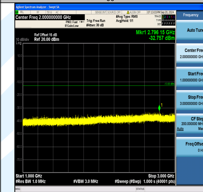
Band5_1.4MHz_QPSK_20643_6RB#0_1000~3000_1000~3000
