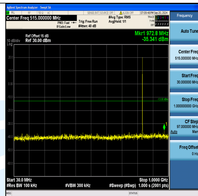
Band5_1.4MHz_16QAM_20525_1RB#5_30~1000_30~1000
