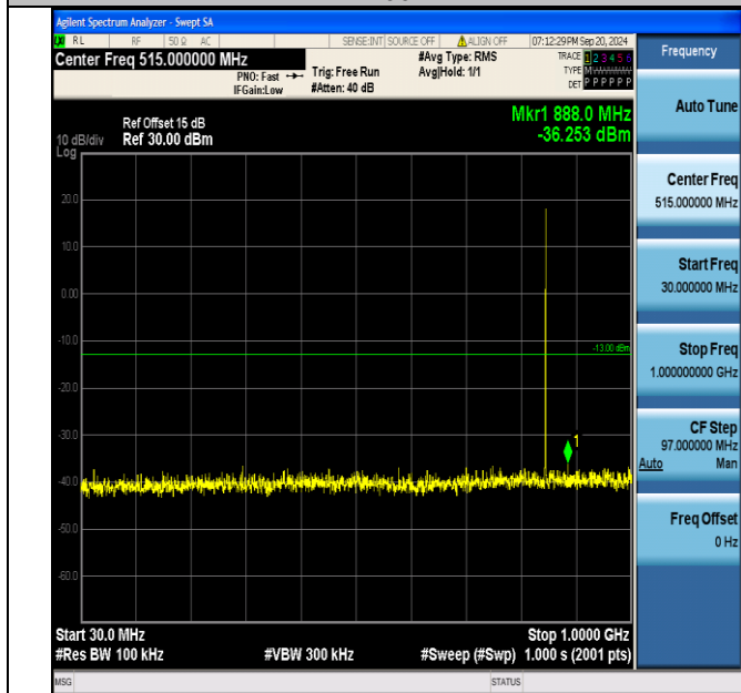
Band5_1.4MHz_16QAM_20643_1RB#5_30~1000_30~1000
