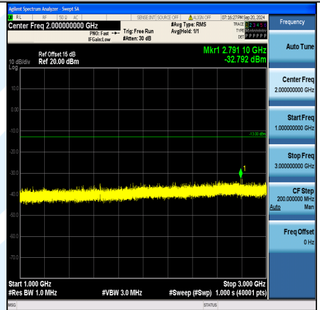
Band5_3MHz_QPSK_20415_15RB#0_1000~3000_1000~3000
