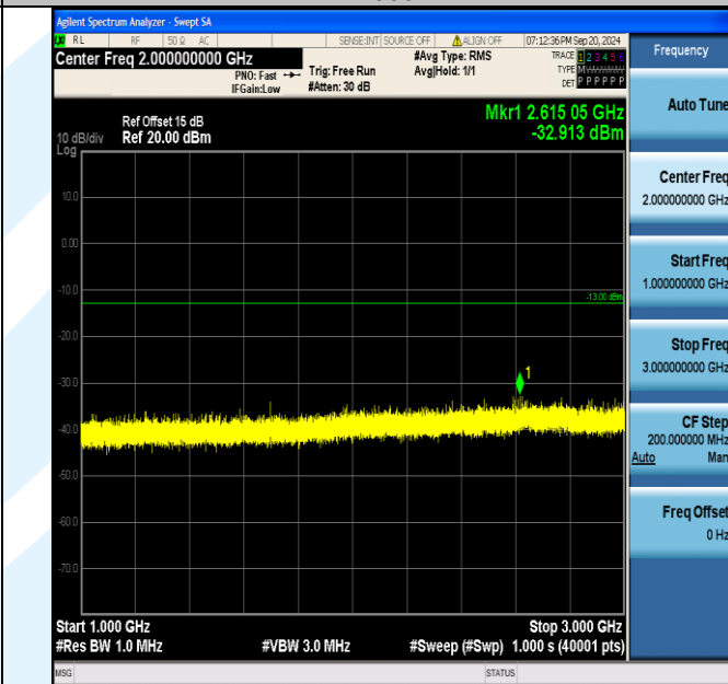
Band5_1.4MHz_16QAM_20643_1RB#5_1000~3000_1000~3000
