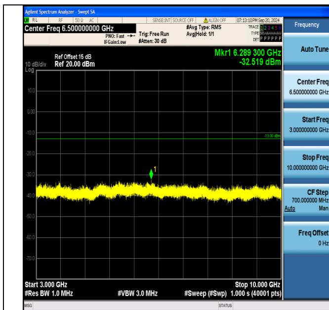
Band5_1.4MHz_QPSK_20643_6RB#0_3000~10000_3000~10000
