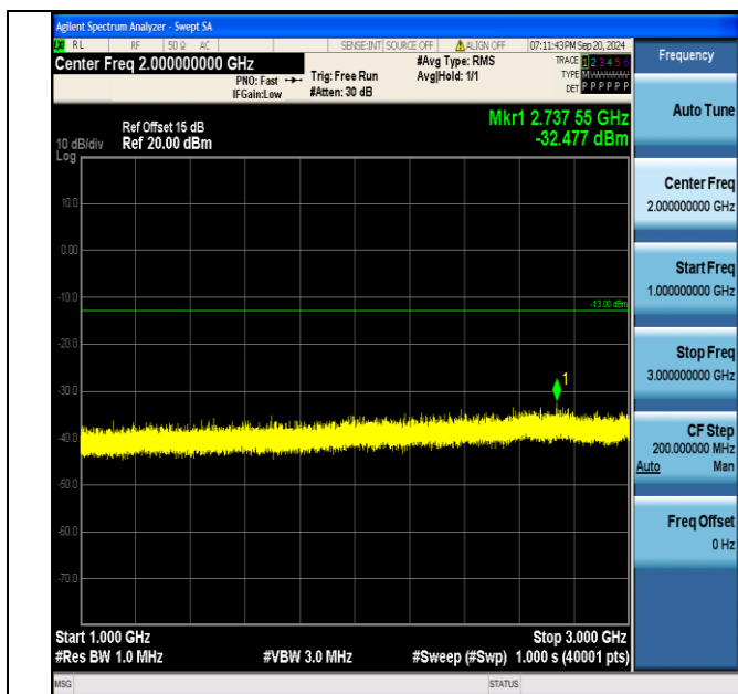
Band5_1.4MHz_16QAM_20643_1RB#0_1000~3000_1000~3000
