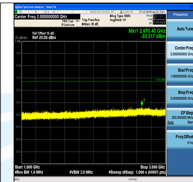
Band5_1.4MHz_16QAM_20525_6RB#0_1000~3000_1000~3000
