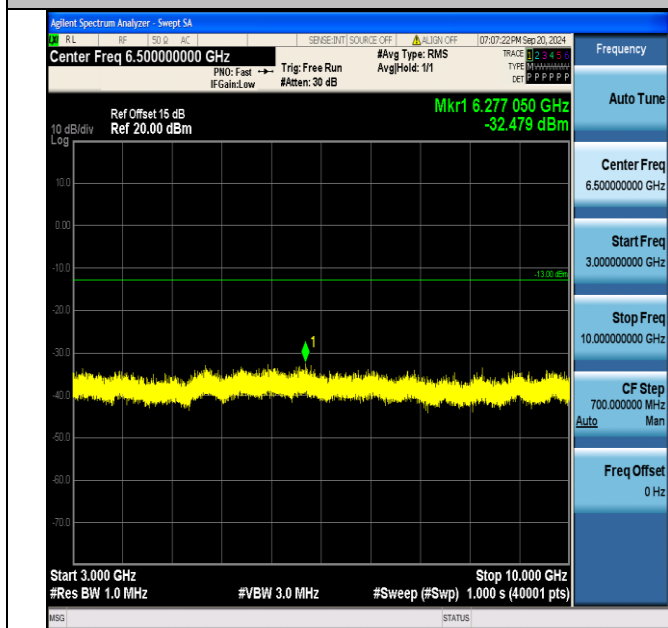
Band5_1.4MHz_16QAM_20407_1RB#5_3000~10000_3000~10000
