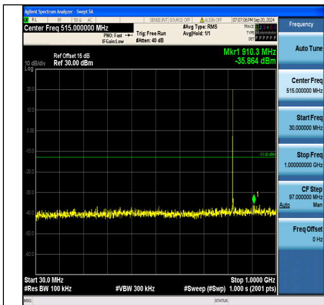
Band5_1.4MHz_16QAM_20407_1RB#5_30~1000_30~1000
