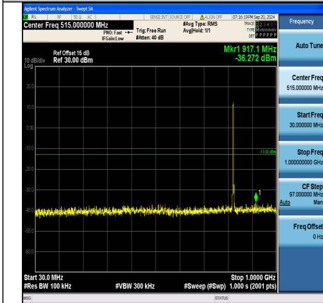
Band5_3MHz_QPSK_20415_15RB#0_30~1000_30~1000
