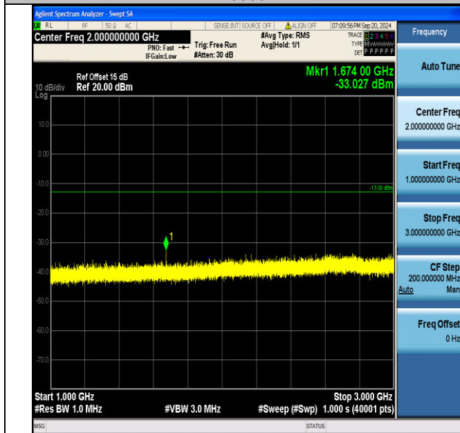
Band5_1.4MHz_16QAM_20525_1RB#5_1000~3000_1000~3000
