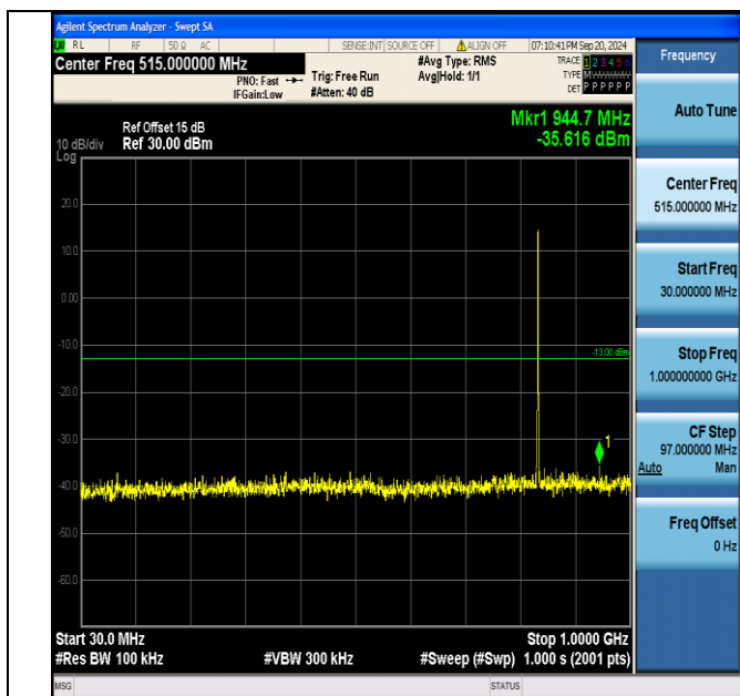
Band5_1.4MHz_16QAM_20525_6RB#0_30~1000_30~1000
