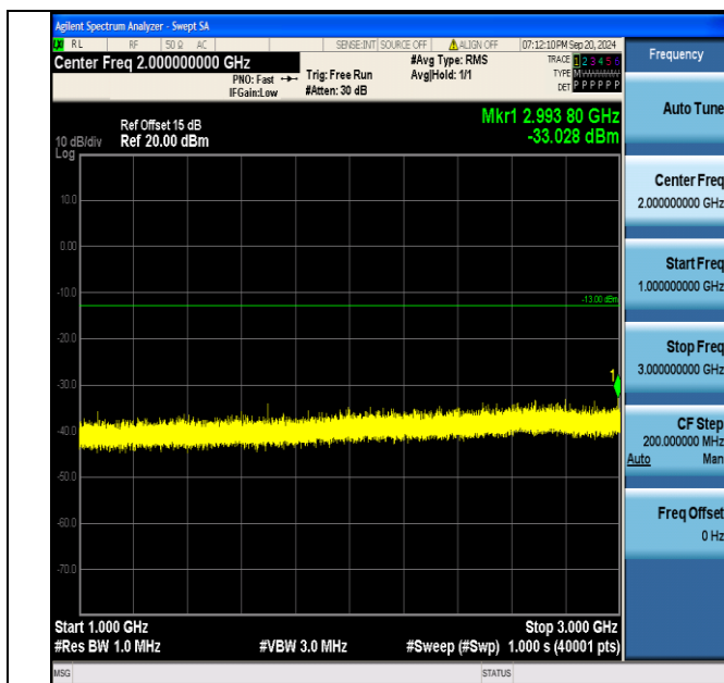
Band5_1.4MHz_QPSK_20643_1RB#5_1000~3000_1000~3000
