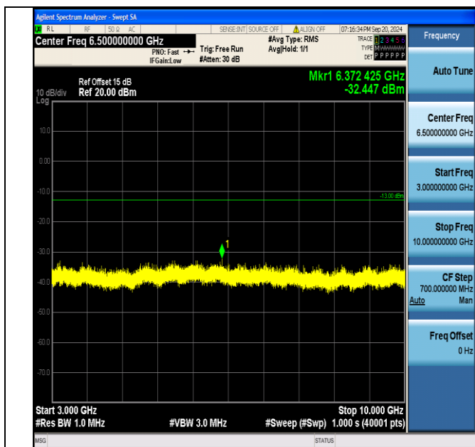
Band5_3MHz_QPSK_20415_15RB#0_3000~10000_3000~10000
