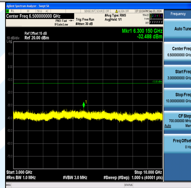
Band5_1.4MHz_16QAM_20525_1RB#5_3000~10000_3000~10000
