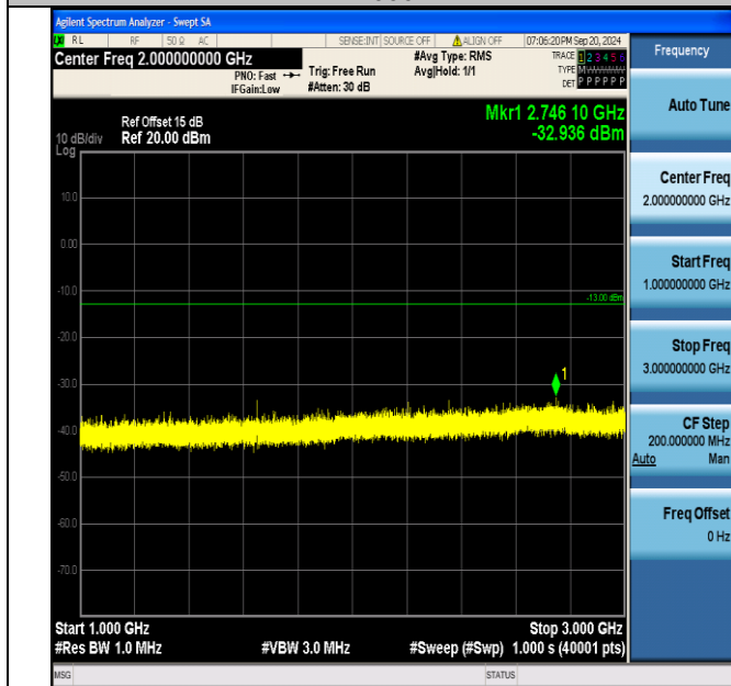
Band5_1.4MHz_16QAM_20407_1RB#0_1000~3000_1000~3000
