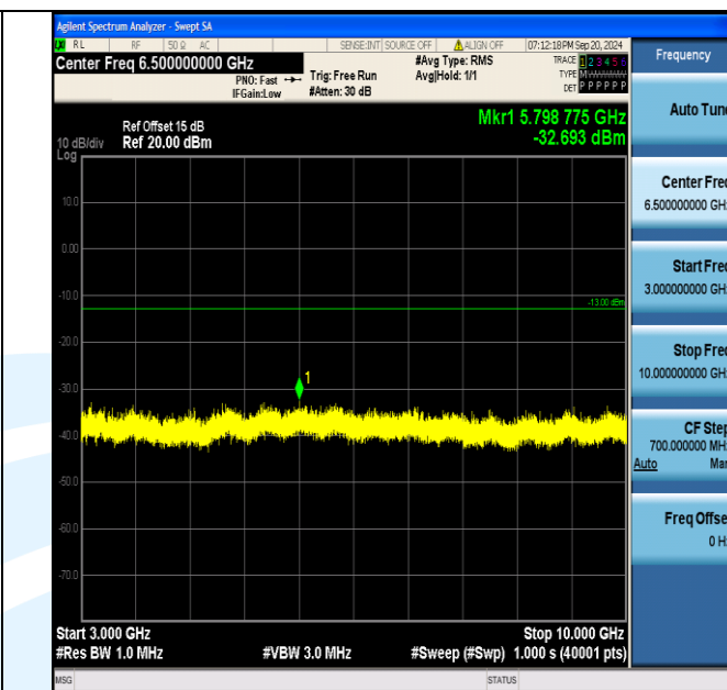
Band5_1.4MHz_QPSK_20643_1RB#5_3000~10000_3000~10000
