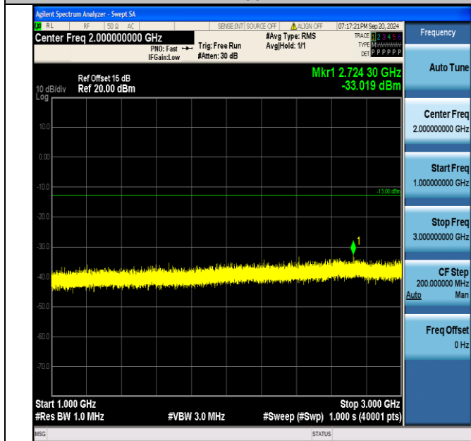
Band5_3MHz_QPSK_20525_1RB#0_1000~3000_1000~3000
