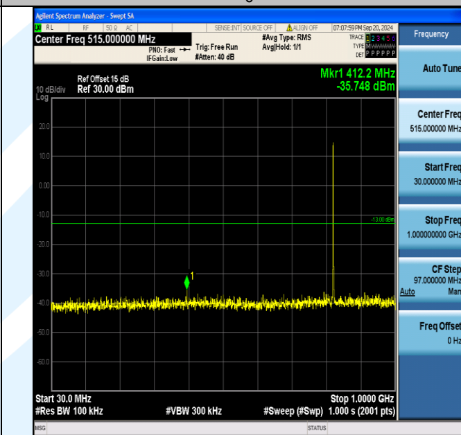
Band5_1.4MHz_16QAM_20407_6RB#0_30~1000_30~1000
