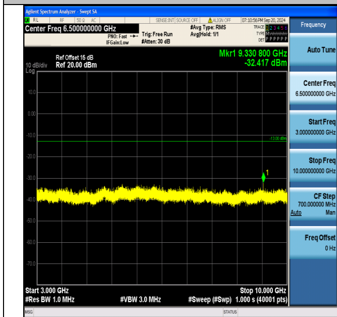
Band5_1.4MHz_16QAM_20525_6RB#0_3000~10000_3000~10000
