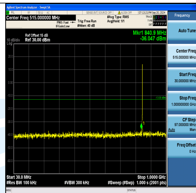
Band5_1.4MHz_16QAM_20643_6RB#0_30~1000_30~1000
