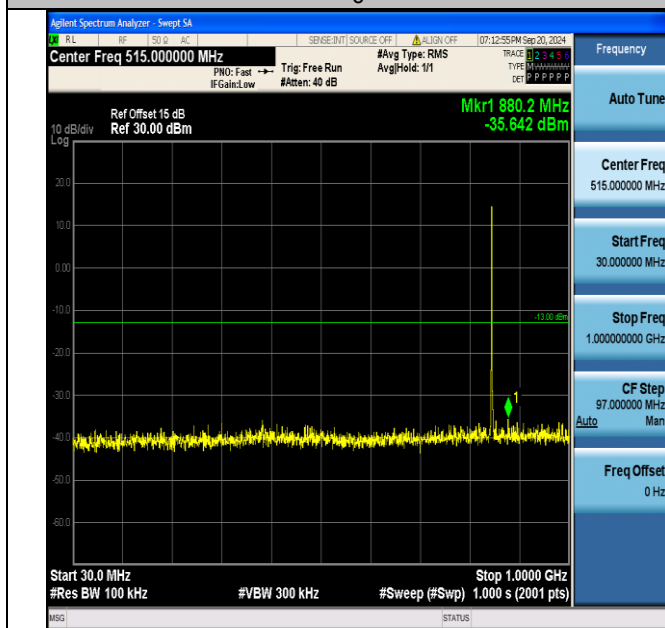
Band5_1.4MHz_QPSK_20643_6RB#0_30~1000_30~1000
