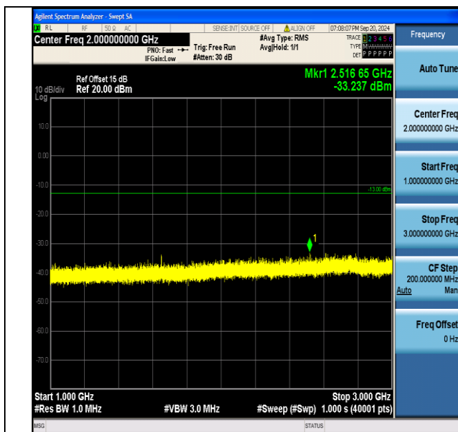
Band5_1.4MHz_16QAM_20407_6RB#0_1000~3000_1000~3000
