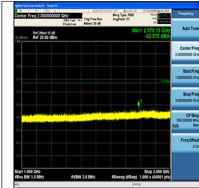
Band5_3MHz_QPSK_20415_1RB#14_1000~3000_1000~3000
