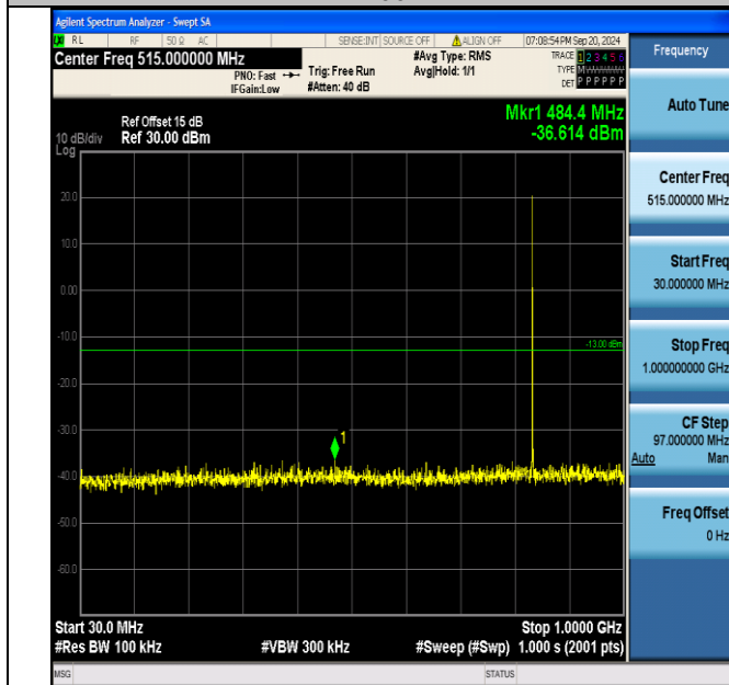
Band5_1.4MHz_16QAM_20525_1RB#0_30~1000_30~1000
