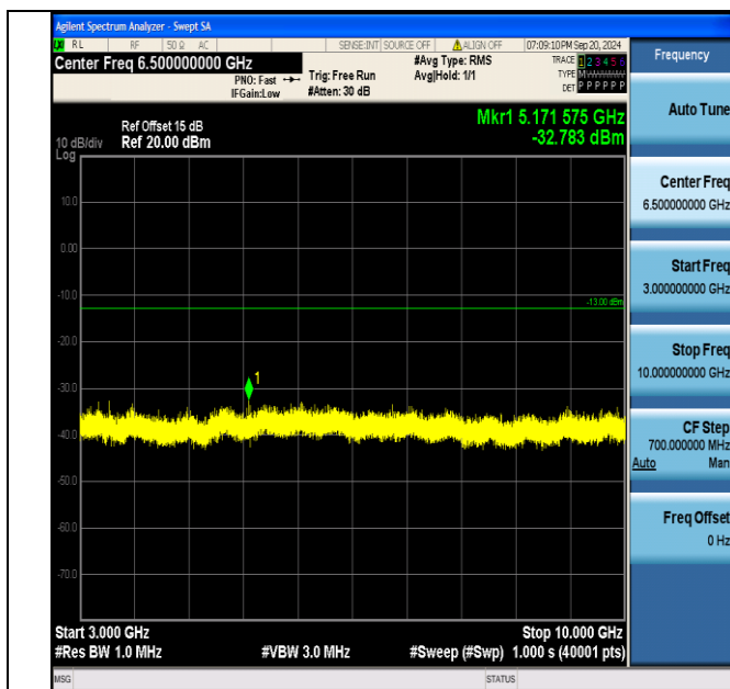
Band5_1.4MHz_16QAM_20525_1RB#0_3000~10000_3000~10000
