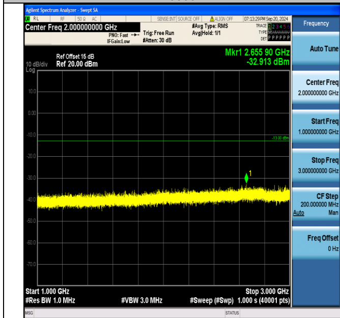
Band5_1.4MHz_16QAM_20643_6RB#0_1000~3000_1000~3000
