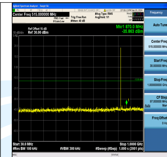
Band5_1.4MHz_16QAM_20407_1RB#0_30~1000_30~1000
