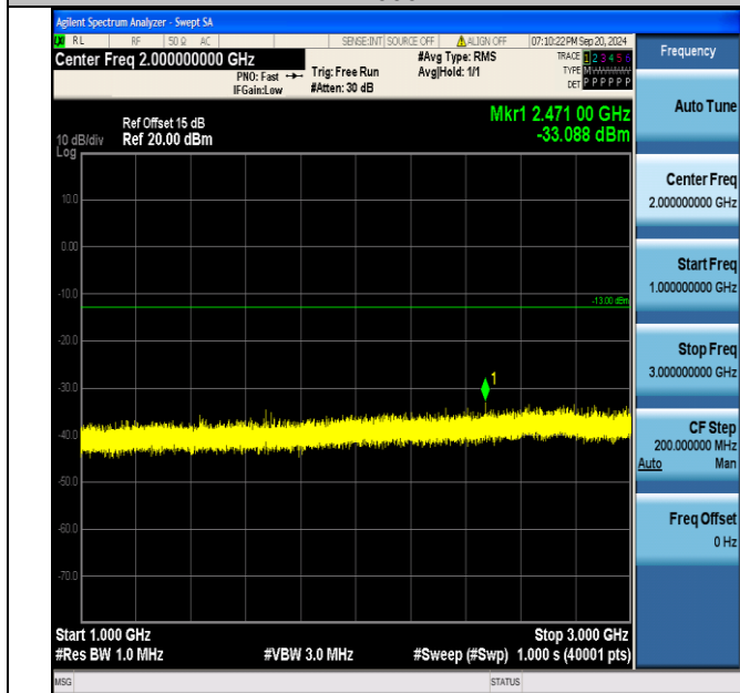
Band5_1.4MHz_QPSK_20525_6RB#0_1000~3000_1000~3000
