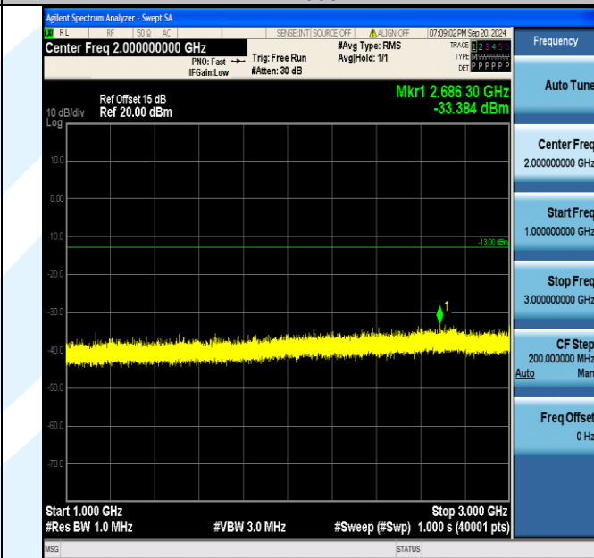
Band5_1.4MHz_16QAM_20525_1RB#0_1000~3000_1000~3000
