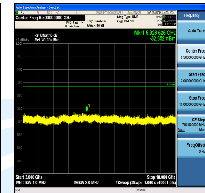
Band5_1.4MHz_16QAM_20407_6RB#0_3000~10000_3000~10000
