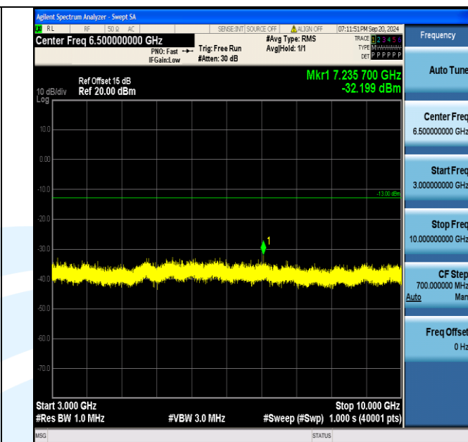
Band5_1.4MHz_16QAM_20643_1RB#0_3000~10000_3000~10000
