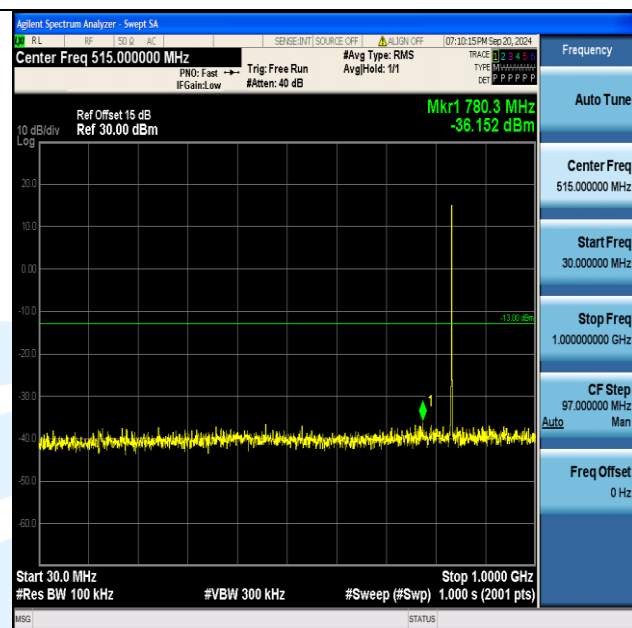
Band5_1.4MHz_QPSK_20525_6RB#0_30~1000_30~1000
