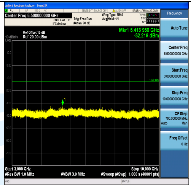
Band5_3MHz_QPSK_20415_1RB#14_3000~10000_3000~10000
