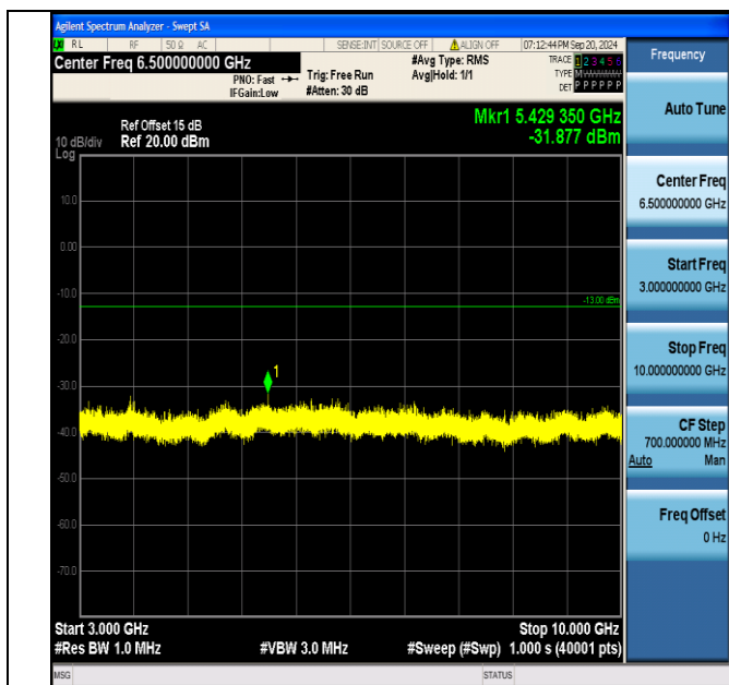
Band5_1.4MHz_16QAM_20643_1RB#5_3000~10000_3000~10000
