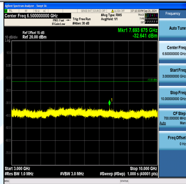
Band5_1.4MHz_QPSK_20525_6RB#0_3000~10000_3000~10000
