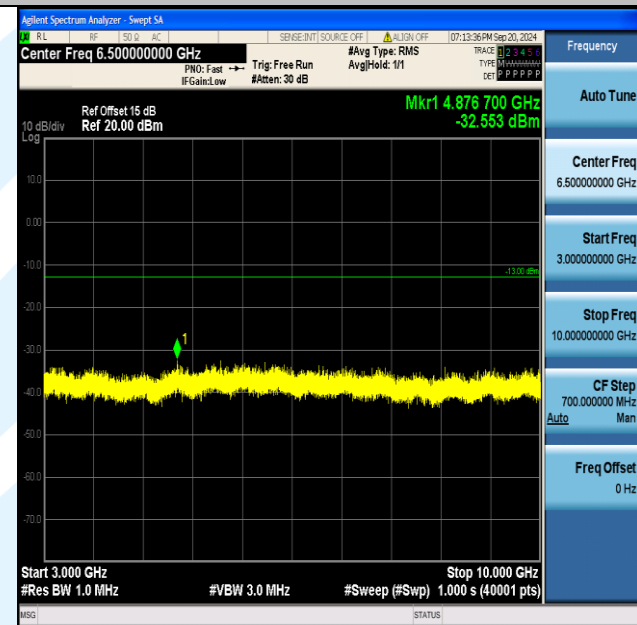
Band5_1.4MHz_16QAM_20643_6RB#0_3000~10000_3000~10000
