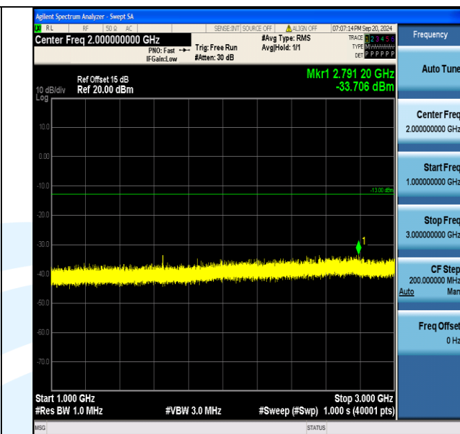
Band5_1.4MHz_16QAM_20407_1RB#5_1000~3000_1000~3000 0
