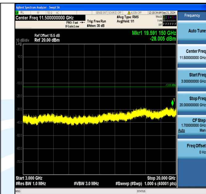
Band4_15MHz_QPSK_20325_1RB#74_3000~20000_3000~20000
