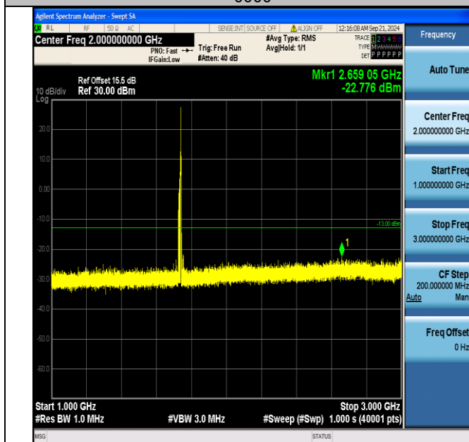
Band4_15MHz_16QAM_20175_1RB#74_1000~3000_1000~3000
