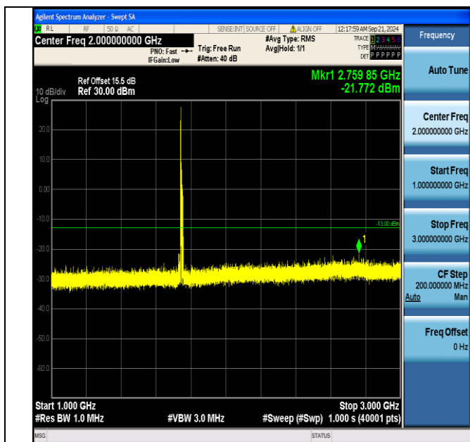
Band4_15MHz_16QAM_20325_1RB#0_1000~3000_1000~3000
