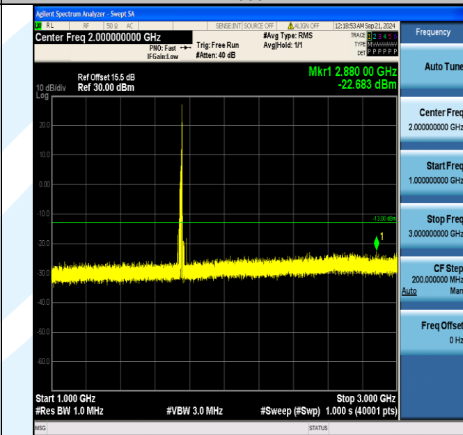
Band4_15MHz_16QAM_20325_1RB#74_1000~3000_1000~3000
