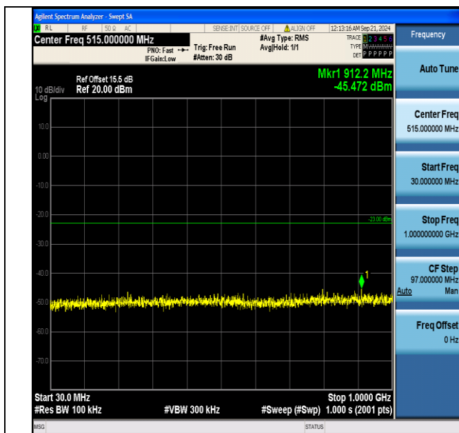
Band4_15MHz_16QAM_20025_1RB#74_30~1000_30~1000
