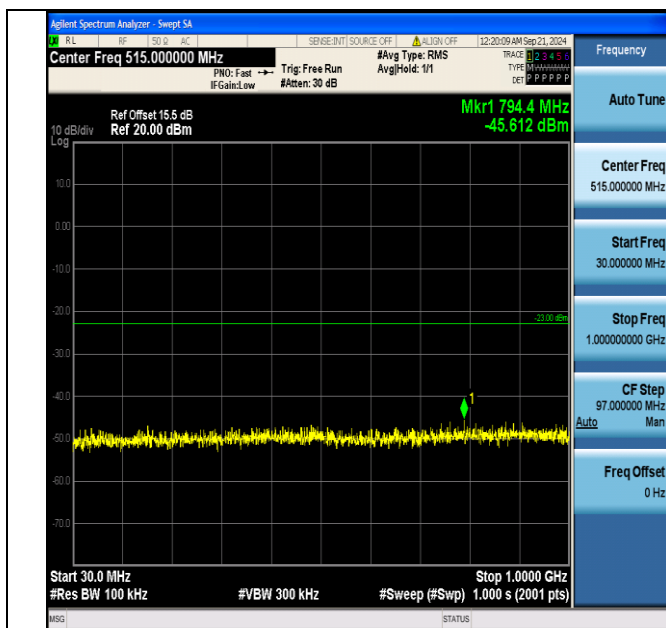
Band4 20MHz QPSK 20050 1RB#0 30~1000 30~1000
