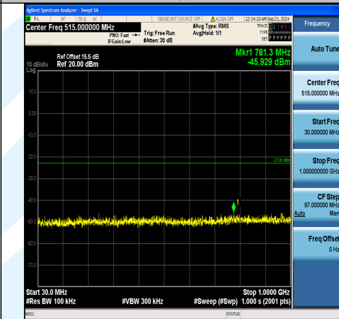
Band4_15MHz_16QAM_20025_75RB#0_30~1000_30~1000
