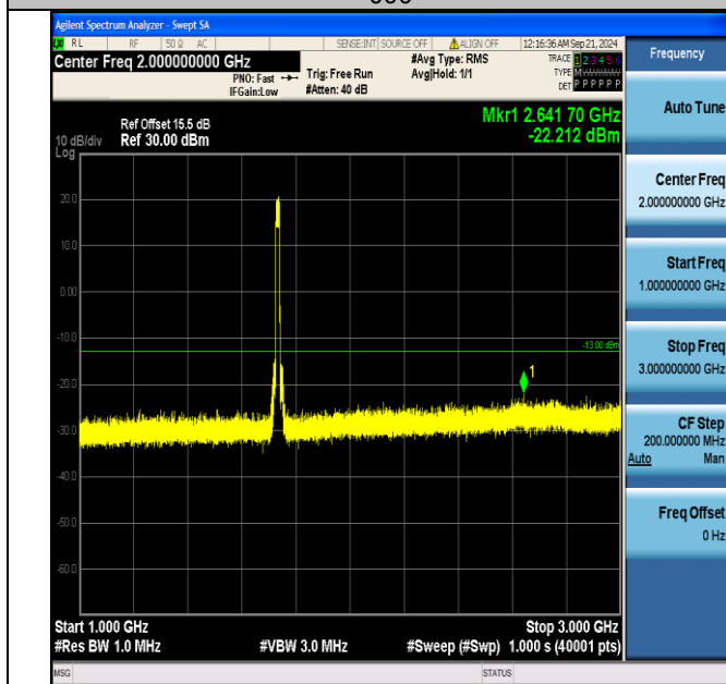
Band4_15MHz_QPSK_20175_75RB#0_1000~3000_1000~3000
