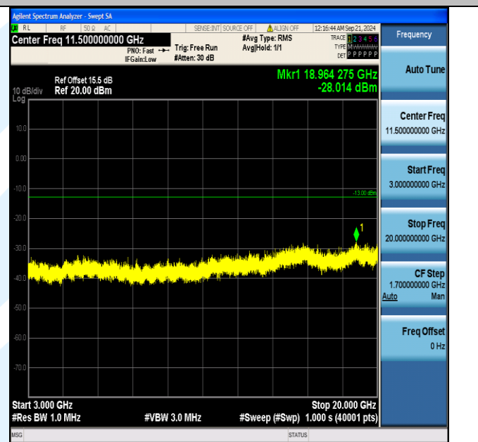
Band4_15MHz_QPSK_20175_75RB#0_3000~20000_3000~20000
