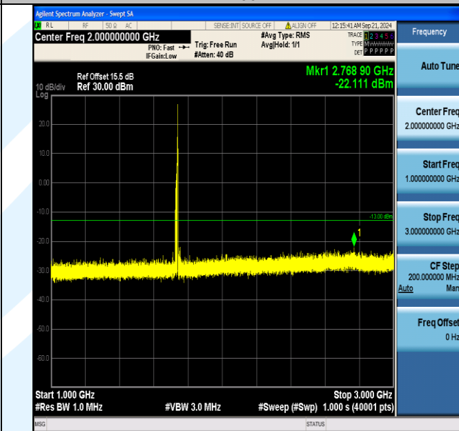
Band4_15MHz_QPSK_20175_1RB#74_1000~3000_1000~3000
