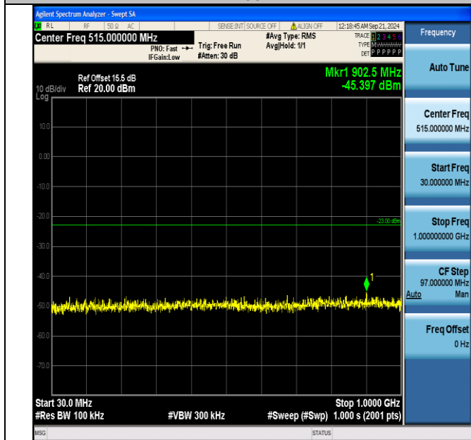
Band4_15MHz_16QAM_20325_1RB#74_30~1000_30~1000
