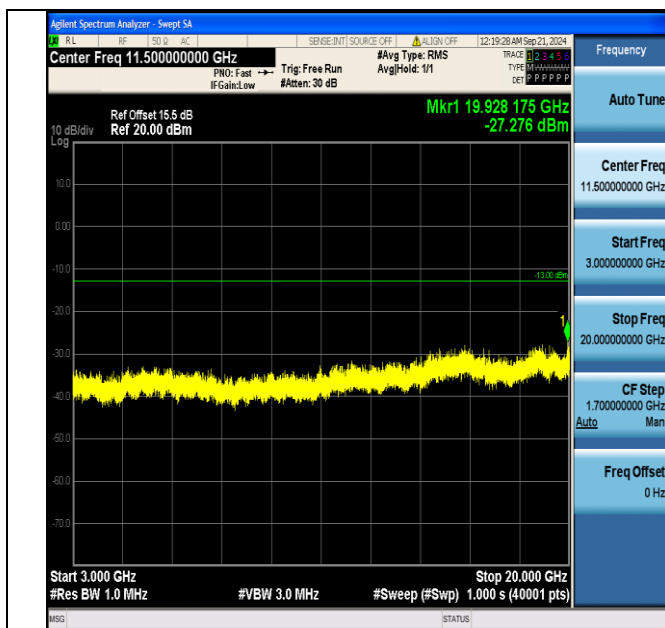
Band4_15MHz_QPSK_20325_75RB#0_3000~20000_3000~20000
