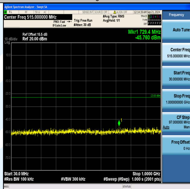
Band4_15MHz_QPSK_20175_1RB#0_30~1000_30~1000
