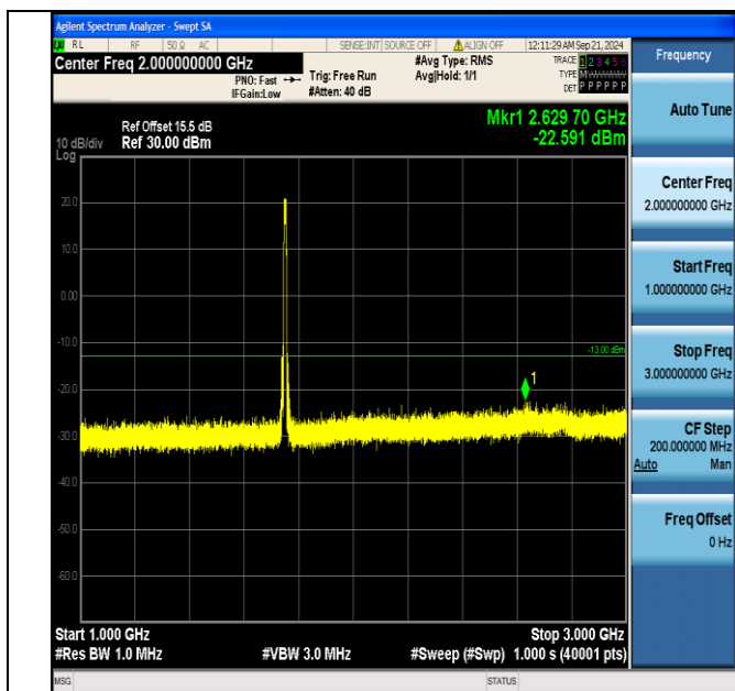
Band4_10MHz_16QAM_20350_50RB#0_1000~3000_1000~3000
