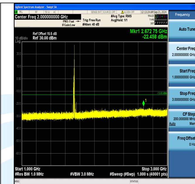
Band4_15MHz_16QAM_20025_1RB#74_1000~3000_1000~3000
