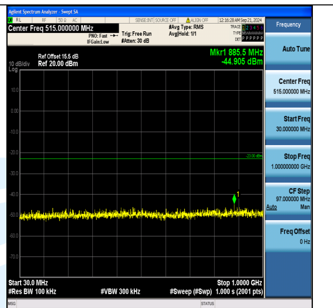
Band4_15MHz_QPSK_20175_75RB#0_30~1000_30~1000
