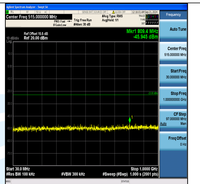
Band4_15MHz_16QAM_20175_1RB#74_30~1000_30~1000
