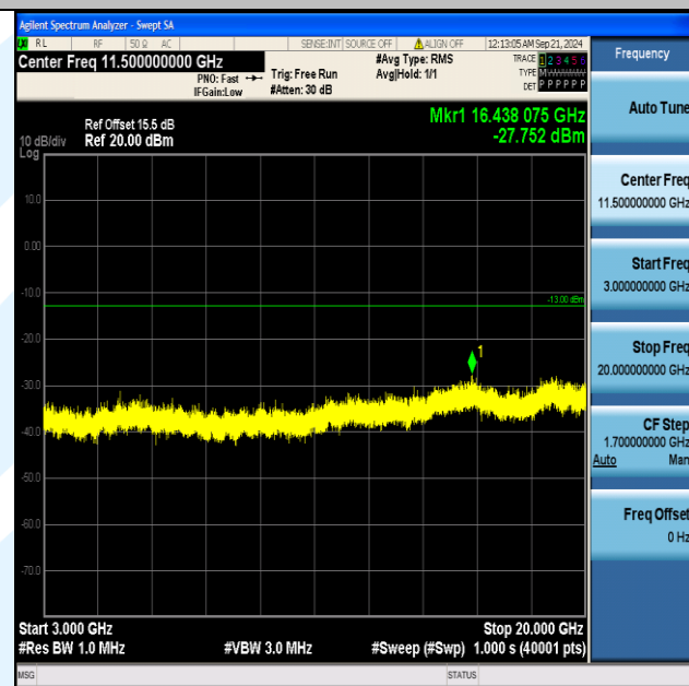
Band4_15MHz_QPSK_20025_1RB#74_3000~20000_3000~20000
