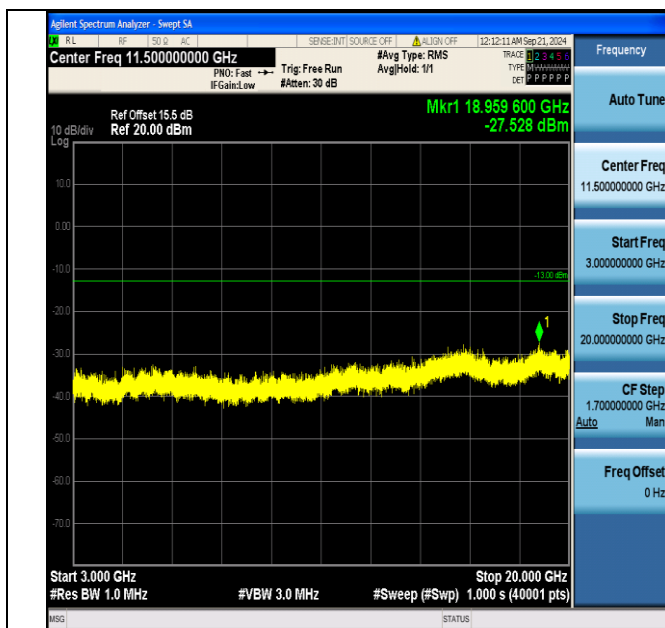
Band4_15MHz_QPSK_20025_1RB#0_3000~20000_3000~20000
