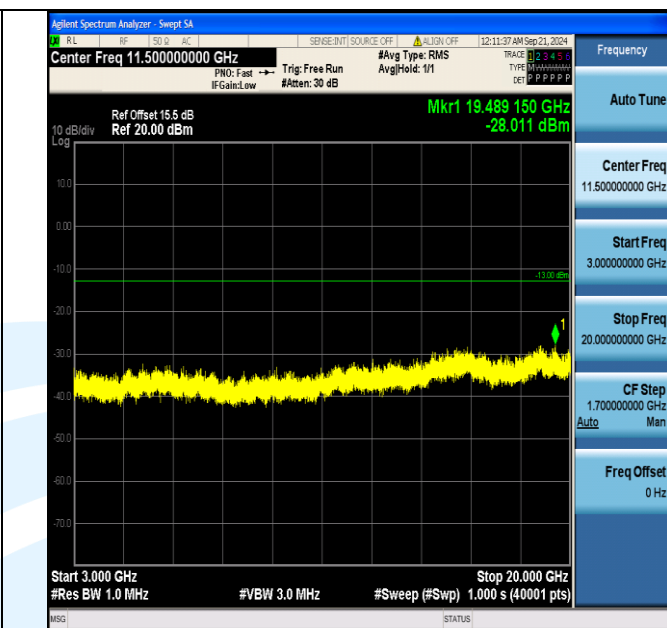
Band4_10MHz_16QAM_20350_50RB#0_3000~20000_3000~20000
