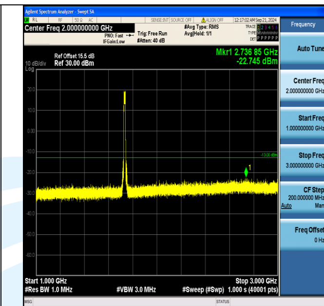
Band4_15MHz_16QAM_20175_75RB#0_1000~3000_1000~3000
