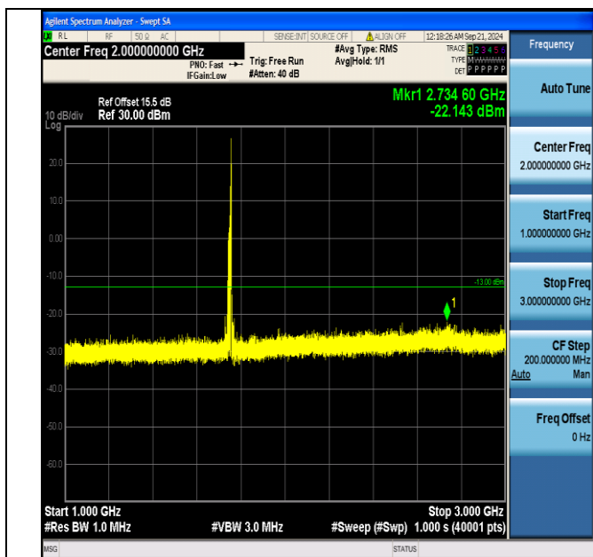
Band4_15MHz_QPSK_20325_1RB#74_1000~3000_1000~3000
