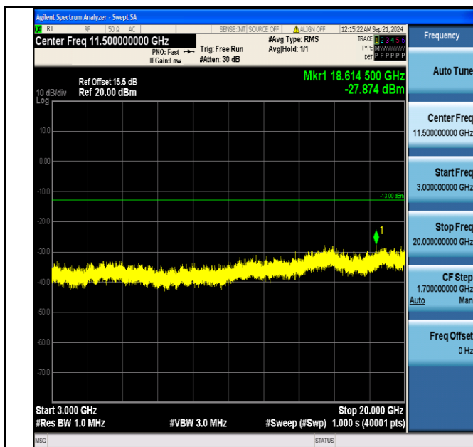
Band4_15MHz_16QAM_20175_1RB#0_3000~20000_3000~20000
