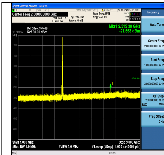
Band4_15MHz_QPSK_20175_1RB#0_1000~3000_1000~3000
