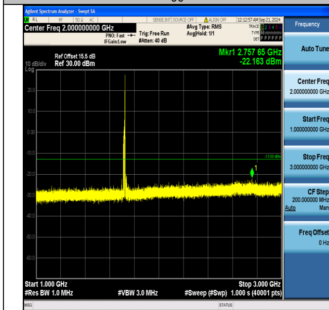
Band4_15MHz_QPSK_20025_1RB#74_1000~3000_1000~3000
