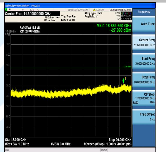
Band4_15MHz_16QAM_20175_1RB#74_3000~20000_3000~20000
