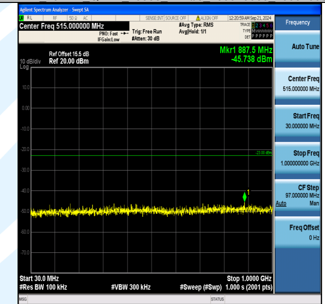
Band4_20MHz_QPSK_20050_1RB#99_30~1000_30~1000
