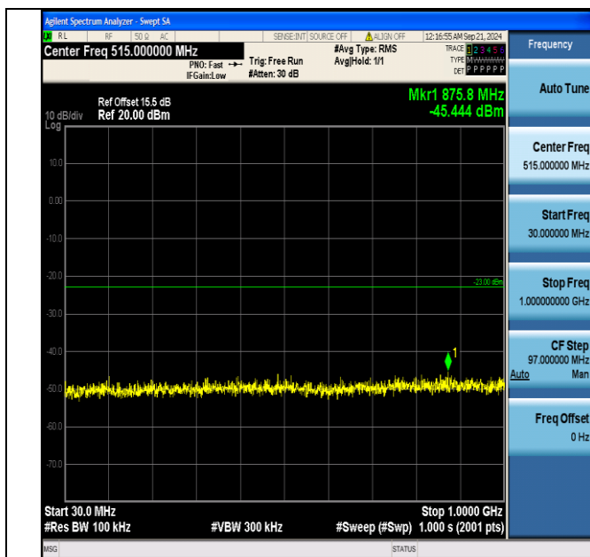
Band4_15MHz_16QAM_20175_75RB#0_30~1000_30~1000
