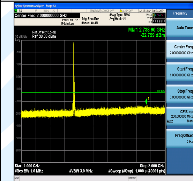
Band4_15MHz_16QAM_20175_1RB#0_1000~3000_1000~3000
