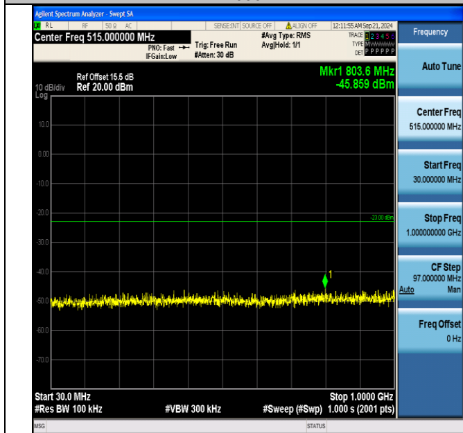
Band4_15MHz_QPSK_2025_1RB#0_30~1000_30~1000
