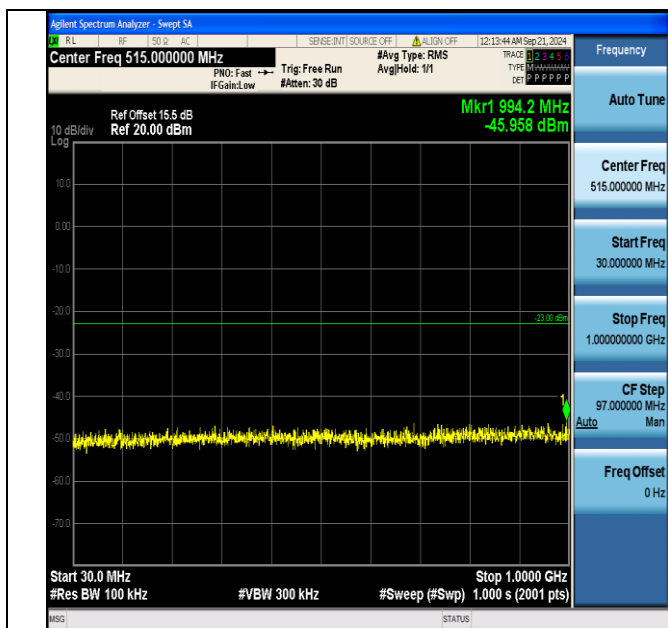
Band4_15MHz_QPSK_20025_75RB#0_30~1000_30~1000
