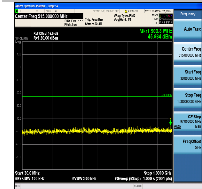
Band4_15MHz_16QAM_20175_1RB#0_30~1000_30~1000
