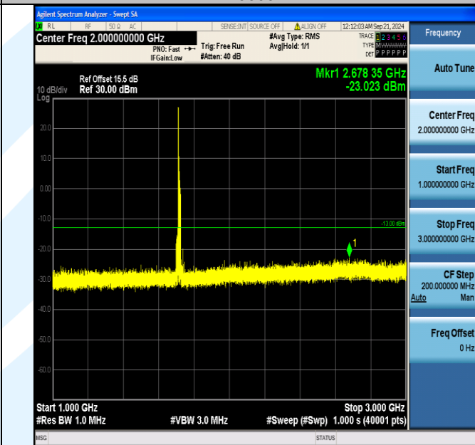
Band4_15MHz_QPSK_2025_1RB#0_1000~3000_1000~3000
