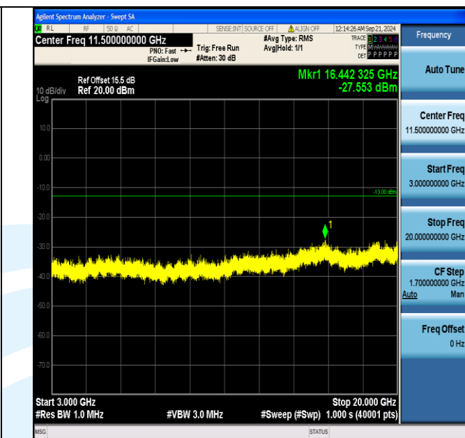
Band4_15MHz_16QAM_20025_75RB#0_3000~20000_3000~20000
