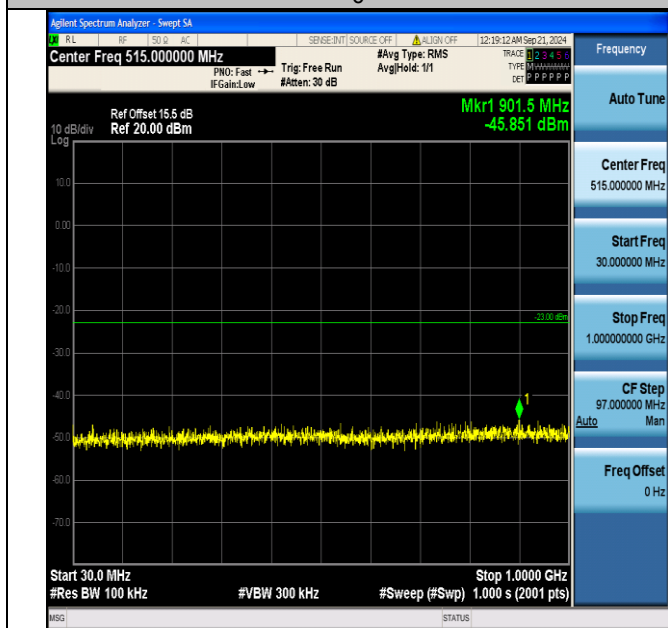
Band4_15MHz_QPSK_20325_75RB#0_30~1000_30~1000
