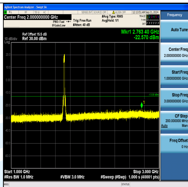
Band4_15MHz_QPSK_20025_75RB#0_1000~3000_1000~3000 0
