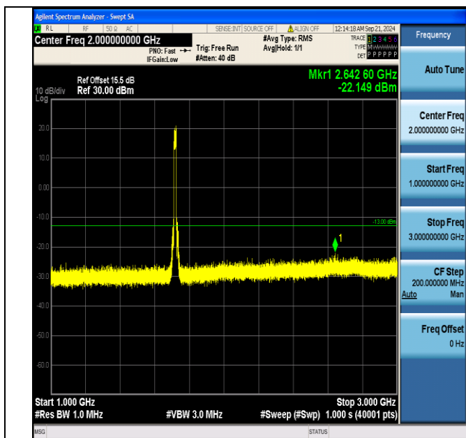
Band4_15MHz_16QAM_20025_75RB#0_1000~3000_1000~3000
