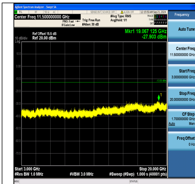
Band4_15MHz_QPSK_20175_1RB#74_3000~20000_3000~20000
