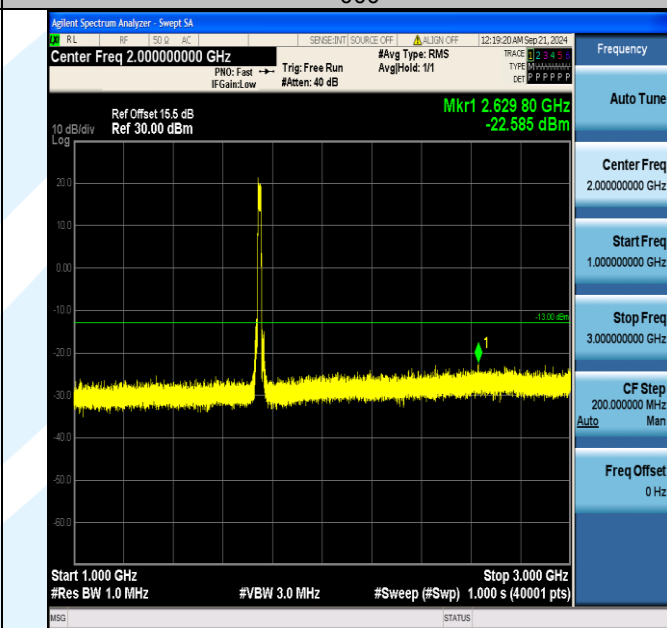
Band4_15MHz_QPSK_20325_75RB#0_1000~3000_1000~3000
