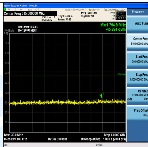
Band4_15MHz_QPSK_20025_1RB#74_30~1000_30~1000
