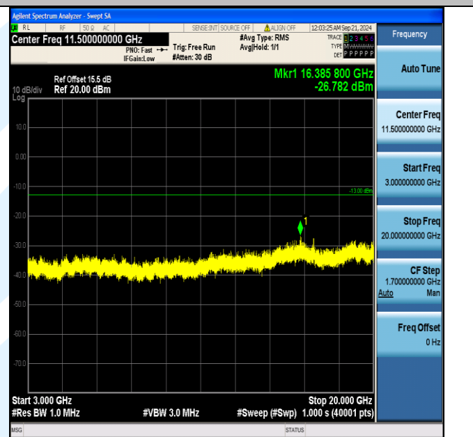
Band4_5MHz_16QAM_20375_25RB#0_3000~20000_3000~20000
