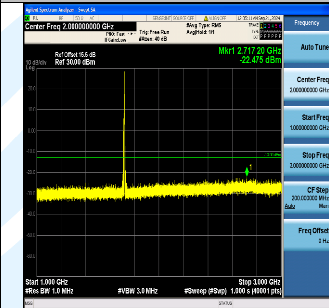
Band4_10MHz_16QAM_20000_1RB#49_1000~3000_1000~3000
