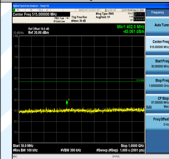
Band4_10MHz_16QAM_20175_1RB#49_30~1000_30~1000
