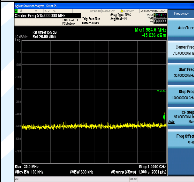
Band4_10MHz_QPSK_20000_1RB#49_30~1000_30~1000
