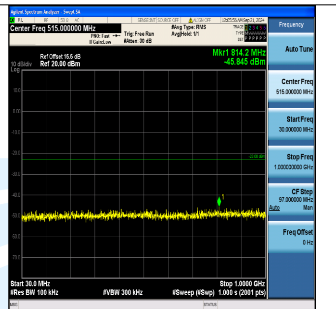
Band4_10MHz_16QAM_20000_50RB#0_30~1000_30~1000
