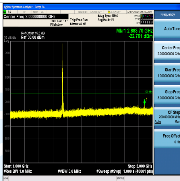
Band4_10MHz_QPSK_20175_1RB#49_1000~3000_1000~3000
