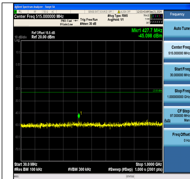
Band4_10MHz_QPSK_20000_1RB#0_30~1000_30~1000
