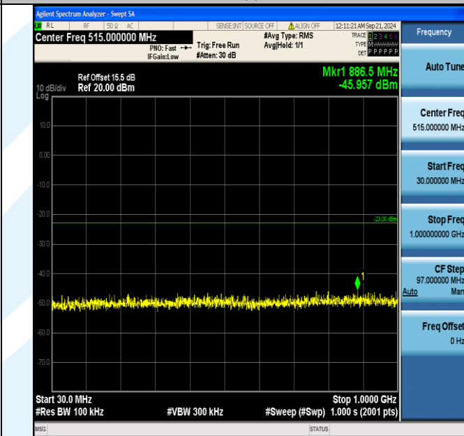
Band4_10MHz_16QAM_20350_50RB#0_30~1000_30~1000
