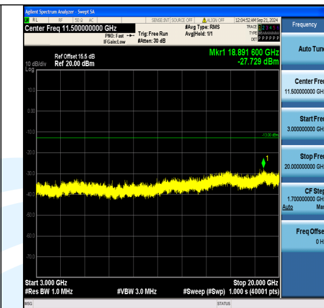
Band4_10MHz_QPSK_20000_1RB#49_3000~20000_3000~20000
