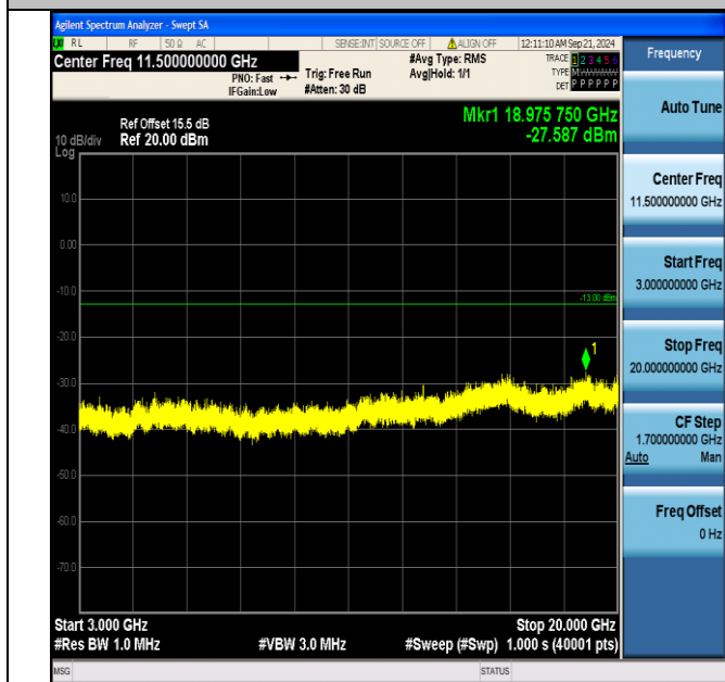
Band4_10MHz_QPSK_20350_50RB#0_3000~20000_3000~20000
