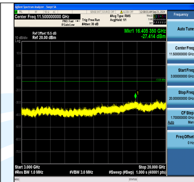
Band4_10MHz_16QAM_20175_1RB#49_3000~20000_3000~20000
