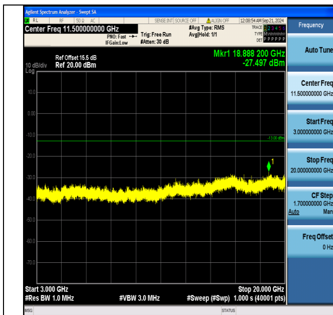
Band4_10MHz_16QAM_20175_50RB#0_3000~20000_3000~20000
