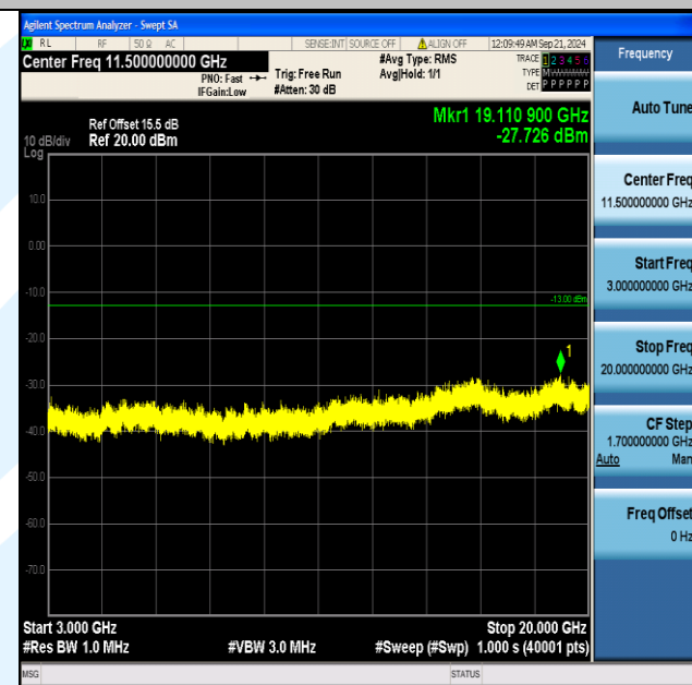
Band4_10MHz_16QAM_20350_1RB#0_3000~20000_3000~20000
