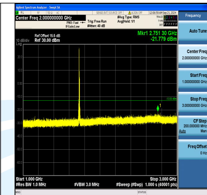
Band4_10MHz_16QAM_20175_1RB#0_1000~3000_1000~3000
