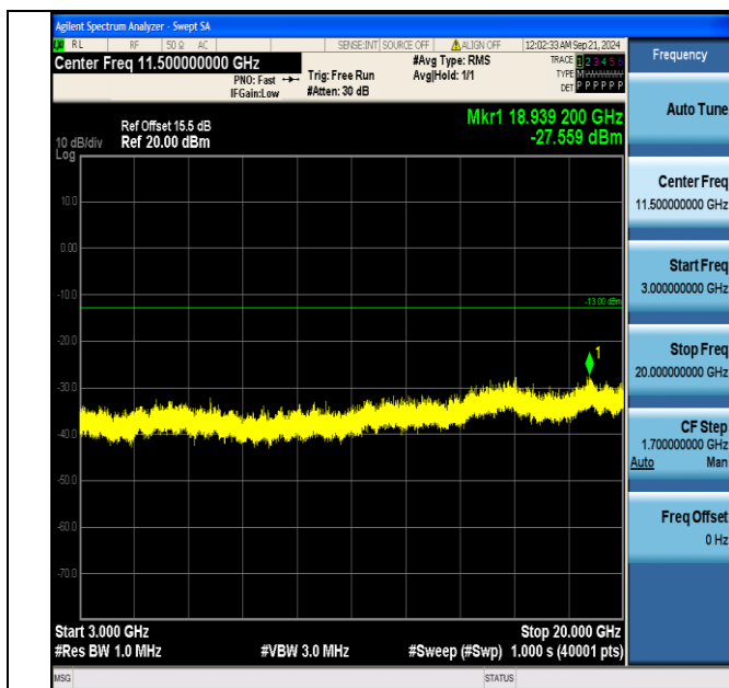
Band4_5MHz_16QAM_20375_1RB#24_3000~20000_3000~20000
