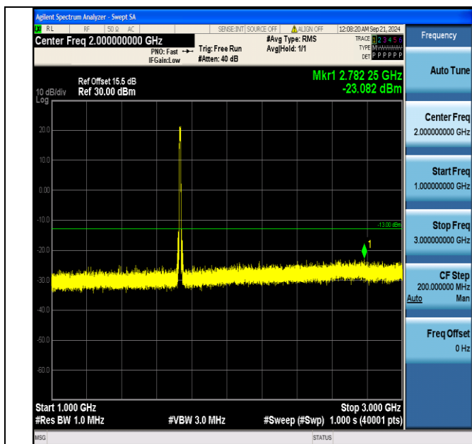
Band4_10MHz_QPSK_20175_50RB#0_1000~3000_1000~3000
