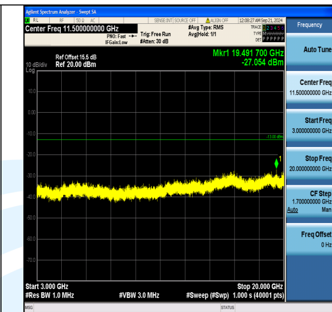
Band4_10MHz_QPSK_20175_50RB#0_3000~20000_3000~20000
