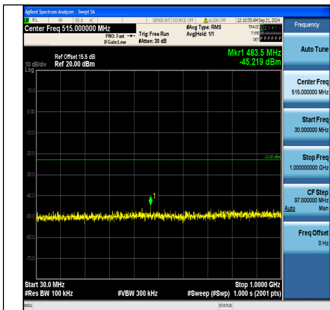
Band4_10MHz_QPSK_20350_50RB#0_30~1000_30~1000
