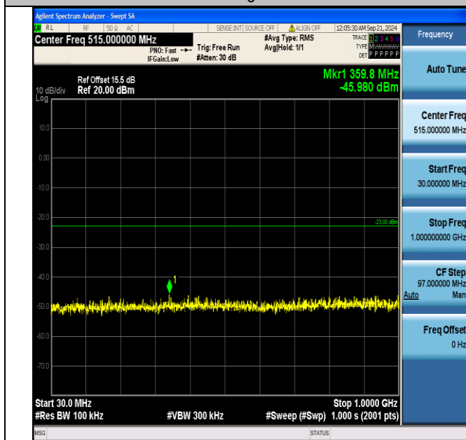
Band4_10MHz_QPSK_20000_50RB#0_30~1000_30~1000
