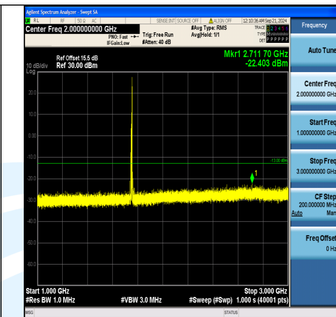
Band4_10MHz_16QAM_20350_1RB#49_1000~3000_1000~3000
