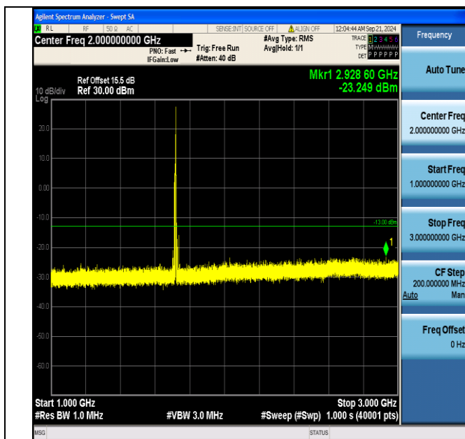
Band4_10MHz_QPSK_20000_1RB#49_1000~3000_1000~3000
