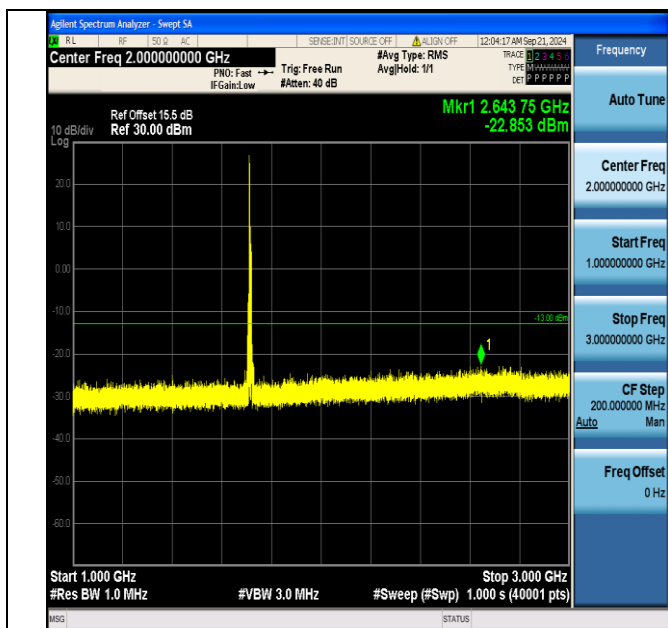
Band4_10MHz_16QAM_20000_1RB#0_1000~3000_1000~3000
