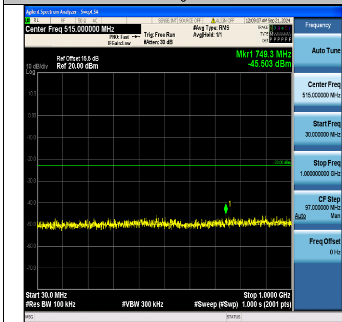
Band4_10MHz_QPSK_20350_1RB#0_30~1000_30~1000
