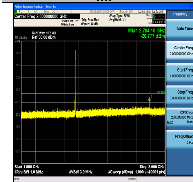
Band4_5MHz_16QAM_20375_25RB#0_1000~3000_1000~3000
