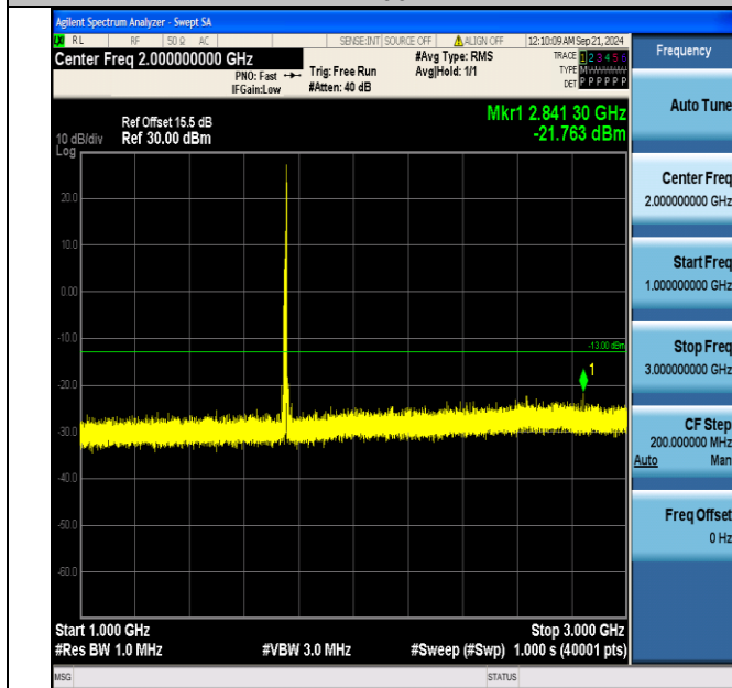
Band4_10MHz_QPSK_20350_1RB#49_1000~3000_1000~3000
