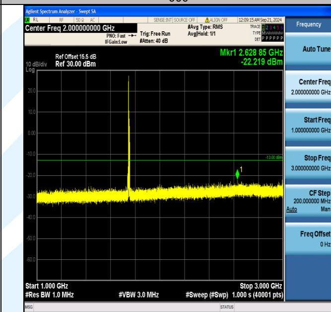
Band4_10MHz_QPSK_20350_1RB#0_1000~3000_1000~3000
