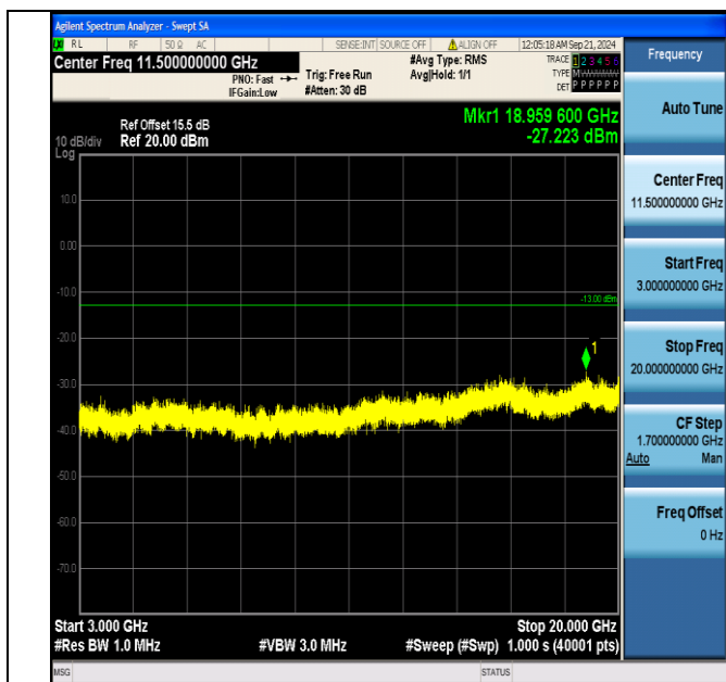
Band4_10MHz_16QAM_20000_1RB#49_3000~20000_3000~20000
