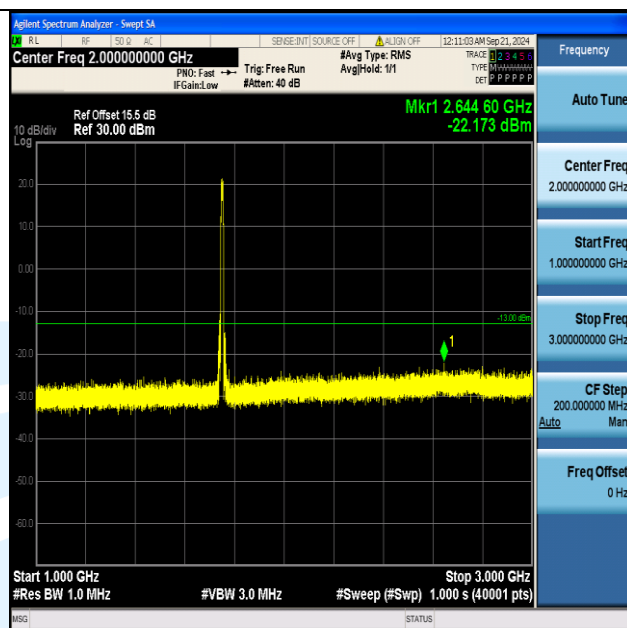
Band4_10MHz_QPSK_20350_50RB#0_1000~3000_1000~3000
