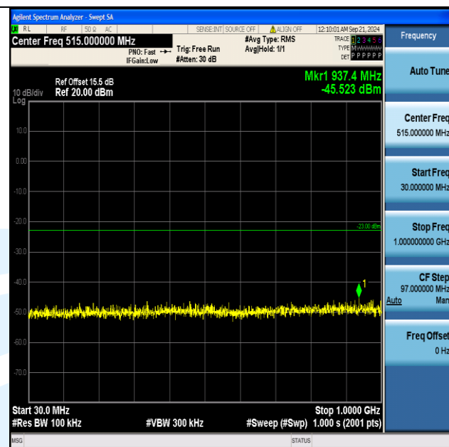
Band4_10MHz_QPSK_20350_1RB#49_30~1000_30~1000
