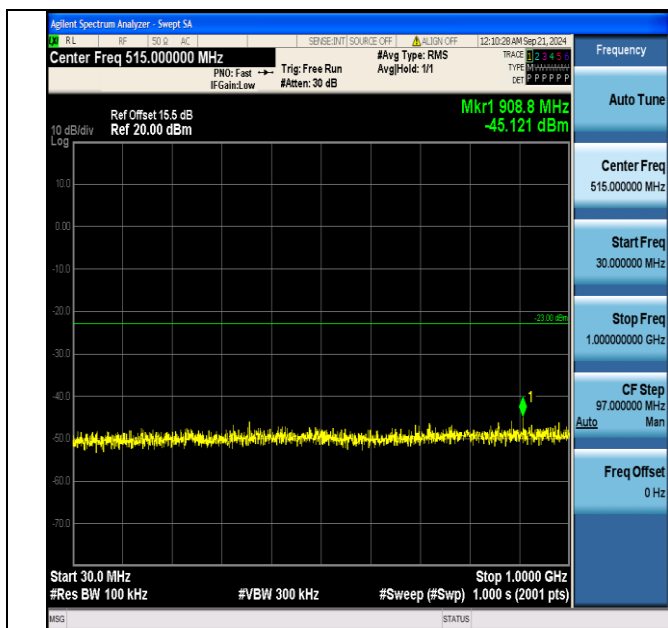
Band4_10MHz_16QAM_20350_1RB#49_30~1000_30~1000
