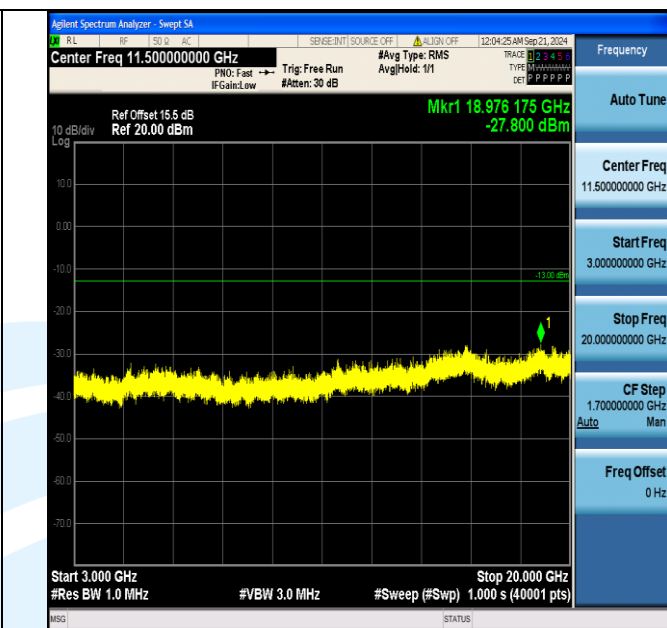
Band4_10MHz_16QAM_20000_1RB#0_3000~20000_3000~20000
