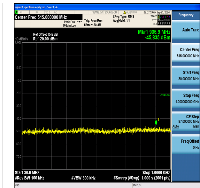
Band4_10MHz_QPSK_20175_1RB#49_30~1000_30~1000
