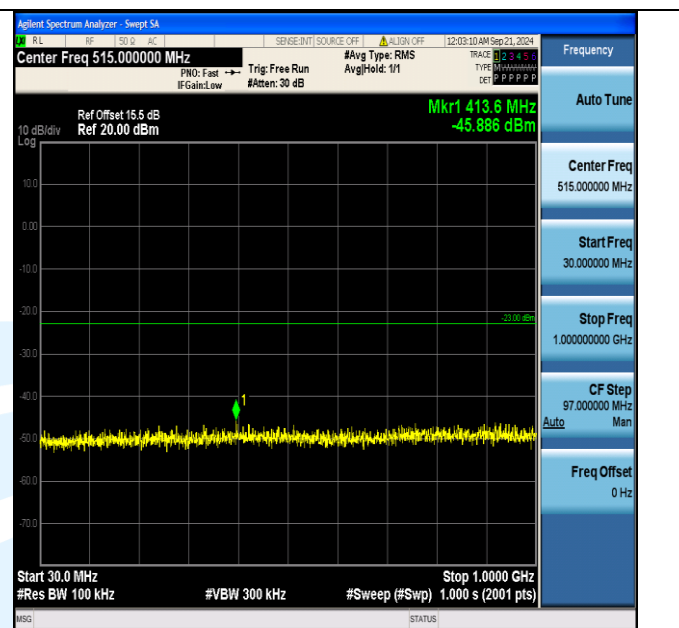
Band4_5MHz_16QAM_20375_25RB#0_30~1000_30~1000
