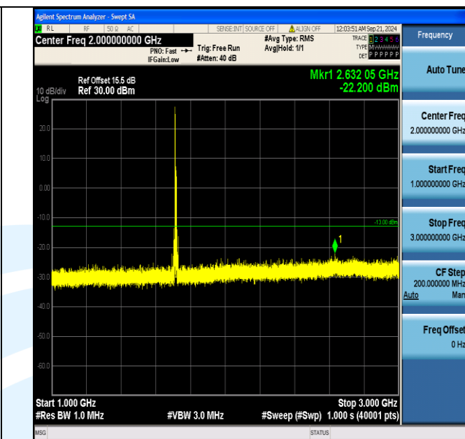
Band4_10MHz_QPSK_20000_1RB#0_1000~3000_1000~3000
