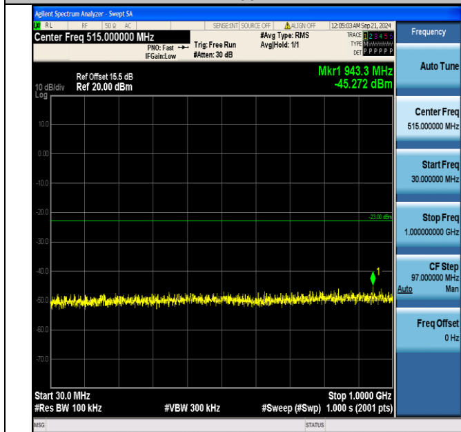
Band4_10MHz_16QAM_20000_1RB#49_30~1000_30~1000
