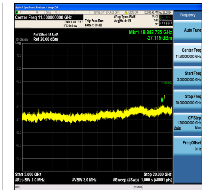
Band4_10MHz_QPSK_20000_50RB#0_3000~20000_3000~20000
