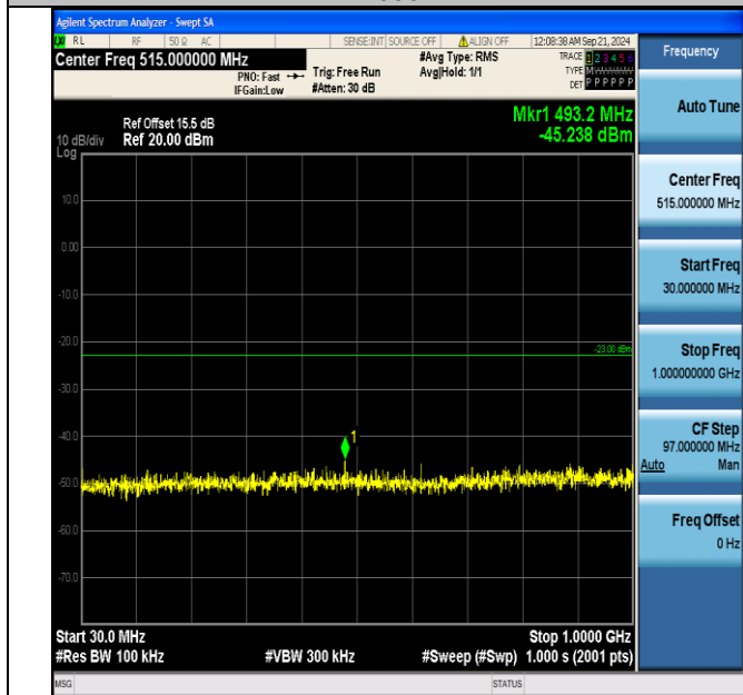
Band4_10MHz_16QAM_20175_50RB#0_30~1000_30~1000
