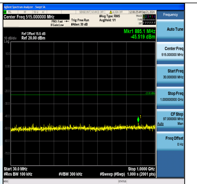
Band4_10MHz_QPSK_20175_1RB#0_30~1000_30~1000
