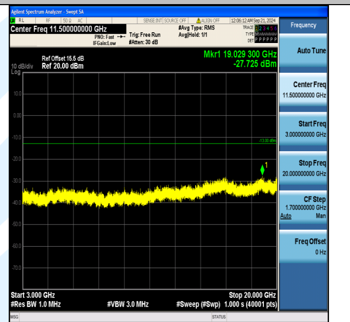
Band4_10MHz_16QAM_20000_50RB#0_3000~20000_3000~20000
