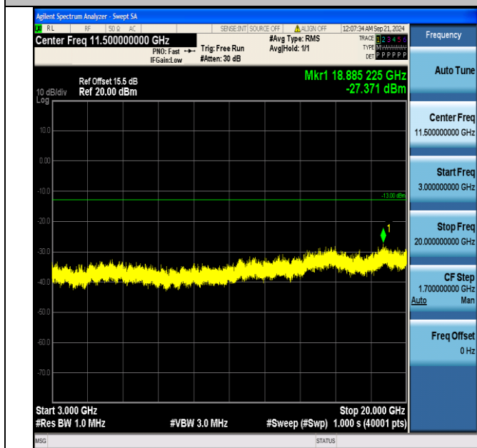
Band4_10MHz_QPSK_20175_1RB#49_3000~20000_3000~20000
