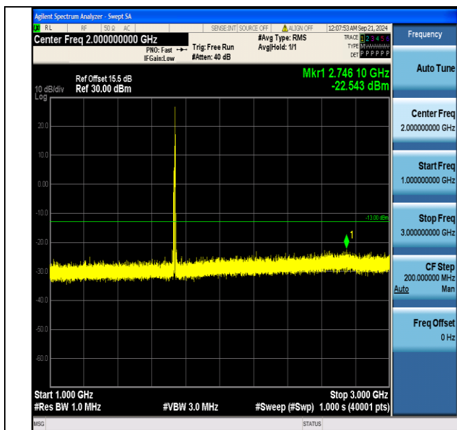
Band4_10MHz_16QAM_20175_1RB#49_1000~3000_1000~3000
