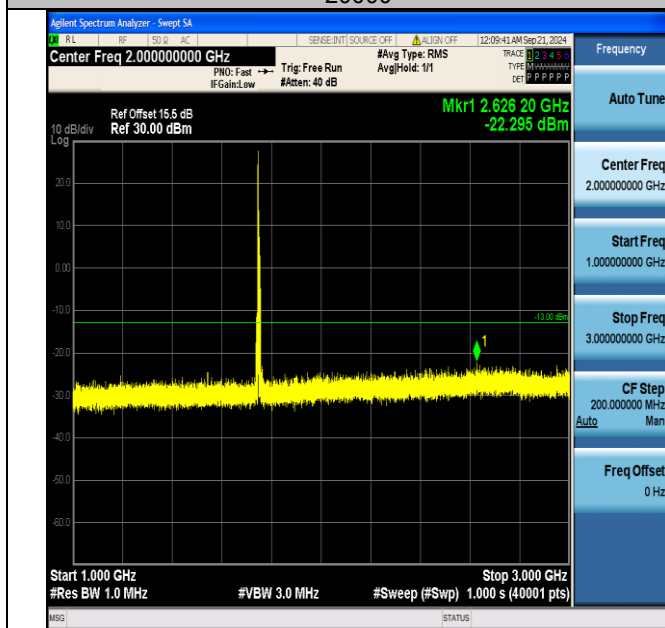
Band4_10MHz_16QAM_20350_1RB#0_1000~3000_1000~3000
