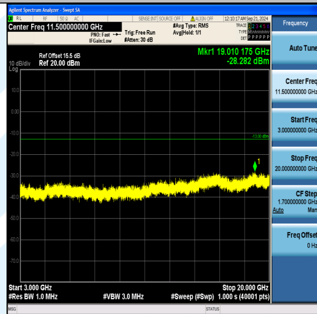
Band4_10MHz_QPSK_20350_1RB#49_3000~20000_3000~20000
