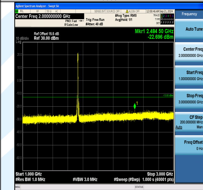
Band4_10MHz_16QAM_20175_50RB#0_1000~3000_1000~3000
