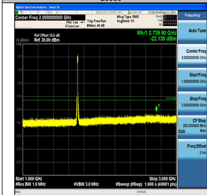
Band4_10MHz_16QAM_20000_50RB#0_1000~3000_1000~3000
