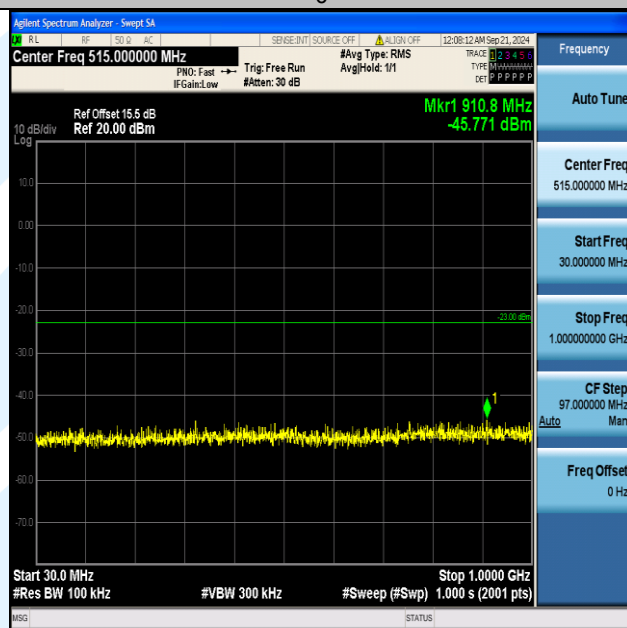
Band4_10MHz_QPSK_20175_50RB#0_30~1000_30~1000
