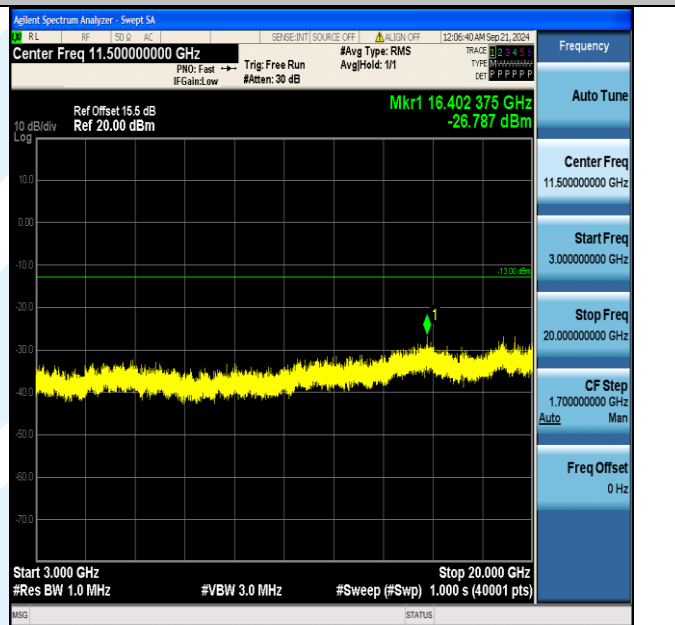
Band4_10MHz_QPSK_20175_1RB#0_3000~20000_3000~20000
