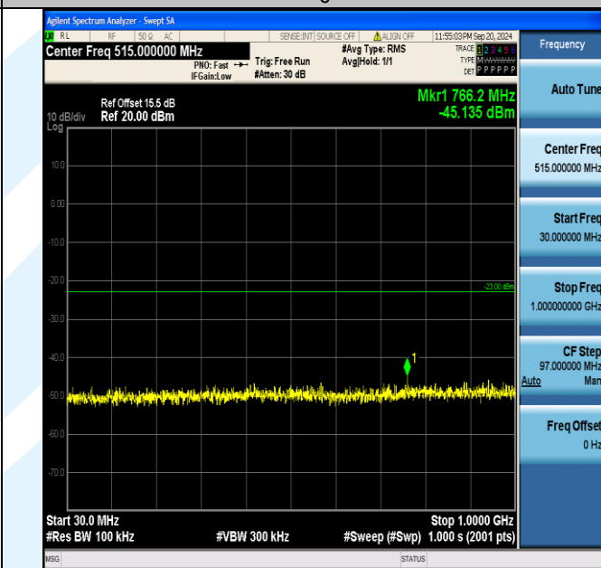
Band4_3MHz_16QAM_20385_15RB#0_30~1000_30~1000
