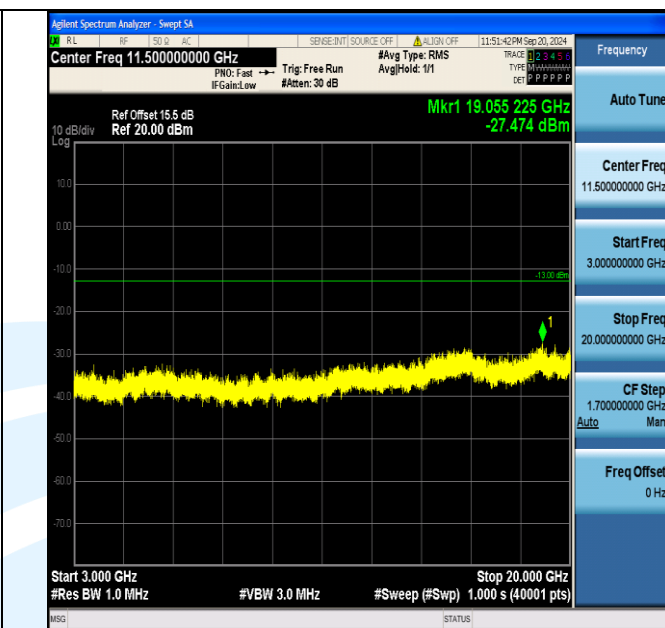
Band4_3MHz_16QAM_20175_1RB#14_3000~20000_3000~20000
