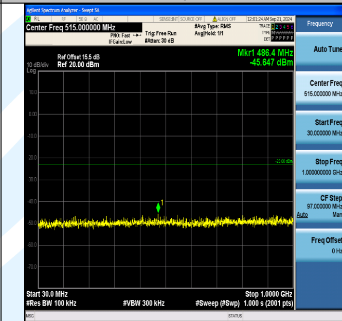
Band4_5MHz_16QAM_20375_1RB#0_30~1000_30~1000
