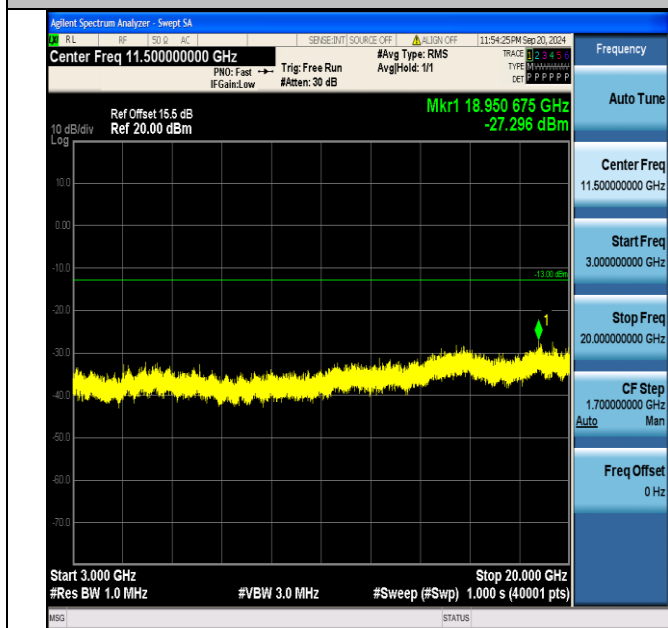
Band4_3MHz_16QAM_20385_1RB#14_3000~20000_3000~20000
