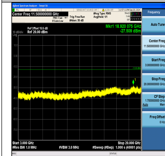
Band4_5MHz_16QAM_19975_1RB#24_3000~20000_3000~20000
