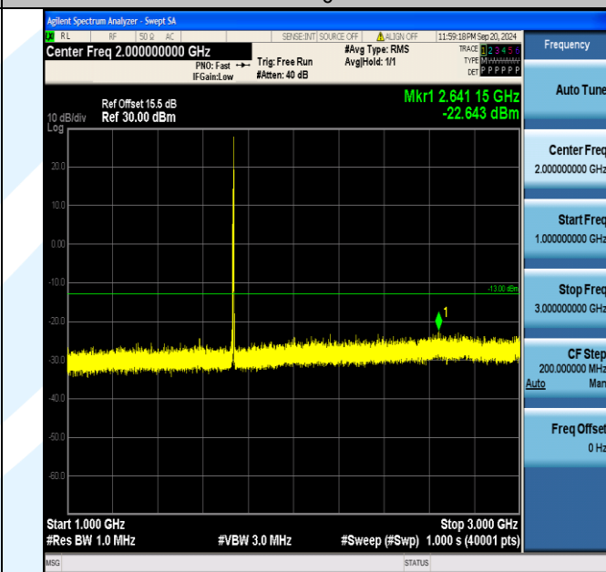
Band4_5MHz_QPSK_20175_1RB#24_1000~3000_1000~3000
