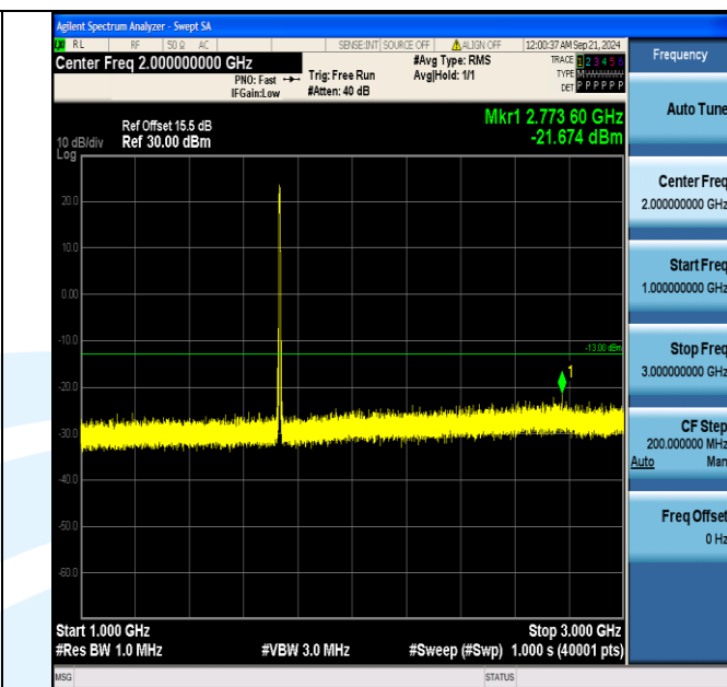
Band4_5MHz_16QAM_20175_25RB#0_1000~3000_1000~3000
