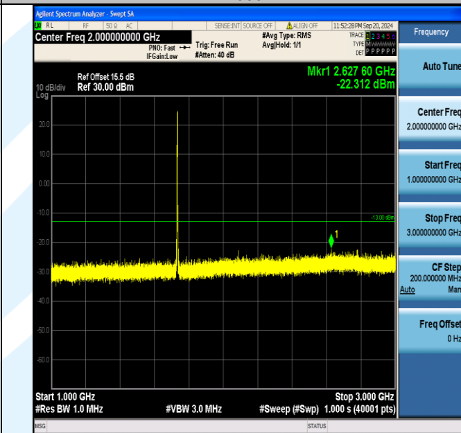
Band4_3MHz_16QAM_20175_15RB#0_1000~3000_1000~3000
