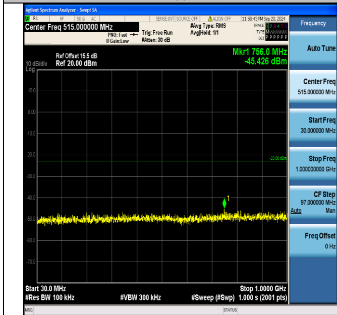
Band4_5MHz_16QAM_20175_1RB#0_30~1000_30~1000
