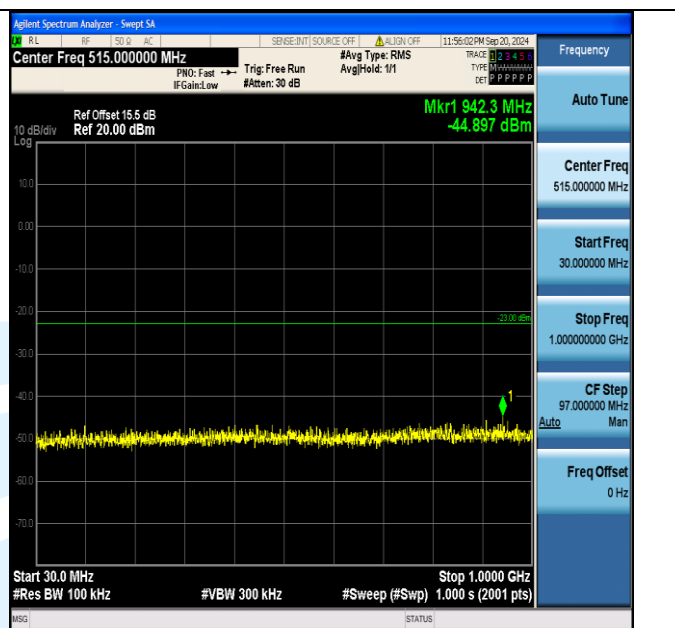
Band4_5MHz_16QAM_19975_1RB#0_30~1000_30~1000
