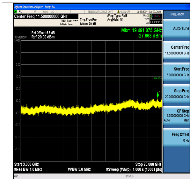
Band4_5MHz_16QAM_20175_1RB#0_3000~20000_3000~20000
