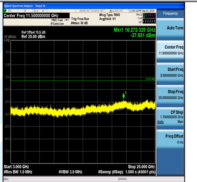
Band4_5MHz_16QAM_19975_1RB#0_3000~20000_3000~20000
