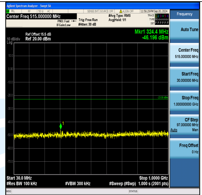
Band4_5MHz_QPSK_19975_1RB#24_30~1000_30~1000
