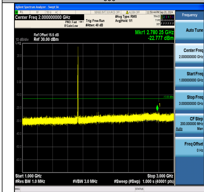
Band4_5MHz_16QAM_20175_1RB#24_1000~3000_1000~3000
