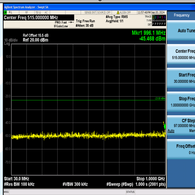
Band4_5MHz_16QAM_19975_25RB#0_30~1000_30~1000
