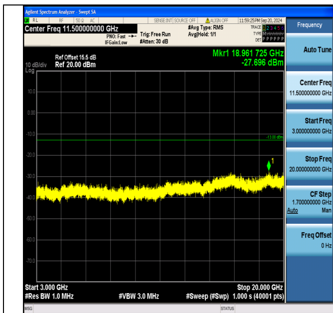
Band4_5MHz_QPSK_20175_1RB#24_3000~20000_3000~20000
