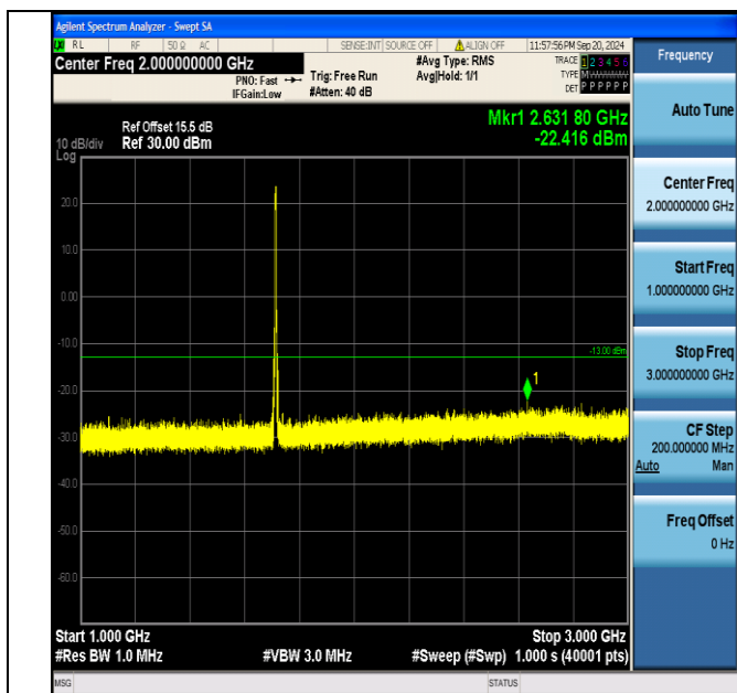
Band4_5MHz_16QAM_19975_25RB#0_1000~3000_1000~3000
