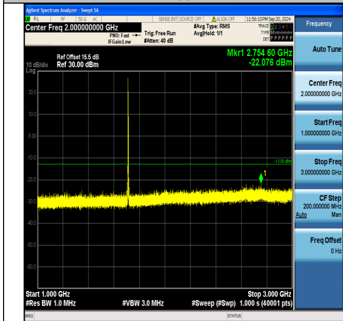
Band4_5MHz_16QAM_19975_1RB#0_1000~3000_1000~3000
