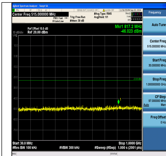
Band4_5MHz_16QAM_19975_1RB#24_30~1000_30~1000
