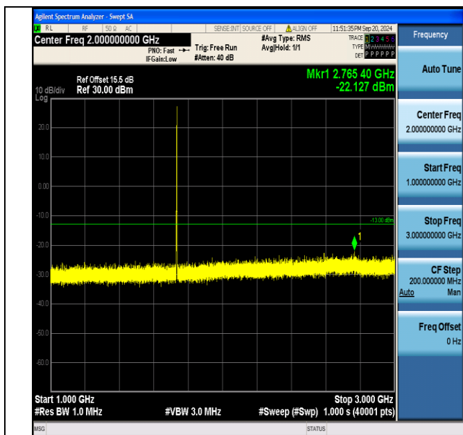
Band4_3MHz_16QAM_20175_1RB#14_1000~3000_1000~3000
