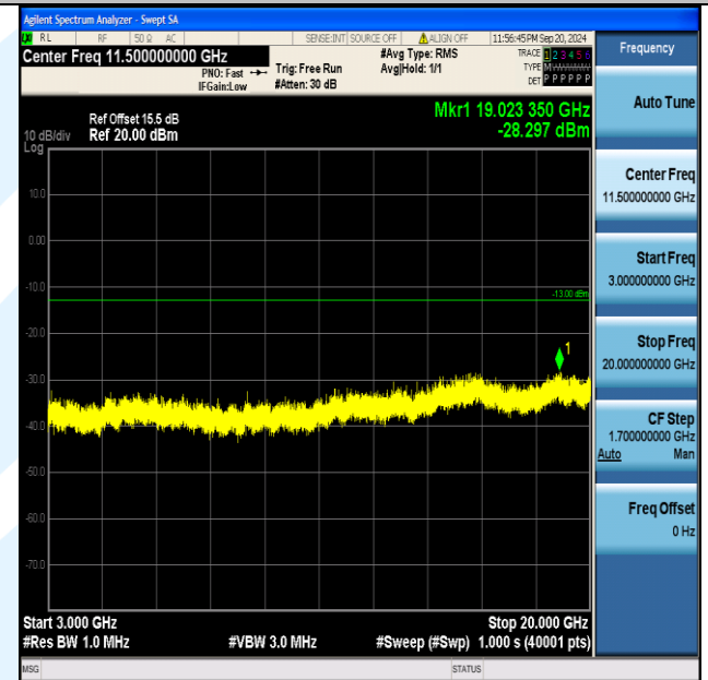
Band4_5MHz_QPSK_19975_1RB#24_3000~20000_3000~20000
