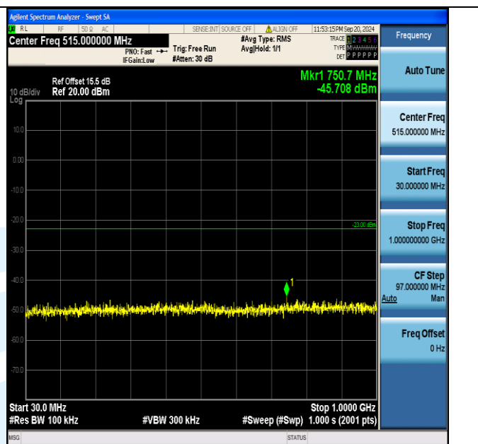
Band4_3MHz_16QAM_20385_1RB#0_30~1000_30~1000
