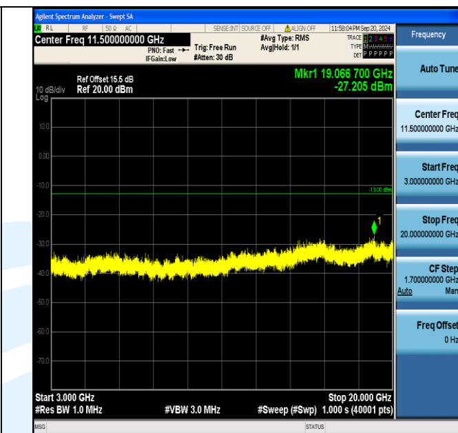
Band4_5MHz_16QAM_19975_25RB#0_3000~20000_3000~20000
