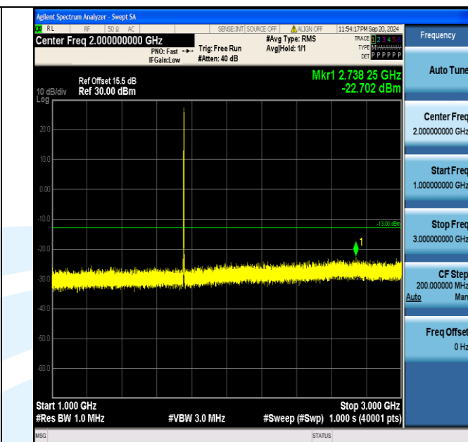
Band4_3MHz_16QAM_20385_1RB#14_1000~3000_1000~3000
