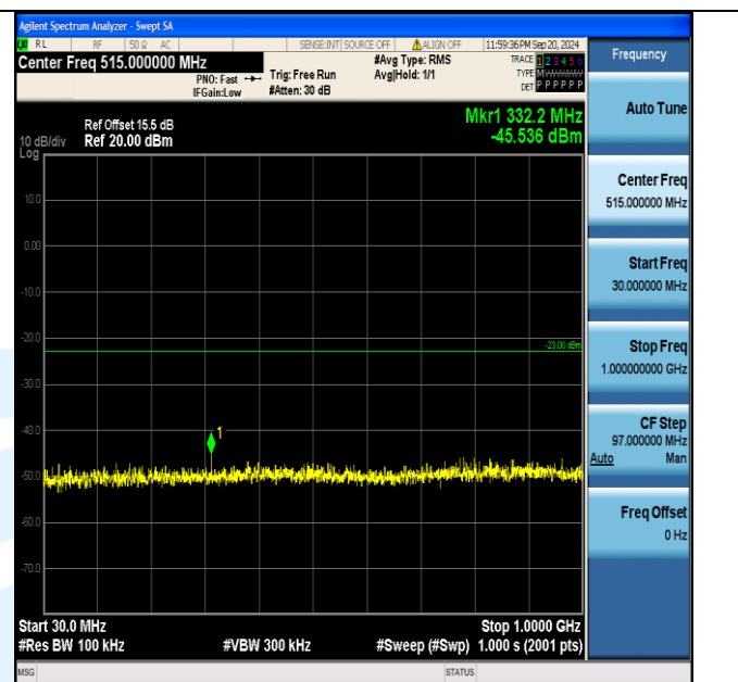
Band4_5MHz_16QAM_20175_1RB#24_30~1000_30~1000
