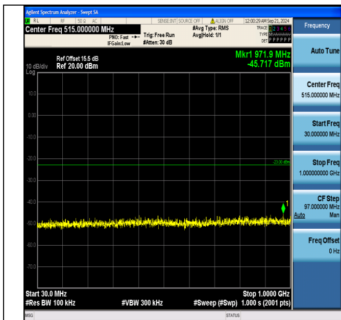
Band4_5MHz_16QAM_20175_25RB#0_30~1000_30~1000
