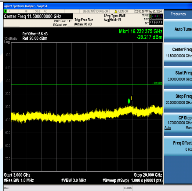
Band4_5MHz_QPSK_20175_25RB#0_3000~20000_3000~20000
