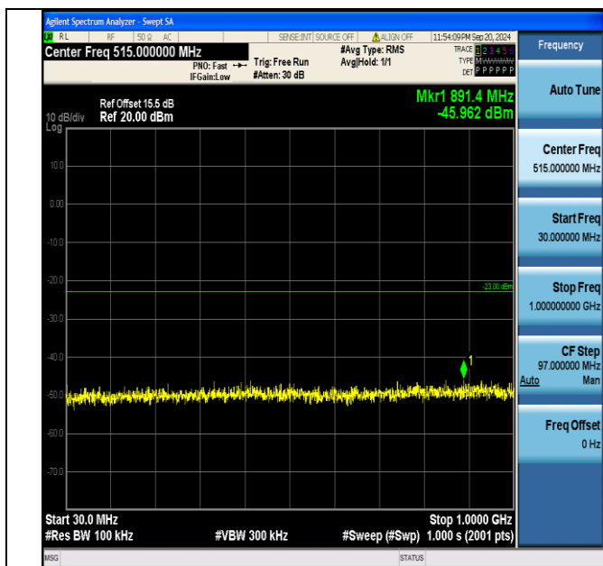
Band4_3MHz_16QAM_20385_1RB#14_30~1000_30~1000
