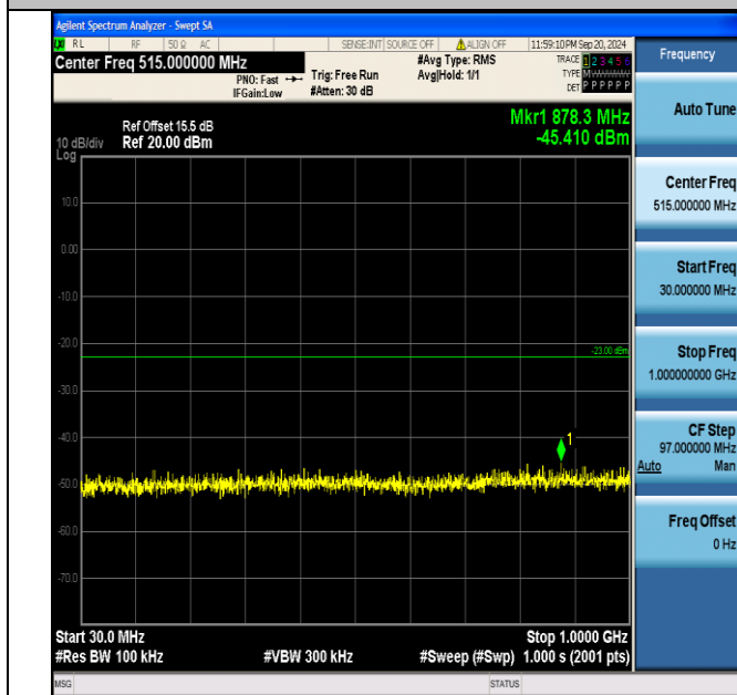
Band4_5MHz_QPSK_20175_1RB#24_30~1000_30~1000
