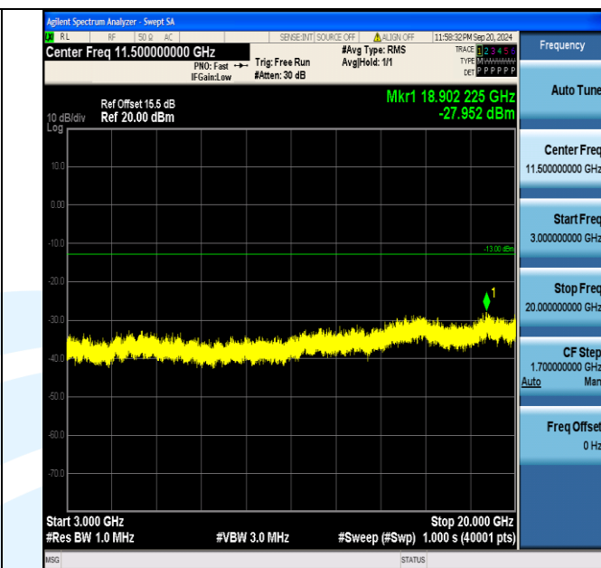
Band4_5MHz_QPSK_20175_1RB#0_3000~20000_3000~20000
