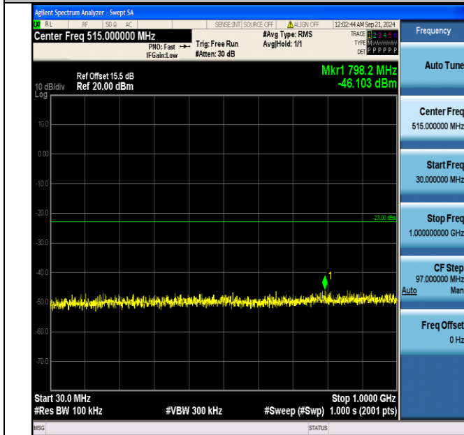
Band4_5MHz_QPSK_20375_25RB#0_30~1000_30~1000
