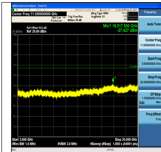
Band4_3MHz_16QAM_20175_15RB#0_3000~20000_3000~20000
