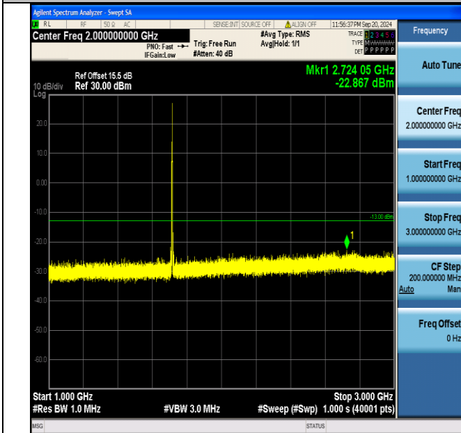
Band4_5MHz_QPSK_19975_1RB#24_1000~3000_1000~3000
