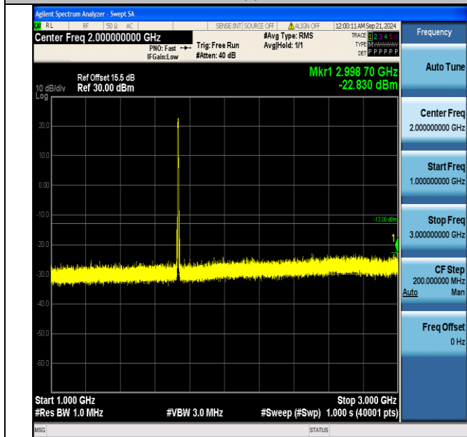
Band4_5MHz_QPSK_20175_25RB#0_1000~3000_1000~3000
