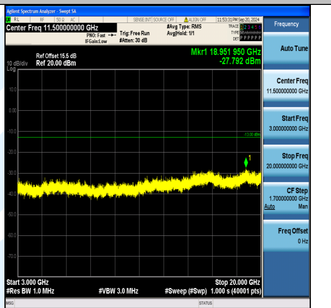
Band4_3MHz_16QAM_20385_1RB#0_3000~20000_3000~20000
