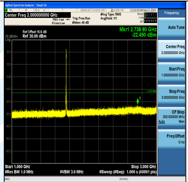
Band4_5MHz_QPSK_20375_25RB#0_1000~3000_1000~3000
