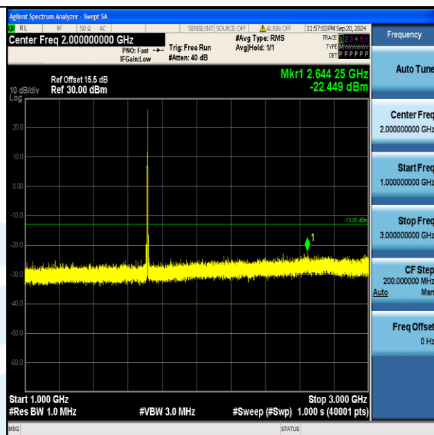
Band4_5MHz_16QAM_19975_1RB#24_1000~3000_1000~3000
