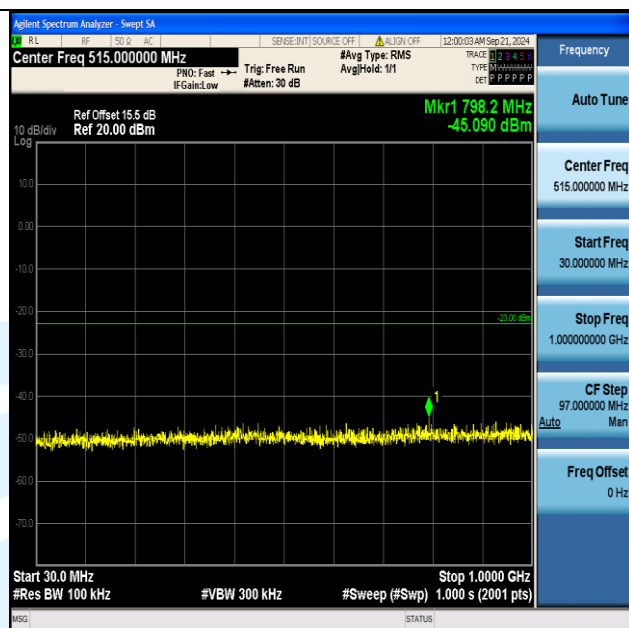
Band4_5MHz_QPSK_20175_25RB#0_30~1000_30~1000
