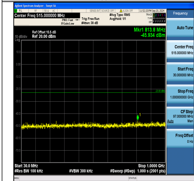
Band4_3MHz_16QAM_20175_15RB#0_30~1000_30~1000
