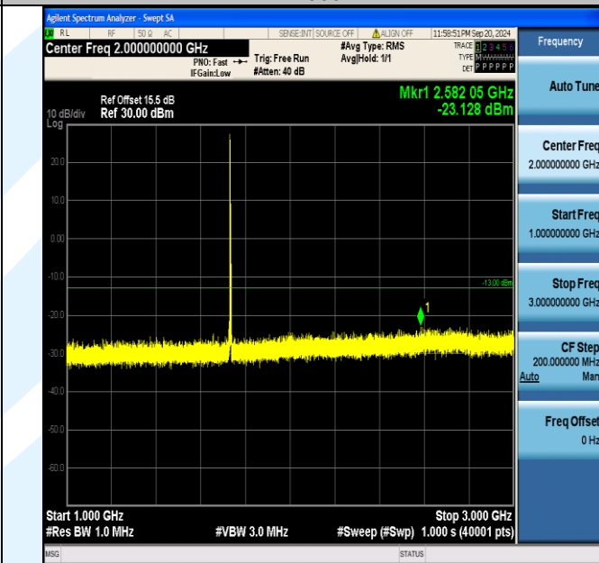
Band4_5MHz_16QAM_20175_1RB#0_1000~3000_1000~3000
