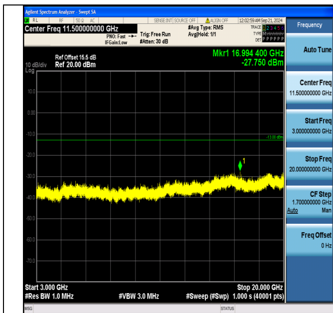
Band4_5MHz_QPSK_20375_25RB#0_3000~20000_3000~20000
