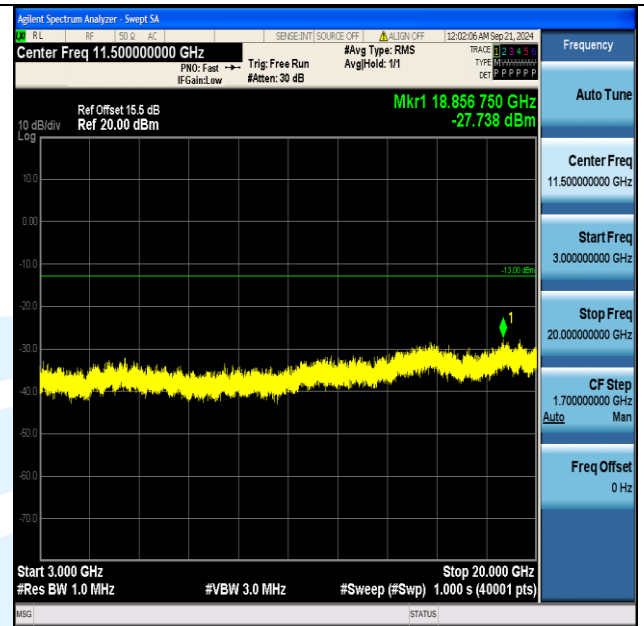
Band4_5MHz_QPSK_20375_1RB#24_3000~20000_3000~20000
