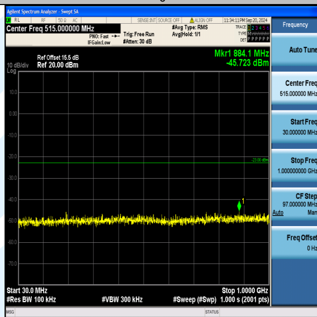
Band2_20MHz_16QAM_18900_1RB#99_30~1000_30~1000
