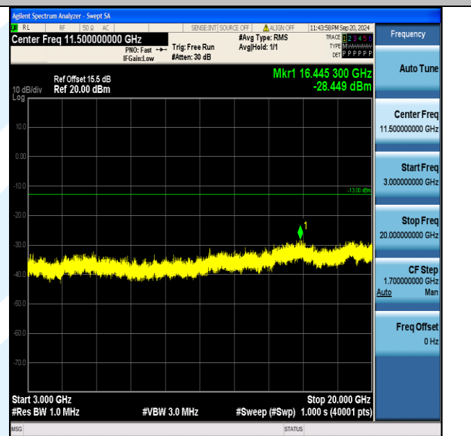
Band4_1.4MHz_QPSK_20175_6RB#0_3000~20000_3000~20000
