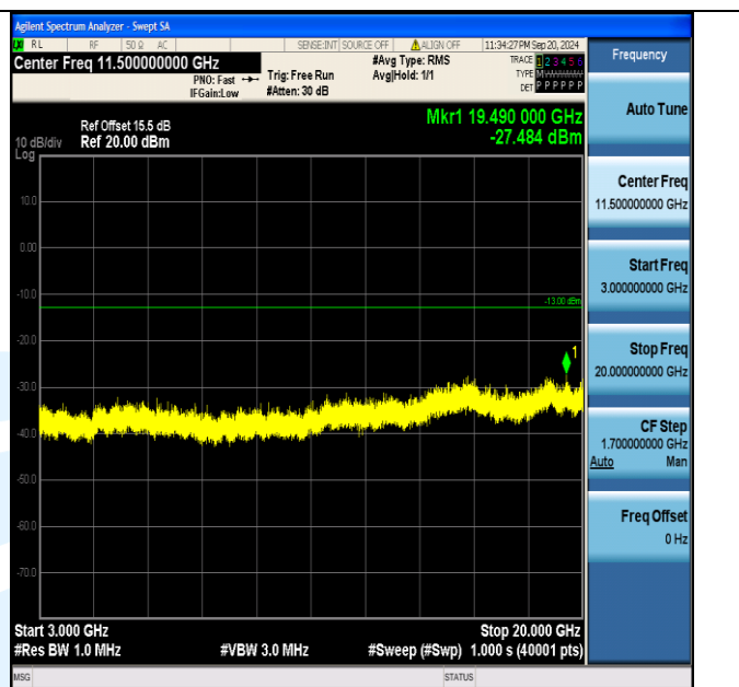
Band2_20MHz_16QAM_18900_1RB#99_3000~20000_3000~20000
