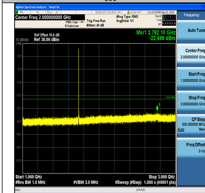
Band4_1.4MHz_QPSK_20175_6RB#0_1000~3000_1000~3000
