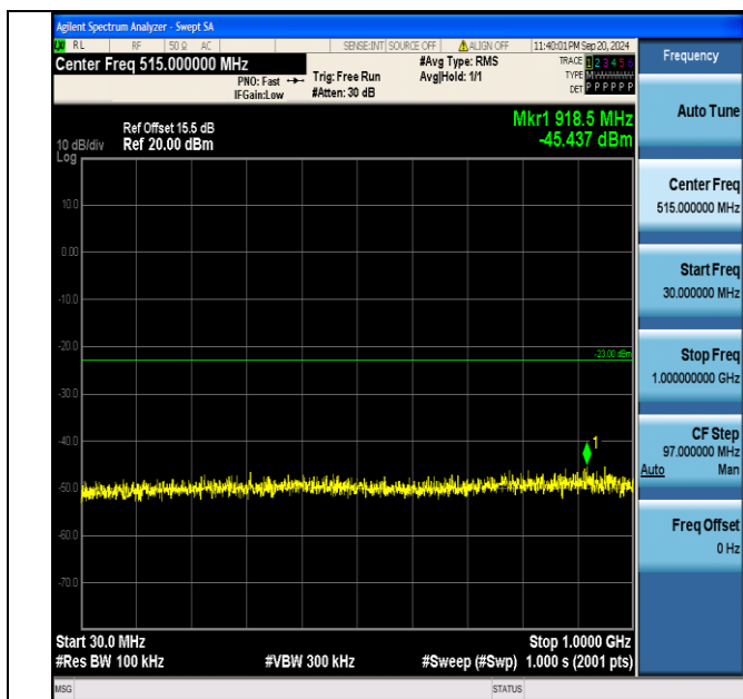
Band4_1.4MHz_16QAM_19957_1RB#5_30~1000_30~1000
