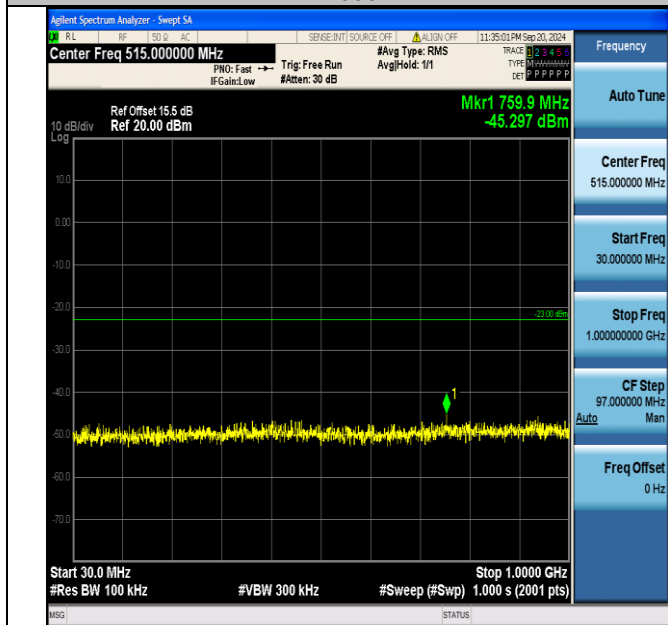
Band2_20MHz_16QAM_18900_100RB#0_30~1000_30~1000
