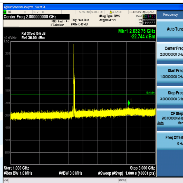
Band2_20MHz_16QAM_18900_1RB#0_1000~3000_1000~3000
