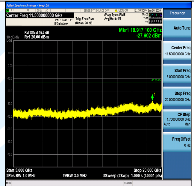
Band4_1.4MHz_QPSK_19957_1RB#5_3000~20000_3000~20000
