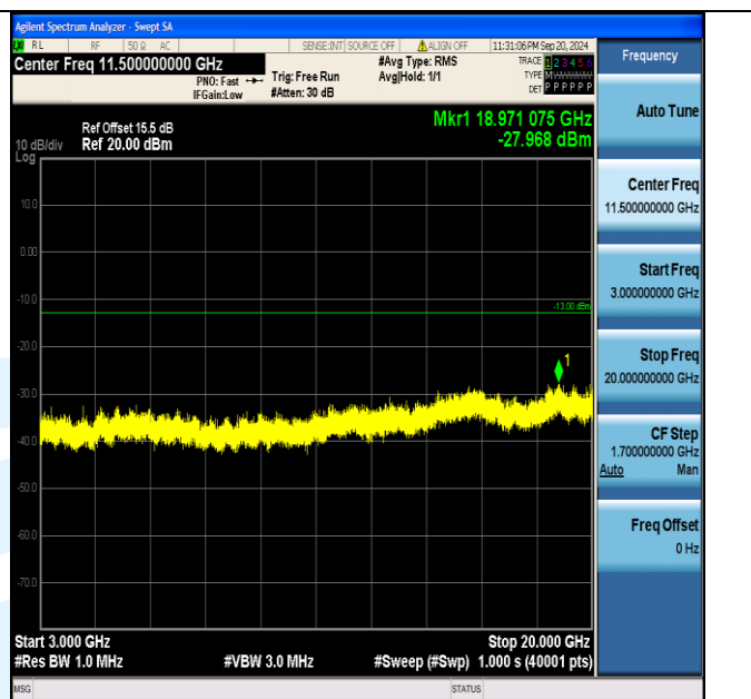
Band2_20MHz_16QAM_18700_1RB#0_3000~20000_3000~20000
