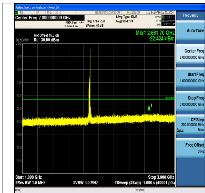
Band2_20MHz_16QAM_18900_1RB#99_1000~3000_1000~3000
