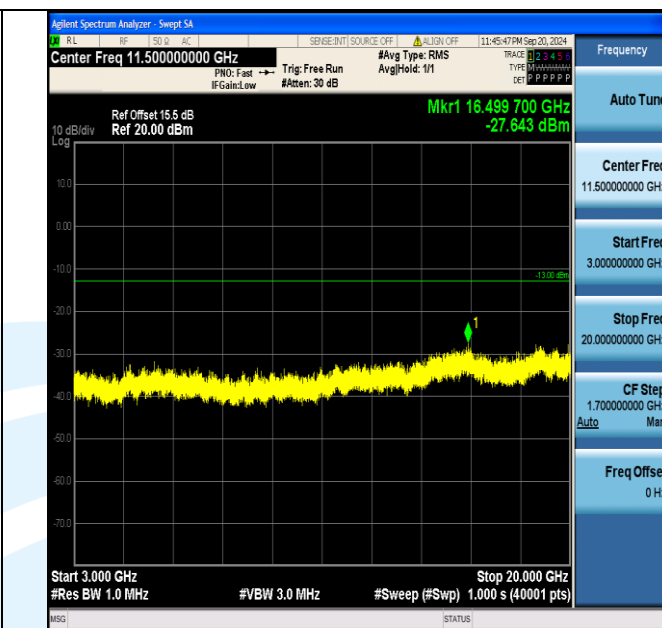
Band4_1.4MHz_QPSK_20393_1RB#5_3000~20000_3000~20000
