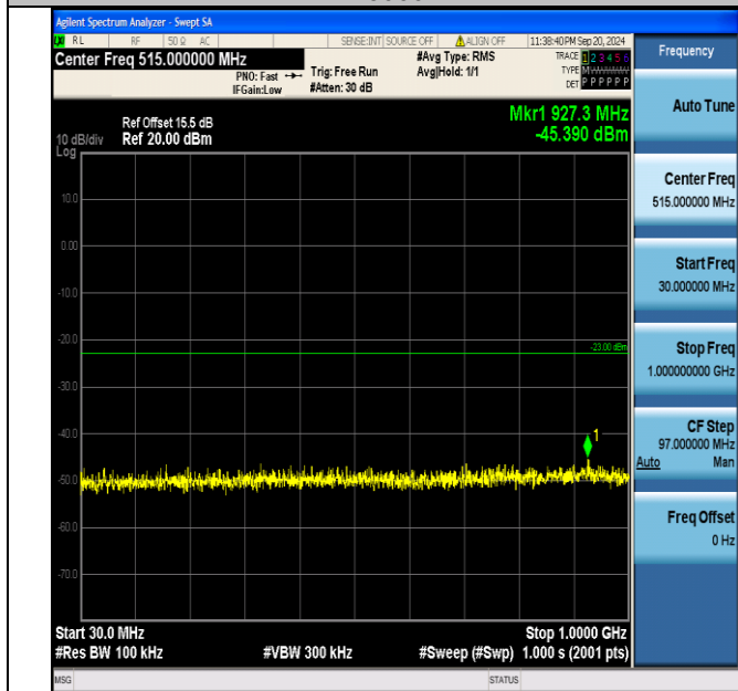
Band4_1.4MHz_QPSK_19957_1RB#0_30~1000_30~1000
