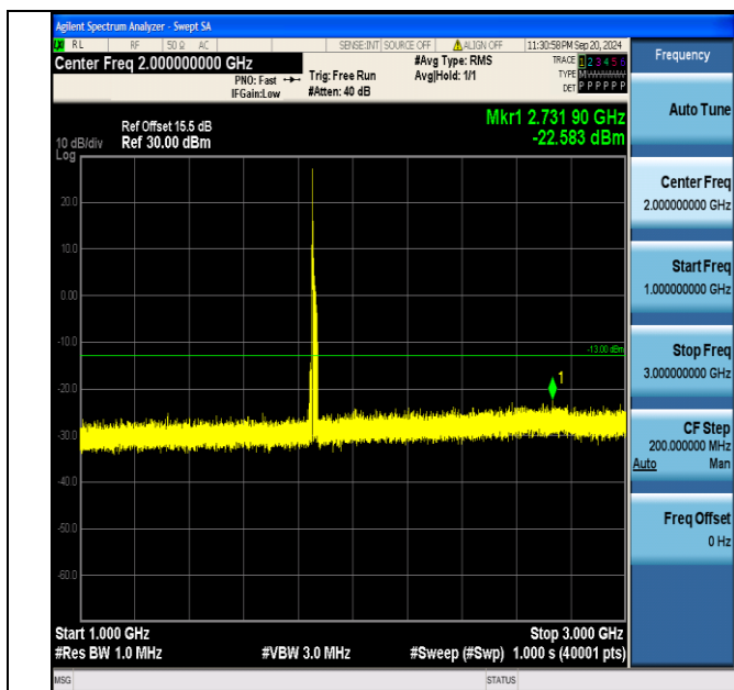
Band2_20MHz_16QAM_18700_1RB#0_1000~3000_1000~3000
