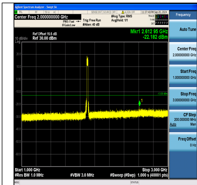
Band2_20MHz_16QAM_19100_100RB#0_1000~3000_1000~3000
