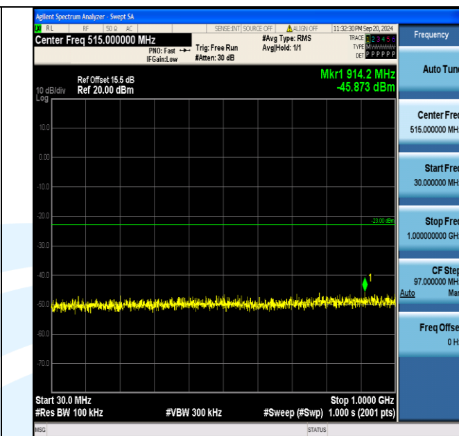
Band2_20MHz_16QAM_18700_100RB#0_30~1000_30~1000
