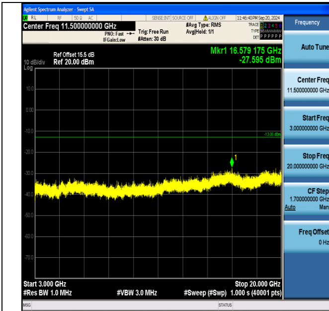
Band4_1.4MHz_QPSK_20393_6RB#0_3000~20000_3000~2000
