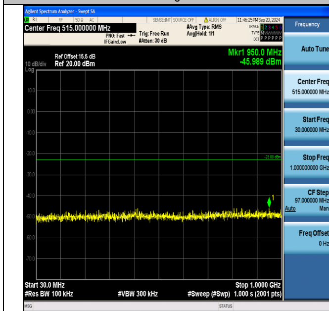
Band4_1.4MHz_QPSK_20393_6RB#0_30~1000_30~1000
