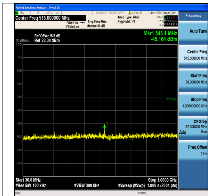
Band4_1.4MHz_QPSK_20393_1RB#0_30~1000_30~1000
