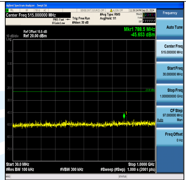
Band4_1.4MHz_QPSK_19957_1RB#5_30~1000_30~1000
