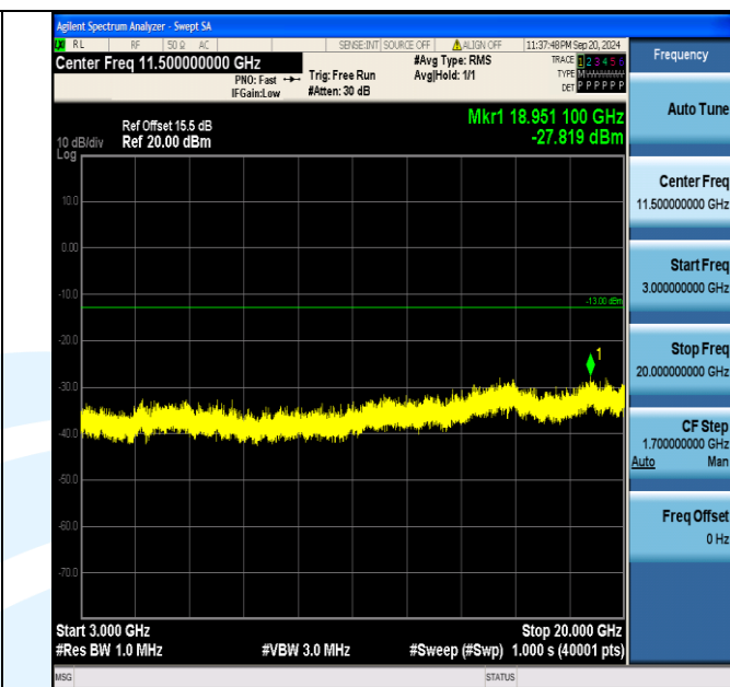
Band2_20MHz_16QAM_19100_100RB#0_3000~20000_3000~20000
