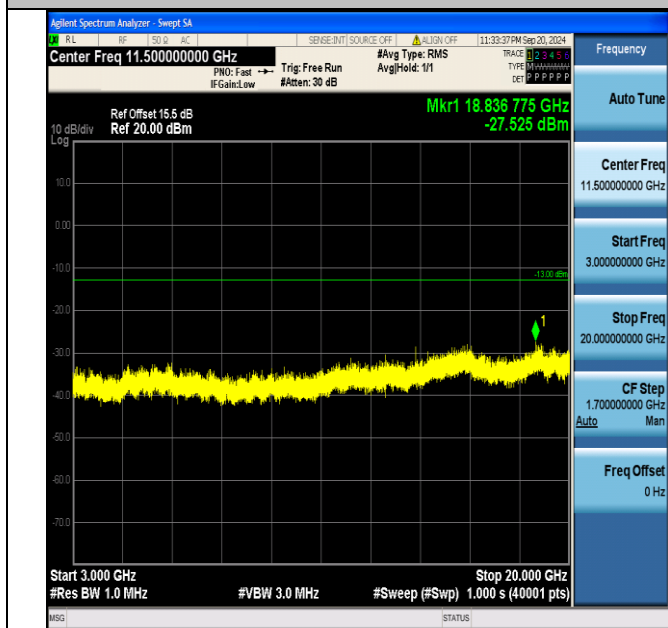
Band2_20MHz_16QAM_18900_1RB#0_3000~20000_3000~20000
