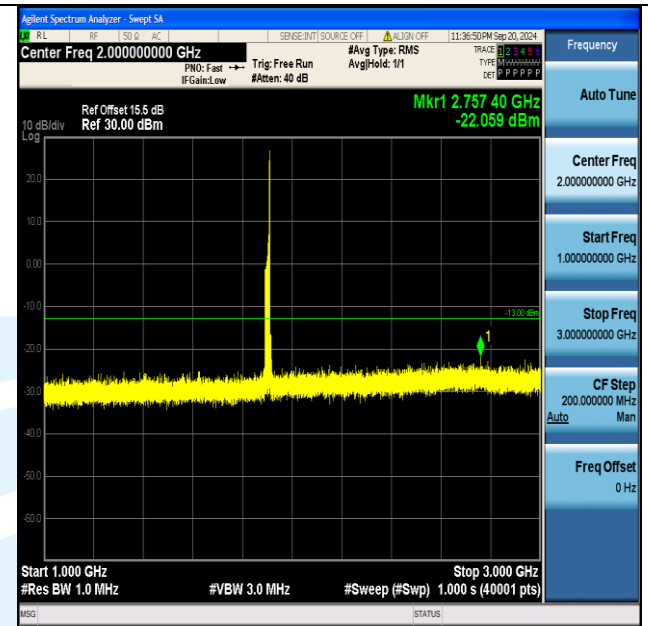
Band2_20MHz_16QAM_19100_1RB#99_1000~3000_1000~3000
