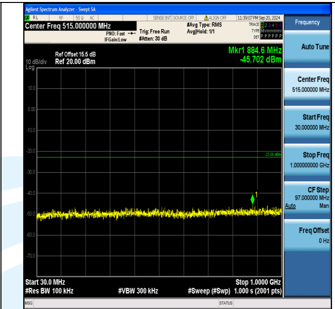
Band4_1.4MHz_16QAM_19957_1RB#0_30~1000_30~1000
