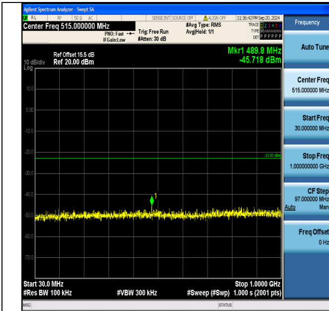
Band2_20MHz_16QAM_19100_1RB#99_30~1000_30~1000
