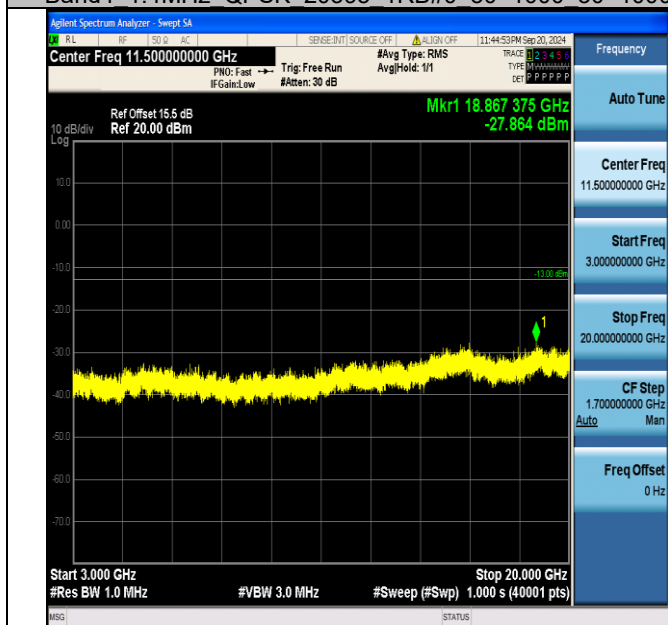
Band4_1.4MHz_QPSK_20393_1RB#0_3000~20000_3000~20000
