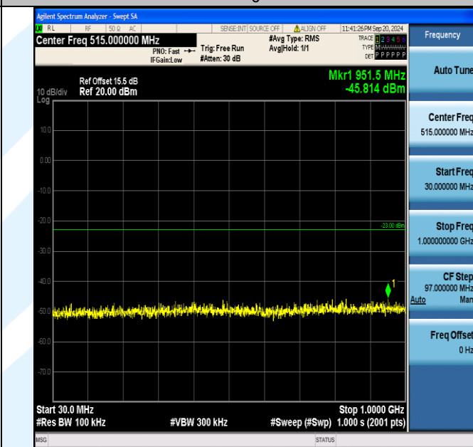
Band4_1.4MHz_16QAM_19957_6RB#0_30~1000_30~1000
