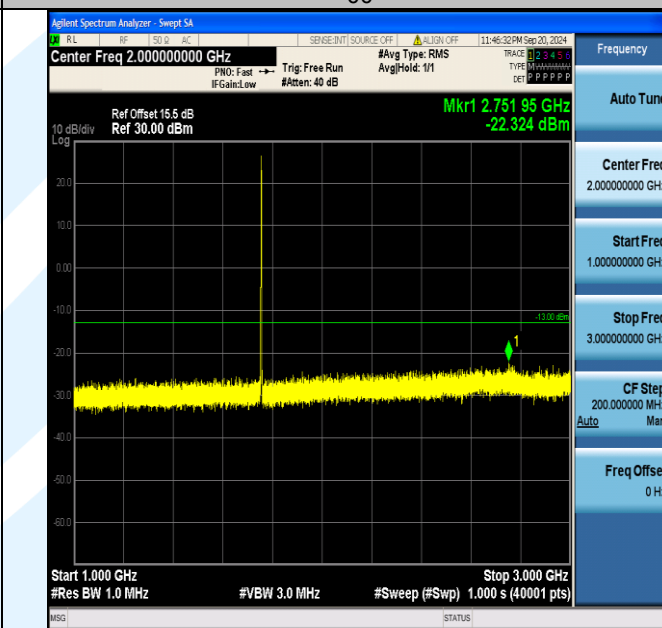
Band4_1.4MHz_QPSK_20393_6RB#0_1000~3000_1000~3000
