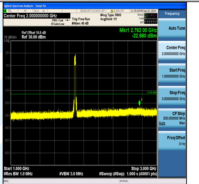
Band2_20MHz_16QAM_18900_100RB#0_1000~3000_1000~3000
