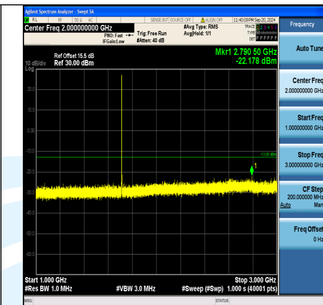
Band4_1.4MHz_16QAM_19957_1RB#5_1000~3000_1000~3000 0
