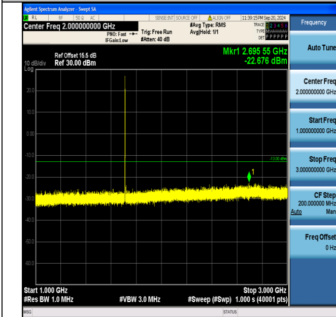
Band4_1.4MHz_16QAM_19957_1RB#0_1000~3000_1000~3000
