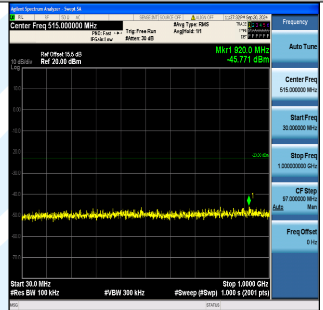
Band2_20MHz_16QAM_19100_100RB#0_30~1000_30~1000
