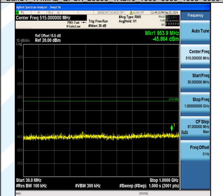
Band4_1.4MHz_QPSK_20393_1RB#5_30~1000_30~1000
