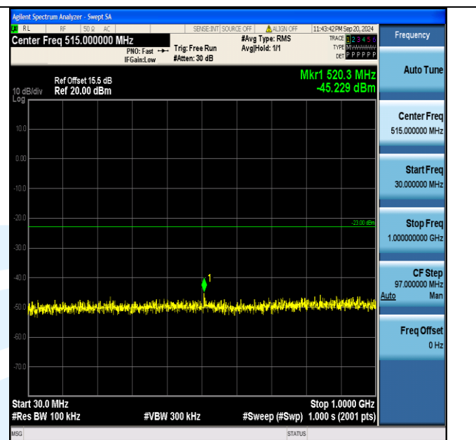
Band4_1.4MHz_QPSK_20175_6RB#0_30~1000_30~1000
