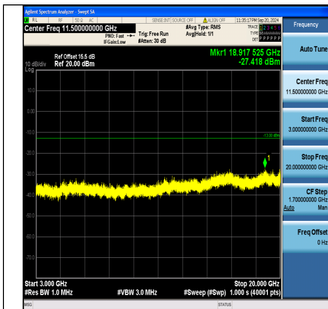
Band2_20MHz_16QAM_18900_100RB#0_3000~20000_3000~20000
