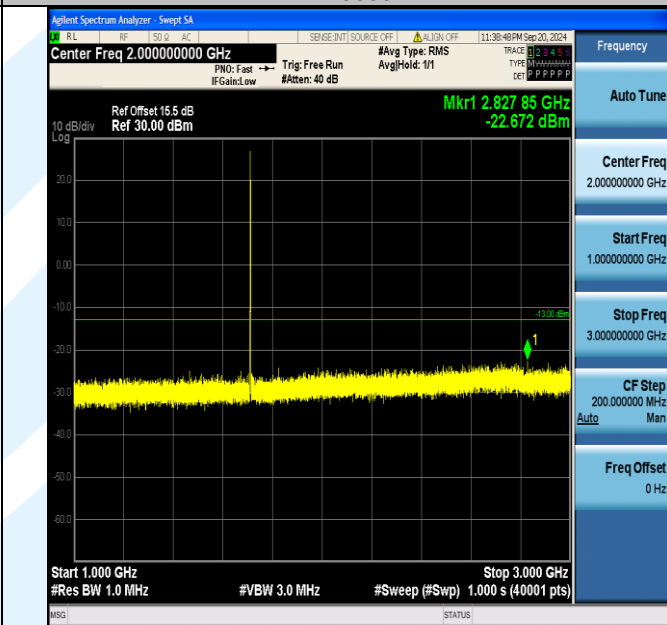
Band4_1.4MHz_QPSK_19957_1RB#0_1000~3000_1000~3000
