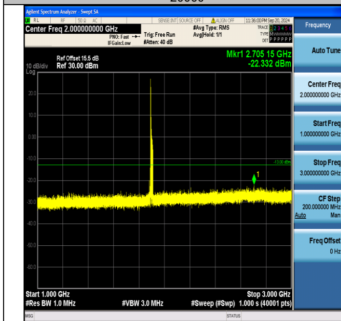
Band2_20MHz_16QAM_19100_1RB#0_1000~3000_1000~3000
