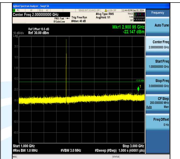
Band4_1.4MHz_QPSK_20393_1RB#0_1000~3000_1000~3000
