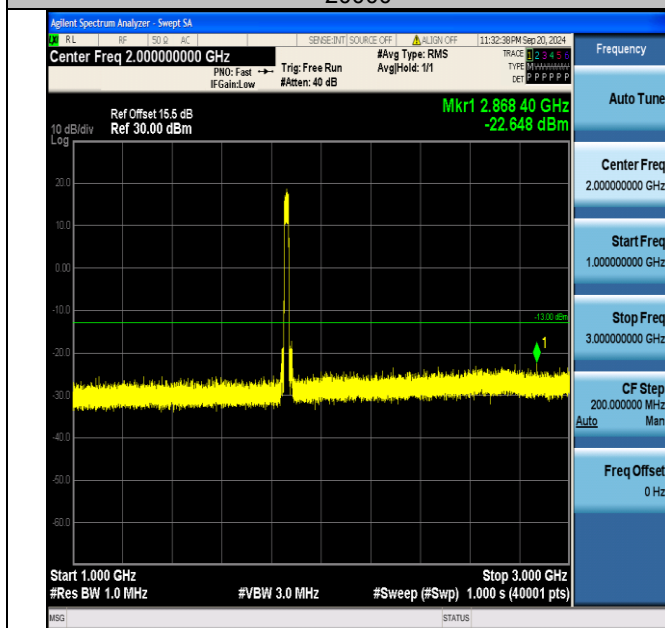
Band2_20MHz_16QAM_18700_100RB#0_1000~3000_1000~3000
