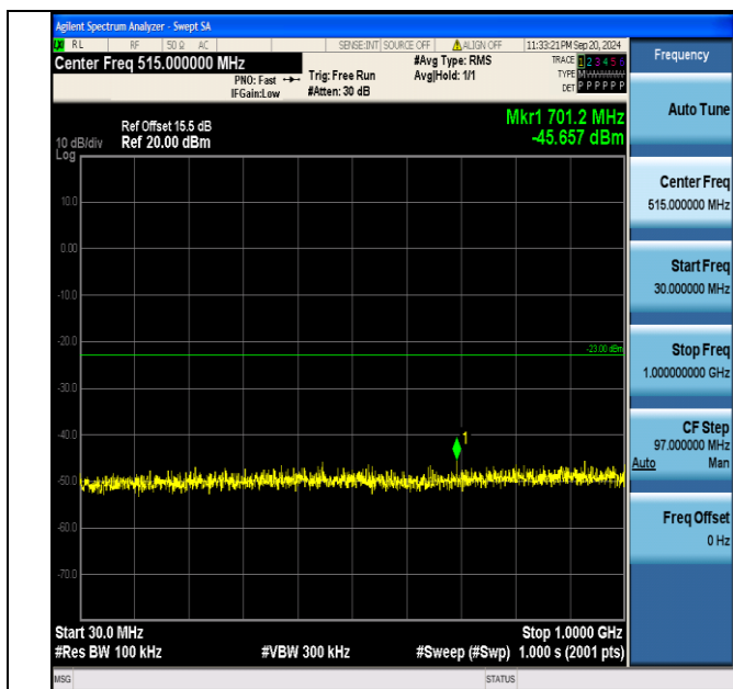
Band2_20MHz_16QAM_18900_1RB#0_30~1000_30~1000
