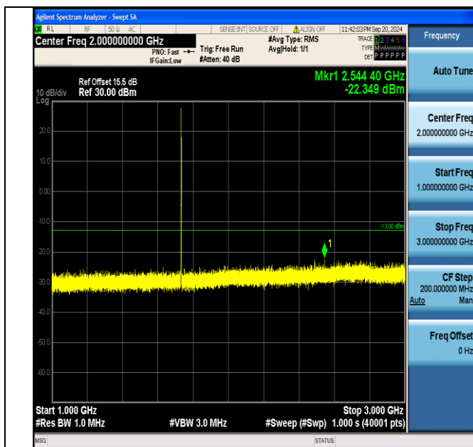
Band4_1.4MHz_QPSK_20175_1RB#0_1000~3000_1000~3000
