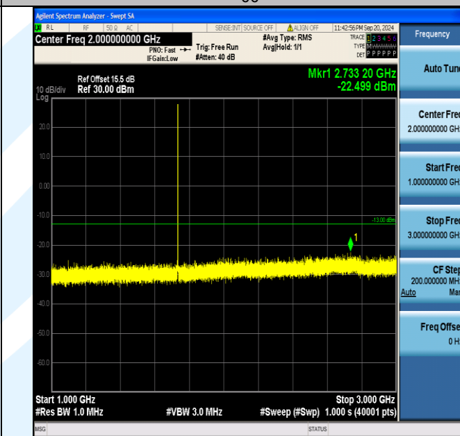
Band4_1.4MHz_QPSK_20175_1RB#5_1000~3000_1000~3000
