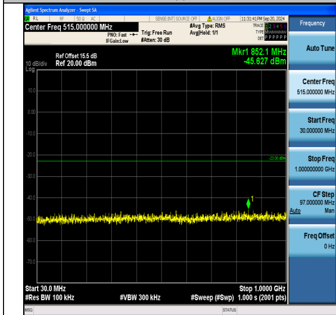
Band2_20MHz_16QAM_18700_1RB#99_30~1000_30~1000
