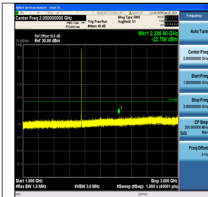
Band4_1.4MHz_QPSK_20393_1RB#5_1000~3000_1000~3000
