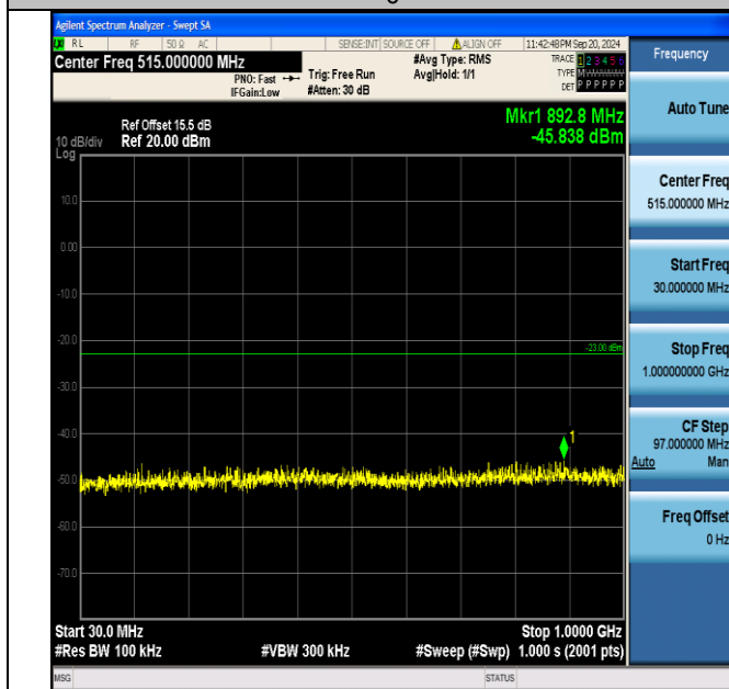
Band4_1.4MHz_QPSK_20175_1RB#5_30~1000_30~1000
