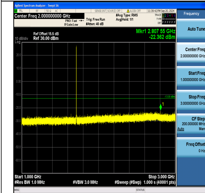
Band4_1.4MHz_QPSK_19957_1RB#5_1000~3000_1000~3000
