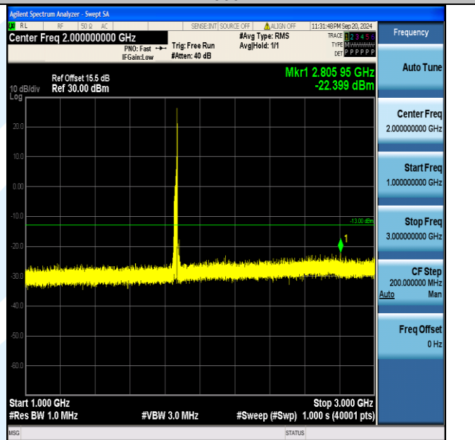
Band2_20MHz_16QAM_18700_1RB#99_1000~3000_1000~3000
