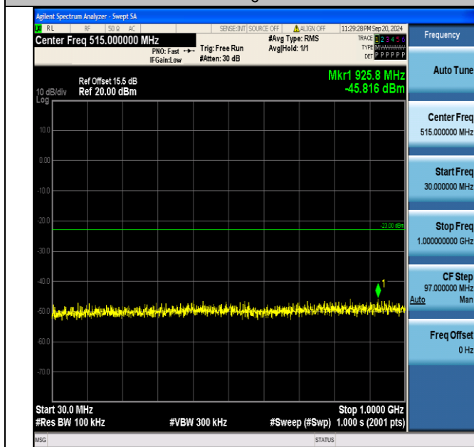
Band2_15MHz_QPSK_19125_75RB#0_30~1000_30~1000
