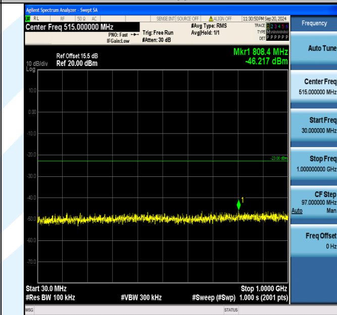
Band2_20MHz_16QAM_18700_1RB#0_30~1000_30~1000
