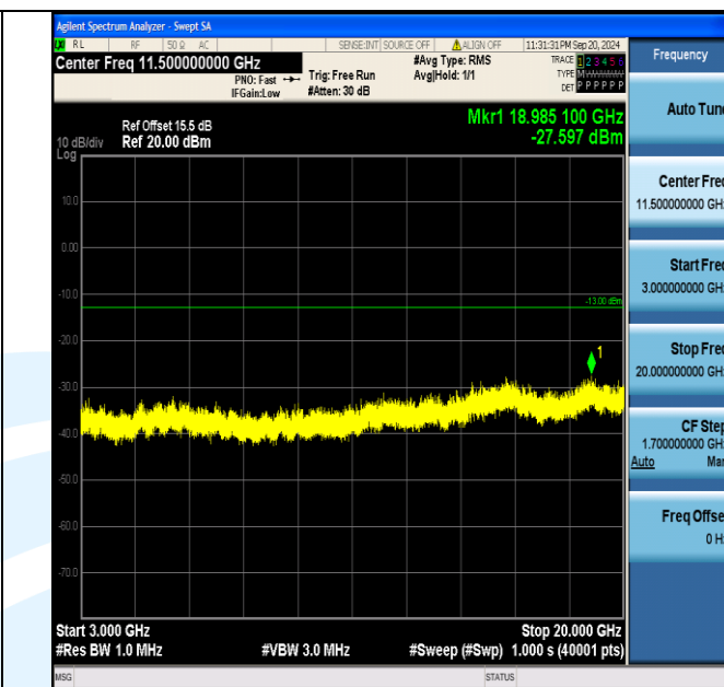
Band2_20MHz_QPSK_18700_1RB#99_3000~20000_3000~20000
