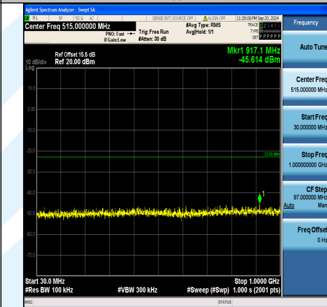
Band2_15MHz_16QAM_19125_1RB#0_30~1000_30~1000
