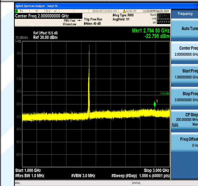
Band2_15MHz_16QAM_19125_1RB#74_1000~3000_1000~3000
