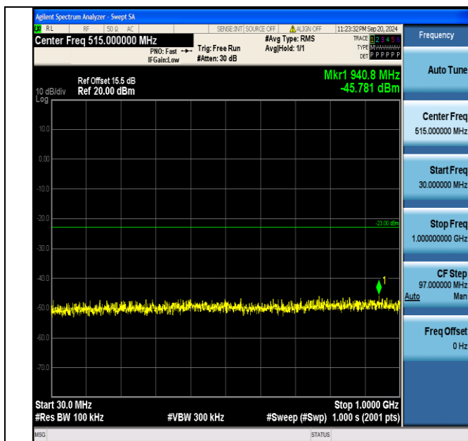
Band2_15MHz_16QAM_18675_1RB#74_30~1000_30~1000
