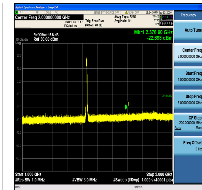
Band2_15MHz_16QAM_18675_75RB#0_1000~3000_1000~3000
