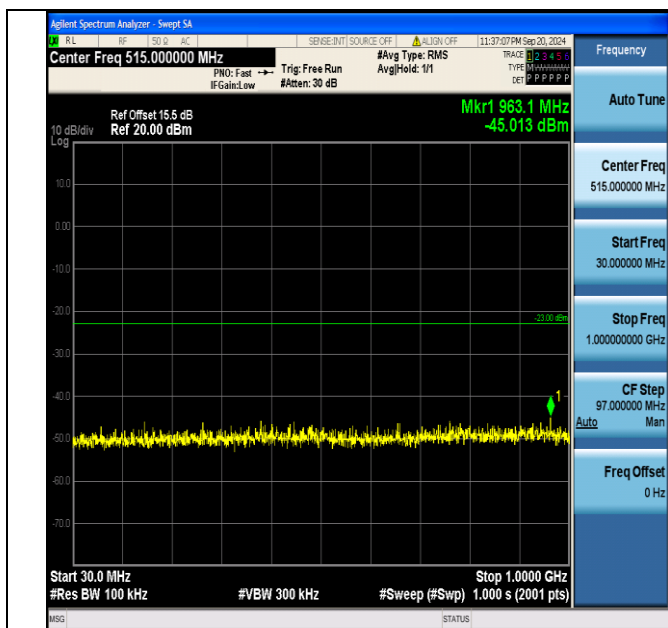
Band2_20MHz_QPSK_19100_100RB#0_30~1000_30~1000
