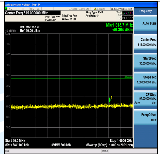
Band2_20MHz_QPSK_19100_1RB#99_30~1000_30~1000
