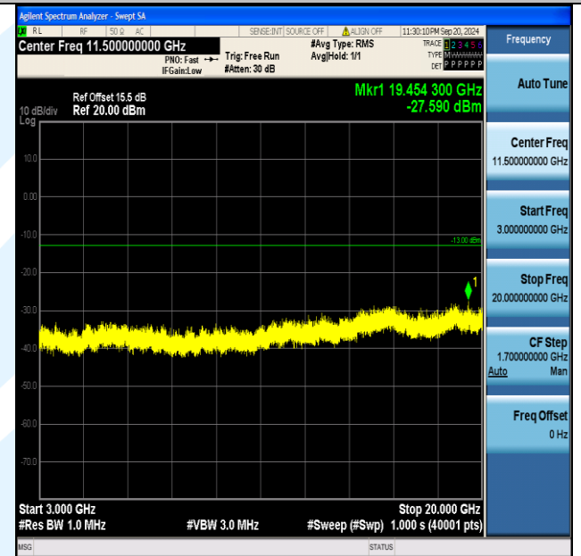
Band2_15MHz_16QAM_19125_75RB#0_3000~20000_3000~20000
