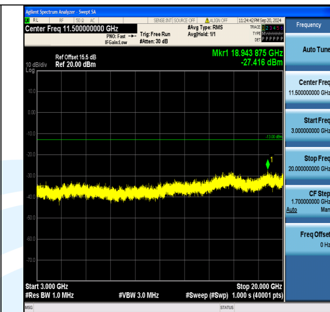
Band2_15MHz_16QAM_18675_75RB#0_3000~20000_3000~20000
