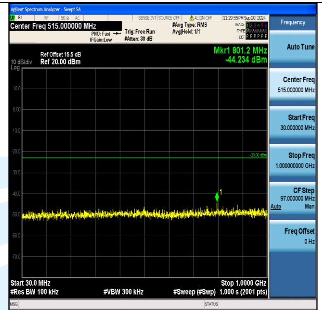
Band2_15MHz_16QAM_19125_75RB#0_30~1000_30~1000
