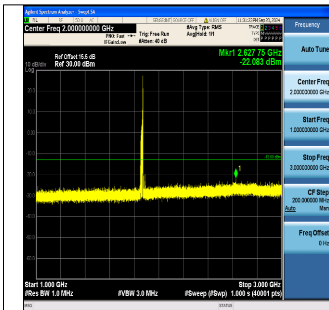
Band2_20MHz_QPSK_18700_1RB#99_1000~3000_1000~3000
