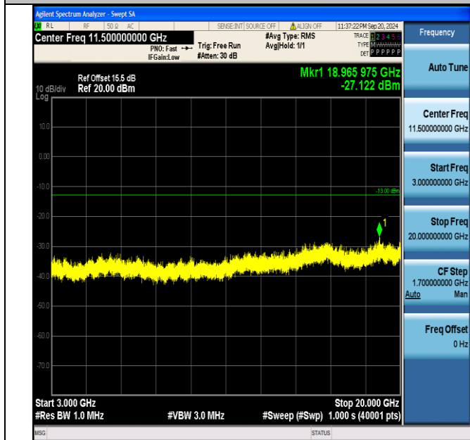
Band2_20MHz_QPSK_19100_100RB#0_3000~20000_3000~20000
