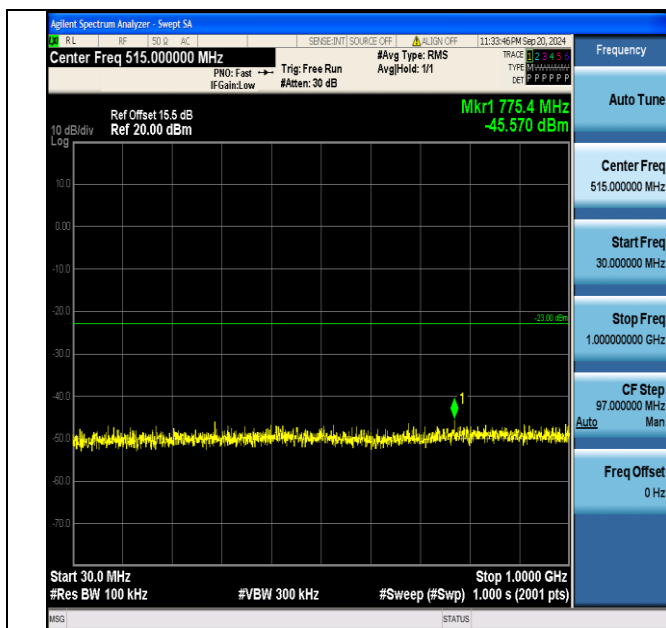
Band2_20MHz_QPSK_18900_1RB#99_30~1000_30~1000
