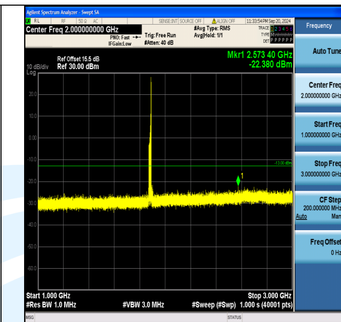
Band2_20MHz_QPSK_18900_1RB#99_1000~3000_1000~3000
