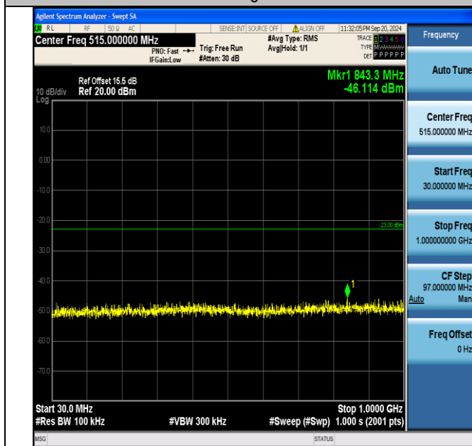
Band2_20MHz_QPSK_18700_100RB#0_30~1000_30~1000
