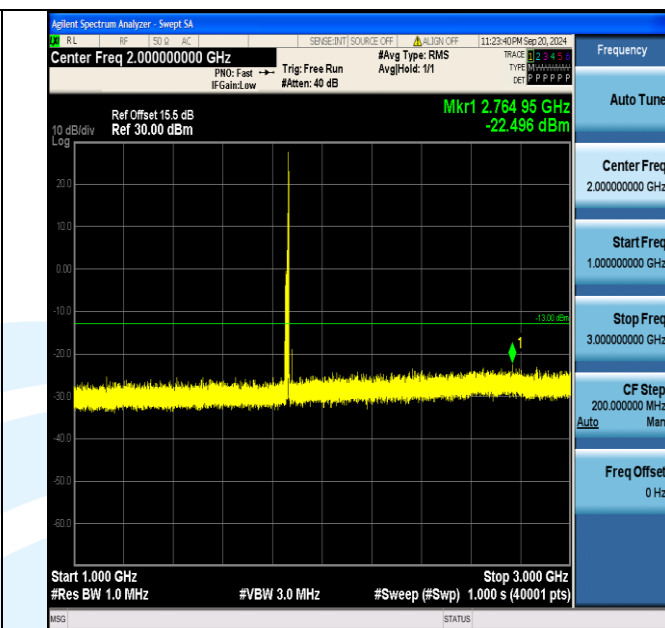
Band2_15MHz_16QAM_18675_1RB#74_1000~3000_1000~3000
