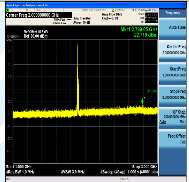
Band2_20MHz_QPSK_19100_1RB#0_1000~3000_1000~3000
