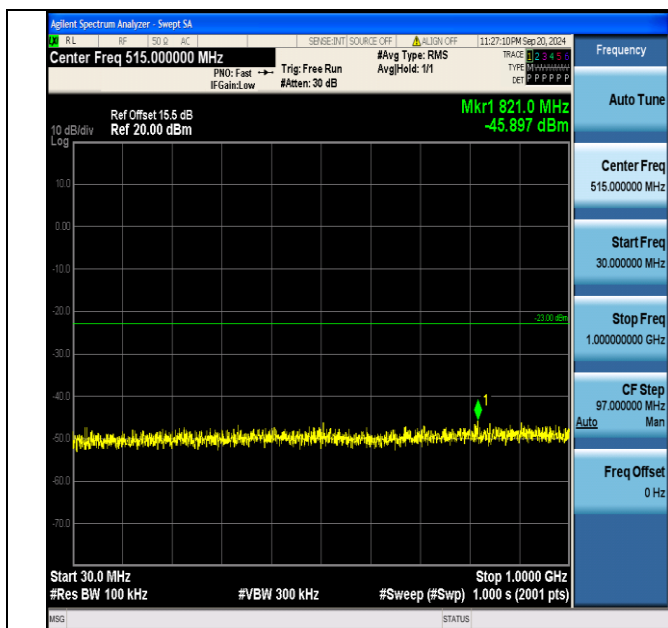
Band2_15MHz_16QAM_18900_75RB#0_30~1000_30~1000
