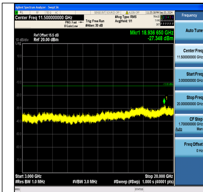
Band2_15MHz_16QAM_18900_1RB#0_3000~20000_3000~20000
