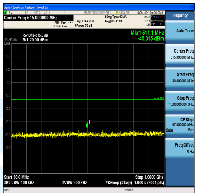
Band2_15MHz_16QAM_18900_1RB#74_30~1000_30~1000
