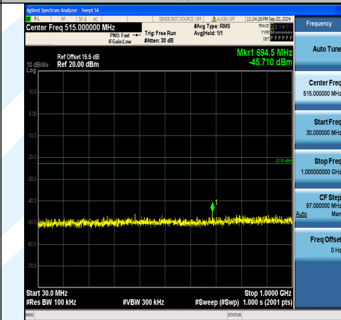
Band2_15MHz_16QAM_18675_75RB#0_30~1000_30~1000
