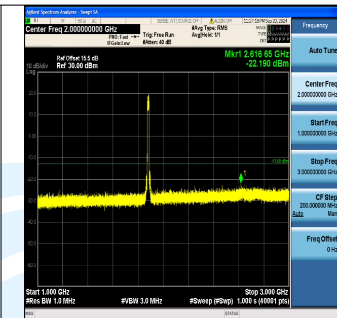
Band2_15MHz_16QAM_18900_75RB#0_1000~3000_1000~3000
