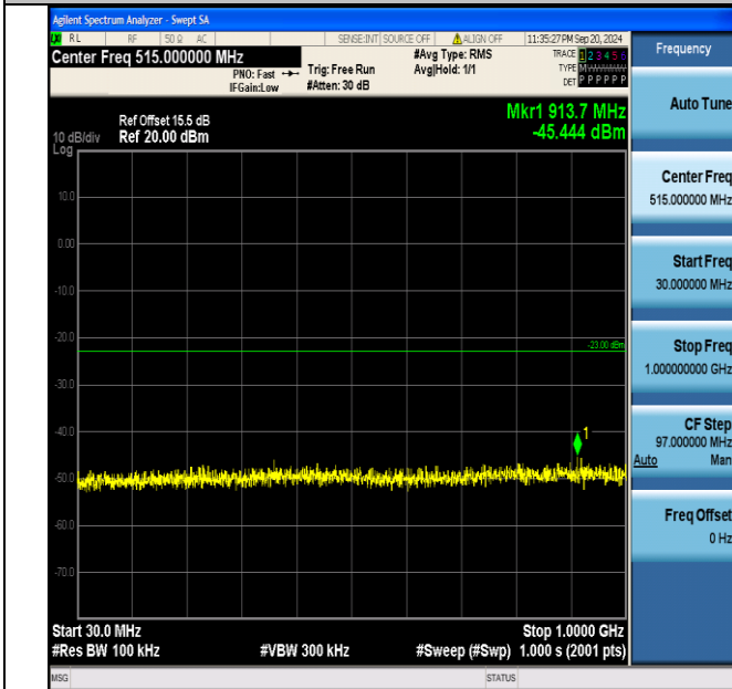
Band2_20MHz_QPSK_19100_1RB#0_30~1000_30~1000
