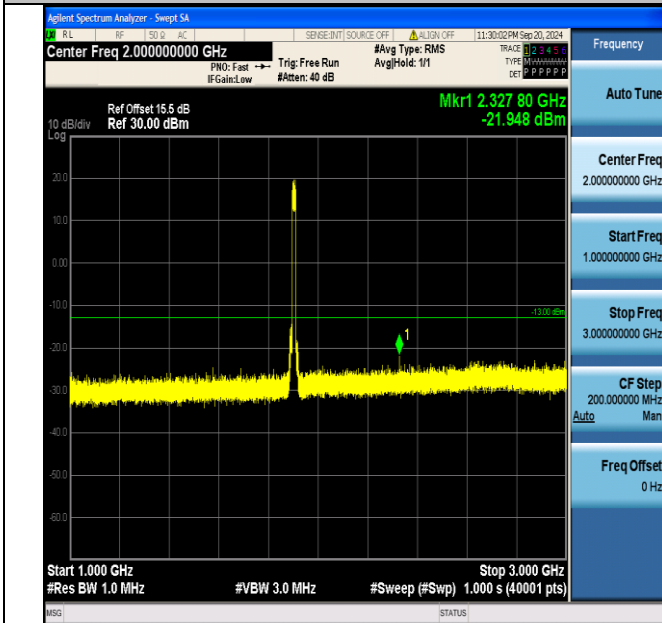
Band2_15MHz_16QAM_19125_75RB#0_1000~3000_1000~3000
