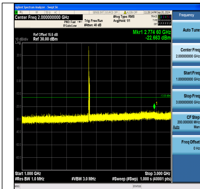
Band2_15MHz_16QAM_19125_1RB#0_1000~3000_1000~3000
