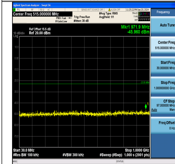
Band2_15MHz_16QAM_18900_1RB#0_30~1000_30~1000
