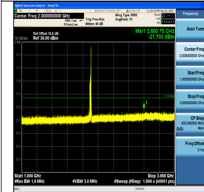
Band2_20MHz_QPSK_19100_1RB#99_1000~3000_1000~3000
