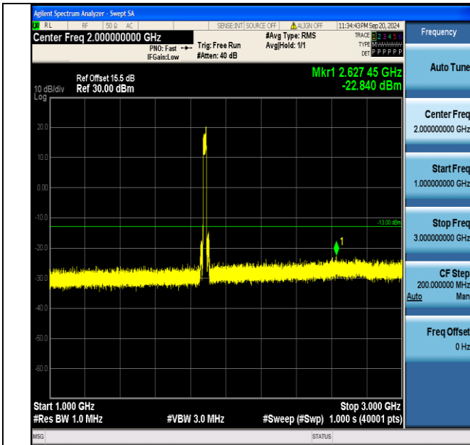
Band2_20MHz_QPSK_18900_100RB#0_1000~3000_1000~3000
