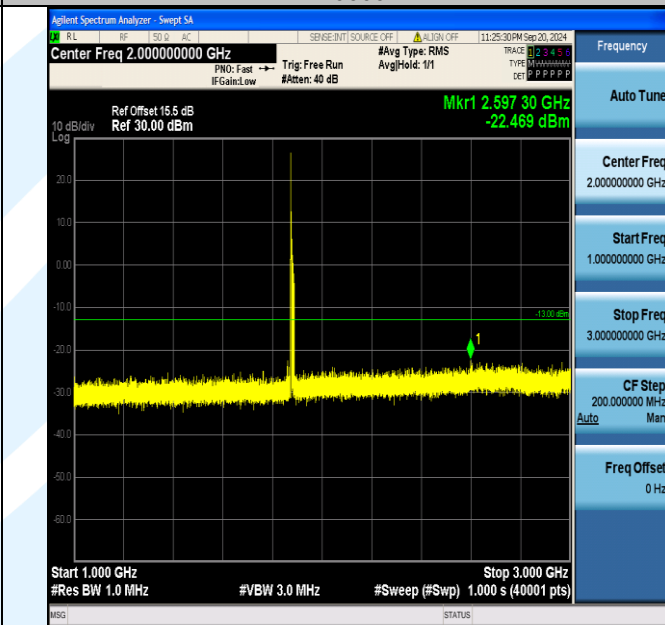
Band2_15MHz_16QAM_18900_1RB#0_1000~3000_1000~3000
