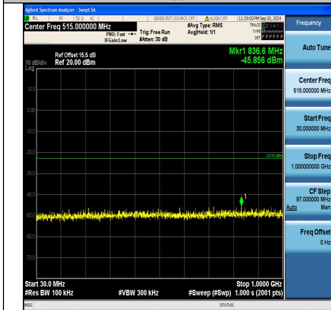
Band2_15MHz_16QAM_19125_1RB#74_30~1000_30~1000
