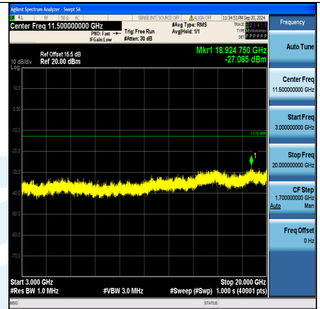
Band2_20MHz_QPSK_18900_100RB#0_3000~20000_3000~20000
