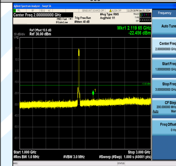
Band2_15MHz_QPSK_19125_75RB#0_1000~3000_1000~3000
