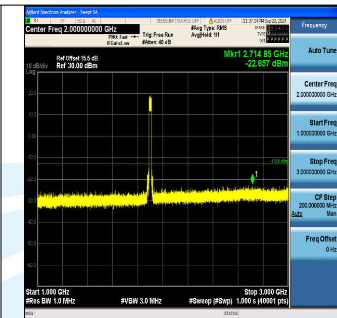
Band2_20MHz_QPSK_19100_100RB#0_1000~3000_1000~3000
