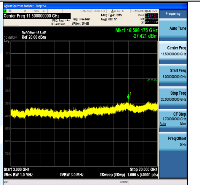
Band2_15MHz_16QAM_18900_1RB#74_3000~20000_3000~20000
