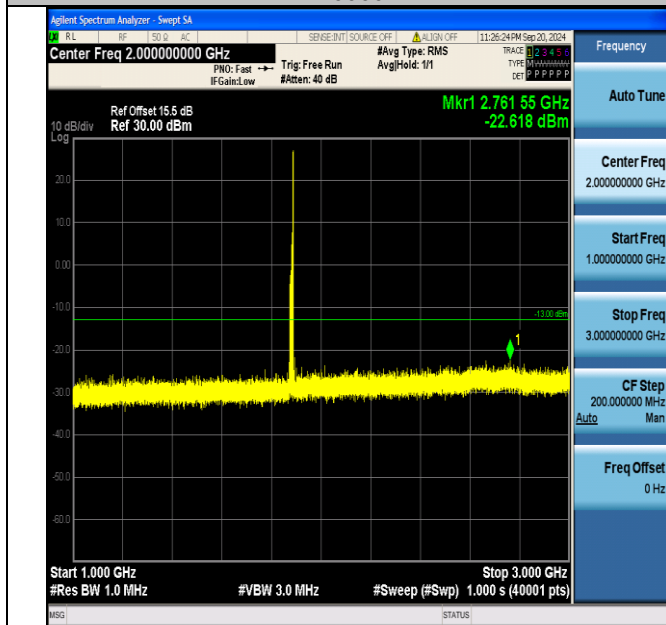
Band2_15MHz_16QAM_18900_1RB#74_1000~3000_1000~3000
