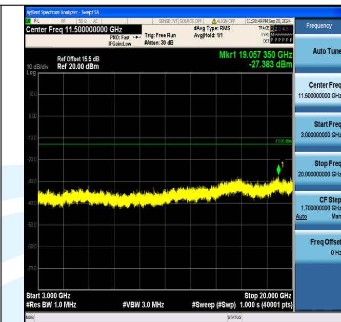
Band2_15MHz_QPSK_19125_1RB#74_3000~20000_3000~20000
