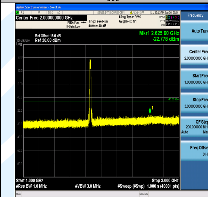
Band2_20MHz_QPSK_18700_100RB#0_1000~3000_1000~3000
