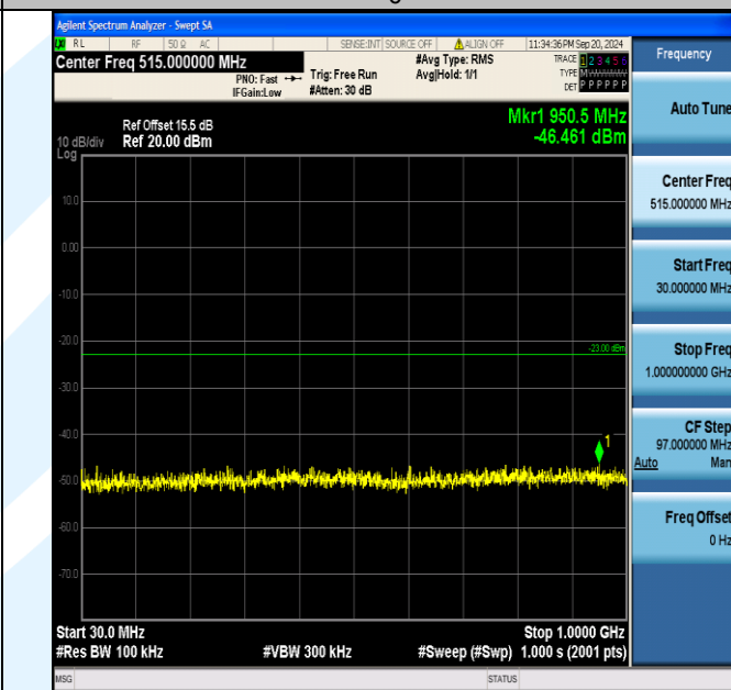
Band2_20MHz_QPSK_18900_100RB#0_30~1000_30~1000
