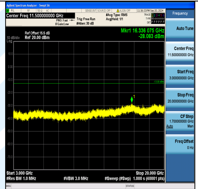
Band2_20MHz_QPSK_19100_1RB#99_3000~20000_3000~20000
