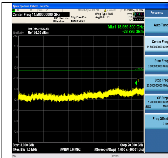
Band2_15MHz_QPSK_18900_1RB#74_3000~20000_3000~20000
