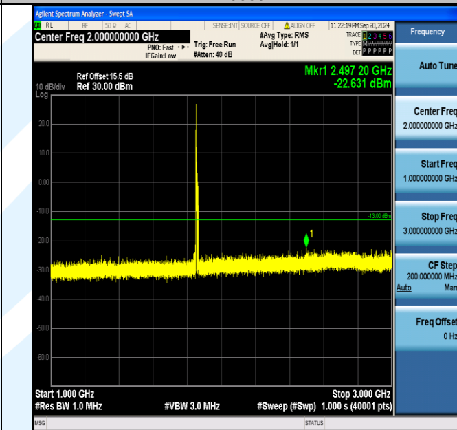
Band2_15MHz_QPSK_18675_1RB#0_1000~3000_1000~3000
