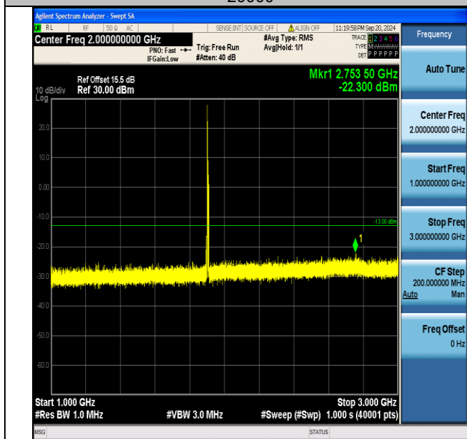
Band2_10MHz_16QAM_19150_1RB#0_1000~3000_1000~3000
