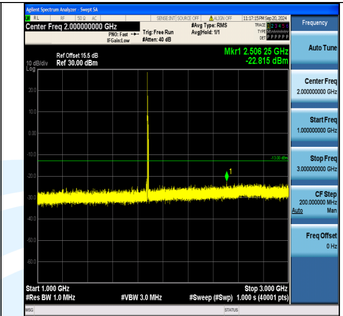
Band2_10MHz_16QAM_18900_1RB#0_1000~3000_1000~3000
