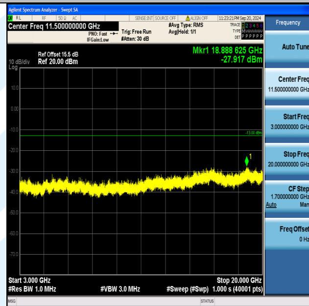
Band2_15MHz_QPSK_18675_1RB#74_3000~20000_3000~20000
