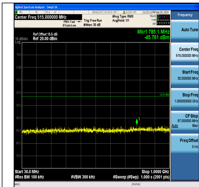
Band2_10MHz_QPSK_19150_50RB#0_30~1000_30~1000
