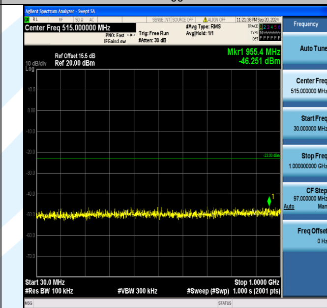
Band2_10MHz_16QAM_19150_50RB#0_30~1000_30~1000
