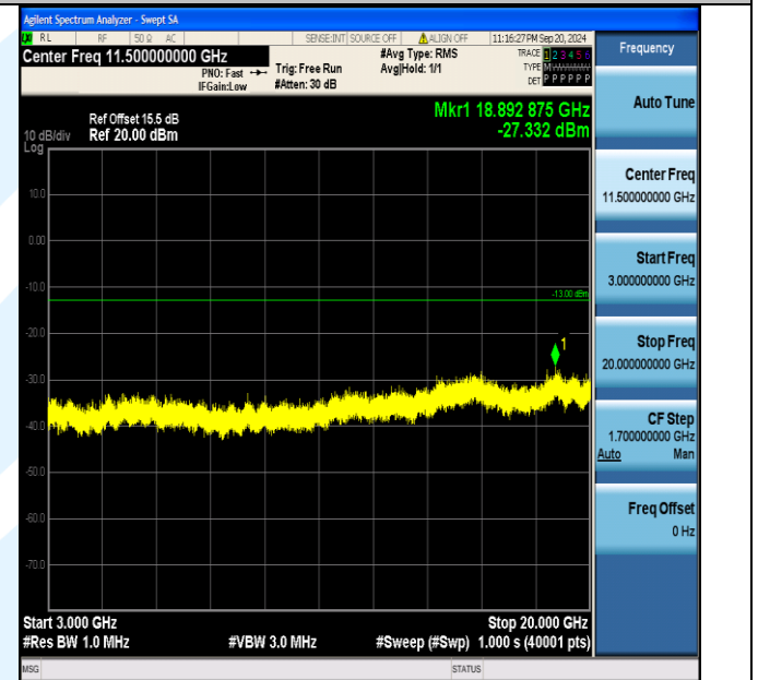
Band2_10MHz_16QAM_18650_50RB#0_3000~20000_3000~20000
