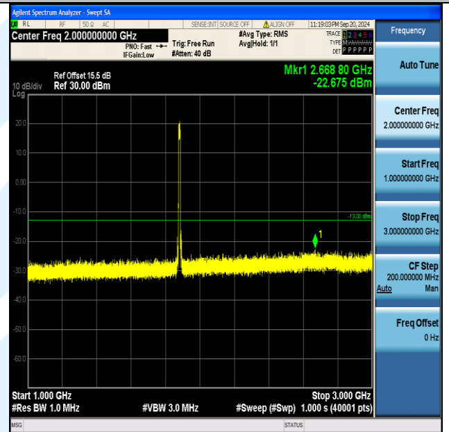
Band2_10MHz_16QAM_18900_50RB#0_1000~3000_1000~3000
