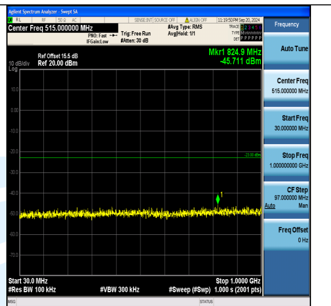
Band2_10MHz_16QAM_19150_1RB#0_30~1000_30~1000
