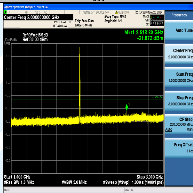
Band2_10MHz_QPSK_19150_1RB#0_1000~3000_1000~3000
