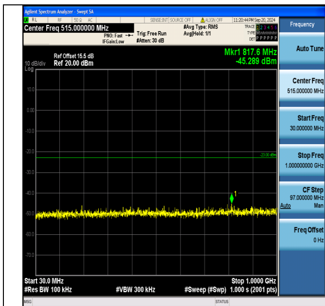
Band2_10MHz_16QAM_19150_1RB#49_30~1000_30~1000
