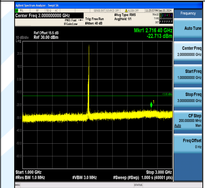
Band2_15MHz_QPSK_18900_1RB#74_1000~3000_1000~3000
