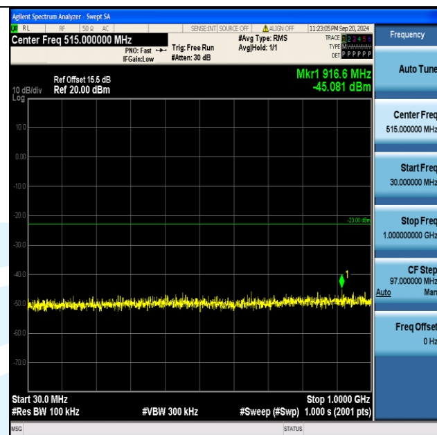
Band2_15MHz_QPSK_18675_1RB#74_30~1000_30~1000
