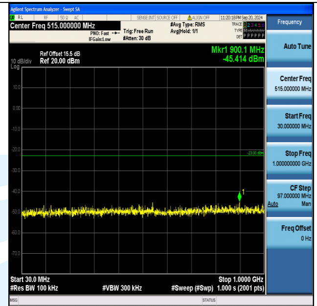
Band2_10MHz_QPSK_19150_1RB#49_30~1000_30~1000
