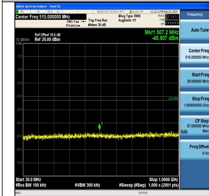
Band2_15MHz_QPSK_18675_1RB#0_30~1000_30~1000
