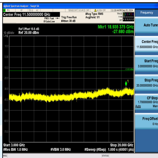
Band2_10MHz_QPSK_18900_50RB#0_3000~20000_3000~20000
