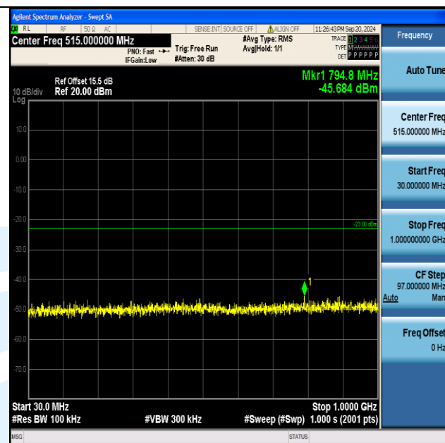
Band2_15MHz_QPSK_18900_75RB#0_30~1000_30~1000
