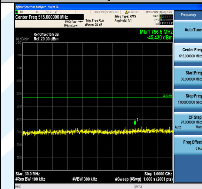
Band2_10MHz_16QAM_18650_1RB#0_30~1000_30~1000
