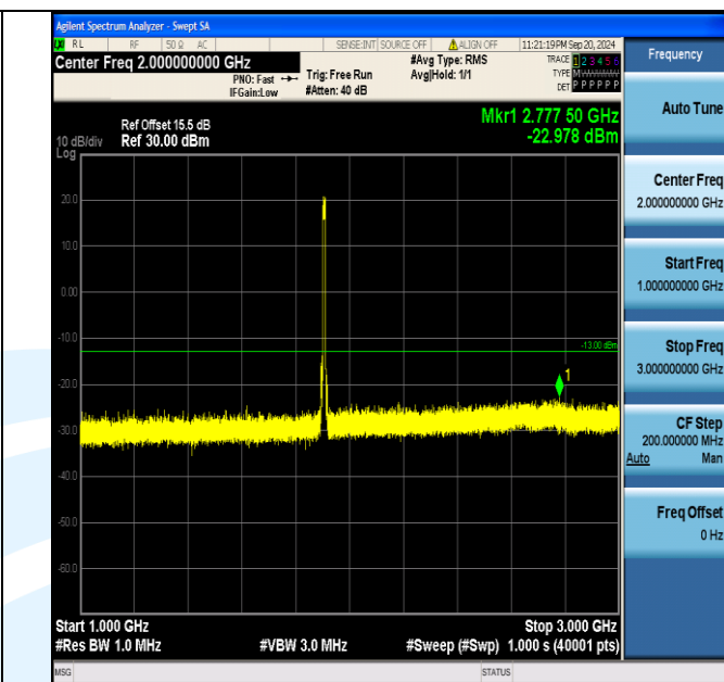
Band2_10MHz_QPSK_19150_50RB#0_1000~3000_1000~3000
