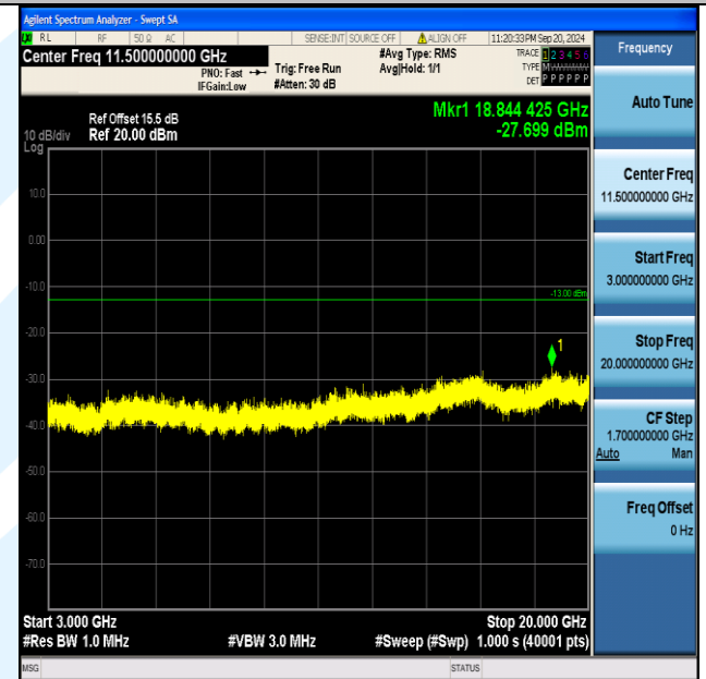
Band2_10MHz_QPSK_19150_1RB#49_3000~20000_3000~20000
