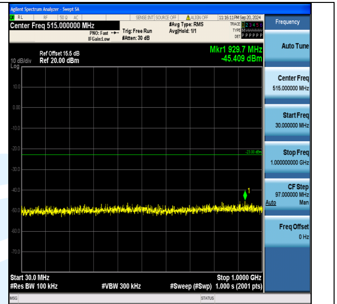
Band2_10MHz_16QAM_18650_50RB#0_30~1000_30~1000
