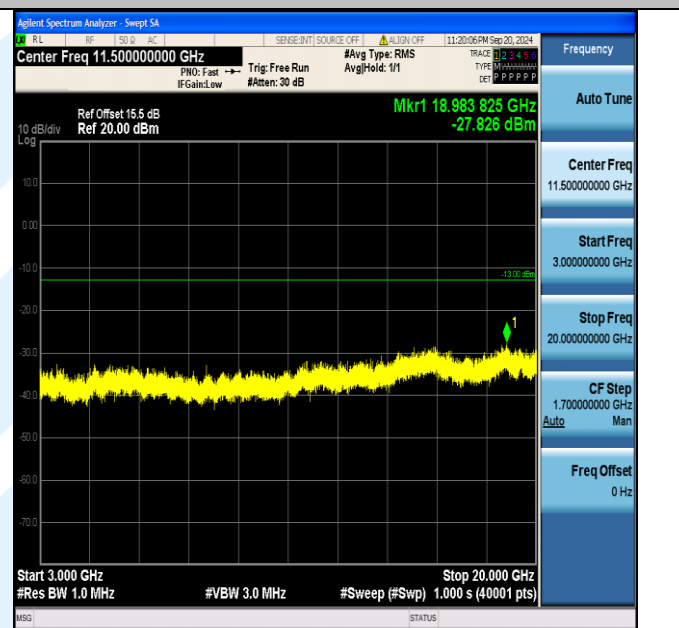
Band2_10MHz_16QAM_19150_1RB#0_3000~20000_3000~20000
