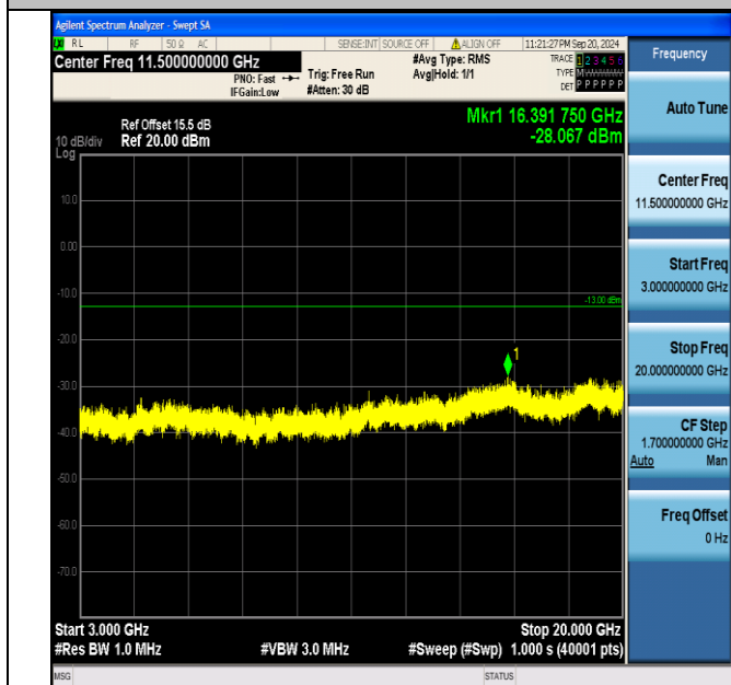
Band2_10MHz_QPSK_19150_50RB#0_3000~20000_3000~20000
