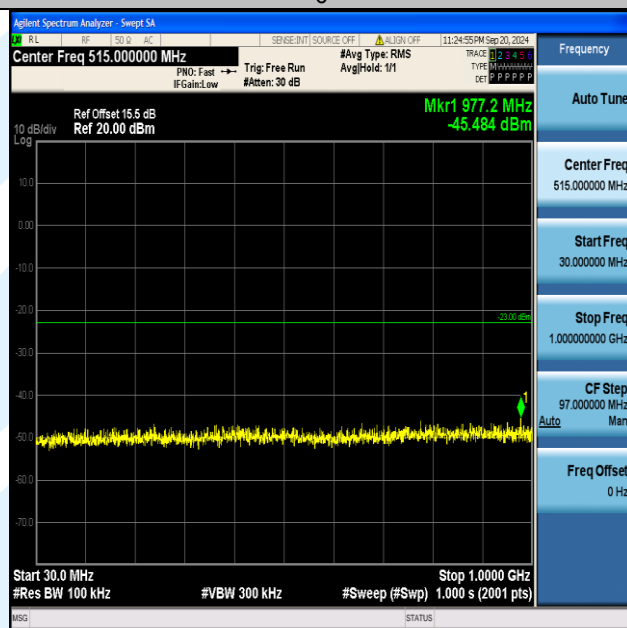
Band2_15MHz_QPSK_18900_1RB#0_30~1000_30~1000
