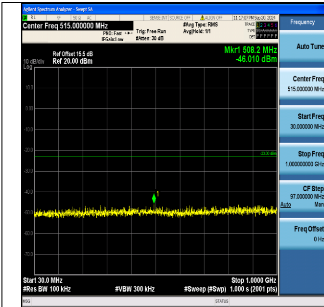
Band2_10MHz_16QAM_18900_1RB#0_30~1000_30~1000
