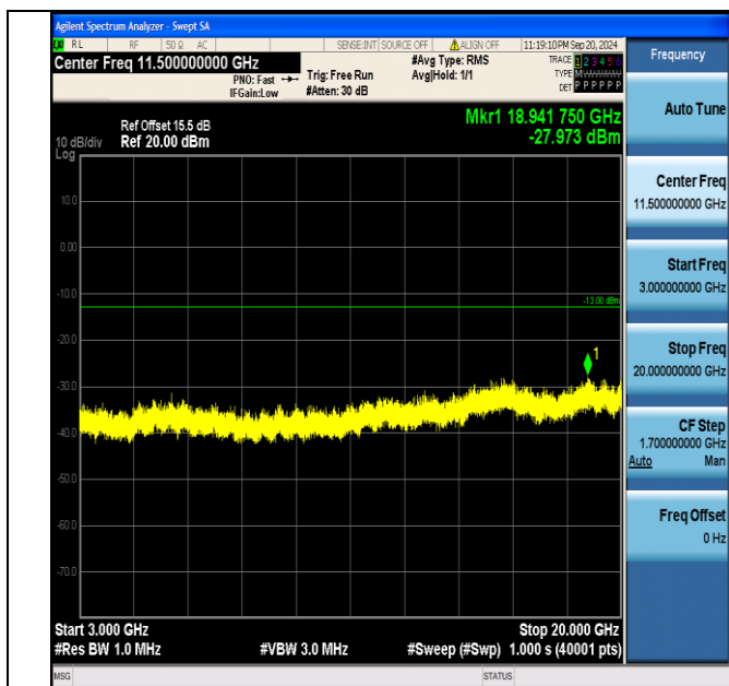
Band2_10MHz_16QAM_18900_50RB#0_3000~20000_3000~20000
