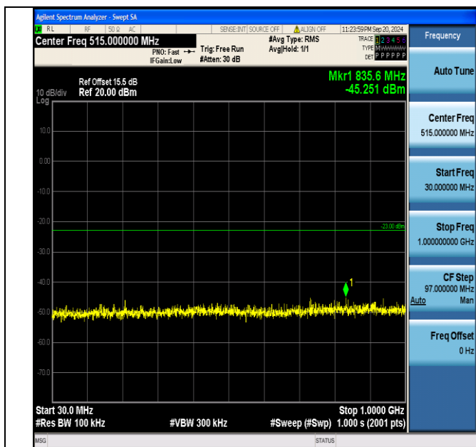
Band2_15MHz_QPSK_18675_75RB#0_30~1000_30~1000
