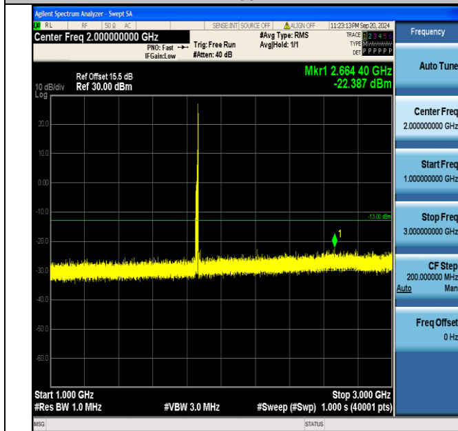
Band2_15MHz_QPSK_18675_1RB#74_1000~3000_1000~3000
