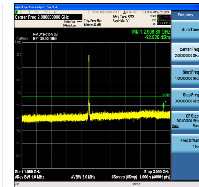
Band2_10MHz_16QAM_19150_50RB#0_1000~3000_1000~3000
