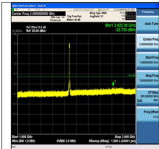
Band2_10MHz_QPSK_18900_50RB#0_1000~3000_1000~3000
