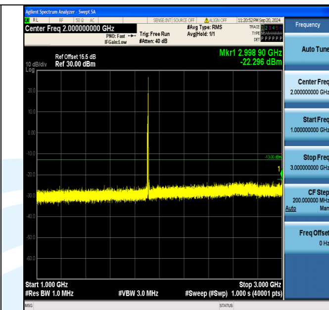
Band2_10MHz_16QAM_19150_1RB#49_1000~3000_1000~3000
