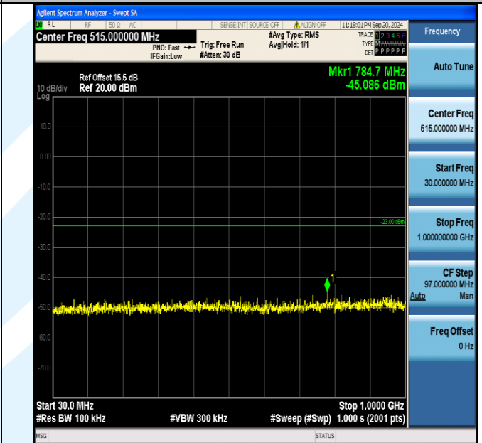
Band2_10MHz_16QAM_18900_1RB#49_30~1000_30~1000
