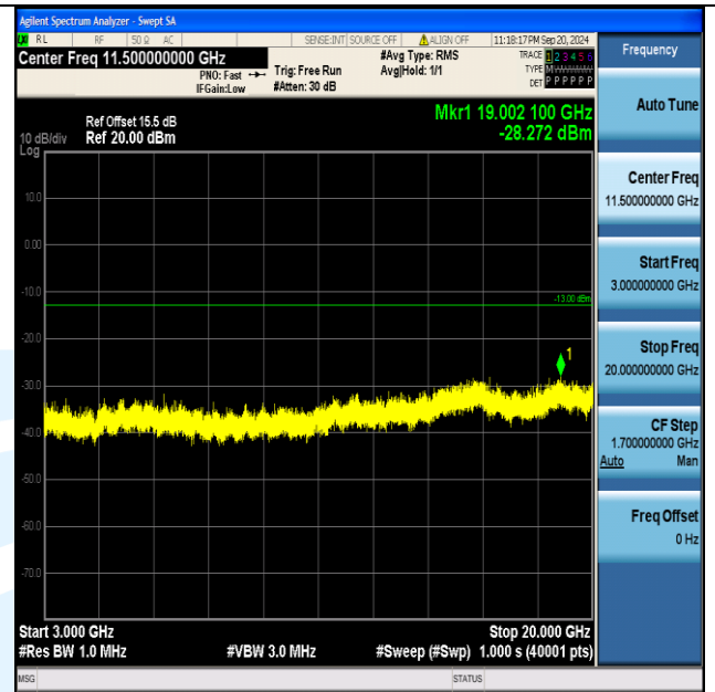
Band2_10MHz_16QAM_18900_1RB#49_3000~20000_3000~20000
