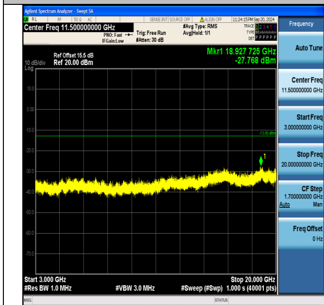
Band2_15MHz_QPSK_18675_75RB#0_3000~20000_3000~20000
