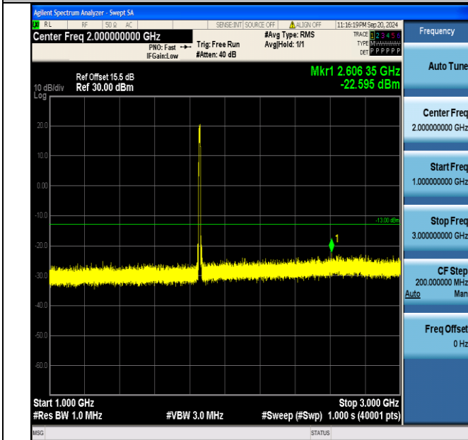
Band2_10MHz_16QAM_18650_50RB#0_1000~3000_1000~3000
