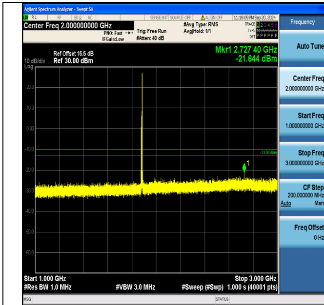
Band2_10MHz_16QAM_18900_1RB#49_1000~3000_1000~3000
