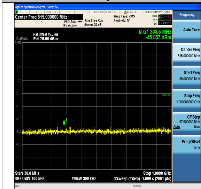
Band2_10MHz_QPSK_19150_1RB#0_30~1000_30~1000
