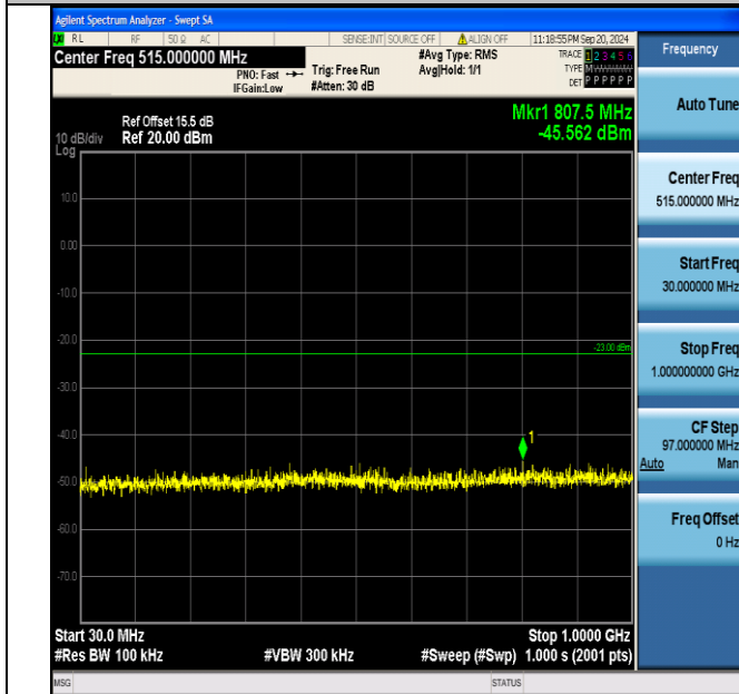
Band2_10MHz_16QAM_18900_50RB#0_30~1000_30~1000
