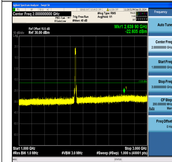
Band2_15MHz_QPSK_18900_75RB#0_1000~3000_1000~3000
