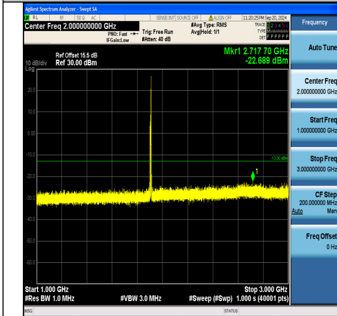
Band2_10MHz_QPSK_19150_1RB#49_1000~3000_1000~3000
