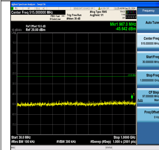
Band2_15MHz_QPSK_18900_1RB#74_30~1000_30~1000
