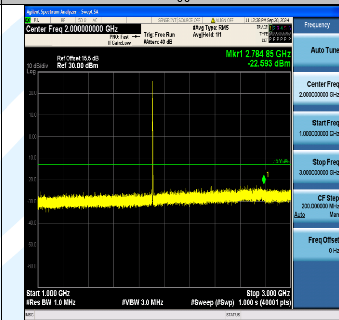
Band2_5MHz_16QAM_19175_1RB#24_1000~3000_1000~3000
