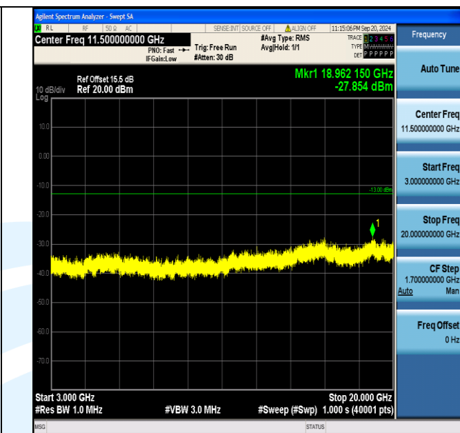
Band2_10MHz_QPSK_18650_1RB#49_3000~20000_3000~20000
