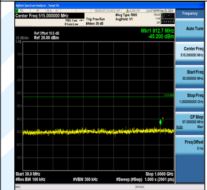
Band2_5MHz_16QAM_18625_25RB#0_30~1000_30~1000
