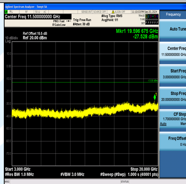
Band2_5MHz_16QAM_18900_1RB#24_3000~20000_3000~20000
