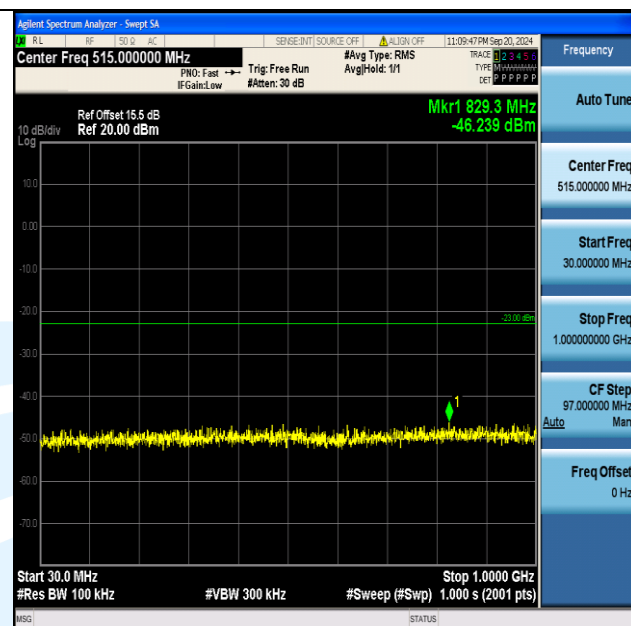
Band2_5MHz_16QAM_18900_1RB#24_30~1000_30~1000
