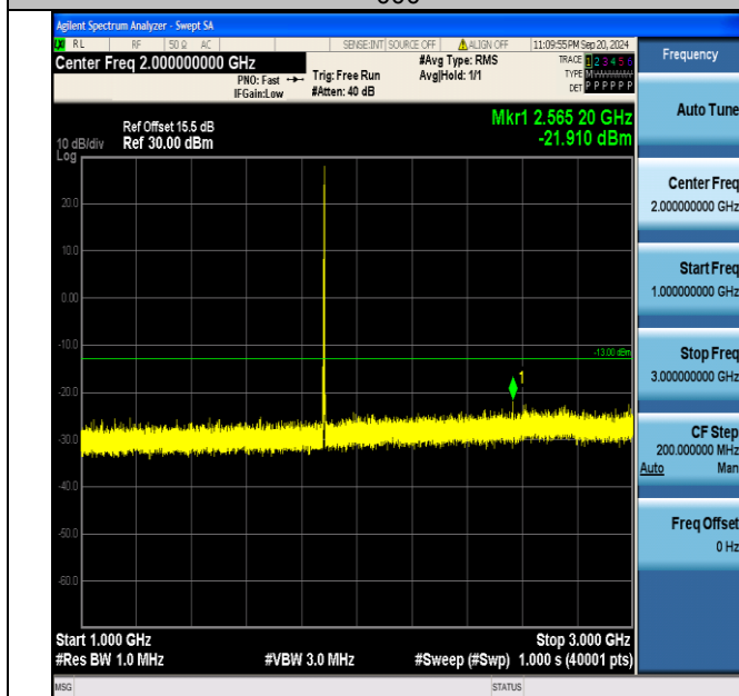
Band2_5MHz_16QAM_18900_1RB#24_1000~3000_1000~3000
