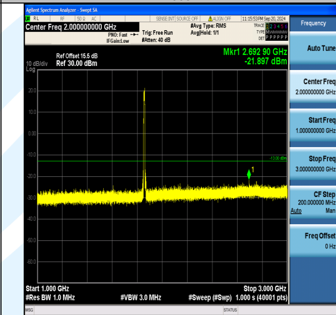
Band2_10MHz_QPSK_18650_50RB#0_1000~3000_1000~3000
