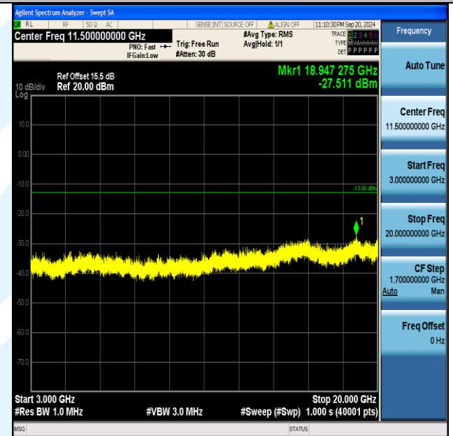
Band2_5MHz_QPSK_18900_25RB#0_3000~20000_3000~20000
