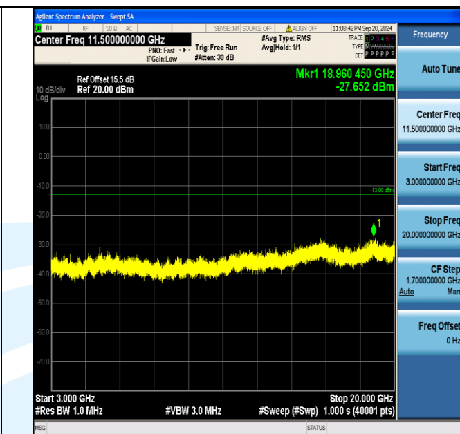
Band2_5MHz_QPSK_18900_1RB#0_3000~20000_3000~20000
