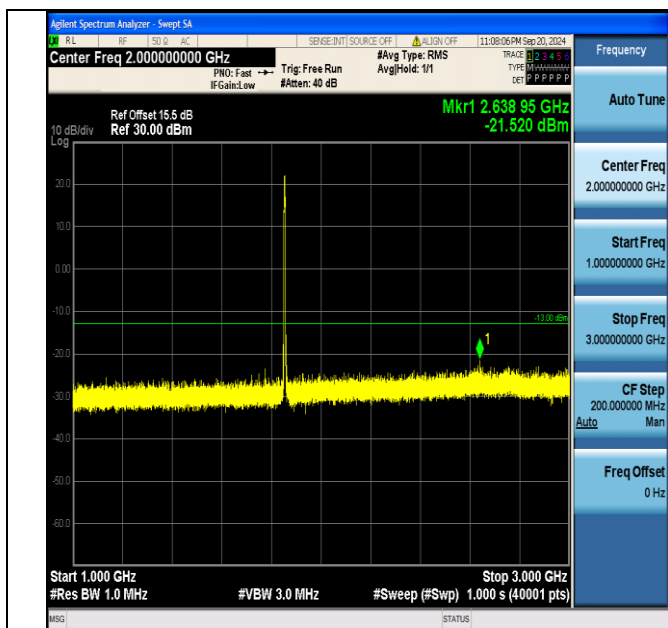
Band2_5MHz_16QAM_18625_25RB#0_1000~3000_1000~3000
