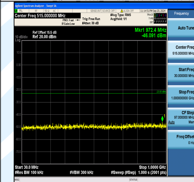
Band2_10MHz_QPSK_18650_1RB#49_30~1000_30~1000
