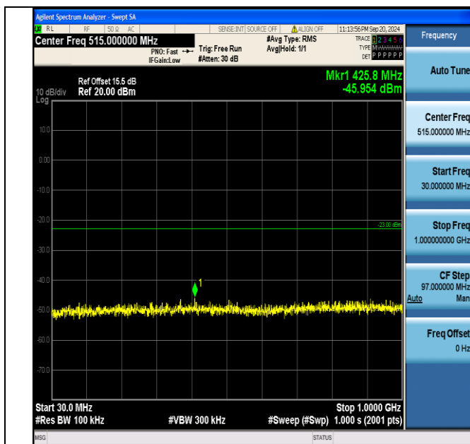
Band2_10MHz_QPSK_18650_1RB#0_30~1000_30~1000
