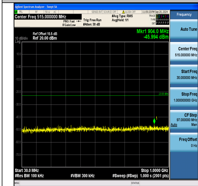
Band2_5MHz_QPSK_18900_1RB#24_30~1000_30~1000
