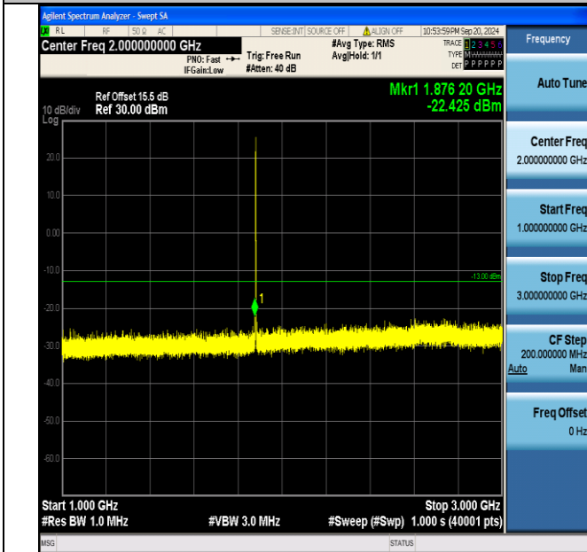
Band2_1.4MHz_QPSK_18900_6RB#0_1000~3000_1000~3000
