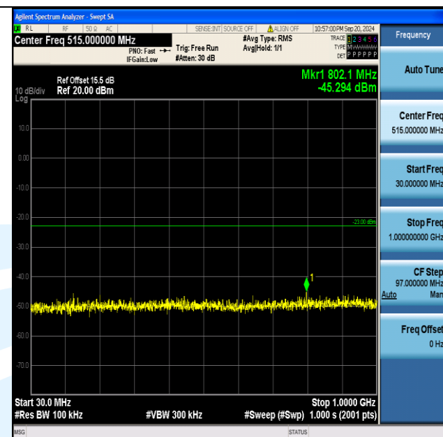
Band2_1.4MHz_16QAM_19193_6RB#0_30~1000_30~1000
