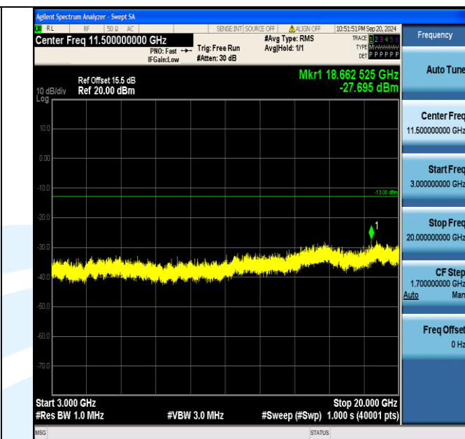
Band2_1.4MHz_16QAM_18607_6RB#0_3000~20000_3000~20000
