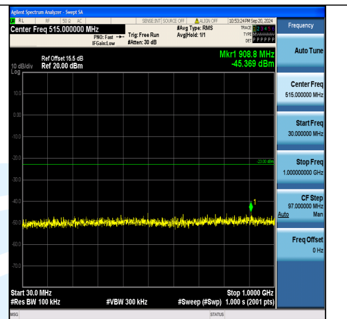
Band2_1.4MHz_16QAM_18900_1RB#5_30~1000_30~1000
