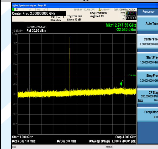
Band2_1.4MHz_QPSK_18900_1RB#5_1000~3000_1000~3000
