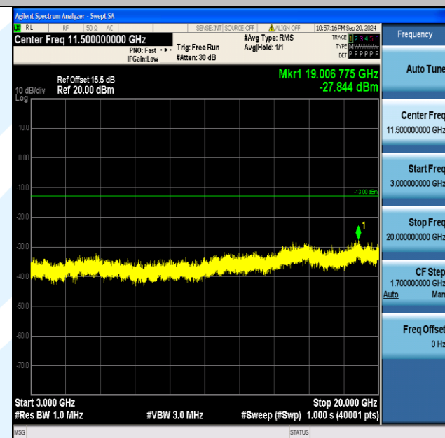
Band2_1.4MHz_16QAM_19193_6RB#0_3000~20000_3000~20000
