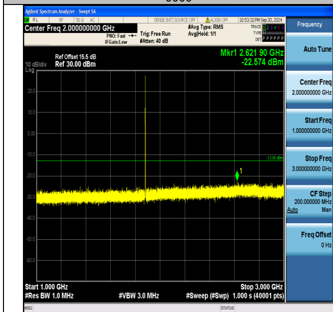
Band2_1.4MHz_16QAM_18900_1RB#5_1000~3000_1000~3000
