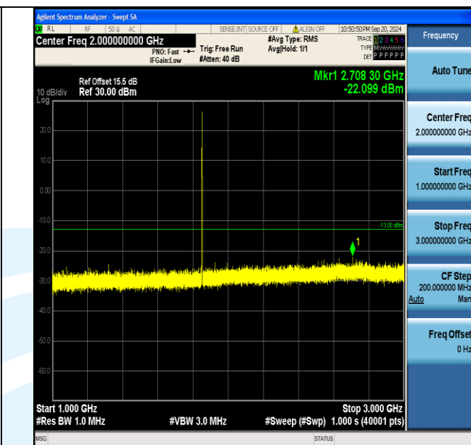
Band2_1.4MHz_16QAM_18607_1RB#5_1000~3000_1000~3000 0
