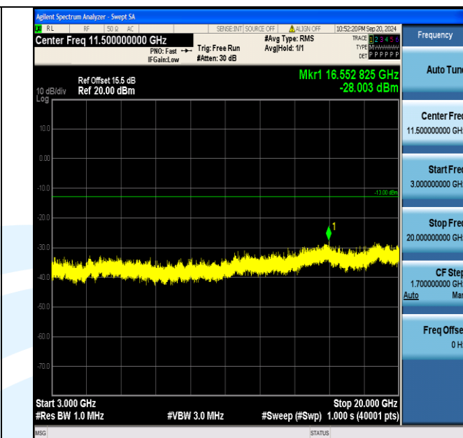
Band2_1.4MHz_QPSK_18900_1RB#0_3000~20000_3000~20000
