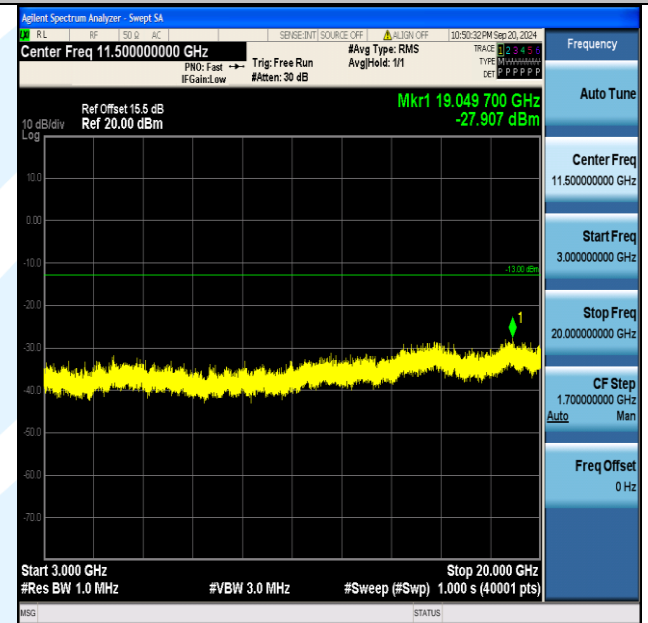
Band2_1.4MHz_QPSK_18607_1RB#5_3000~20000_3000~20000
