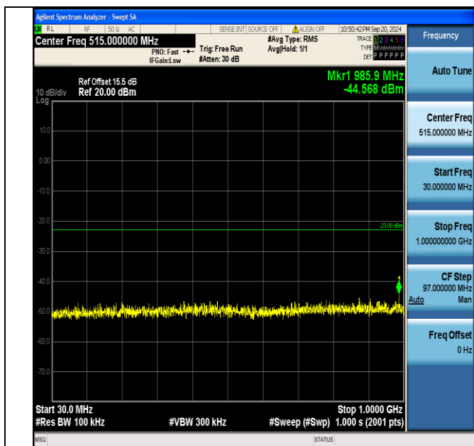
Band2_1.4MHz_16QAM_18607_1RB#5_30~1000_30~1000
