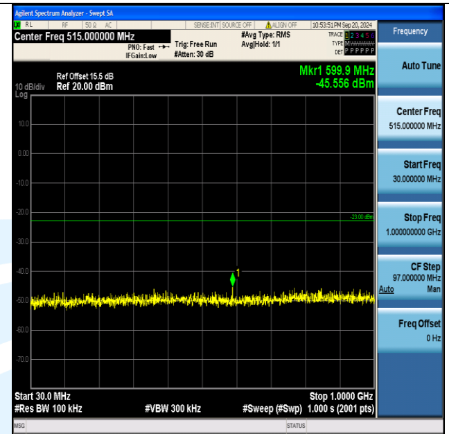
Band2_1.4MHz_QPSK_18900_6RB#0_30~1000_30~1000
