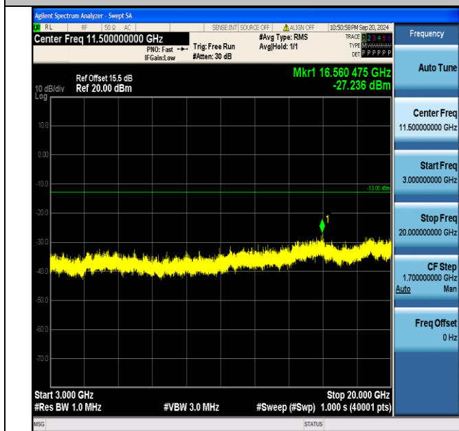
Band2_1.4MHz_16QAM_18607_1RB#5_3000~20000_3000~20000
