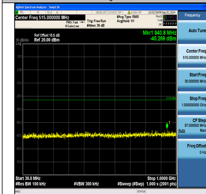
Band2_1.4MHz_QPSK_18900_1RB#5_30~1000_30~1000
