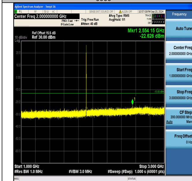
Band2_1.4MHz_16QAM_19193_6RB#0_1000~3000_1000~3000
