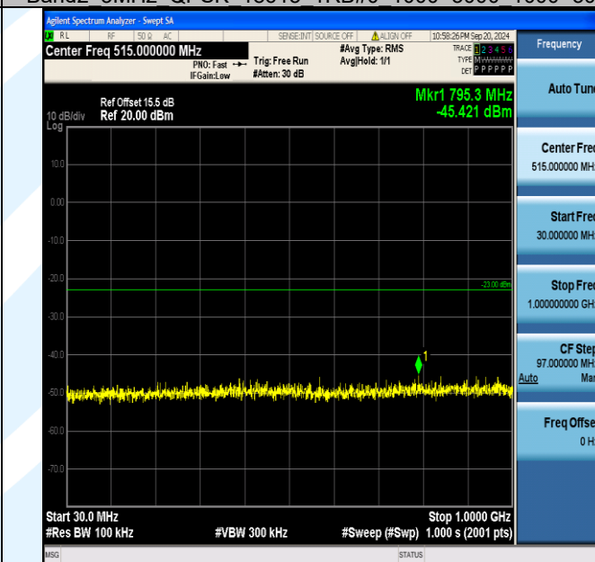
Band2_3MHz_QPSK_18615_1RB#14_30~1000_30~1000
