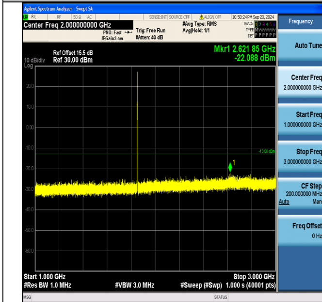
Band2_1.4MHz_QPSK_18607_1RB#5_1000~3000_1000~3000
