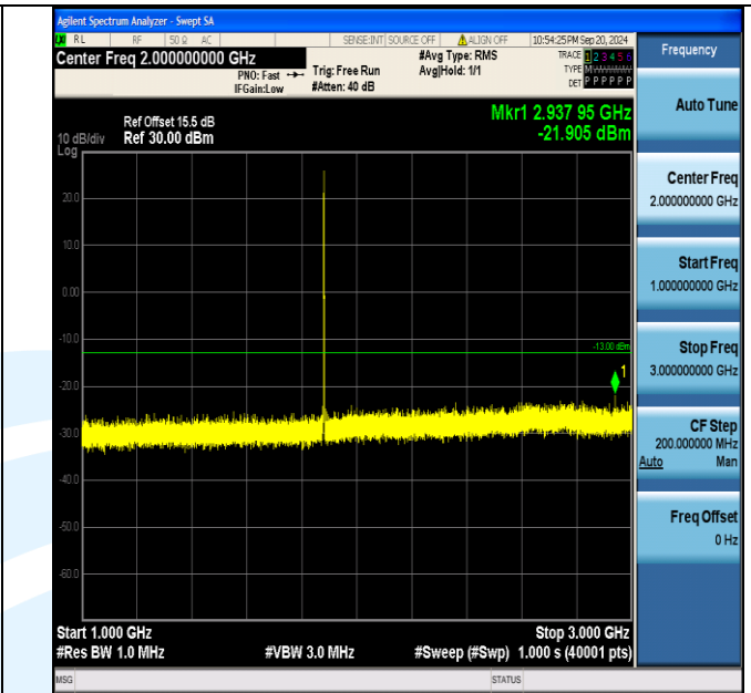
Band2_1.4MHz_16QAM_18900_6RB#0_1000~3000_1000~3000
