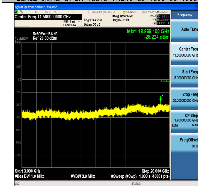
Band2_3MHz_QPSK_18615_1RB#0_3000~20000_3000~2000 0
