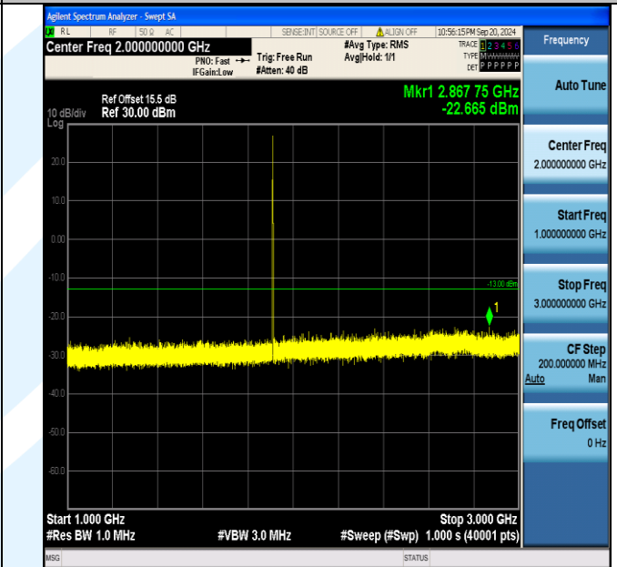
Band2_1.4MHz_16QAM_19193_1RB#5_1000~3000_1000~3000
