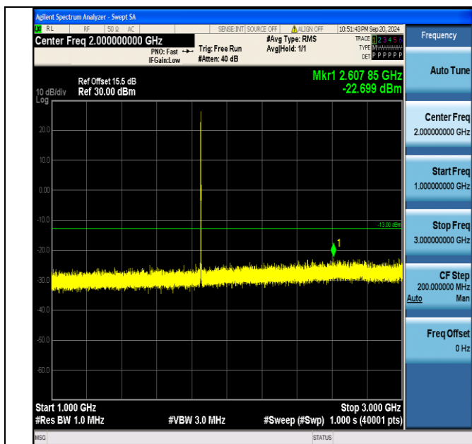
Band2_1.4MHz_16QAM_18607_6RB#0_1000~3000_1000~3000
