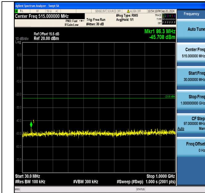
Band2_1.4MHz_16QAM_18900_6RB#0_30~1000_30~1000
