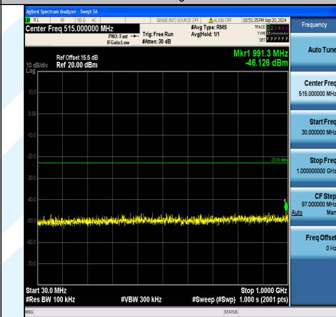
Band2_1.4MHz_16QAM_18607_6RB#0_30~1000_30~1000
