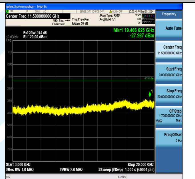
Band2_1.4MHz_16QAM_18900_1RB#5_3000~20000_3000~20000
