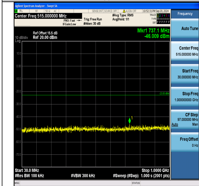
Band2_1.4MHz_16QAM_18900_1RB#0_30~1000_30~1000
