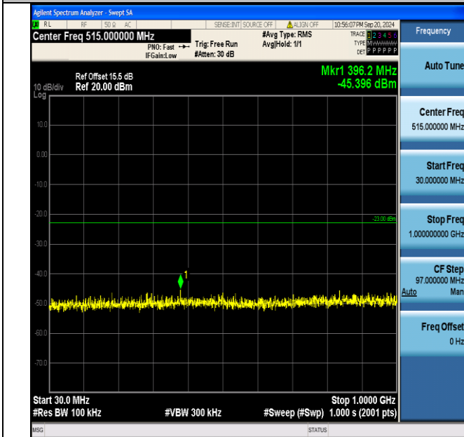
Band2_1.4MHz_16QAM_19193_1RB#5_30~1000_30~1000
