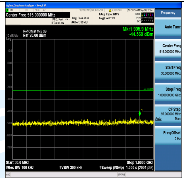
Band2_1.4MHz_QPSK_18607_1RB#5_30~1000_30~1000
