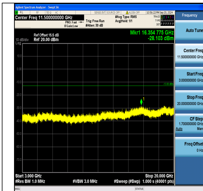
Band2_1.4MHz_16QAM_19193_1RB#5_3000~20000_3000~20000
