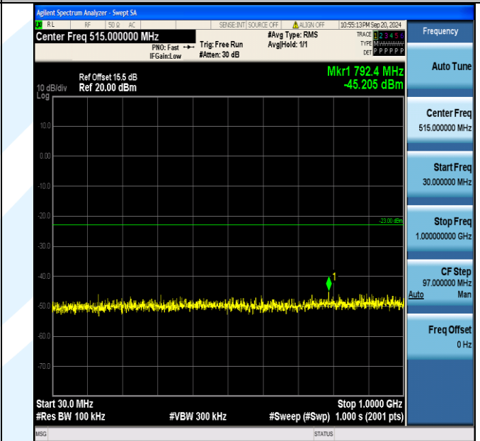
Band2_1.4MHz_16QAM_19193_1RB#0_30~1000_30~1000
