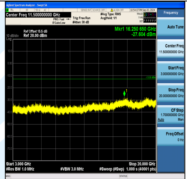
Band2_1.4MHz_QPSK_18900_6RB#0_3000~20000_3000~20000
