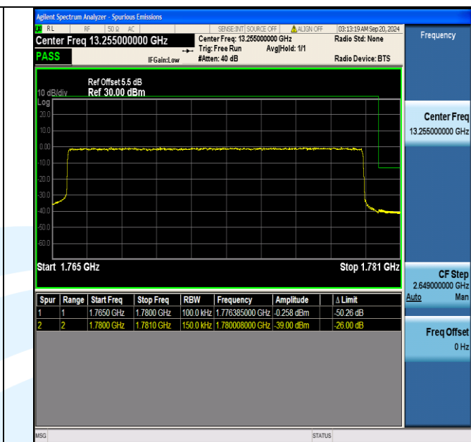
Band66 15MHz QPSK 132597 75RB#0
