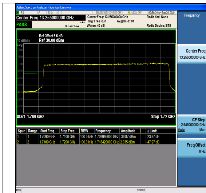
Band66 10MHz 16QAM 132022 50RB#0
