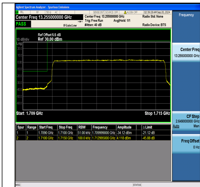
Band66 5MHz 16QAM 131997 25RB#0
