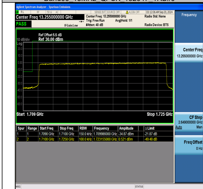
Band66 15MHz QPSK 132047 75RB#0
