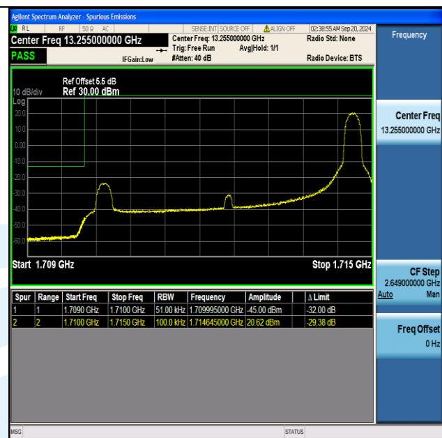
Band66 5MHz QPSK 131997 1RB#24
