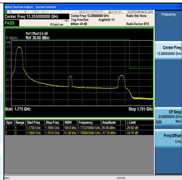
Band66 5MHz 16QAM 132647 1RB#0
