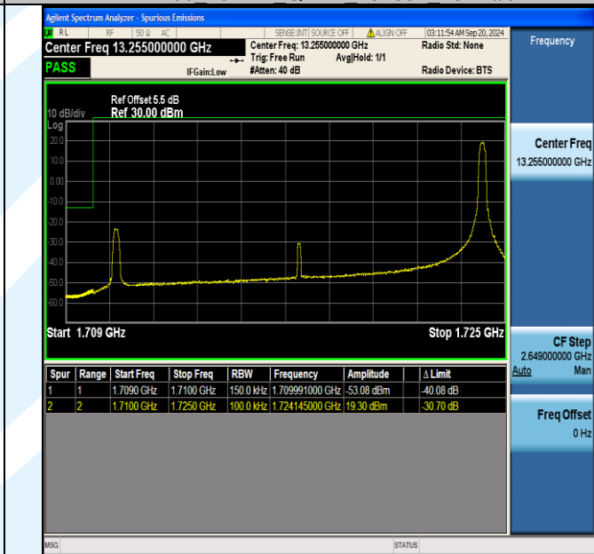
Band66 15MHz 16QAM 132047 1RB#74
