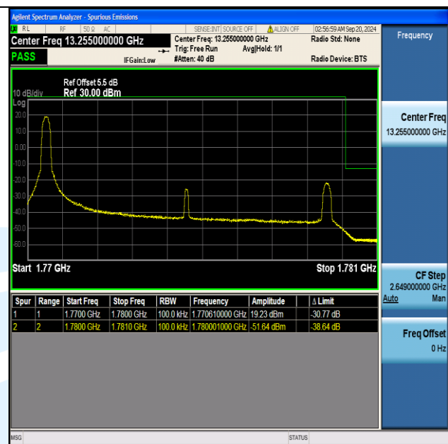
Band66 10MHz 16QAM 132622 1RB#0
