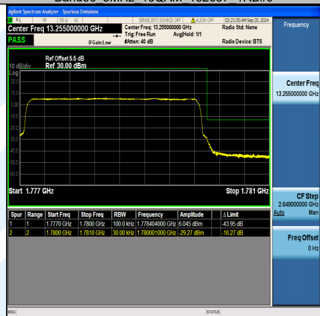
Band66 3MHz 16QAM 132657 15RB#0
