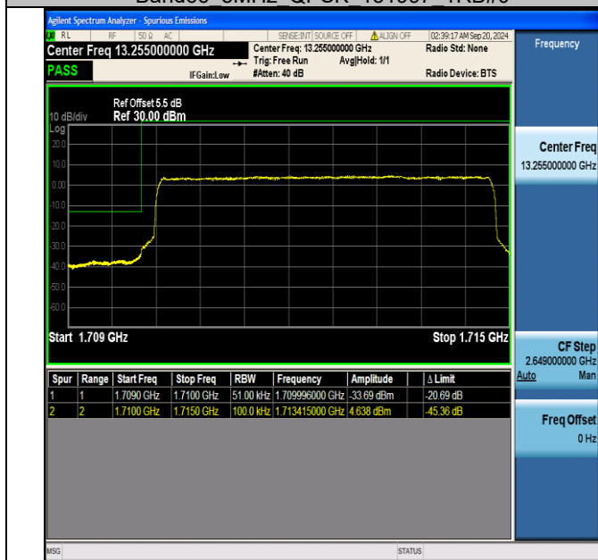
Band66 5MHz QPSK 131997 25RB#0
