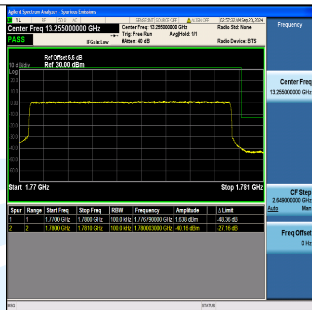
Band66 10MHz QPSK 132622 50RB#0
