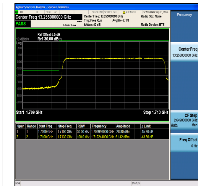
Band66 3MHz 16QAM 131987 15RB#0
