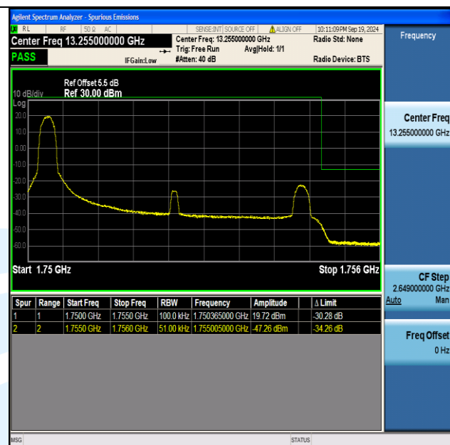
Band4_5MHz_16QAM_20375_1RB#0
