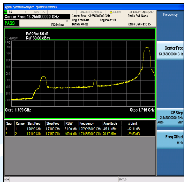
Band4_5MHz_QPSK_19975_1RB#24
