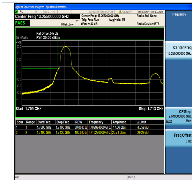
Band4_3MHz_QPSK_19965_1RB#0
