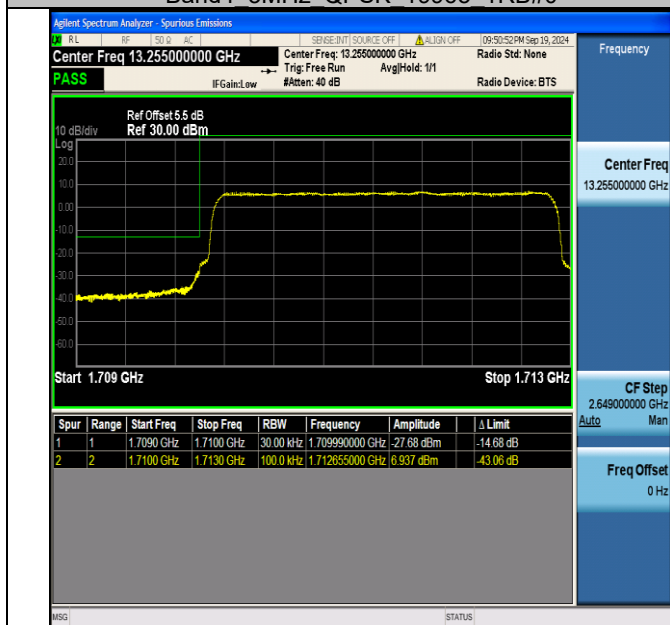
Band4_3MHz_QPSK_19965_15RB#0
