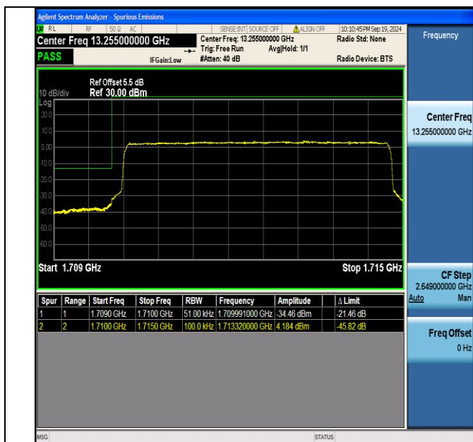
Band4_5MHz_16QAM_19975_25RB#0
