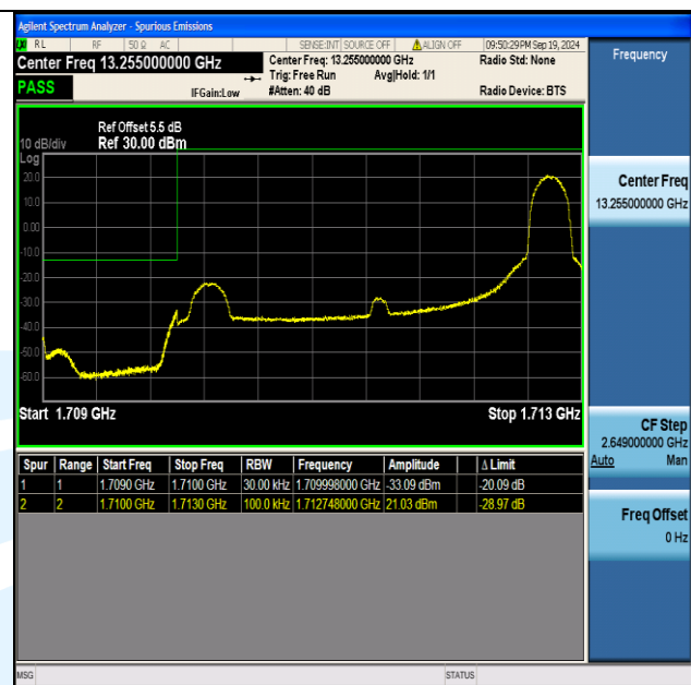
Band4_3MHz_QPSK_19965_1RB#14
