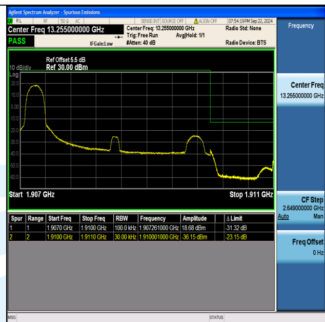
Band2 3MHz 16QAM 19185 1RB#0
