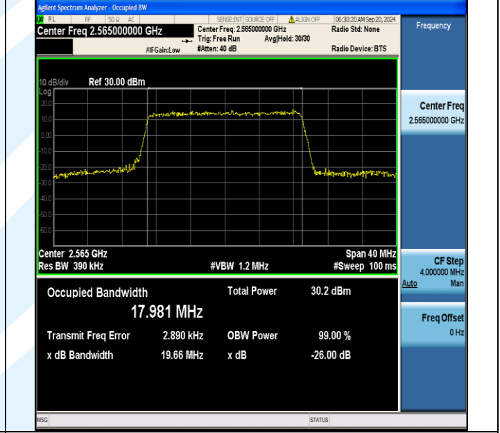
Band41(2555-2655)-20MHz-16QAM-40340-100RB#0-PASS
