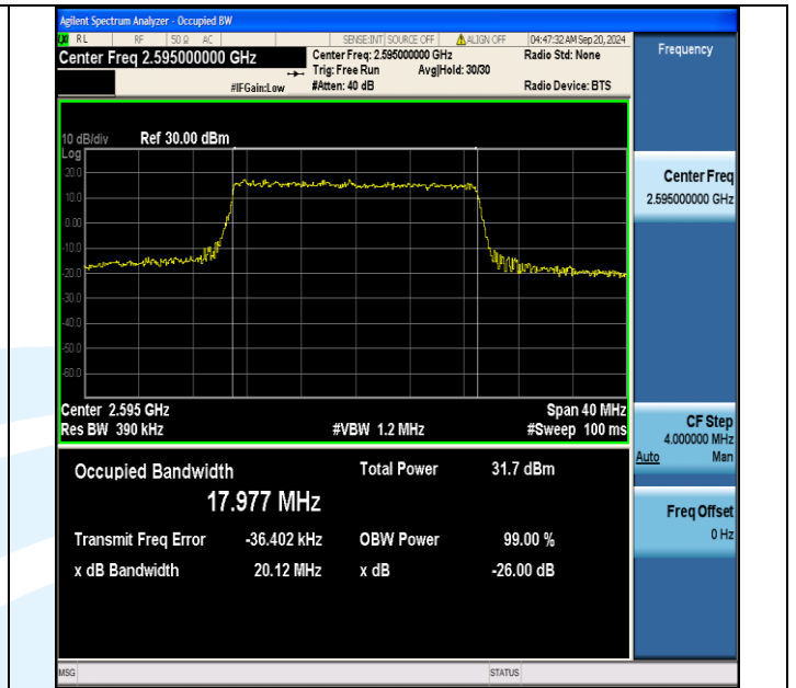
Band38-20MHz-QPSK-38000-100RB#0-PASS
