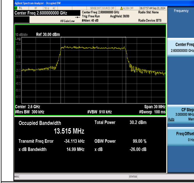
Band41(2555-2655)-15MHz-16QAM-40690-75RB#0-PASS
