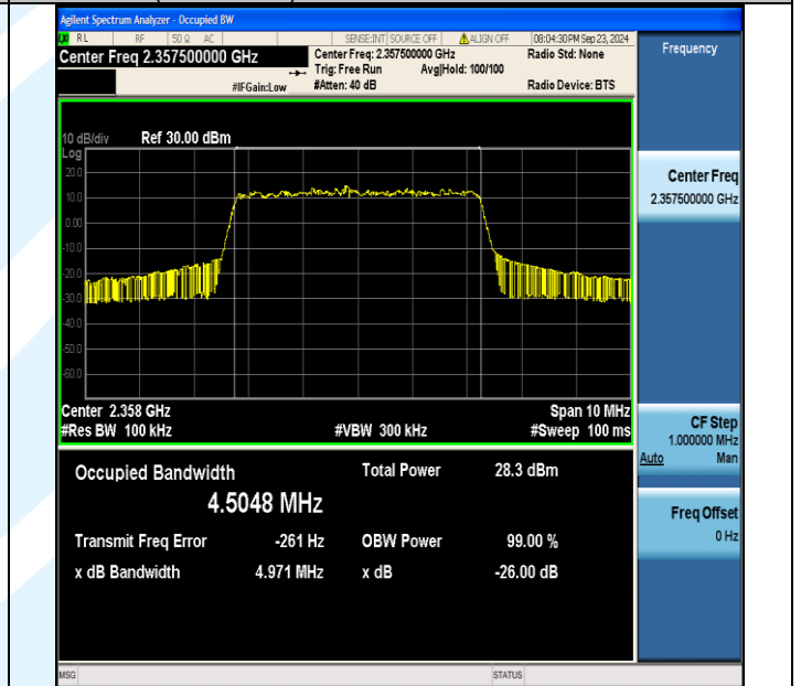
Band40(2350-2360)-5MHz-16QAM-39225-25RB#0-PASS
