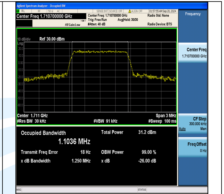
Band66-1.4MHz-16QAM-131979-6RB#0-PASS
