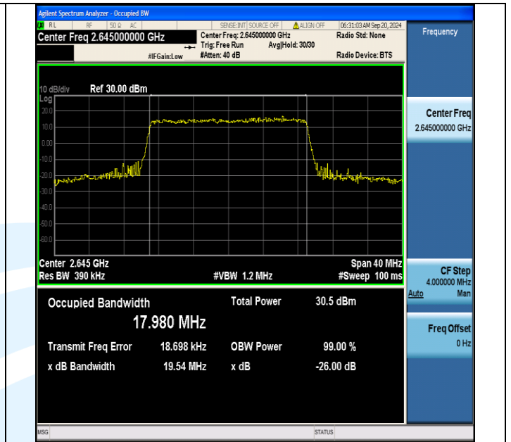
Band41(2555-2655)-20MHz-16QAM-41140-100RB#0-PASS
