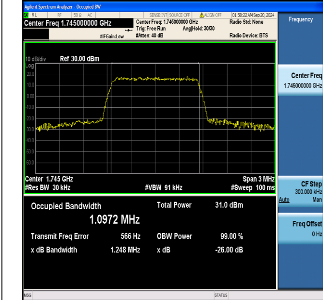
Band66-1.4MHz-16QAM-132322-6RB#0-PASS
