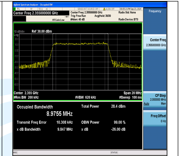
Band40(2350-2360)-10MHz-16QAM-39200-50RB#0-PASS
