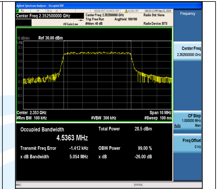
Band40(2350-2360)-5MHz-16QAM-39175-25RB#0-PASS
