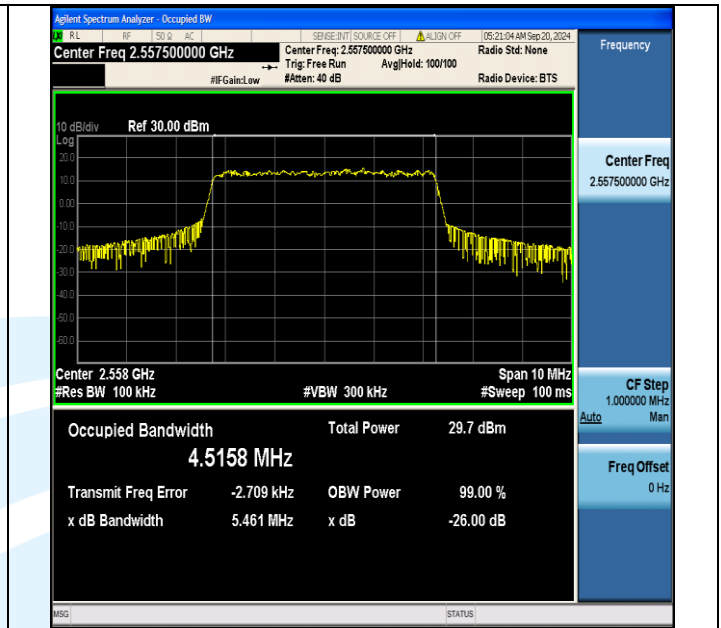
Band41(2555-2655)-5MHz-16QAM-40265-25RB#0-PASS
