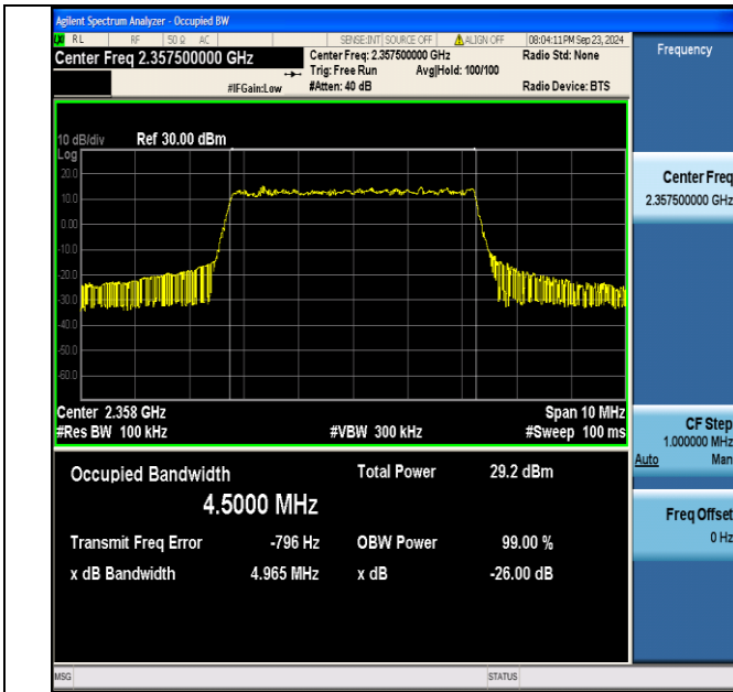
Band40(2350-2360)-5MHz-QPSK-39225-25RB#0-PASS
