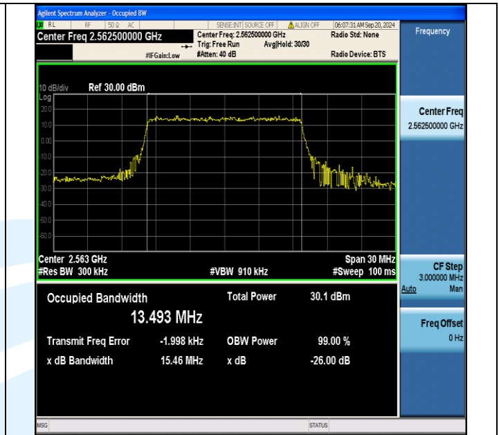
Band41(2555-2655)-15MHz-16QAM-40315-75RB#0-PASS
