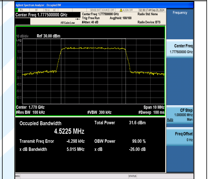
Band66-5MHz-16QAM-132647-25RB#0-PASS
