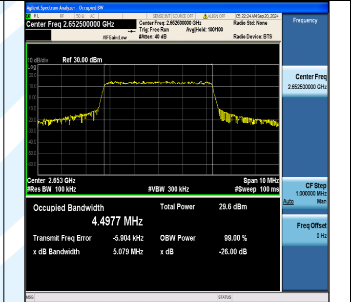
Band41(2555-2655)-5MHz-16QAM-41215-25RB#0-PASS
