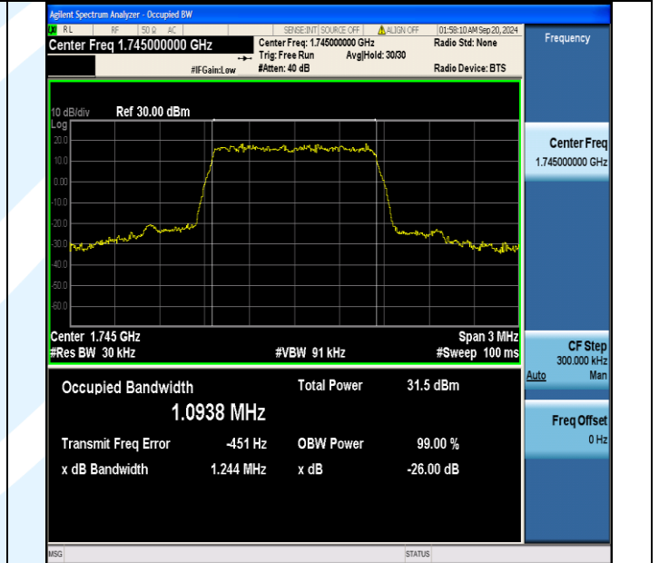
Band66-1.4MHz-QPSK-132322-6RB#0-PASS
