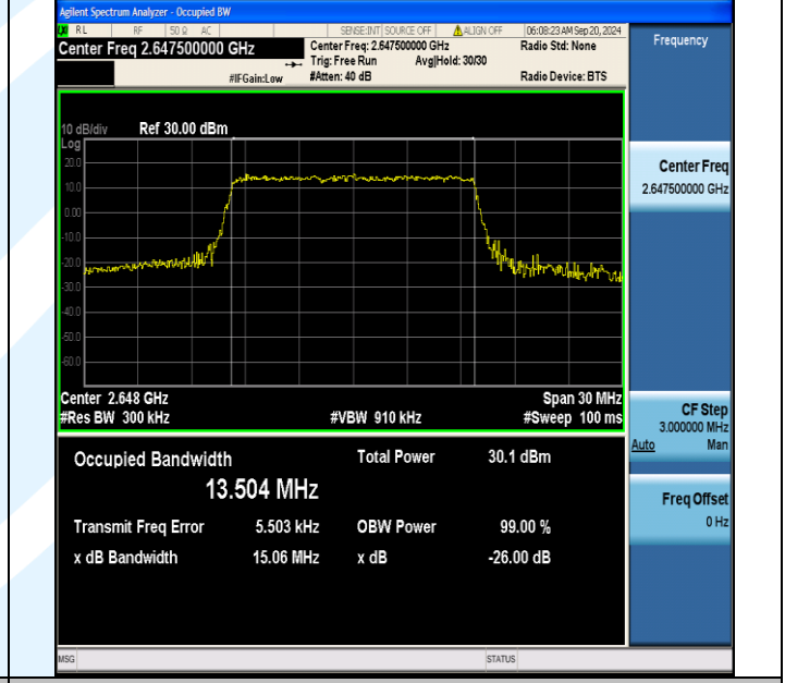
Band41(2555-2655)-15MHz-16QAM-41165-75RB#0-PASS
