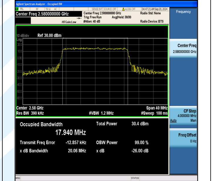
Band38-20MHz-16QAM-37850-100RB#0-PASS
