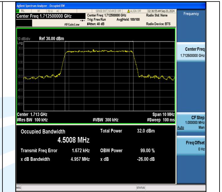
Band66-5MHz-16QAM-131997-25RB#0-PASS
