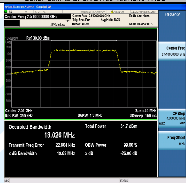
Band7-20MHz-16QAM-20850-100RB#0-PASS
