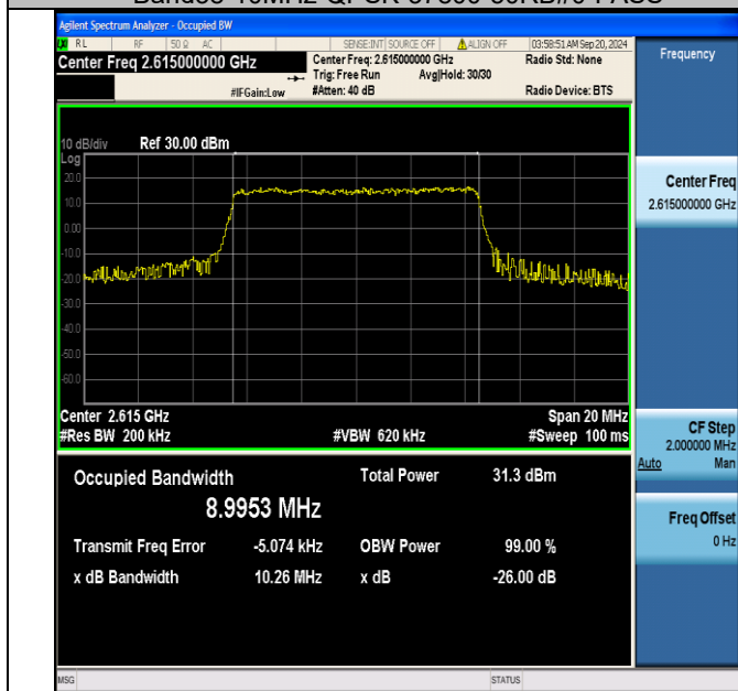
Band38-10MHz-QPSK-38200-50RB#0-PASS
