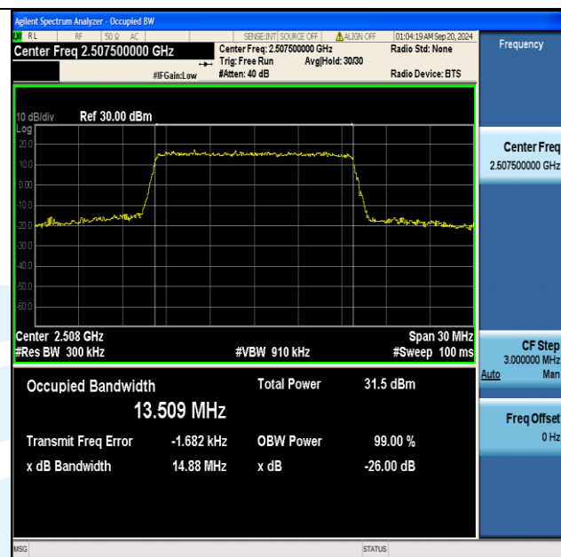
Band7-15MHz-16QAM-20825-75RB#0-PASS
