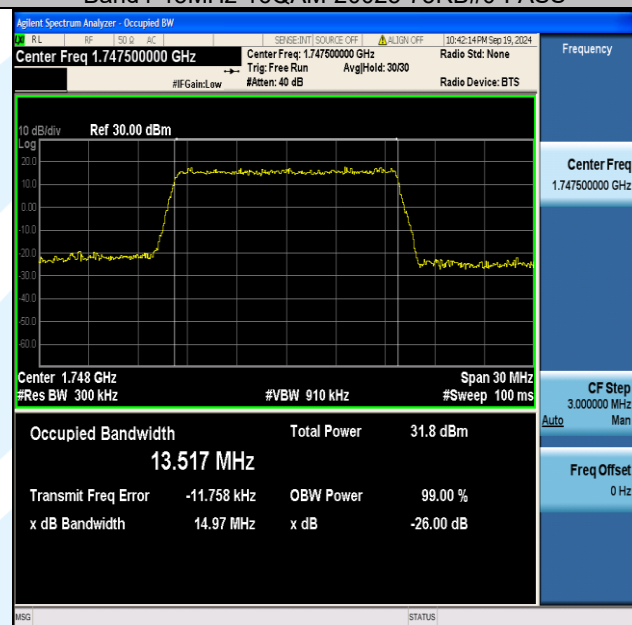
Band4-15MHz-16QAM-20325-75RB#0-PASS
