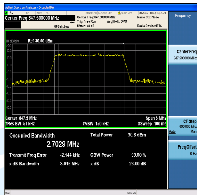
Band5-3MHz-16QAM-20635-15RB#0-PASS
