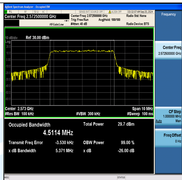
Band38-5MHz-16QAM-37775-25RB#0-PASS
