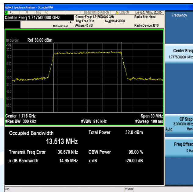
Band4-15MHz-16QAM-20025-75RB#0-PASS
