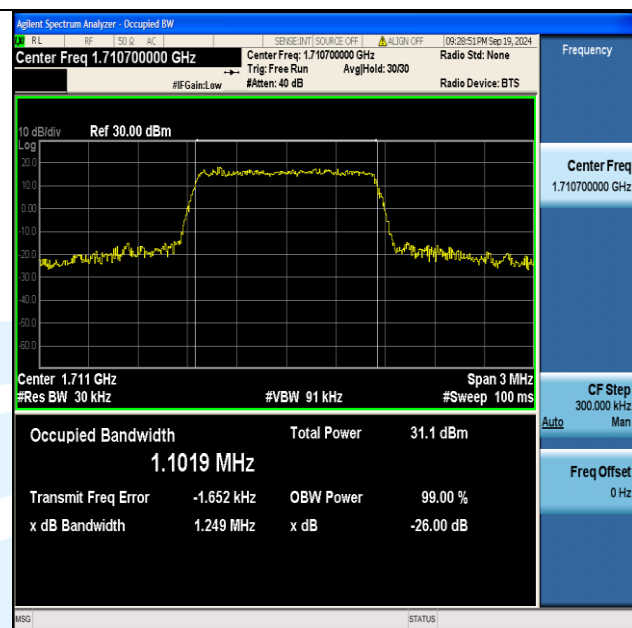
Band4-1.4MHz-16QAM-19957-6RB#0-PASS
