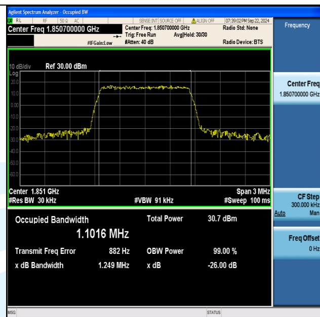
Band2-1.4MHz-16QAM-18607-6RB#0-PASS
