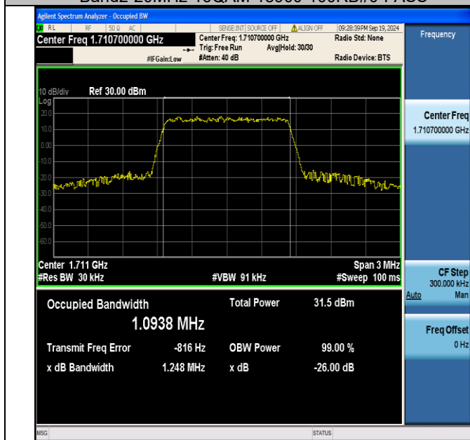
Band4-1.4MHz-QPSK-19957-6RB#0-PASS
