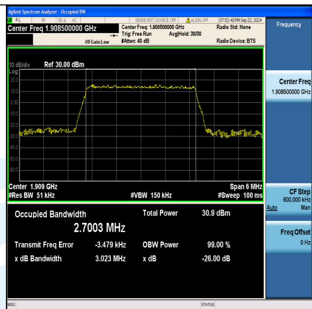
Band2-3MHz-16QAM-19185-15RB#0-PASS
