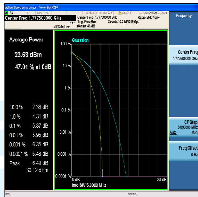
Band66-5MHz-QPSK-132647-25RB#0-PASS
