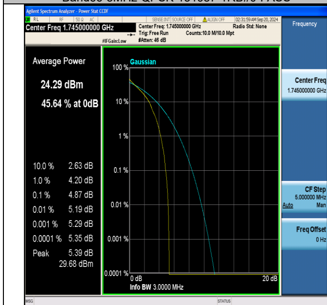
Band66-3MHz-QPSK-132322-1RB#0-PASS
