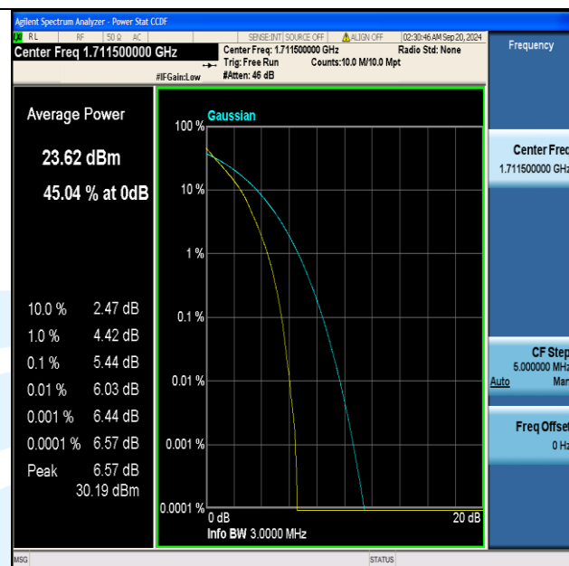
Band66-3MHz-QPSK-131987-15RB#0-PASS
