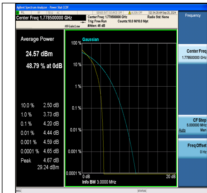
Band66-3MHz-QPSK-132657-1RB#0-PASS
