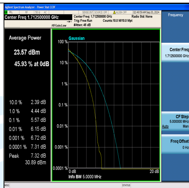
Band66-5MHz-QPSK-131997-25RB#0-PASS
