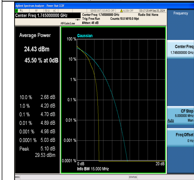
Band66-15MHz-QPSK-132322-1RB#0-PASS
