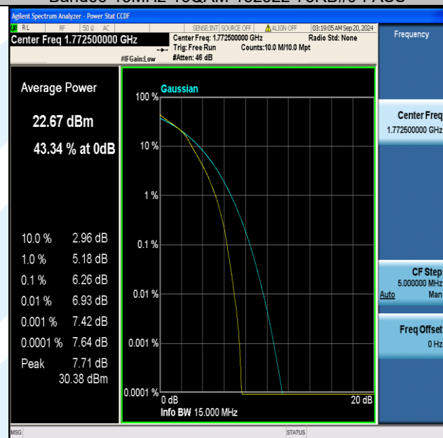
Band66-15MHz-16QAM-132597-75RB#0-PASS
