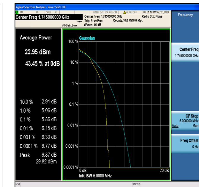
Band66-5MHz-16QAM-132322-1RB#0-PASS
