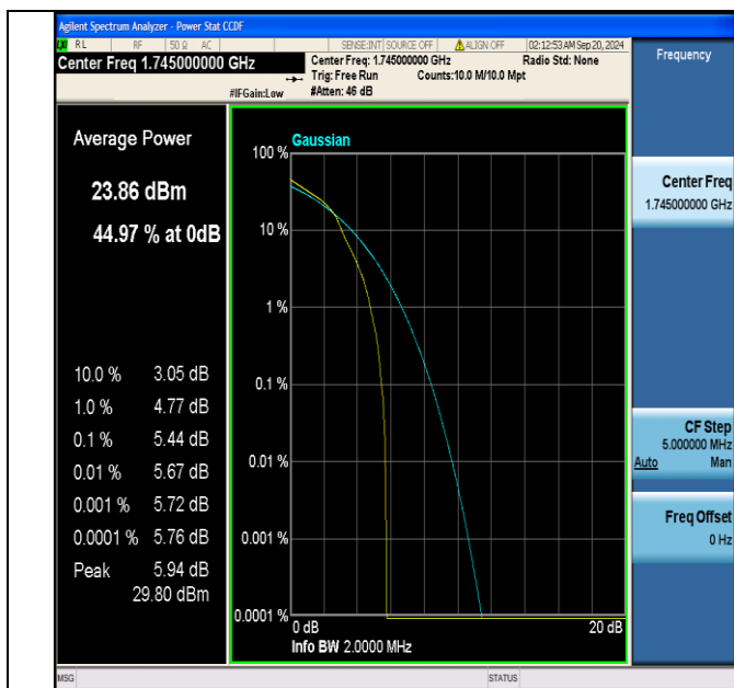
Band66-1.4MHz-16QAM-132322-1RB#0-PASS
