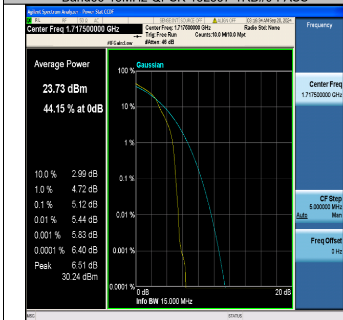
Band66-15MHz-16QAM-132047-1RB#0-PASS
