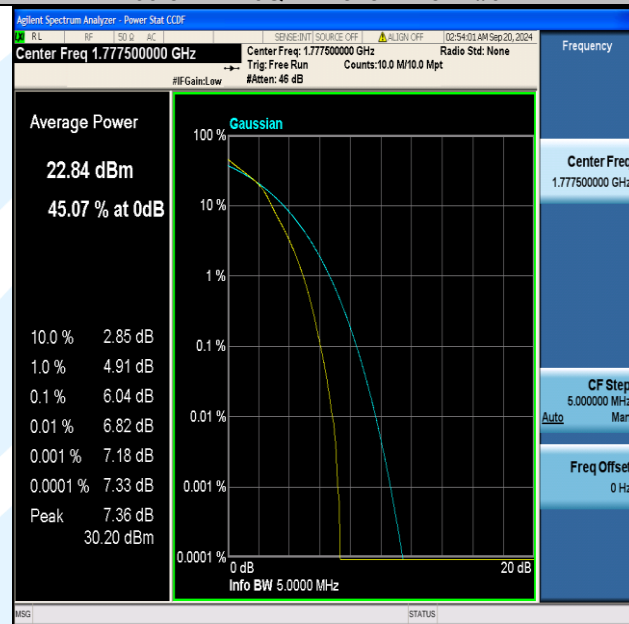
Band66-5MHz-16QAM-132647-25RB#0-PASS
