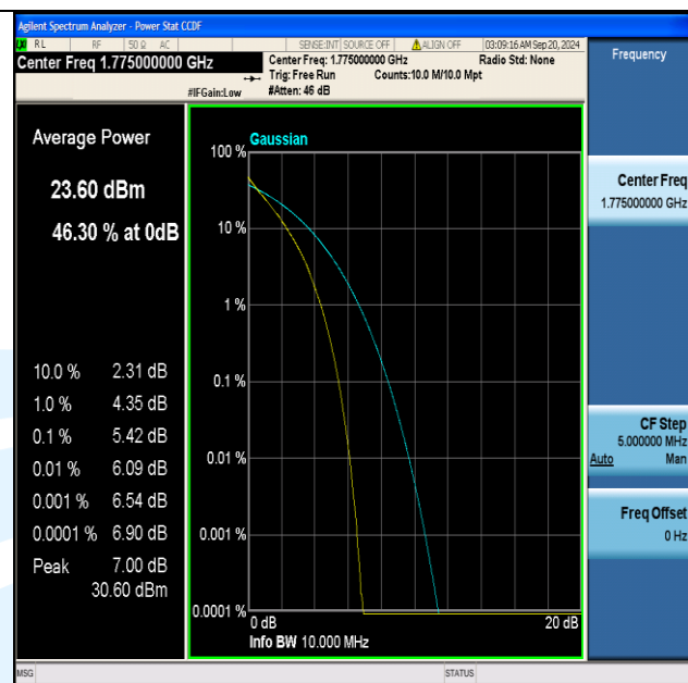
Band66-10MHz-QPSK-132622-50RB#0-PASS
