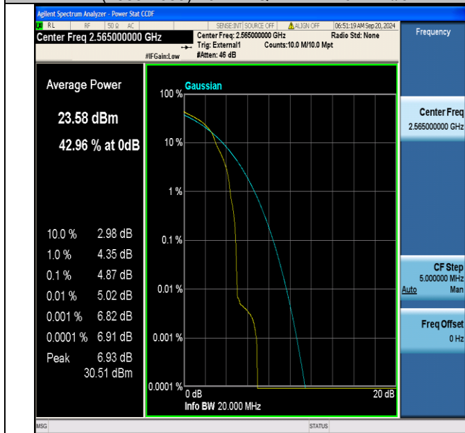
Band41(2555-2655)-20MHz-16QAM-40340-1RB#0-PASS
