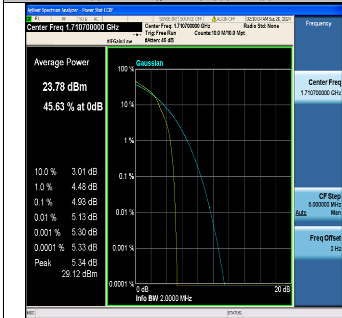
Band66-1.4MHz-16QAM-131979-1RB#0-PASS
