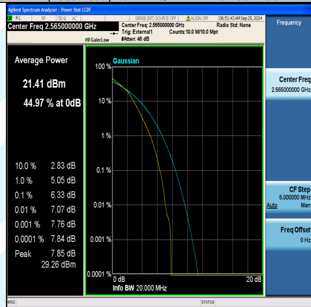
Band41(2555-2655)-20MHz-16QAM-40340-100RB#0-PASS
