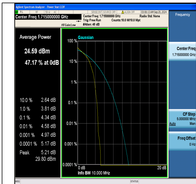
Band66-10MHz-QPSK-132022-1RB#0-PASS
