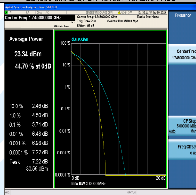
Band66-3MHz-QPSK-132322-15RB#0-PASS
