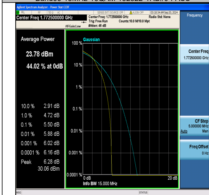
Band66-15MHz-16QAM-132597-1RB#0-PASS
