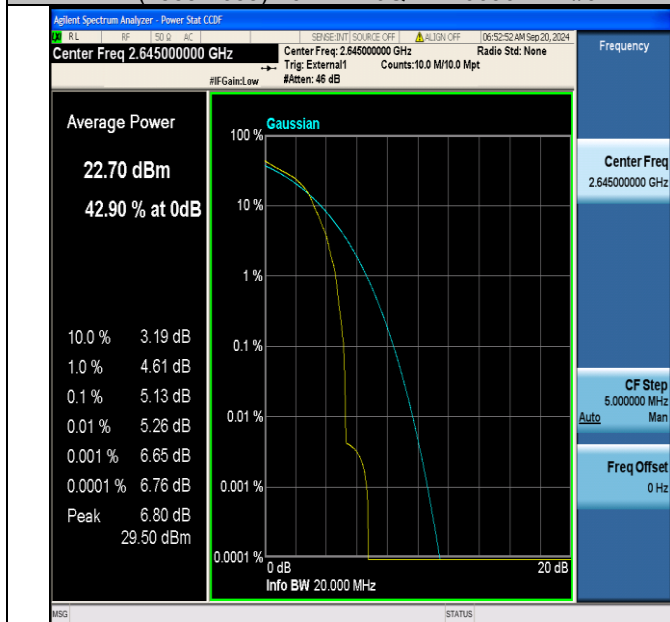
Band41(2555-2655)-20MHz-16QAM-41140-1RB#0-PASS
