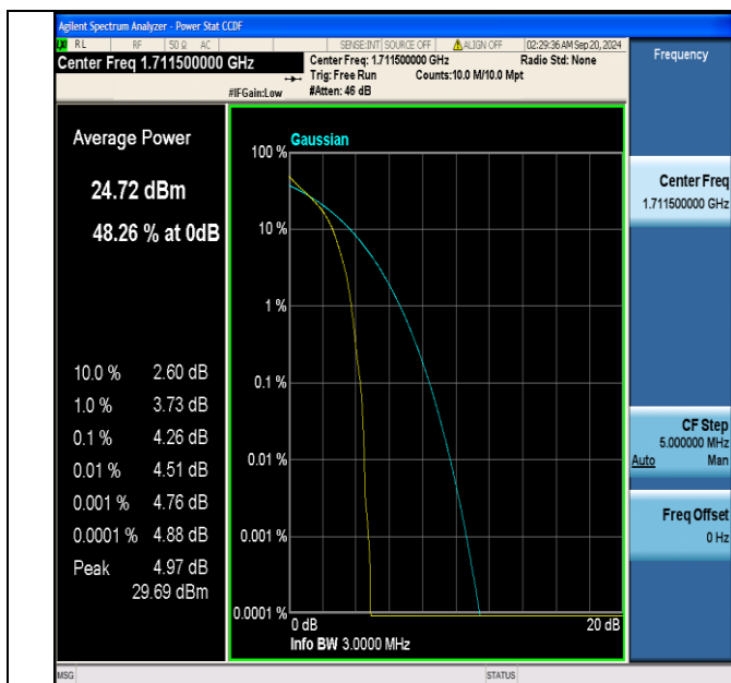
Band66-3MHz-QPSK-131987-1RB#0-PASS
