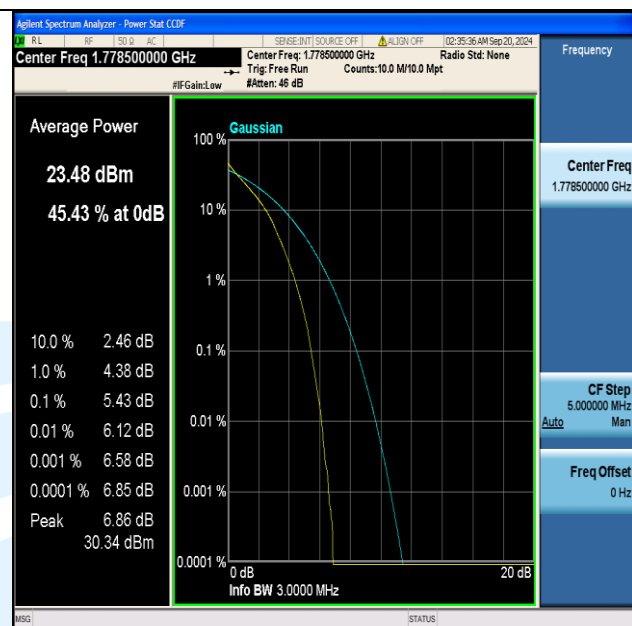
Band66-3MHz-QPSK-132657-15RB#0-PASS
