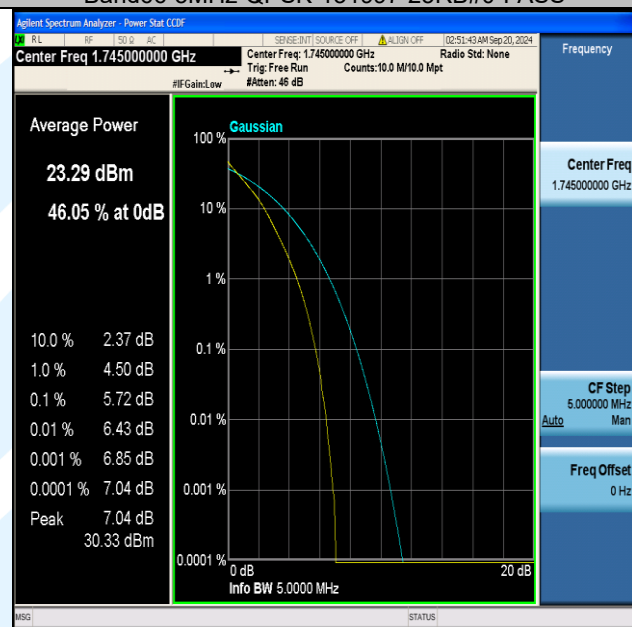
Band66-5MHz-QPSK-132322-25RB#0-PASS
