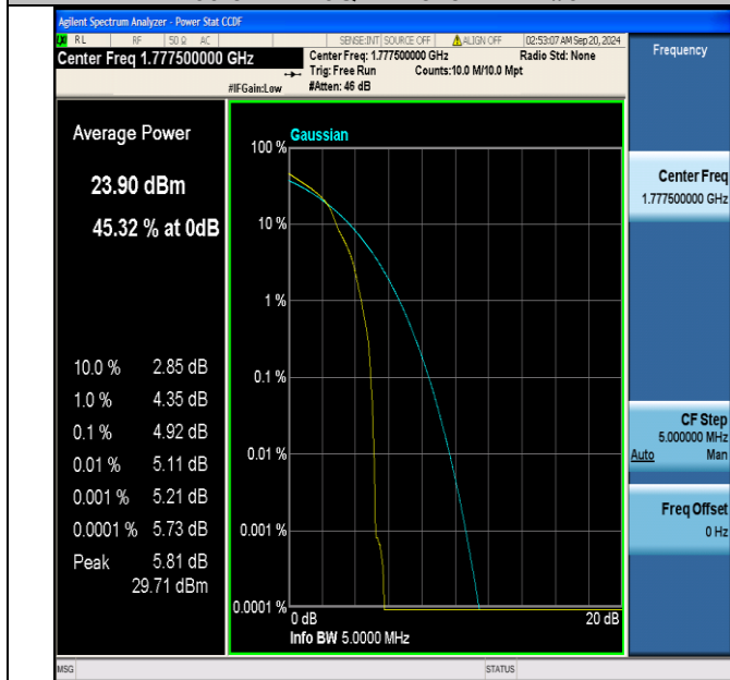
Band66-5MHz-16QAM-132647-1RB#0-PASS
