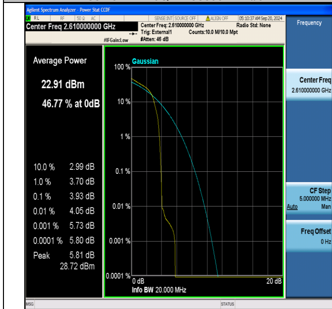
Band38-20MHz-16QAM-38150-1RB#0-PASS
