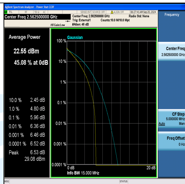
Band41(2555-2655)-15MHz-QPSK-40315-75RB#0-PASS
