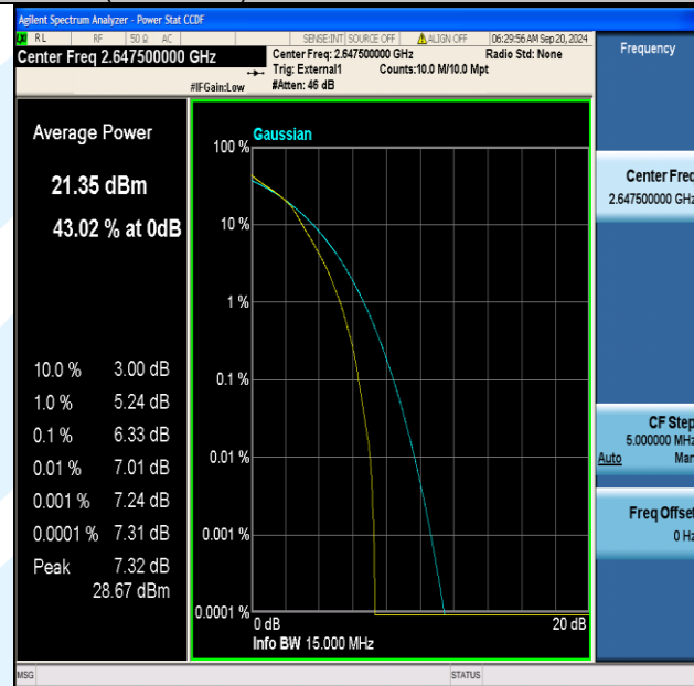
Band41(2555-2655)-15MHz-16QAM-41165-75RB#0-PASS
