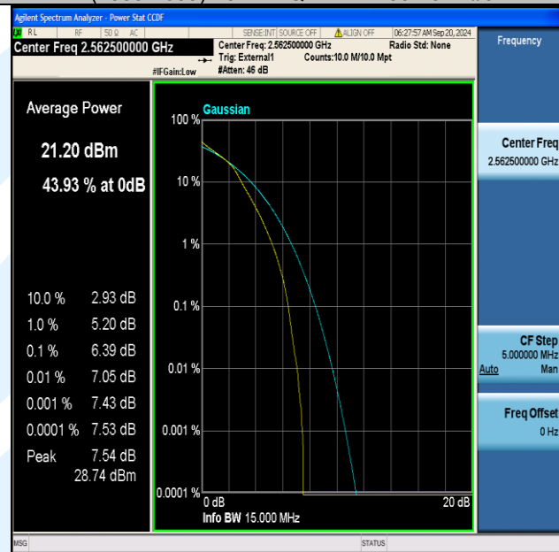
Band41(2555-2655)-15MHz-16QAM-40315-75RB#0-PASS
