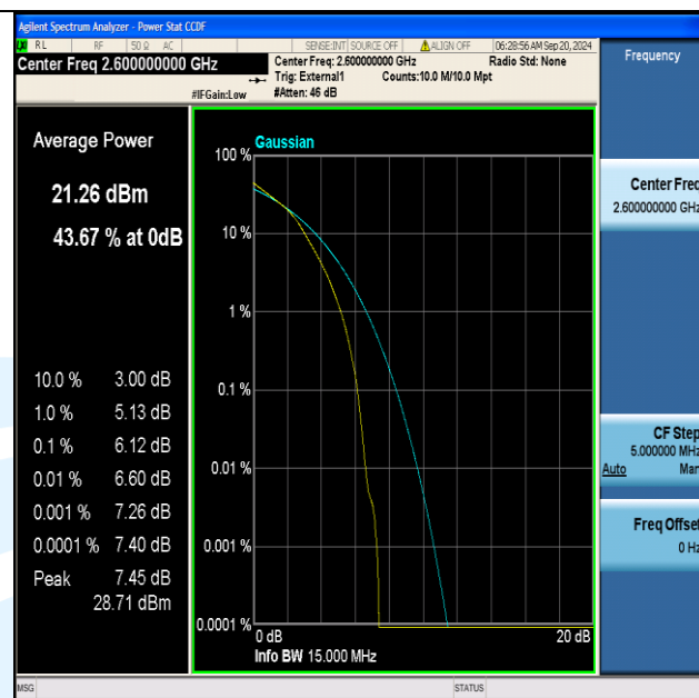
Band41(2555-2655)-15MHz-16QAM-40690-75RB#0-PASS
