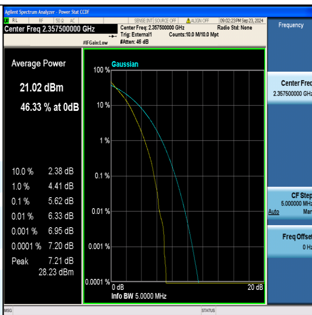
Band40(2350-2360)-5MHz-QPSK-39225-25RB#0-PASS
