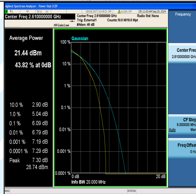
Band38-20MHz-16QAM-38150-100RB#0-PASS
