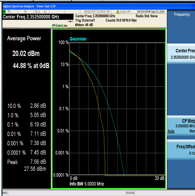
Band40(2350-2360)-5MHz-16QAM-39175-25RB#0-PASS
