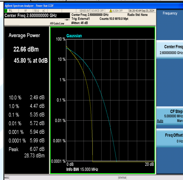
Band41(2555-2655)-15MHz-QPSK-40690-75RB#0-PASS
