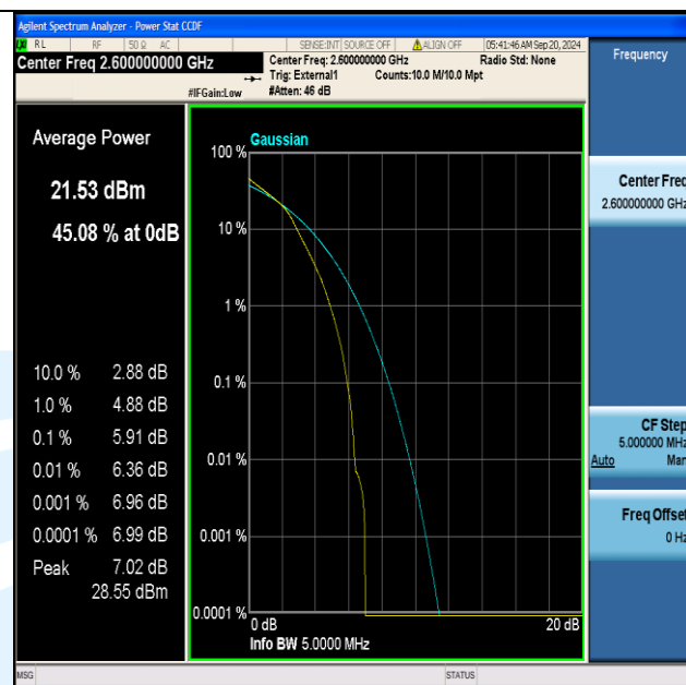
Band41(2555-2655)-5MHz-16QAM-40690-25RB#0-PASS
