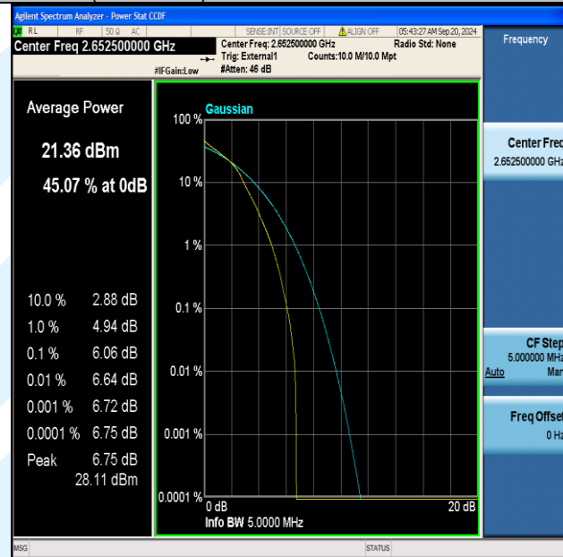
Band41(2555-2655)-5MHz-16QAM-41215-25RB#0-PASS
