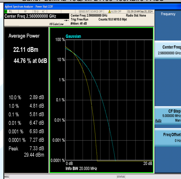
Band7-20MHz-16QAM-21350-100RB#0-PASS
