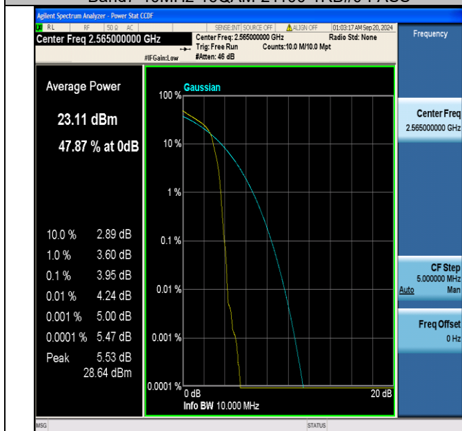
Band7-10MHz-16QAM-21400-1RB#0-PASS
