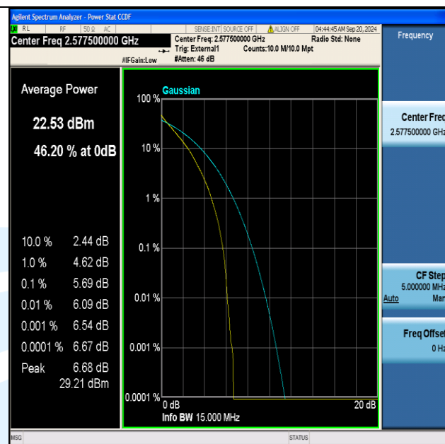
Band38-15MHz-QPSK-37825-75RB#0-PASS
