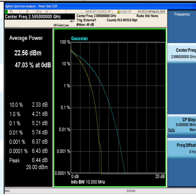
Band38-10MHz-QPSK-38000-50RB#0-PASS
