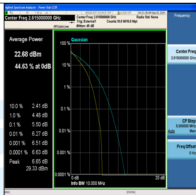
Band38-10MHz-QPSK-38200-50RB#0-PASS
