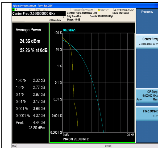
Band7-20MHz-QPSK-21350-1RB#0-PASS
