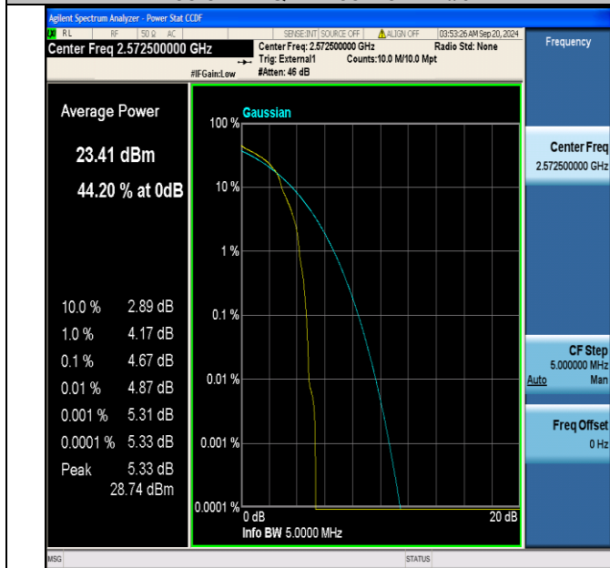
Band38-5MHz-16QAM-37775-1RB#0-PASS
