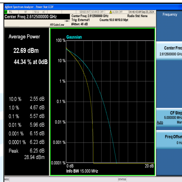
Band38-15MHz-QPSK-38175-75RB#0-PASS
