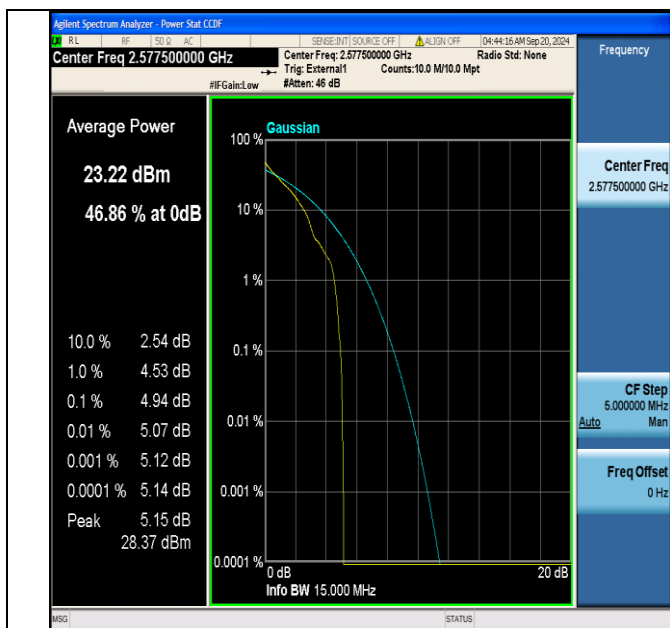
Band38-15MHz-QPSK-37825-1RB#0-PASS
