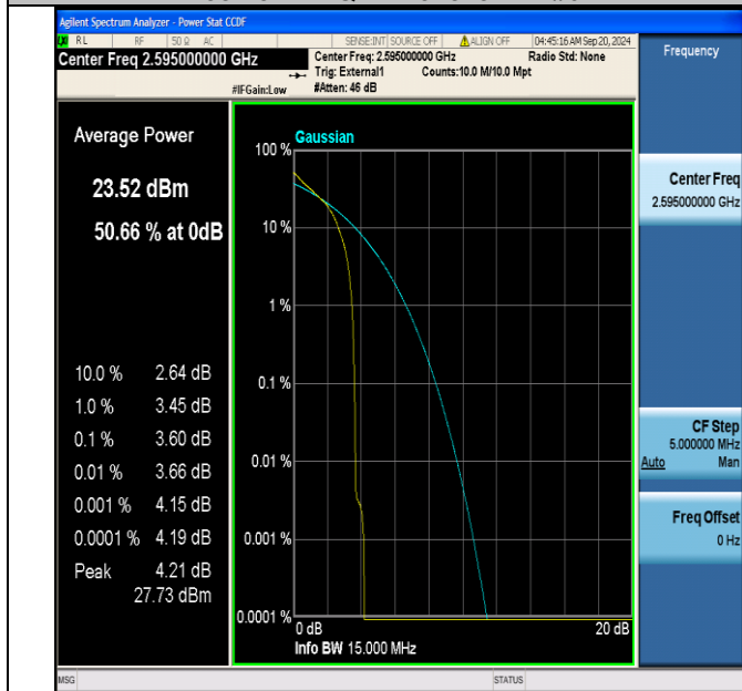
Band38-15MHz-QPSK-38000-1RB#0-PASS
