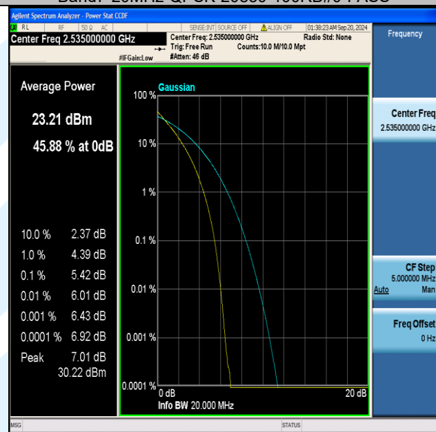
Band7-20MHz-QPSK-21100-100RB#0-PASS
