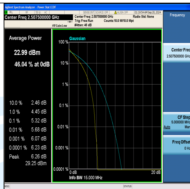
Band7-15MHz-QPSK-20825-75RB#0-PASS
