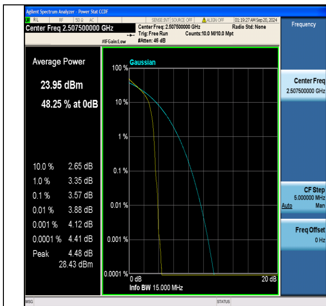
Band7-15MHz-QPSK-20825-1RB#0-PASS
