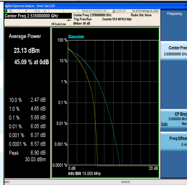
Band7-15MHz-QPSK-21100-75RB#0-PASS
