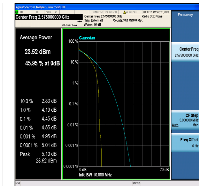
Band38-10MHz-QPSK-37800-1RB#0-PASS
