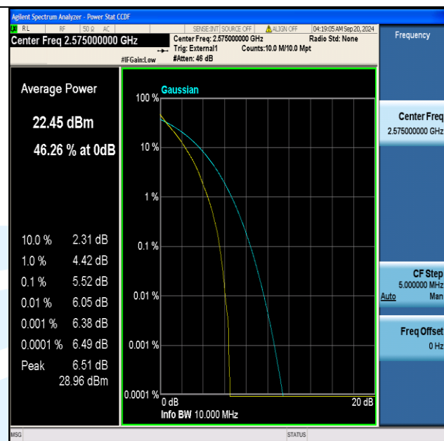
Band38-10MHz-QPSK-37800-50RB#0-PASS
