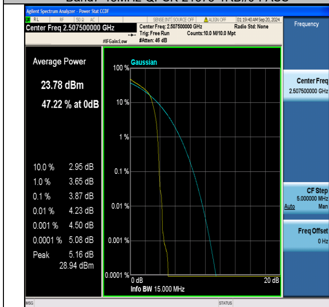
Band7-15MHz-16QAM-20825-1RB#0-PASS
