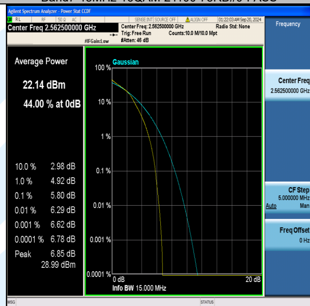
Band7-15MHz-16QAM-21375-75RB#0-PASS
