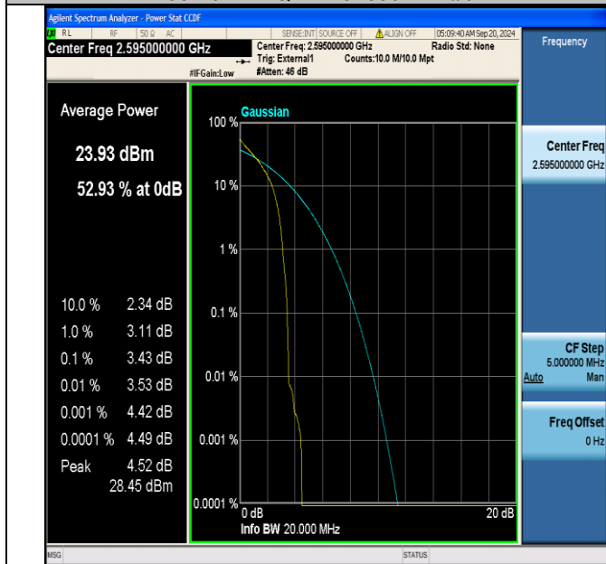
Band38-20MHz-QPSK-38000-1RB#0-PASS
