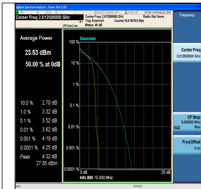
Band38-15MHz-QPSK-38175-1RB#0-PASS
