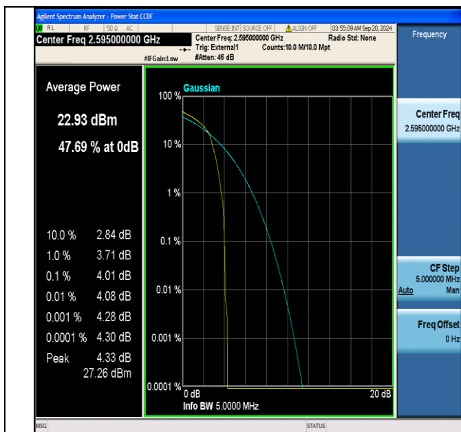
Band38-5MHz-16QAM-38000-1RB#0-PASS
