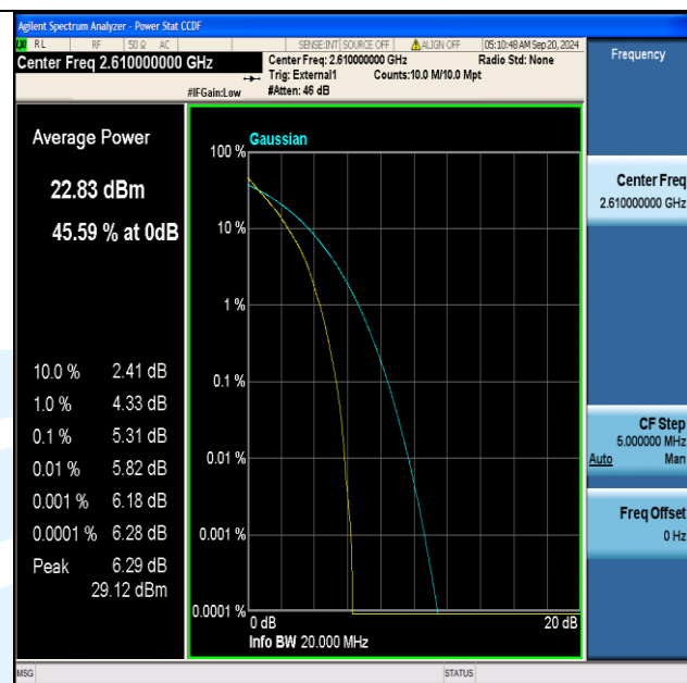
Band38-20MHz-QPSK-38150-100RB#0-PASS
