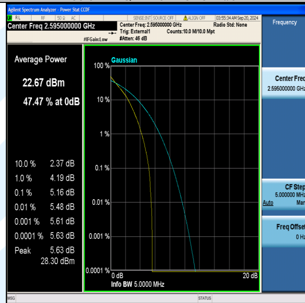
Band38-5MHz-QPSK-38000-25RB#0-PASS
