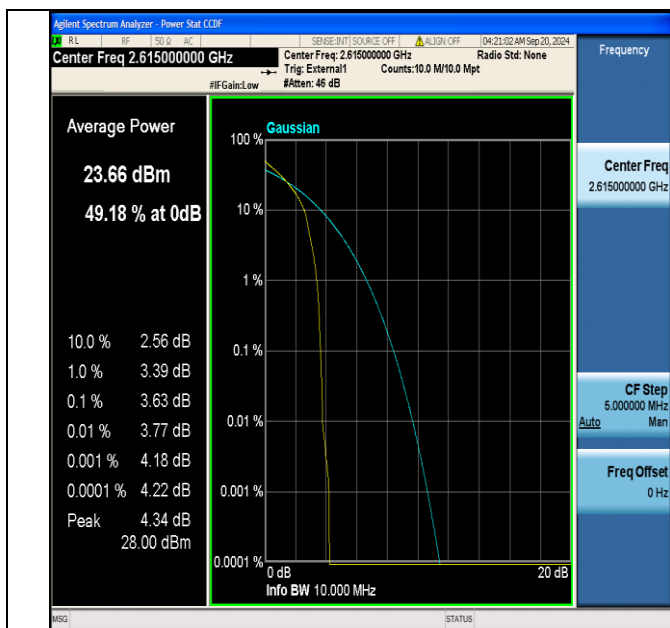
Band38-10MHz-QPSK-38200-1RB#0-PASS
