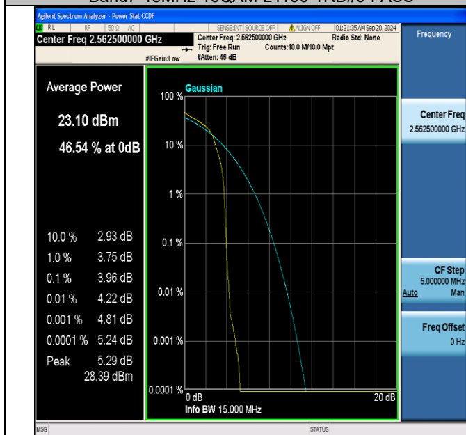
Band7-15MHz-16QAM-21375-1RB#0-PASS
