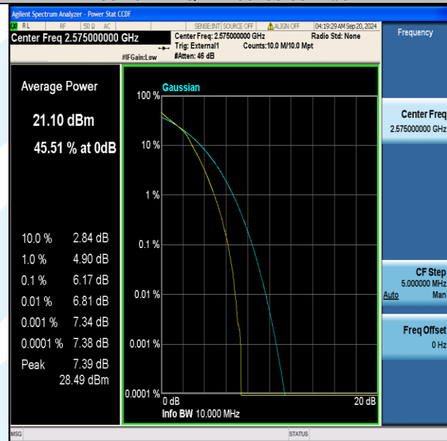
Band38-10MHz-16QAM-37800-50RB#0-PASS
