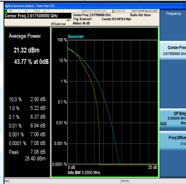
Band38-5MHz-16QAM-38225-25RB#0-PASS
