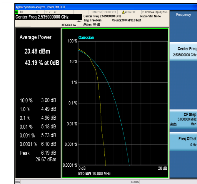
Band7-10MHz-16QAM-21100-1RB#0-PASS
