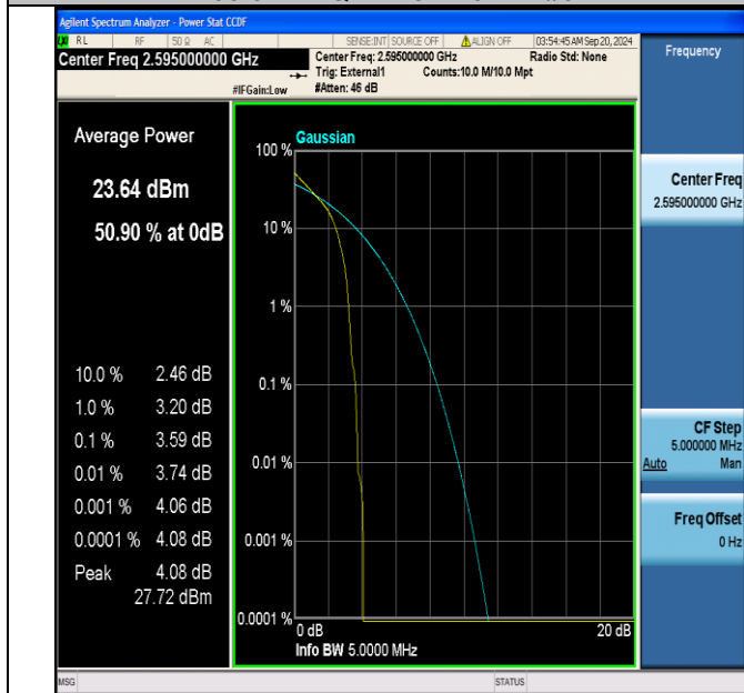
Band38-5MHz-QPSK-38000-1RB#0-PASS
