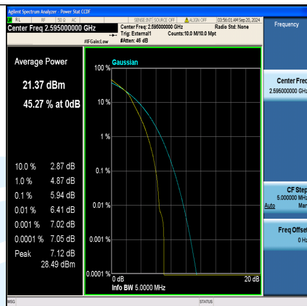
Band38-5MHz-16QAM-38000-25RB#0-PASS
