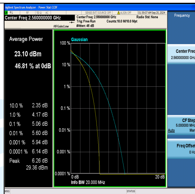
Band7-20MHz-QPSK-21350-100RB#0-PASS
