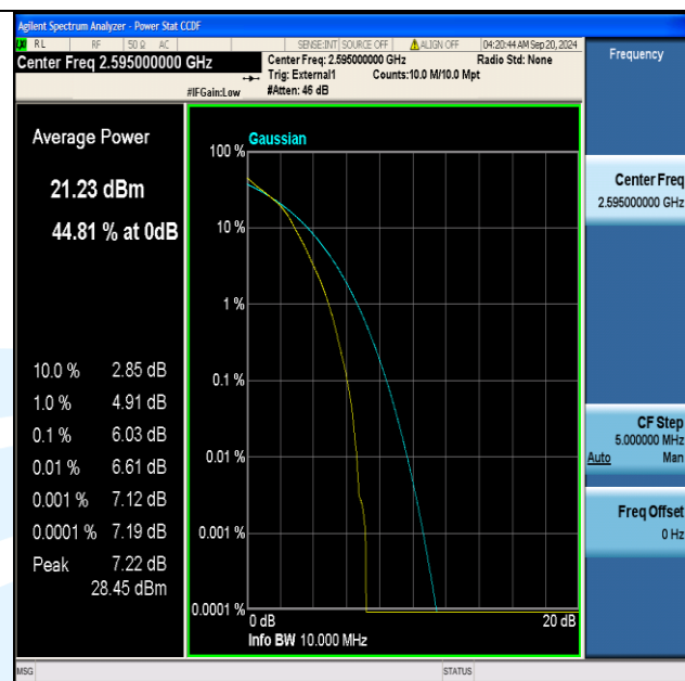
Band38-10MHz-16QAM-38000-50RB#0-PASS
