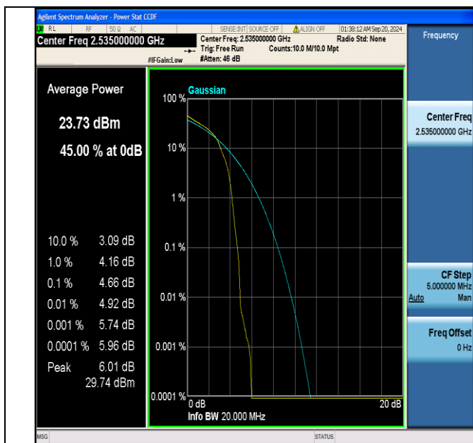
Band7-20MHz-16QAM-21100-1RB#0-PASS
