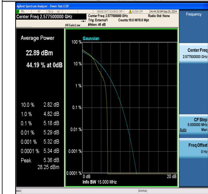
Band38-15MHz-16QAM-37825-1RB#0-PASS
