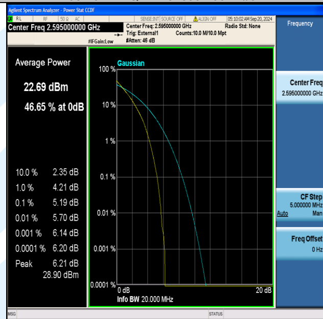
Band38-20MHz-QPSK-38000-100RB#0-PASS
