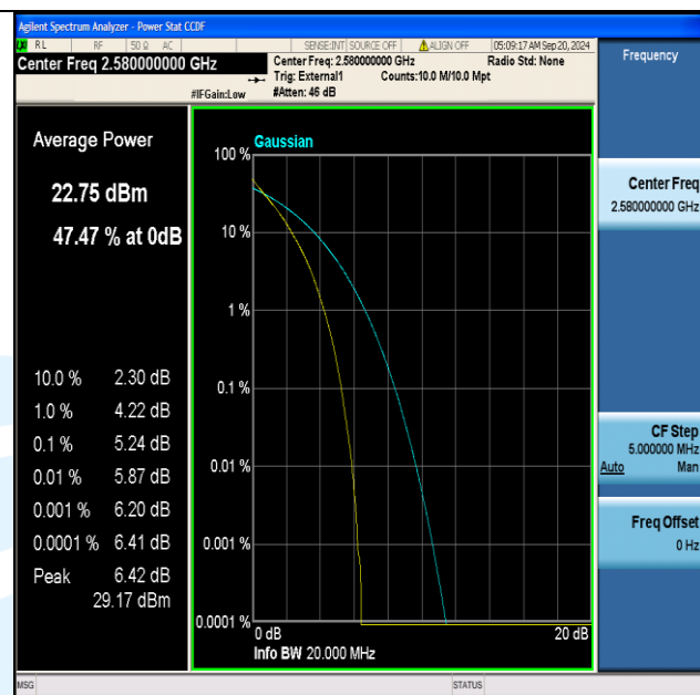
Band38-20MHz-QPSK-37850-100RB#0-PASS
