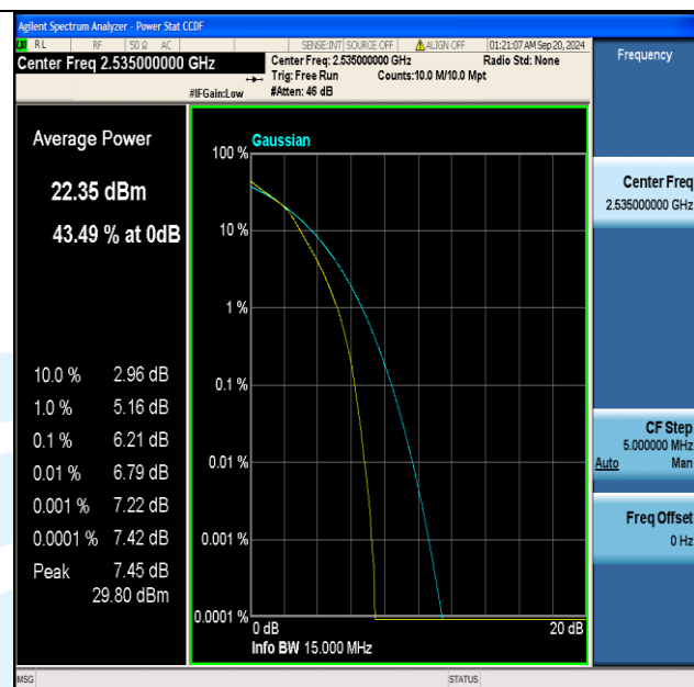
Band7-15MHz-16QAM-21100-75RB#0-PASS
