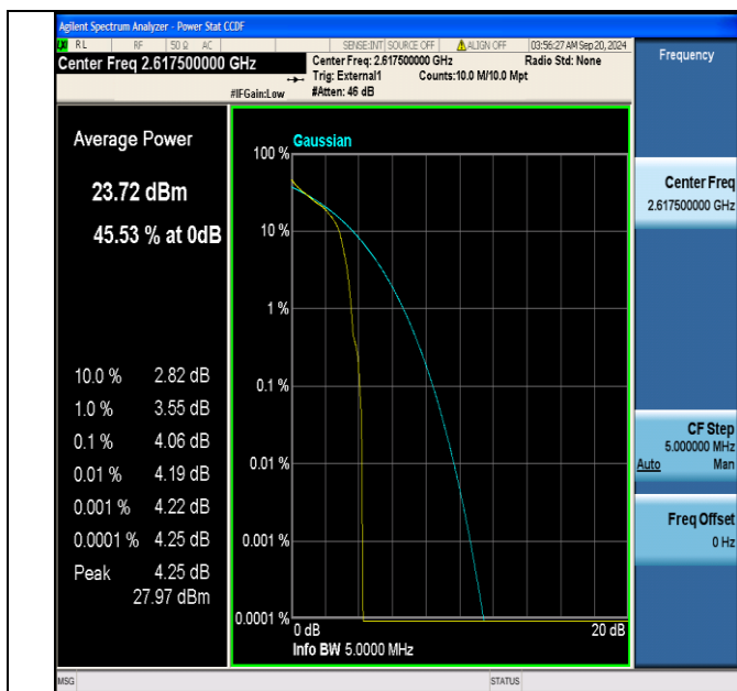
Band38-5MHz-QPSK-38225-1RB#0-PASS
