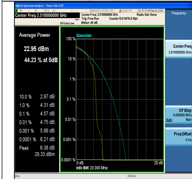
Band7-20MHz-16QAM-20850-1RB#0-PASS
