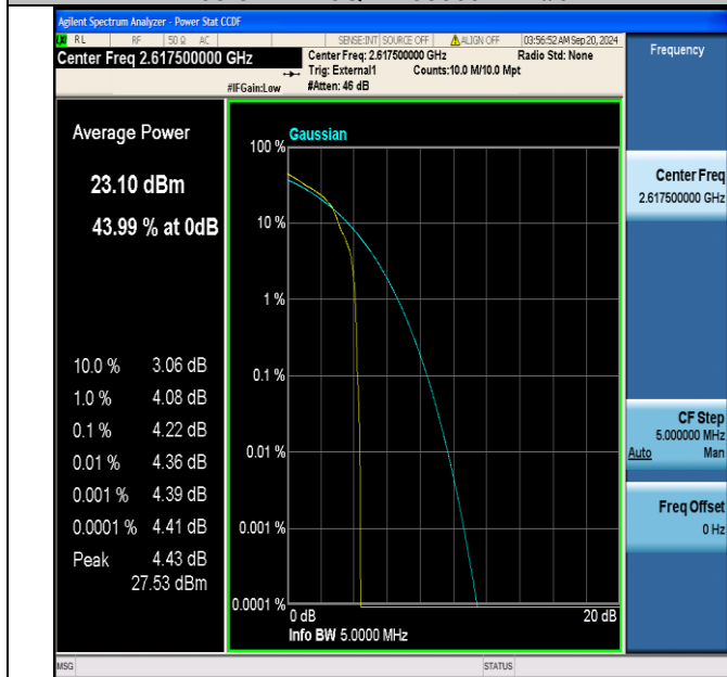
Band38-5MHz-16QAM-38225-1RB#0-PASS
