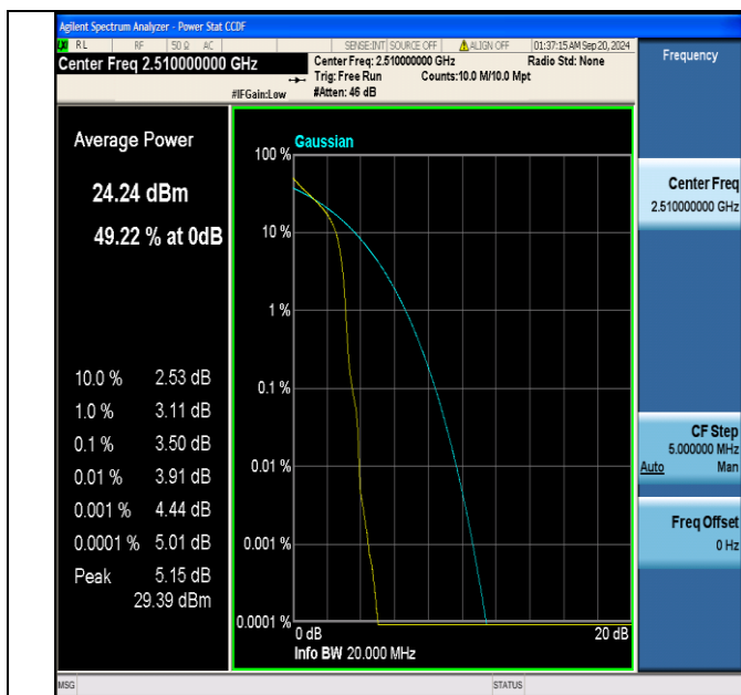
Band7-20MHz-QPSK-20850-1RB#0-PASS
