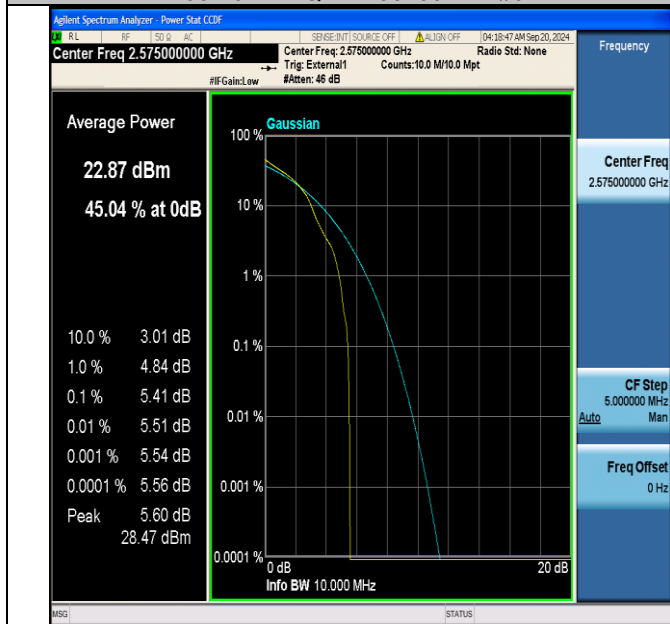
Band38-10MHz-16QAM-37800-1RB#0-PASS
