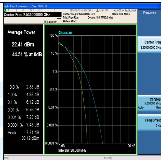
Band7-20MHz-16QAM-21100-100RB#0-PASS
