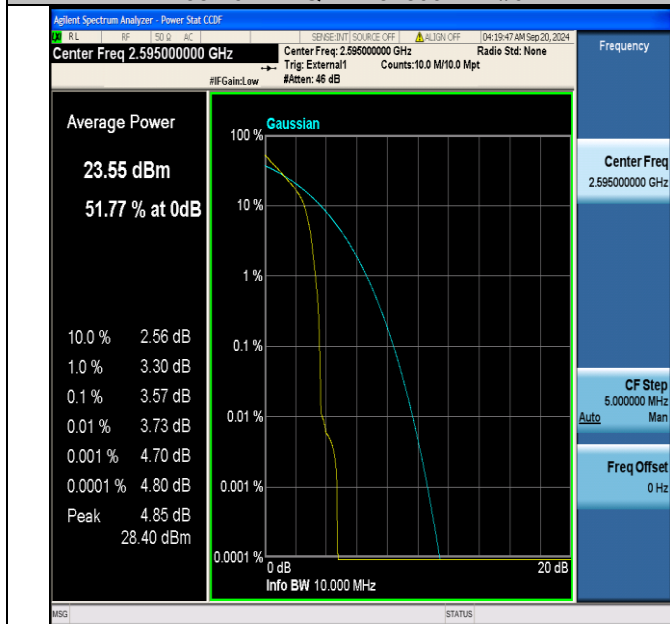
Band38-10MHz-QPSK-38000-1RB#0-PASS
