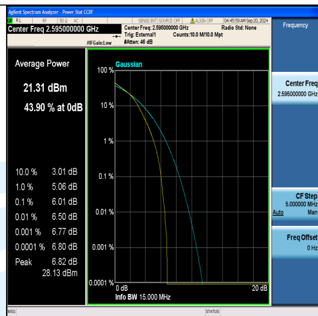
Band38-15MHz-16QAM-38000-75RB#0-PASS
