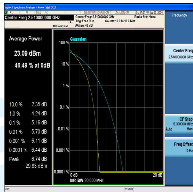
Band7-20MHz-QPSK-20850-100RB#0-PASS
