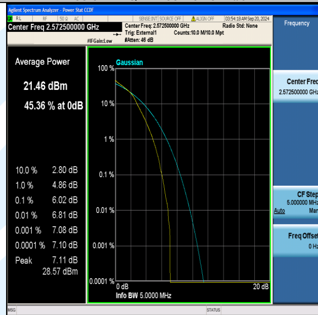
Band38-5MHz-16QAM-37775-25RB#0-PASS
