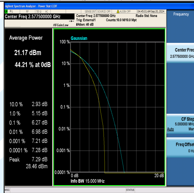
Band38-15MHz-16QAM-37825-75RB#0-PASS
