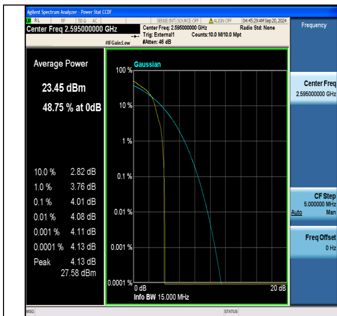
Band38-15MHz-16QAM-38000-1RB#0-PASS
