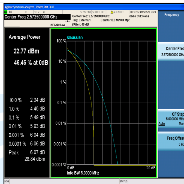
Band38-5MHz-QPSK-37775-25RB#0-PASS
