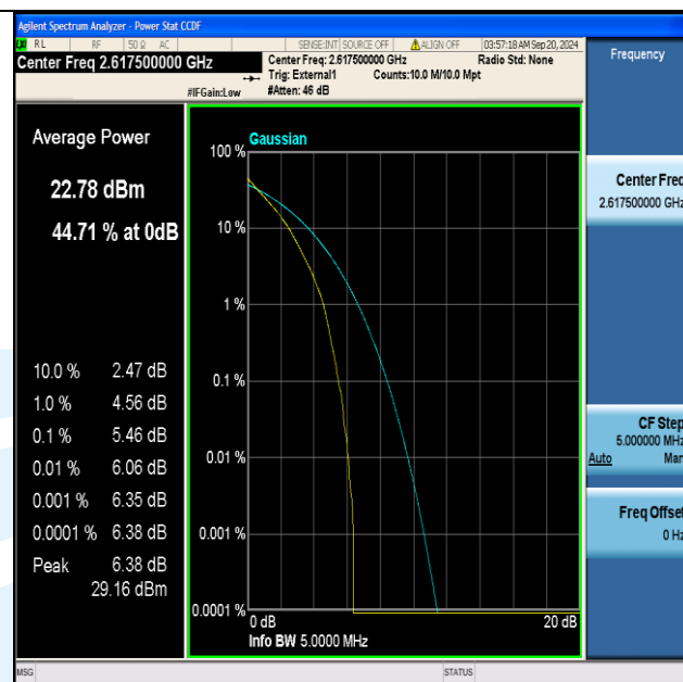
Band38-5MHz-QPSK-38225-25RB#0-PASS
