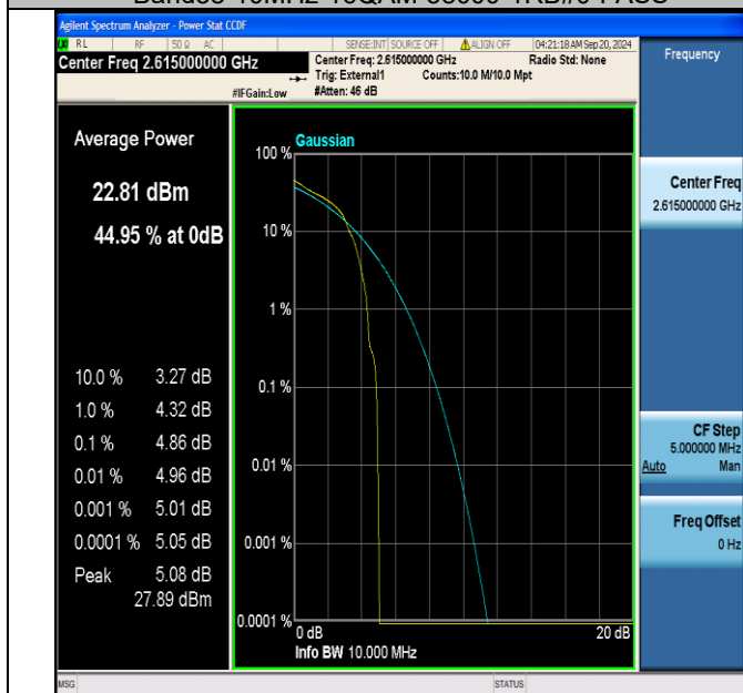
Band38-10MHz-16QAM-38200-1RB#0-PASS
