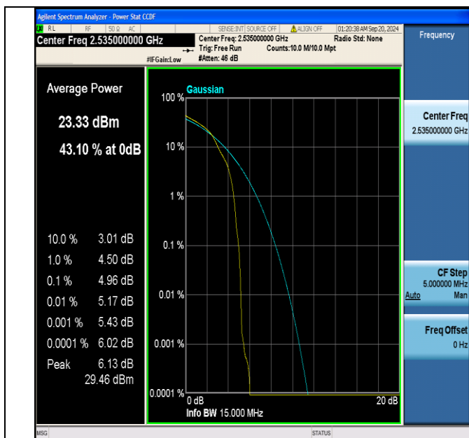
Band7-15MHz-16QAM-21100-1RB#0-PASS
