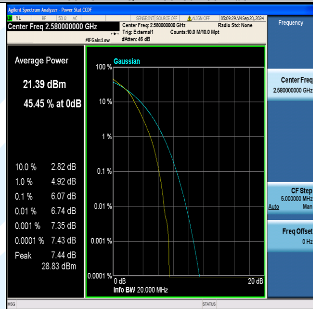
Band38-20MHz-16QAM-37850-100RB#0-PASS
