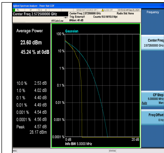
Band38-5MHz-QPSK-37775-1RB#0-PASS
