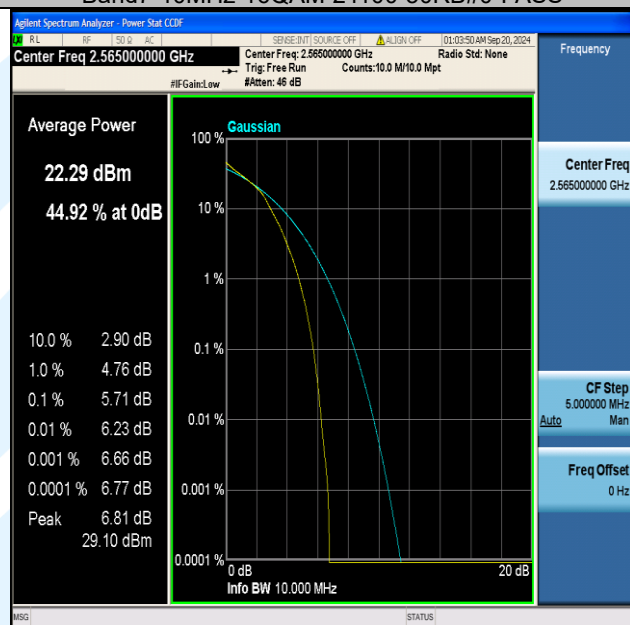
Band7-10MHz-16QAM-21400-50RB#0-PASS
