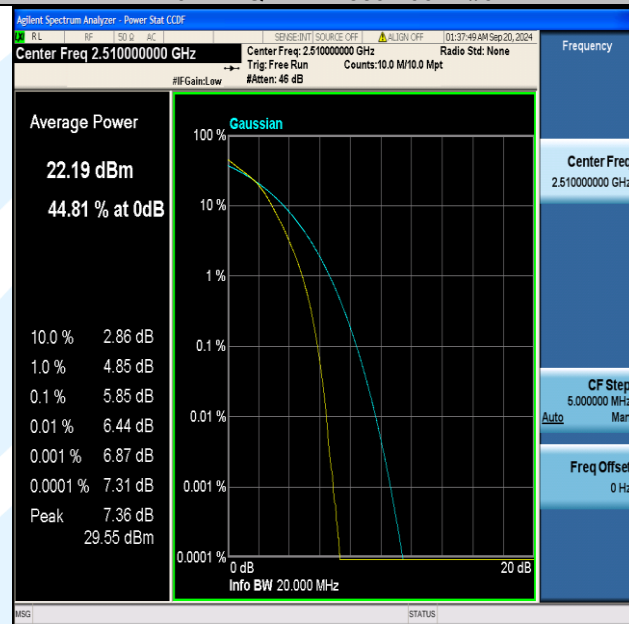
Band7-20MHz-16QAM-20850-100RB#0-PASS
