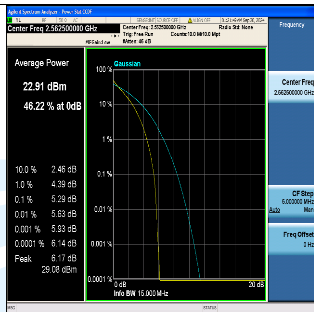
Band7-15MHz-QPSK-21375-75RB#0-PASS
