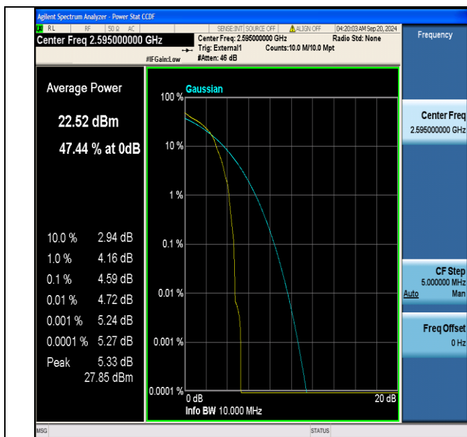
Band38-10MHz-16QAM-38000-1RB#0-PASS
