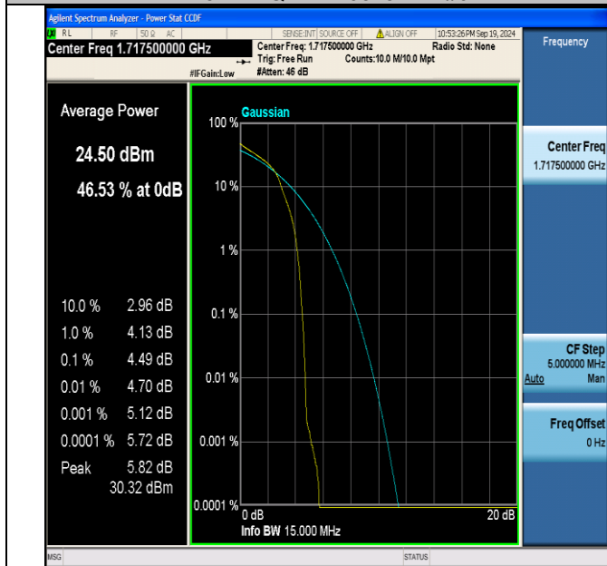
Band4-15MHz-16QAM-20025-1RB#0-PASS
