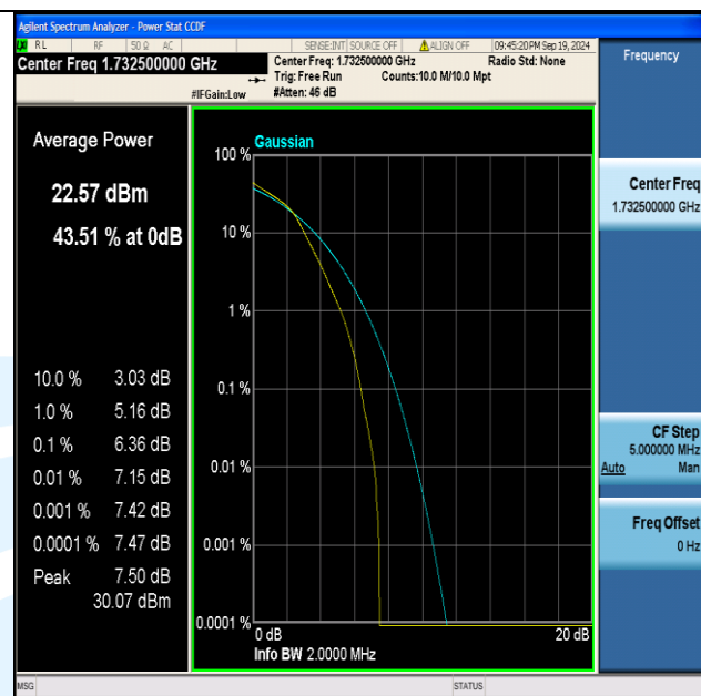
Band4-1.4MHz-16QAM-20175-6RB#0-PASS
