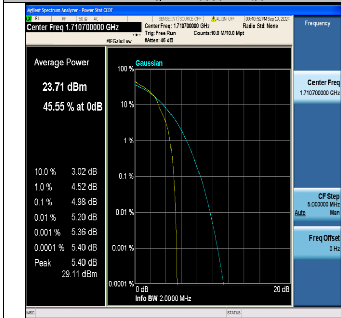
Band4-1.4MHz-16QAM-19957-1RB#0-PASS
