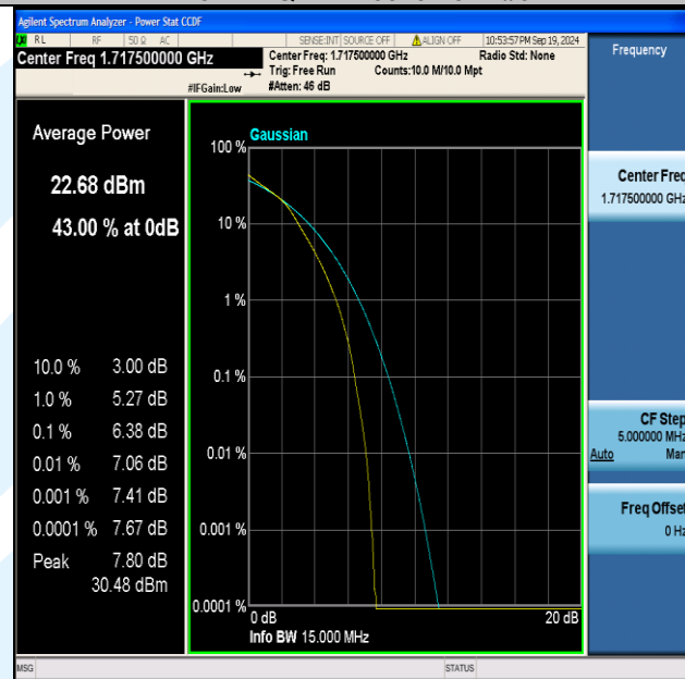
Band4-15MHz-16QAM-20025-75RB#0-PASS
