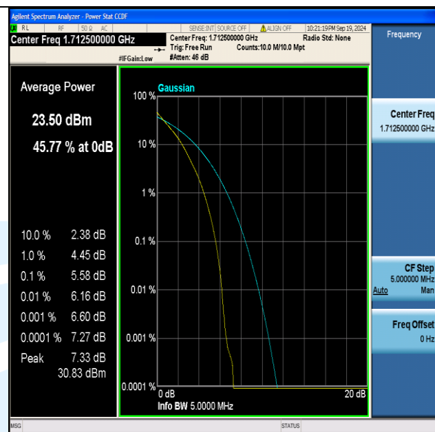
Band4-5MHz-QPSK-19975-25RB#0-PASS
