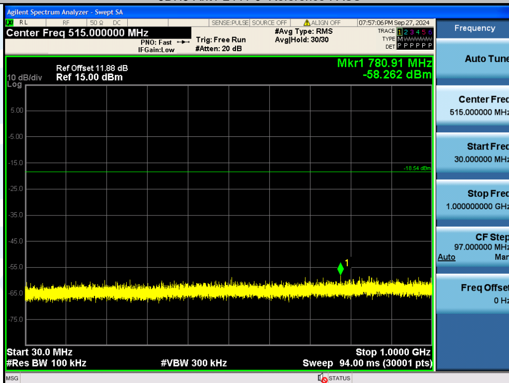
3DH5-Ant1-2441-30~1000-PASS
