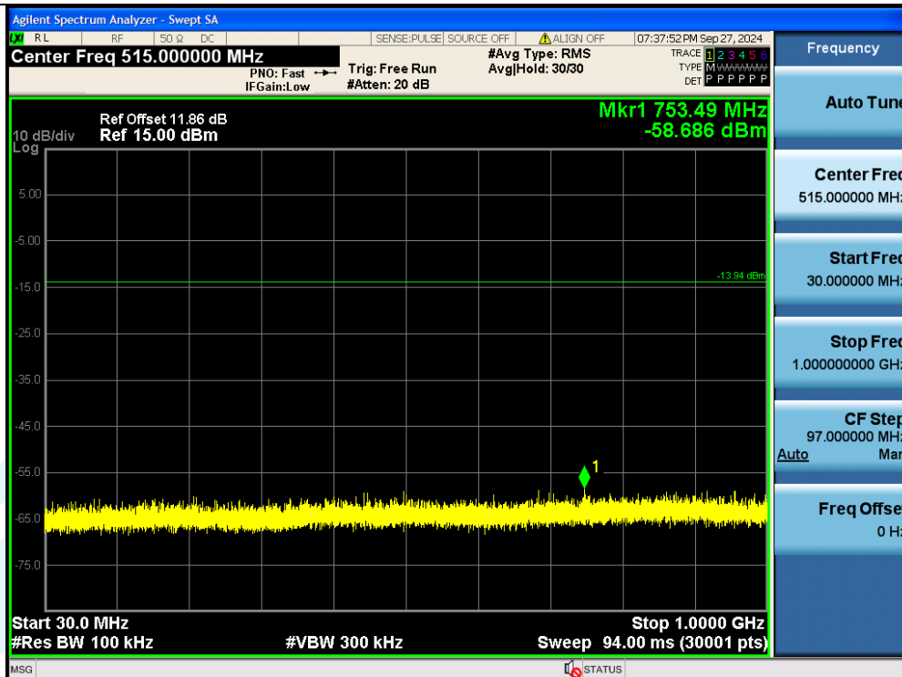
DH5-Ant1-2402-30~1000-PASS
