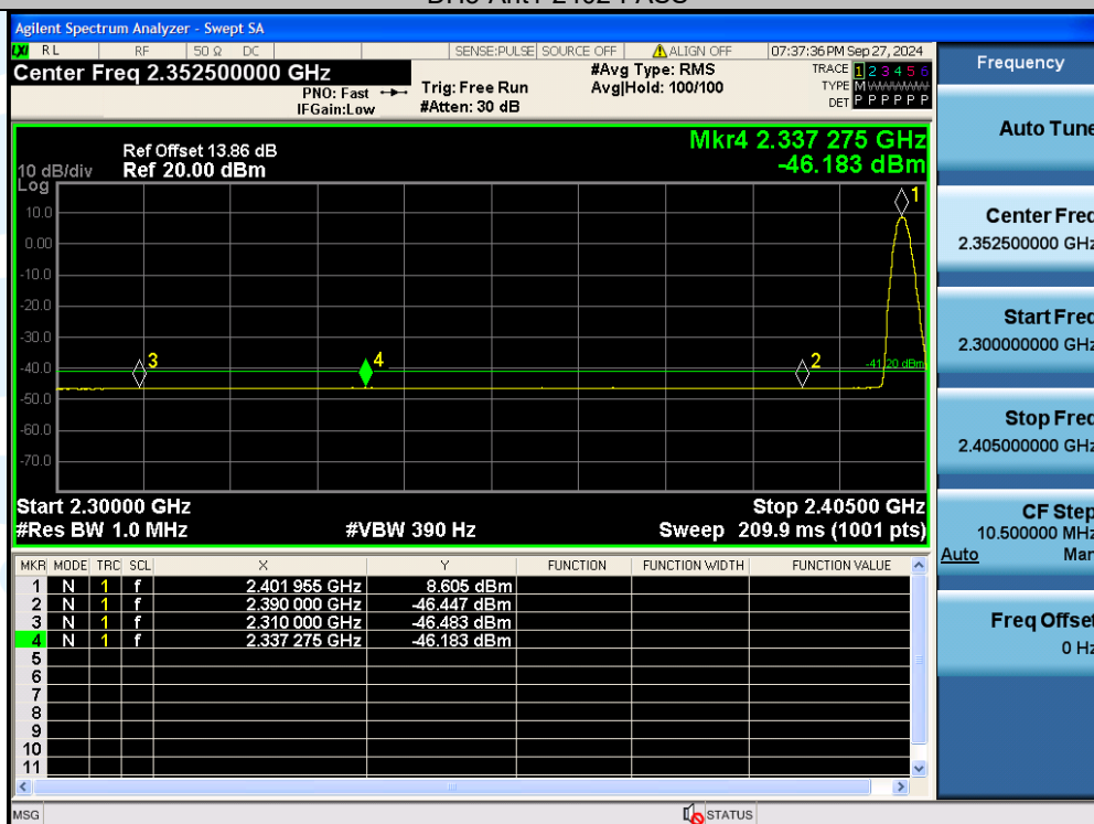
DH5-Ant1-2402-PASS
