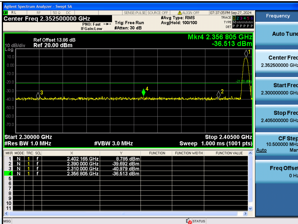
DH5-Ant1-2402-PASS
