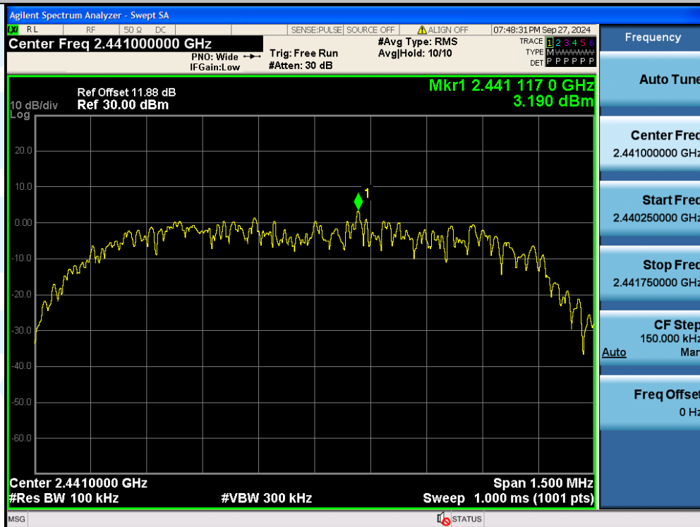
2DH5-Ant1-2441-0~Reference-PASS
