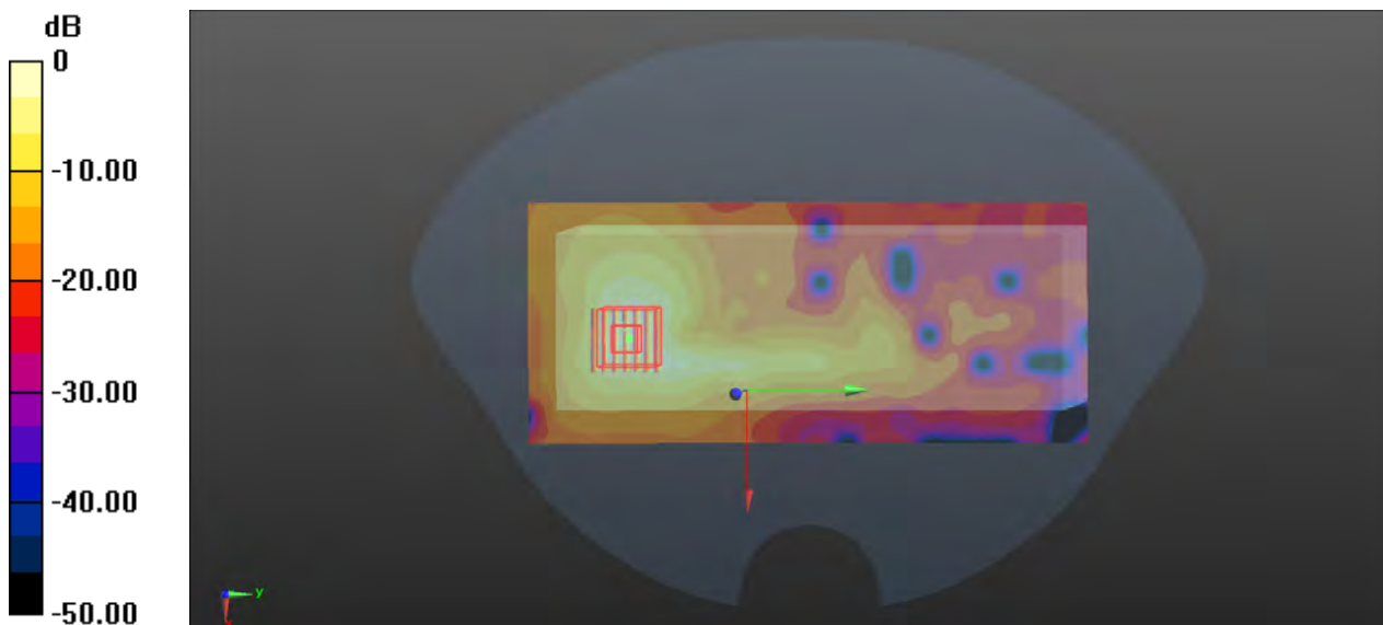
0 dB = 1.73 W/kg
