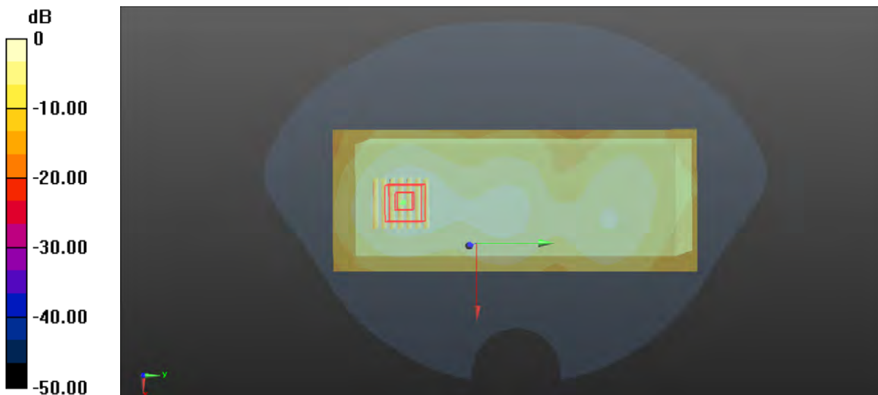
0 dB = 0.135 W/kg
