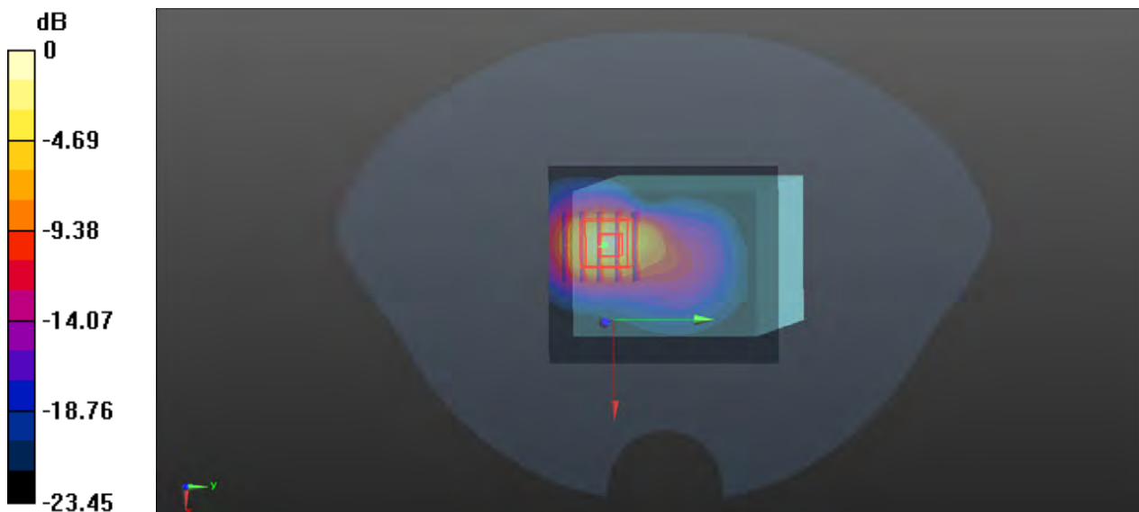
0 dB = 8.96 W/kg
