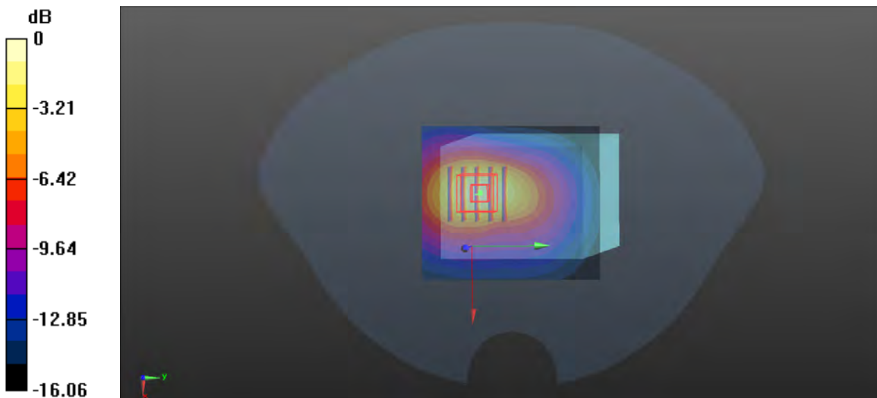
0 dB = 1.29 W/kg
