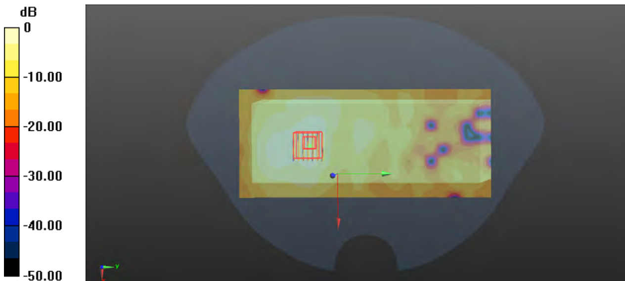
0 dB = 0.522 W/kg
