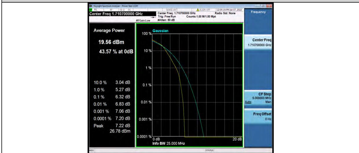
Band4-1.4MHz-16QAM-20175-1RB#0
