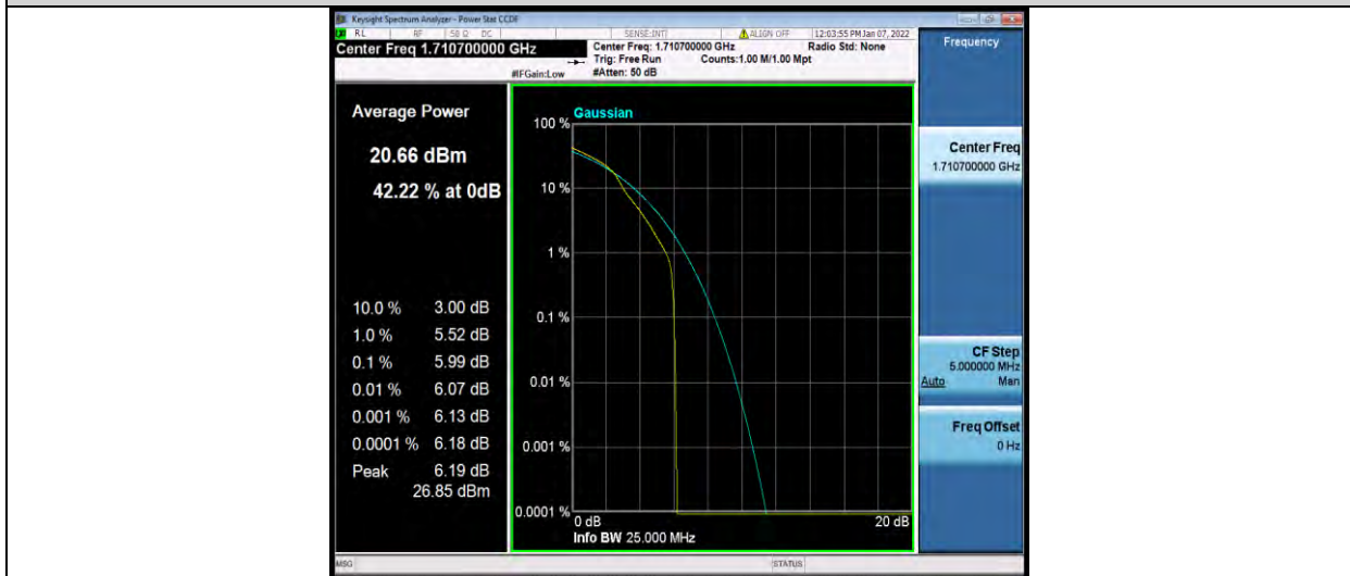
Band4-1.4MHz-16QAM-19957-6RB#0
