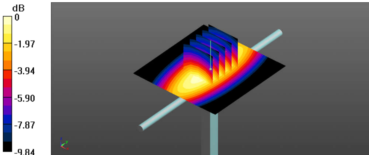
0 dB = 2.79 W/kg
