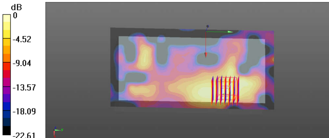
0 dB = 0.0335 W/kg
