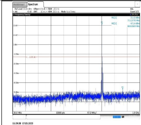
Band12-10MHz-QPSK-23060-1RB#0- Range1:30~1000MHz
