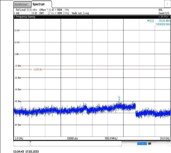
Band17-10MHz-QPSK-23790-1RB#0-Range2:1000~10000MHz
