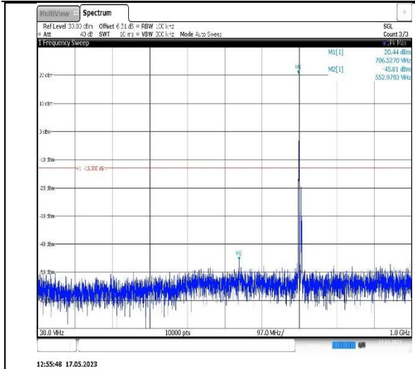
Band17-10MHz-16QAM-23780-1RB#0- Range1:30~1000MHz
