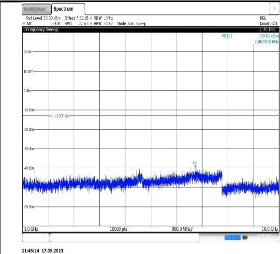
Band13-5MHz-QPSK-23205-1RB#0-Range2:1000~10000MHz
