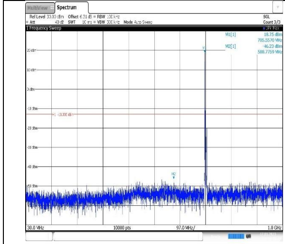
Band17-10MHz-16QAM-23800-1RB#0- Range1:30~1000MHz
