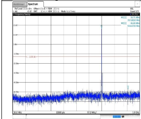
Band17-5MHz-16QAM-23790-1RB#0- Range1:30~1000MHz
