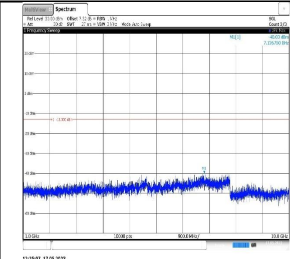
Band17-10MHz-QPSK-23780-1RB#0-Range2:1000~10000MHz
