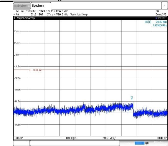
Band17-5MHz-QPSK-23825-1RB#0-Range2:1000~10000MHz
