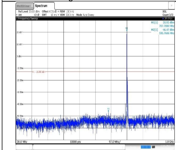
Band17-5MHz-QPSK-23825-1RB#0-Range1:30~1000MHz
