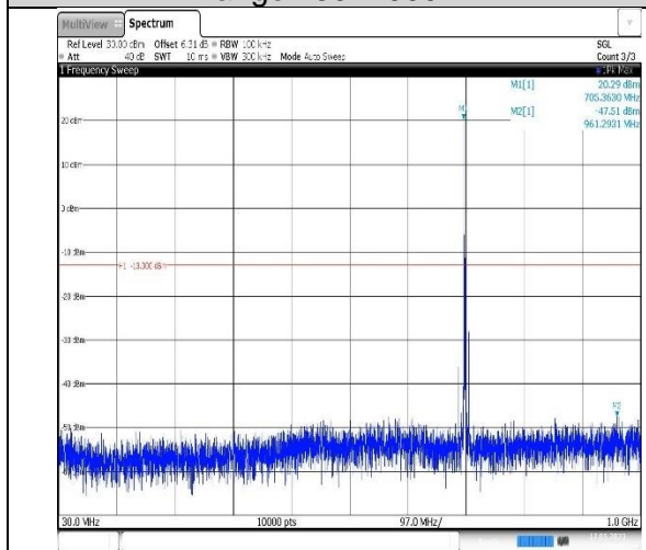
Band12-5MHz-QPSK-23155-1RB#0- Range1:30~1000MHz
