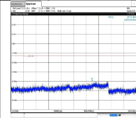
Band12-10MHz-QPSK-23060-1RB#0- Range2:1000~10000MHz
