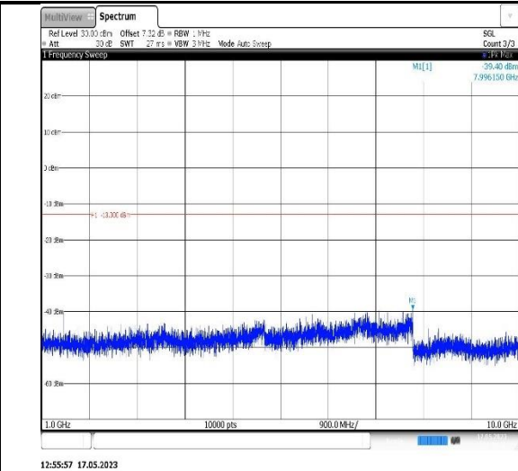
Band17-10MHz-16QAM-23780-1RB#0- Range2:1000~10000MHz
