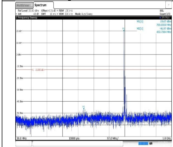
Band12-10MHz-QPSK-23095-1RB#0- Range1:30~1000MHz
