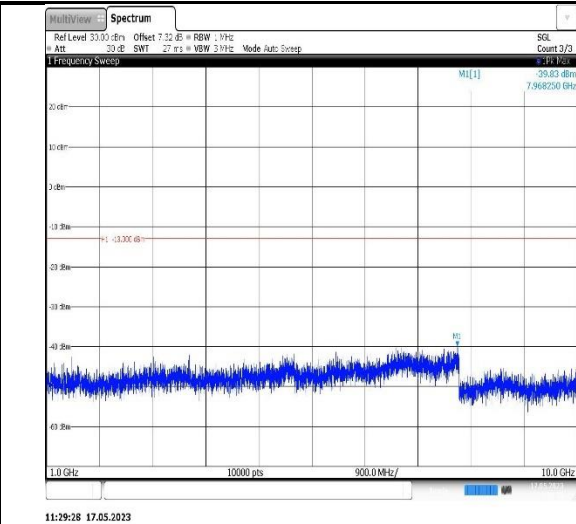
Band12-5MHz-16QAM-23035-1RB#0- Range2:1000~10000MHz
