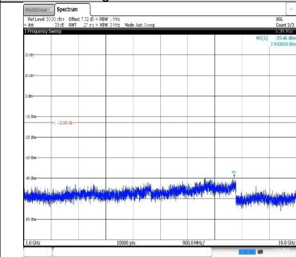
Band12-5MHz-QPSK-23035-1RB#0- Range2:1000~10000MHz
