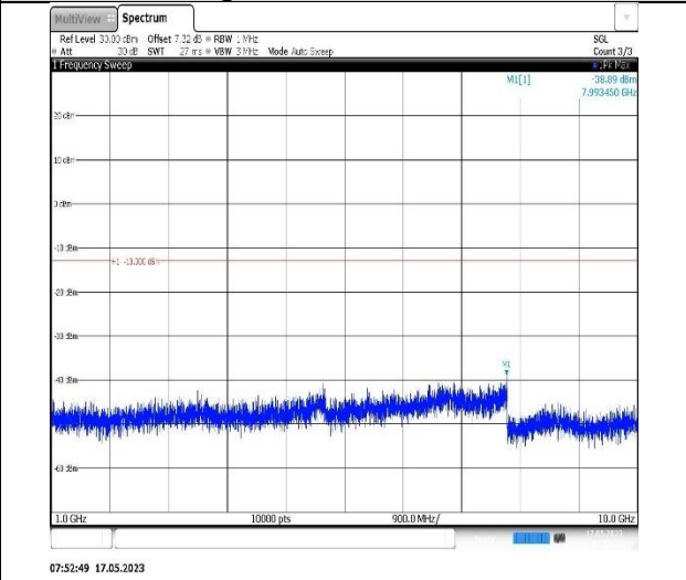
Band12-3MHz-QPSK-23095-1RB#0-Range2:1000~10000MHz
