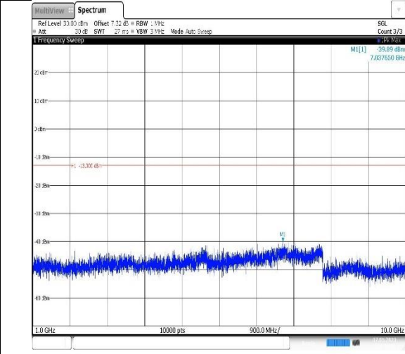
Band17-10MHz-16QAM-23790-1RB#0- Range2:1000~10000MHz
