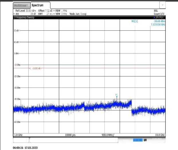
Band12-3MHz-QPSK-23025-1RB#0-Range2:1000~10000MHz
