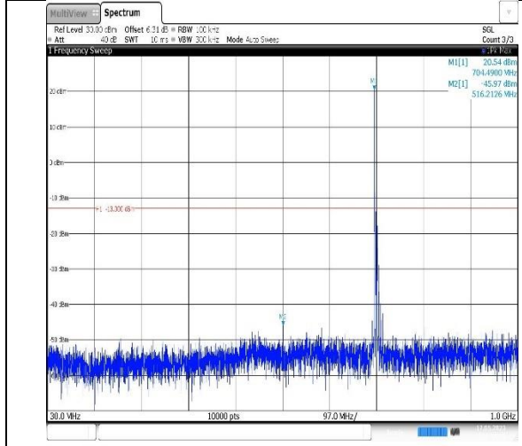
Band17-10MHz-16QAM-23790-1RB#0- Range1:30~1000MHz
