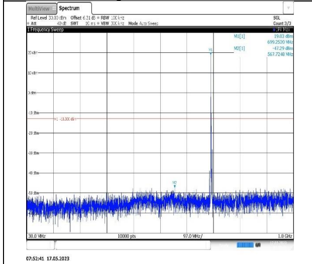
Band12-3MHz-QPSK-23095-1RB#0-Range1:30~1000MHz
