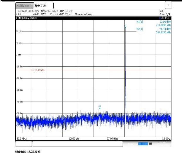
Band12-3MHz-QPSK-23025-1RB#0-Range1:30~1000MHz
