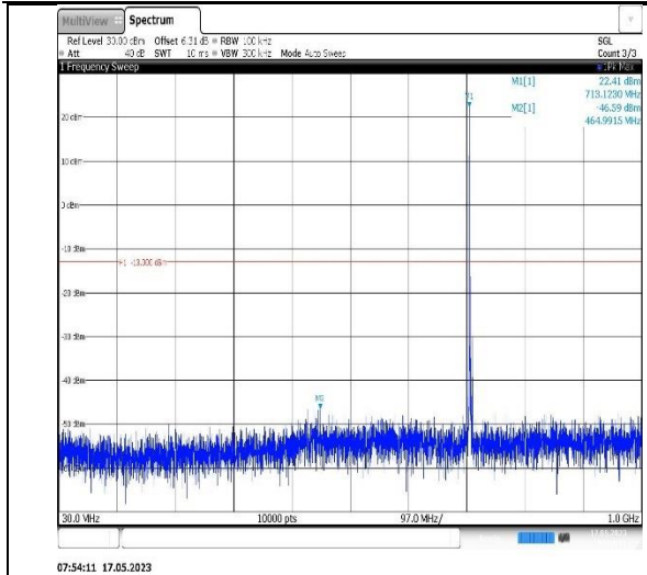
Band12-5MHz-QPSK-23035-1RB#0- Range1:30~1000MHz
