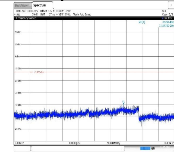
Band12-10MHz-QPSK-23095-1RB#0- Range2:1000~10000MHz
