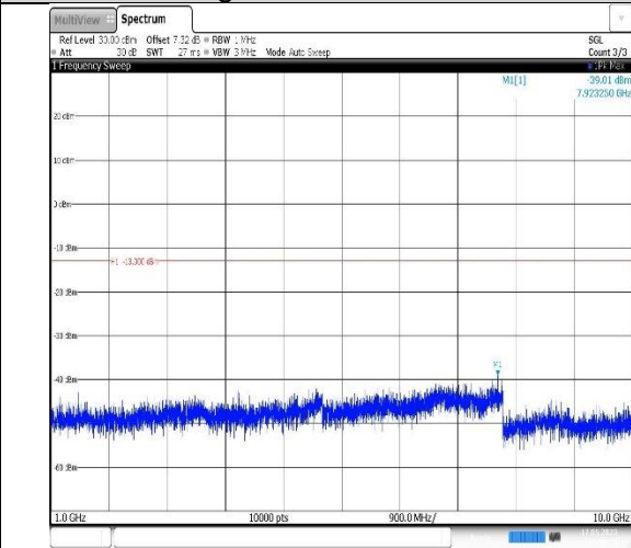
Band17-5MHz-16QAM-23790-1RB#0- Range2:1000~10000MHz
