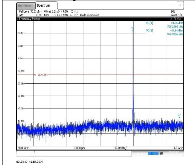
Band12-3MHz-QPSK-23165-1RB#0-Range1:30~1000MHz
