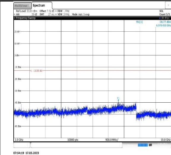
Band12-5MHz-QPSK-23035-1RB#0- Range2:1000~10000MHz
