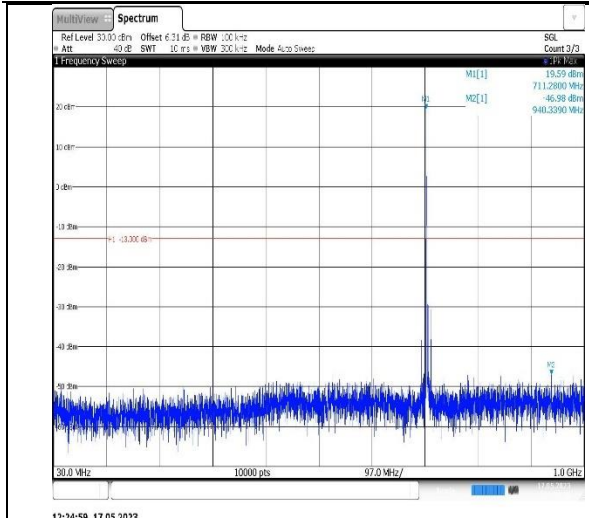
Band17-10MHz-QPSK-23780-1RB#0-Range1:30~1000MHz
