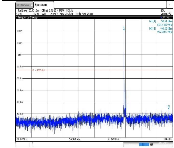
Band12-10MHz-QPSK-23060-1RB#0- Range1:30~1000MHz
