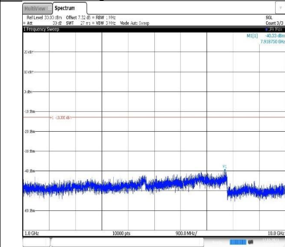
Band17-5MHz-16QAM-23755-1RB#0- Range2:1000~10000MHz
