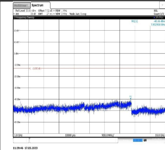
Band12-10MHz-QPSK-23060-1RB#0- Range2:1000~10000MHz
