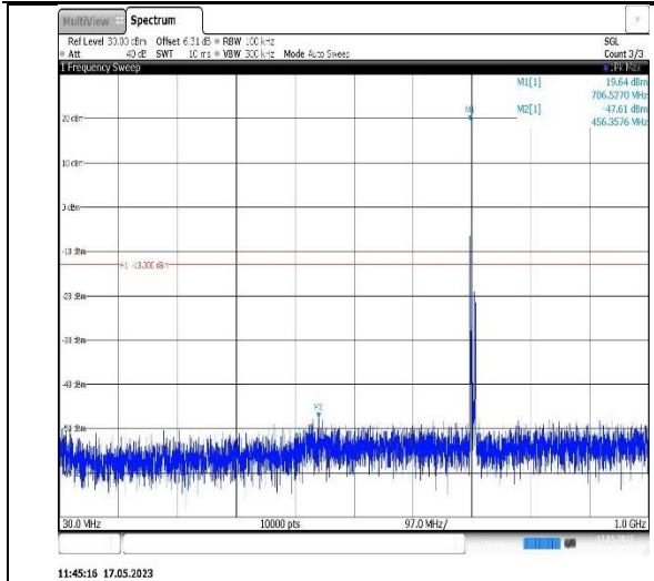
Band13-5MHz-QPSK-23205-1RB#0-Range1:30~1000MHz
