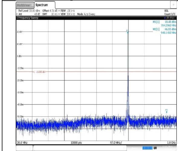
Band17-5MHz-16QAM-23755-1RB#0- Range1:30~1000MHz
