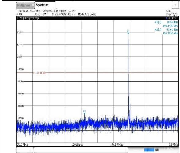
Band12-5MHz-16QAM-23035-1RB#0- Range1:30~1000MHz
