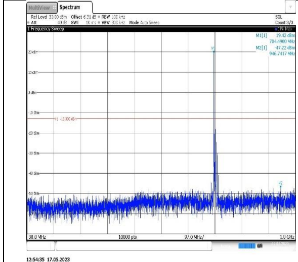
Band17-10MHz-QPSK-23790-1RB#0-Range1:30~1000MHz
