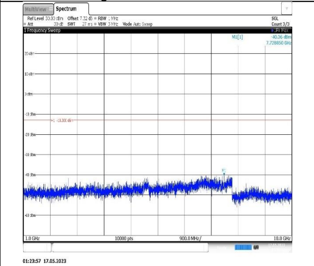
Band5-3MHz-QPSK-20635-1RB#0- Range2:1000~10000MHz
