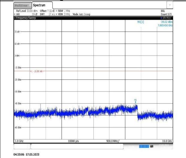
Band5-10MHz-QPSK-20600-1RB#0-Range2:1000~10000MHz
