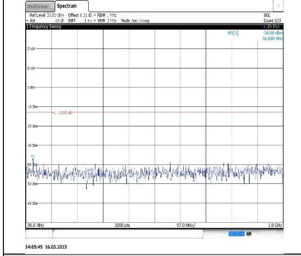
14:05:45 16.05.2023 Band4-5MHz-16QAM-20175-1RB#0-Range1:30~1000MHz
