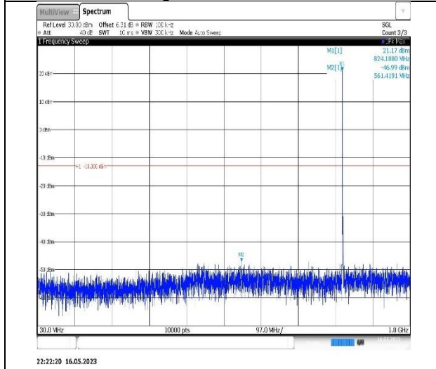
Band5-1.4MHz-QPSK-20525-1RB#0-Range1:30~1000MHz
