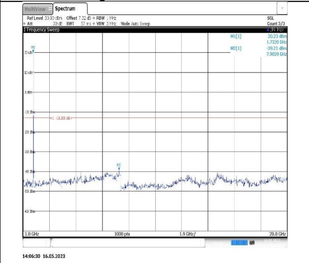
14:06:30 16.05.2023 Band4-5MHz-16QAM-20375-1RB#0-Range2:1000~20000MHz
