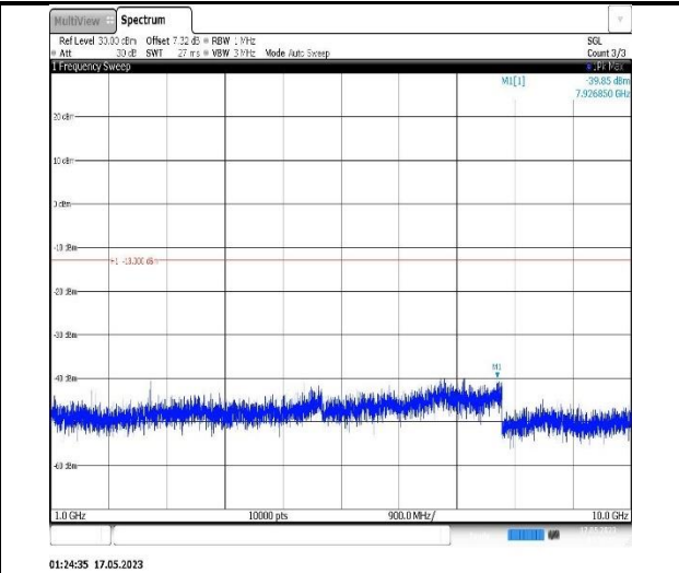
Band5-3MHz-16QAM-20415-1RB#0-Range2:1000~10000MHz
