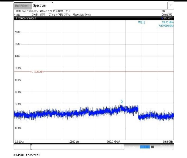
Band5-10MHz-QPSK-20450-1RB#0-Range2:1000~10000MHz
