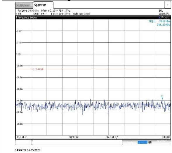
Band4-10MHz-QPSK-20350-1RB#0-Range1:30~1000MHz
