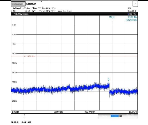
Band5-3MHz-QPSK-20525-1RB#0- Range2:1000~10000MHz
