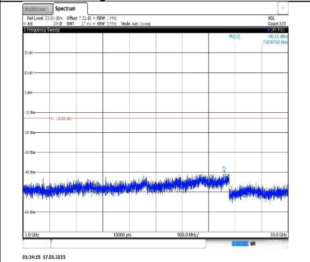
Band5-3MHz-16QAM-20635-1RB#0-Range2:1000~10000MHz
