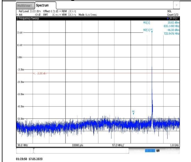
Band5-3MHz-QPSK-20635-1RB#0- Range1:30~1000MHz
