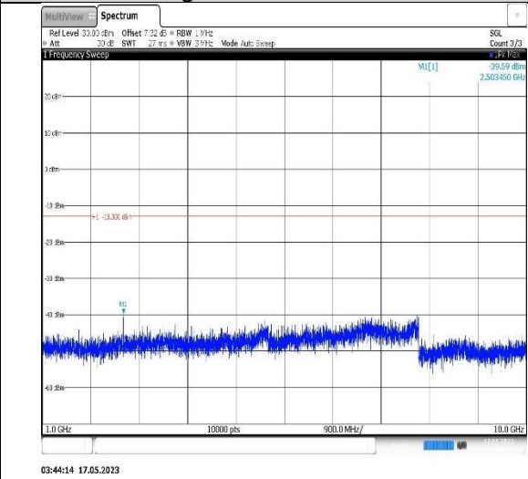
Band5-5MHz-QPSK-20625-1RB#0- Range2:1000~10000MHz
