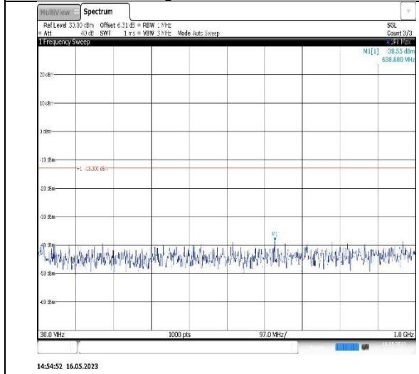
Band4-15MHz-QPSK-20175-1RB#0-Range1:30~1000MHz
