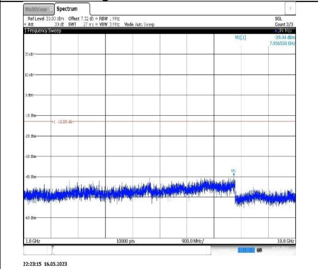
Band5-1.4MHz-QPSK-20643-1RB#0-Range2:1000~10000MHz
