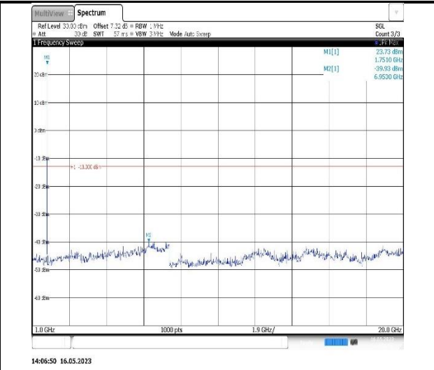
14:06:50 16.05.2023 Band4-5MHz-16QAM-19975-1RB#0-Range2:1000~20000MHz
