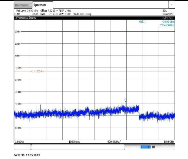
Band5-10MHz-QPSK-20525-1RB#0-Range2:1000~10000MHz
