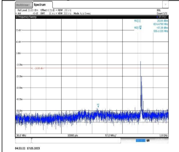
Band5-10MHz-QPSK-20525-1RB#0-Range1:30~1000MHz
