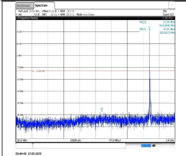
Band5-5MHz-16QAM-20425-1RB#0-Range1:30~1000MHz
