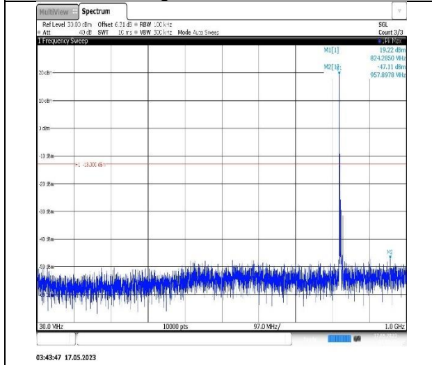
Band5-5MHz-16QAM-20525-1RB#0-Range1:30~1000MHz
