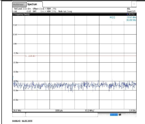
14:06:42 16.05.2023 Band4-5MHz-16QAM-19975-1RB#0-Range1:30~1000MHz
