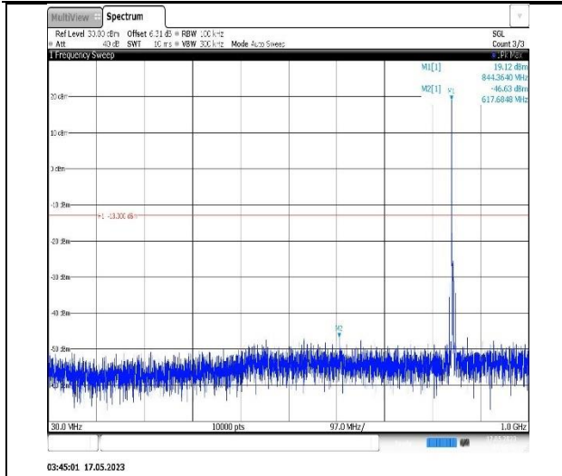
Band5-10MHz-QPSK-20450-1RB#0-Range1:30~1000MHz
