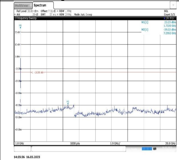
Band4-15MHz-QPSK-20325-1RB#0-Range2:1000~20000MHz
