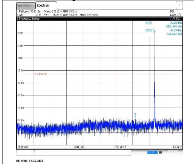
Band5-3MHz-16QAM-20635-1RB#0-Range1:30~1000MHz
