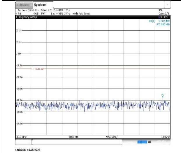
Band4-5MHz-QPSK-20175-1RB#0- Range1:30~1000MHz
