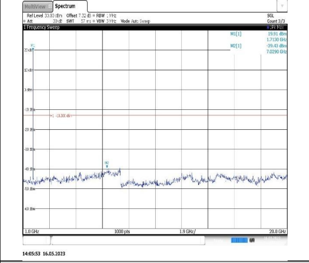
14:05:53 16.05.2023 Band4-5MHz-16QAM-20175-1RB#0-Range2:1000~20000MHz
