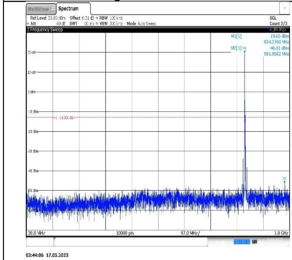
Band5-5MHz-QPSK-20625-1RB#0- Range1:30~1000MHz
