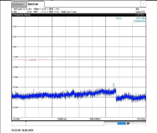
Band5-1.4MHz-QPSK-20525-1RB#0-Range2:1000~10000MHz
