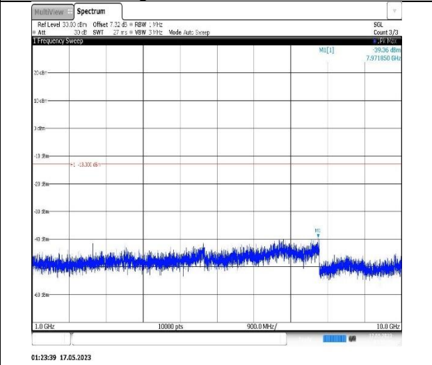
Band5-3MHz-16QAM-20525-1RB#0-Range2:1000~10000MHz
