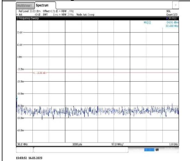
Band4-20MHz-QPSK-20300-1RB#0-Range1:30~1000MHz
