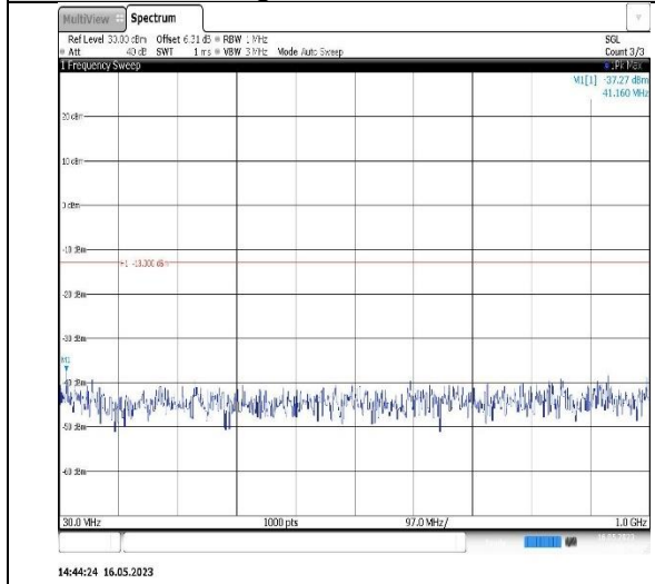
Band4-10MHz-QPSK-20175-1RB#0-Range1:30~1000MHz
