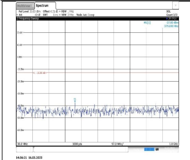
Band4-20MHz-QPSK-20050-1RB#0-Range1:30~1000MHz
