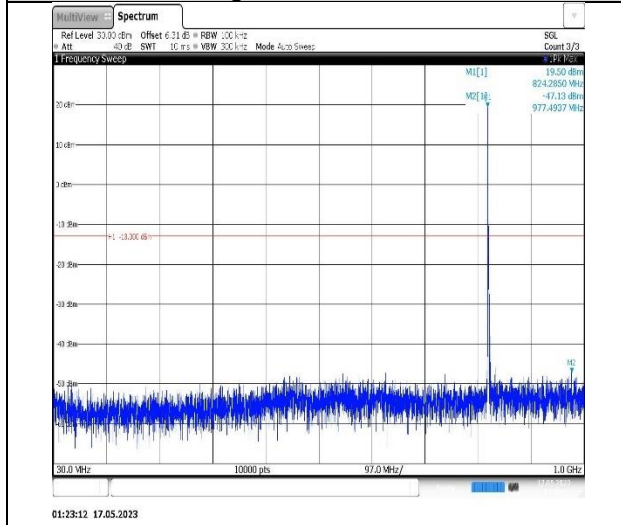
Band5-3MHz-QPSK-20525-1RB#0- Range1:30~1000MHz
