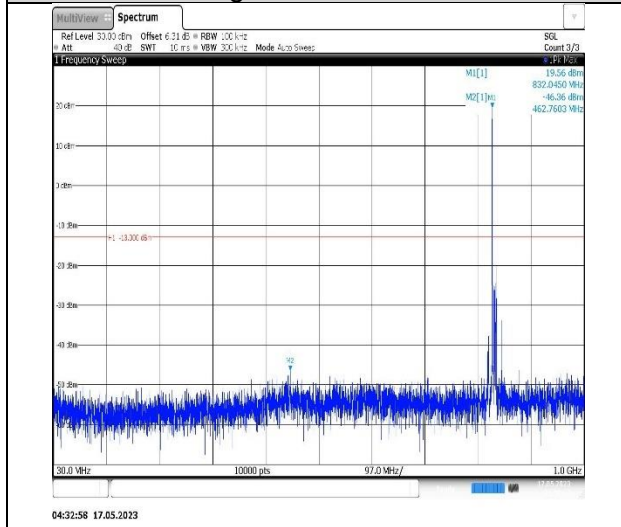
Band5-10MHz-QPSK-20600-1RB#0-Range1:30~1000MHz
