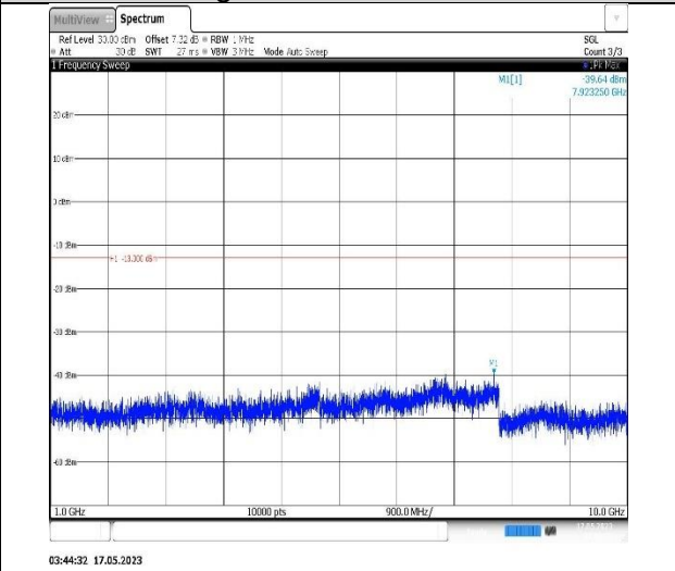
Band5-5MHz-16QAM-20625-1RB#0-Range2:1000~10000MHz
