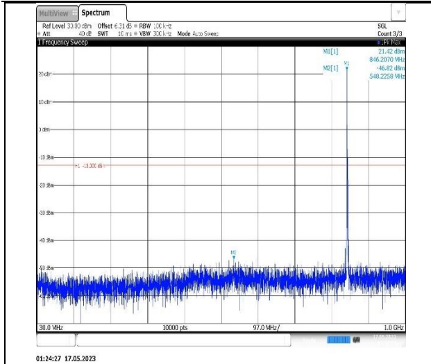
Band5-3MHz-16QAM-20415-1RB#0-Range1:30~1000MHz
