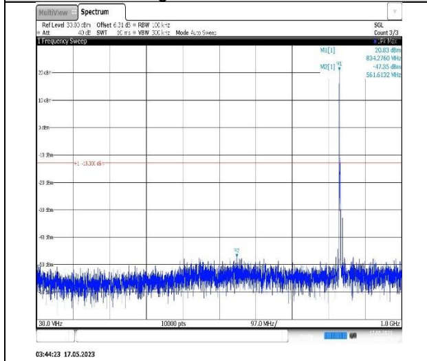
Band5-5MHz-16QAM-20625-1RB#0-Range1:30~1000MHz
