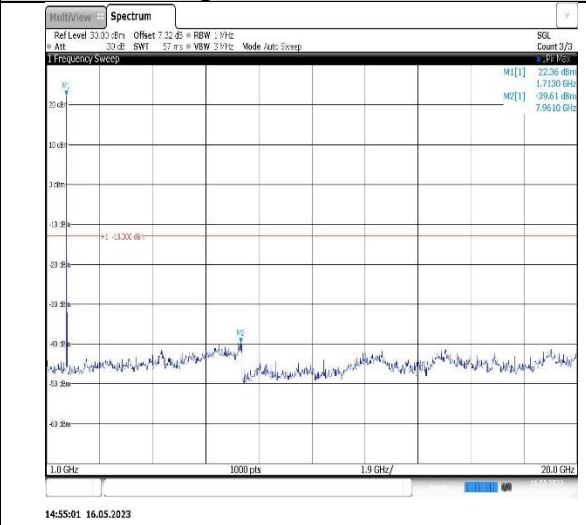
Band4-15MHz-QPSK-20175-1RB#0-Range2:1000~20000MHz
