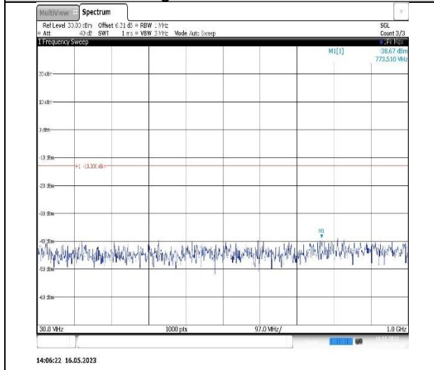
14:06:22 16.05.2023 Band4-5MHz-16QAM-20375-1RB#0-Range1:30~1000MHz
