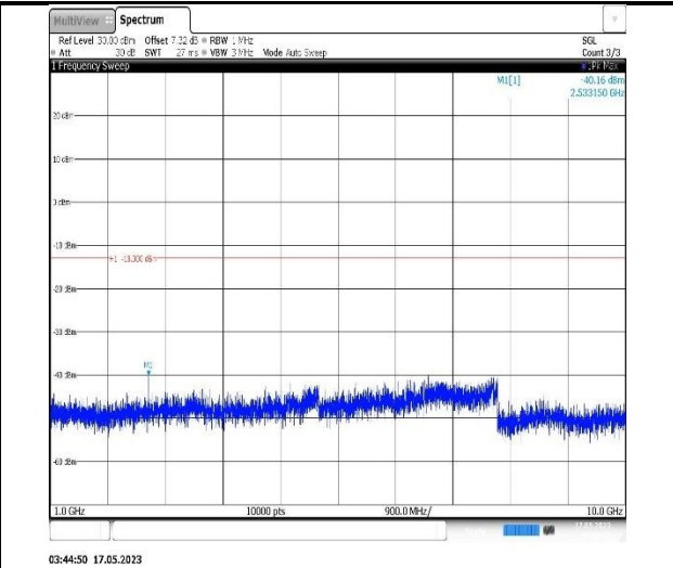
Band5-5MHz-16QAM-20425-1RB#0-Range2:1000~10000MHz
