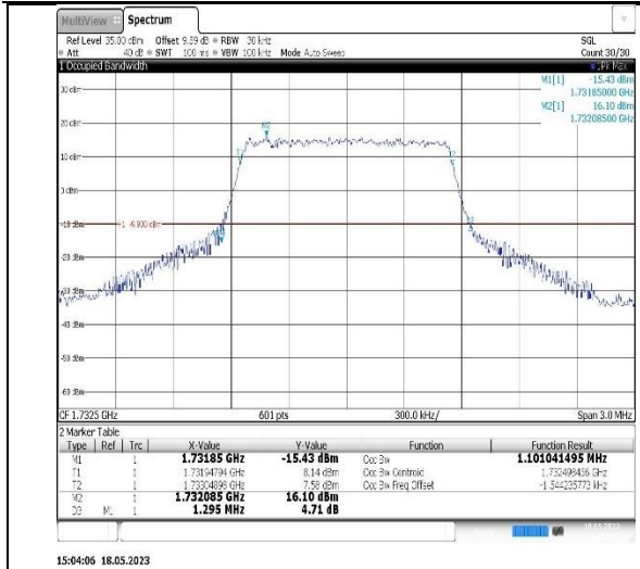
Band4-3MHz-QPSK-20175-15RB#0
