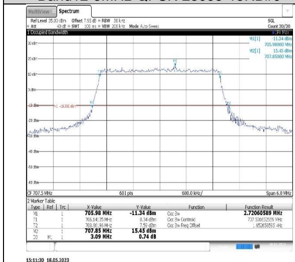
Band12-5MHz-QPSK-23095-25RB#0
