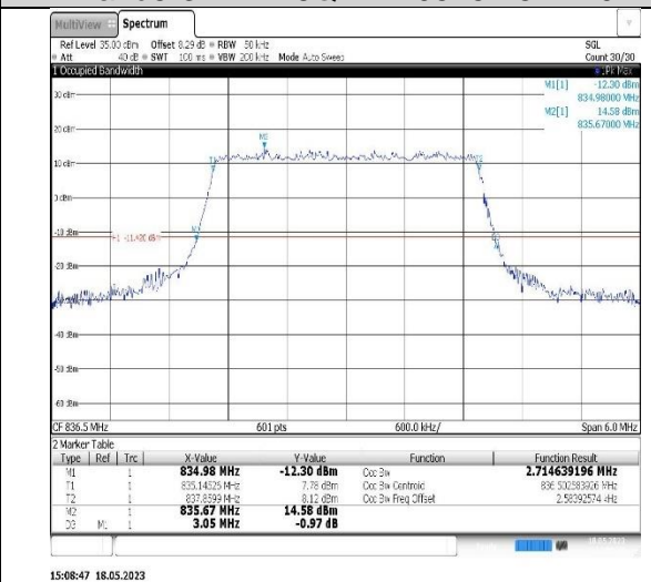
Band5-5MHz-16QAM-20525-25RB#0
