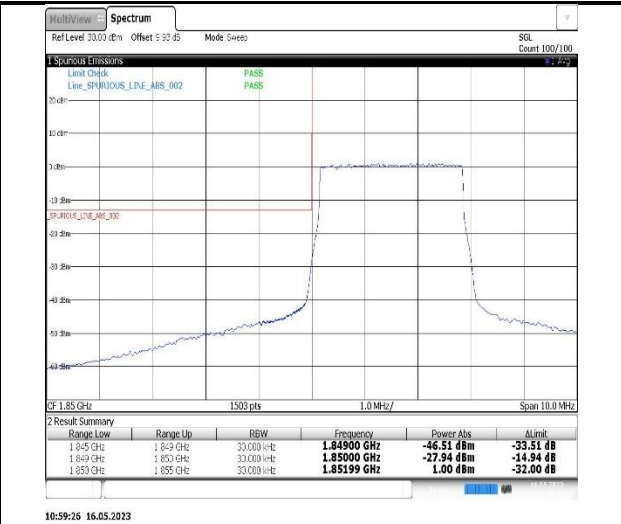
Band2-3MHz-16QAM-19185-15RB#0
