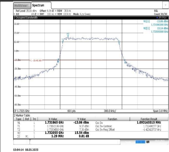
Band4-3MHz-16QAM-20175-15RB#0
