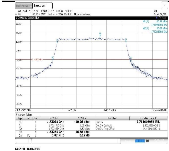
Band4-5MHz-QPSK-20175-25RB#0
