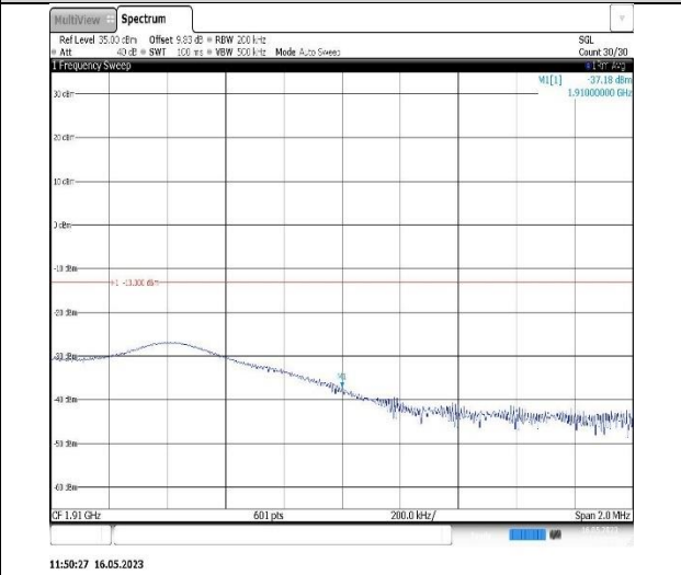
Band2-10MHz-QPSK-19150-50RB#0
