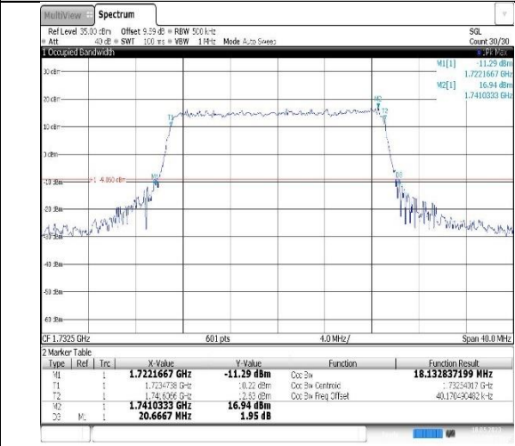
Band4-20MHz-16QAM-20175-100RB#0
