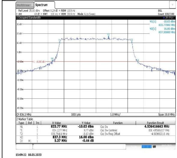
Band5-10MHz-QPSK-20525-50RB#0
