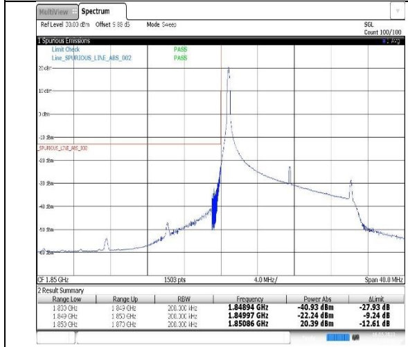
Band2-15MHz-16QAM-18675-1RB#0
