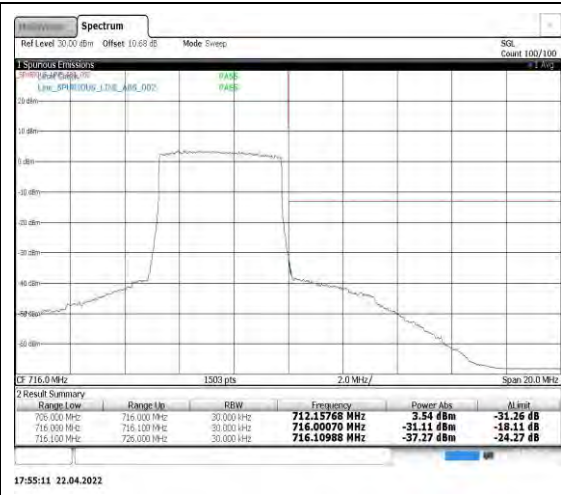
Band17-5MHz-16QAM-23825-25RB#0
