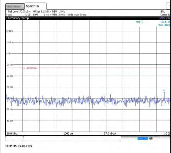
Band4-5MHz-QPSK-20175-1RB#0-Range1: 30~1000MHz
