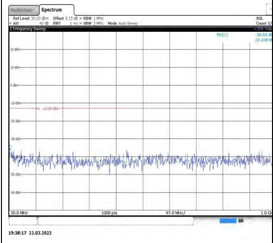
Band4-10MHz-QPSK-20175-1RB#0-Range 1:30~1000MHz
