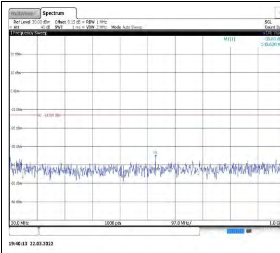
Band4-15MHz-QPSK-20025-1RB#0-Range 1:30~1000MHz
