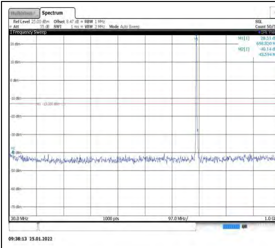
Band12-3MHz-QPSK-23025-1RB#0-Range 1:30~1000MHz
