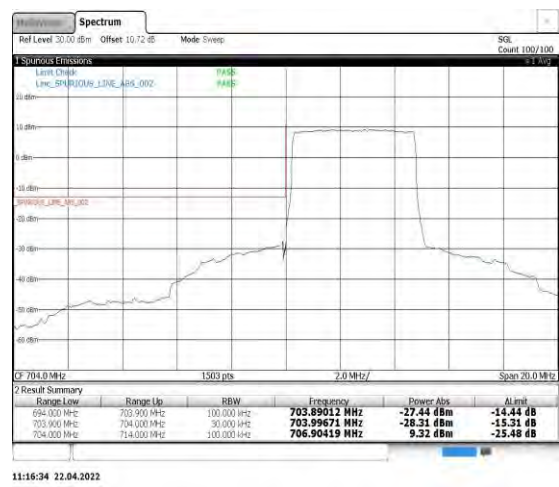
Band17-5MHz-QPSK-23755-25RB#0
