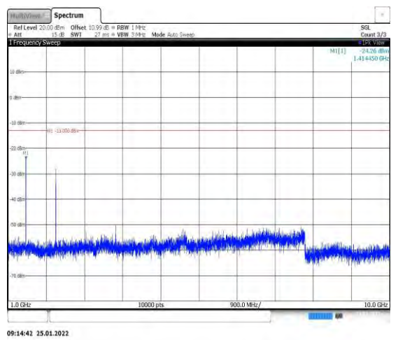
Band12-1.4MHz-QPSK-23095-1RB#0-Range2 :1000~10000MHz
