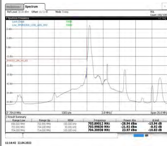
Band17-5MHz-QPSK-23755-1RB#0
