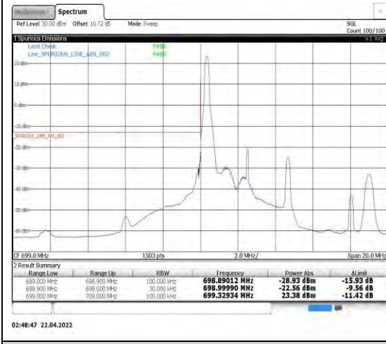
Band12-5MHz-QPSK-23035-1RB#0
