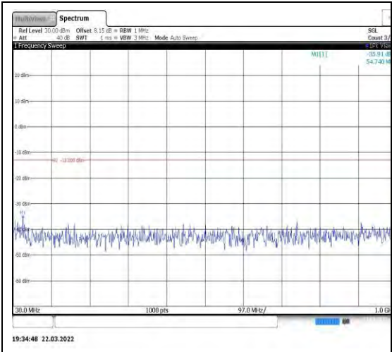
Band4-5MHz-QPSK-19975-1RB#0-Range1: 30~1000MHz
