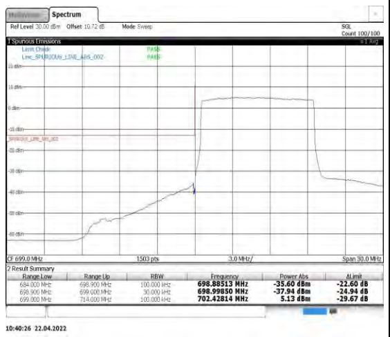
Band12-10MHz-16QAM-23060-50RB#0
