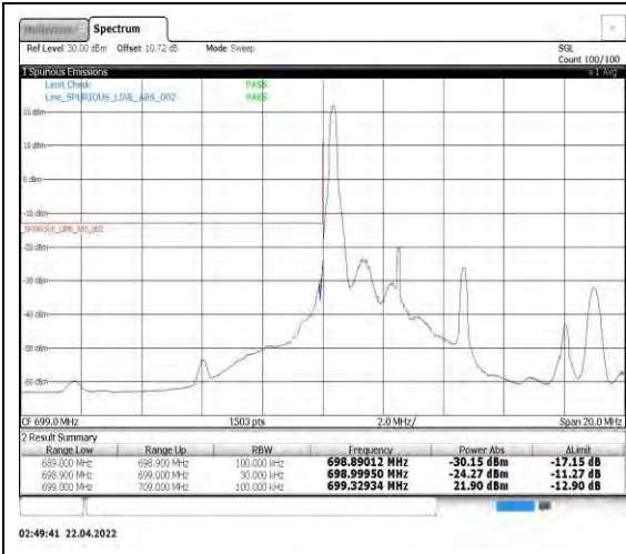
Band12-5MHz-16QAM-23035-1RB#0
