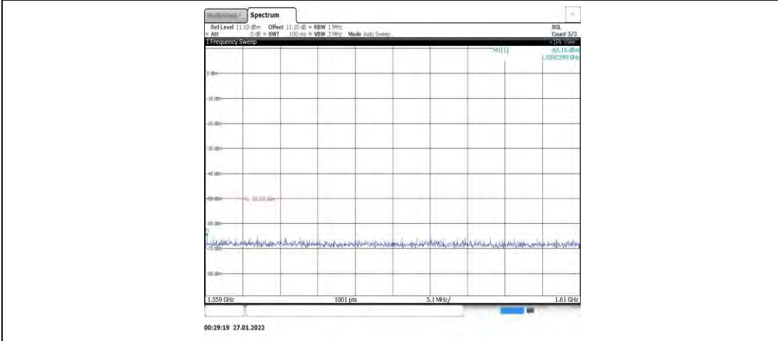
Band13-5MHz-QPSK-23230-1RB#0-Range5:1559~1610MHz
