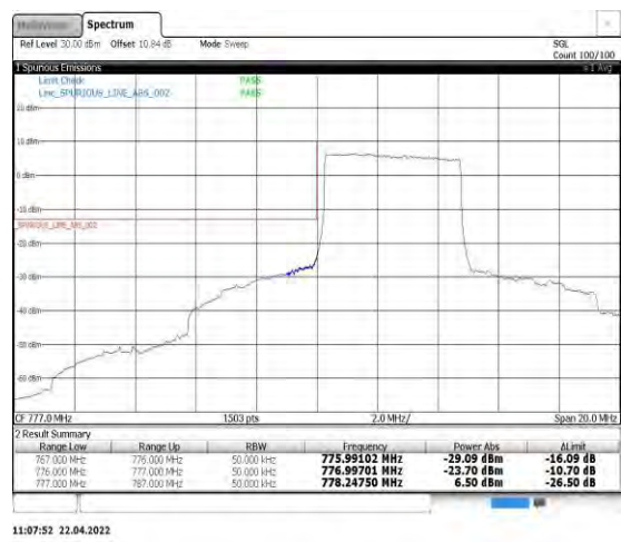
Band13-5MHz-QPSK-23205-25RB#0
