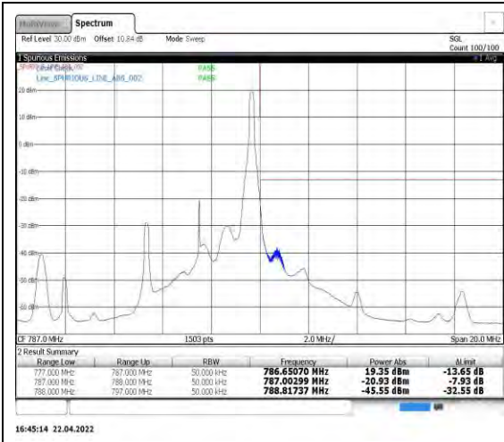
Band13-5MHz-16QAM-23255-1RB#24
