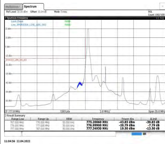
Band13-5MHz-16QAM-23205-1RB#0
