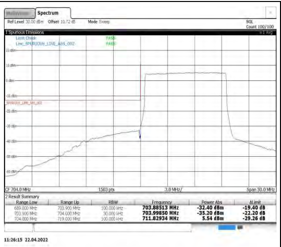
Band17-10MHz-16QAM-23780-50RB#0
