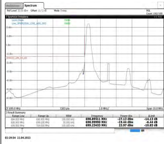
Band12-3MHz-QPSK-23025-1RB#0
