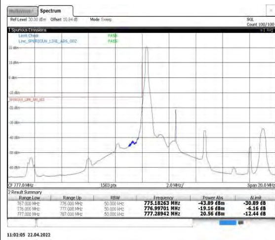
Band13-5MHz-QPSK-23205-1RB#0
