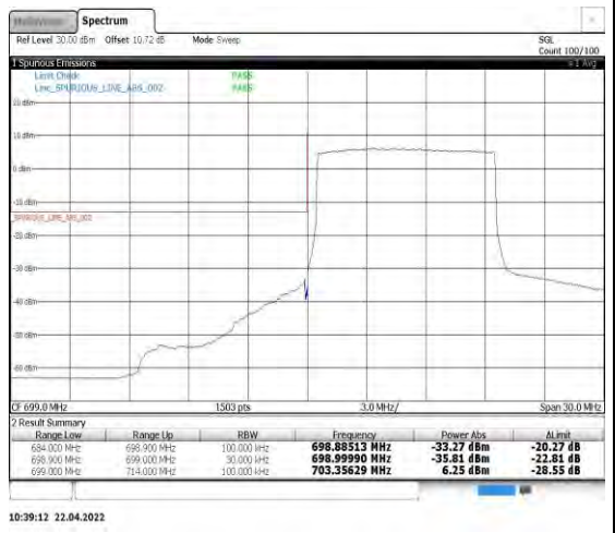
Band12-10MHz-QPSK-23060-50RB#0
