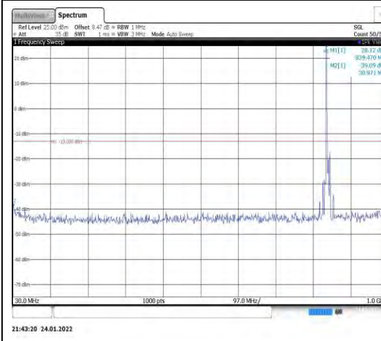
Band5-10MHz-QPSK-20600-1RB#0-Range 1:30~1000MHz
