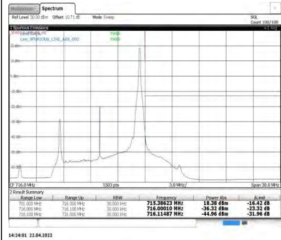
Band17-10MHz-16QAM-23800-1RB#49
