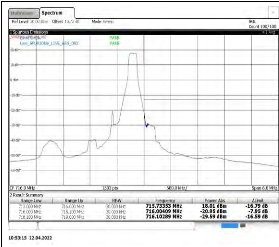
Band12-1.4MHz-16QAM-23173-1RB#5
