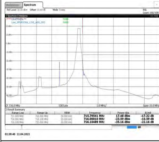
Band12-3MHz-16QAM-23165-1RB#14
