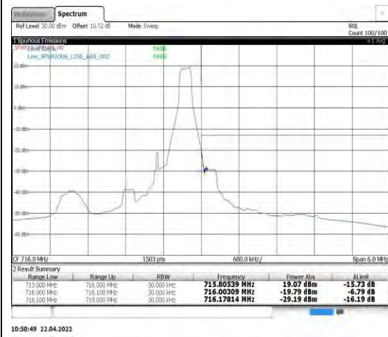
Band12-1.4MHz-QPSK-23173-1RB#5
