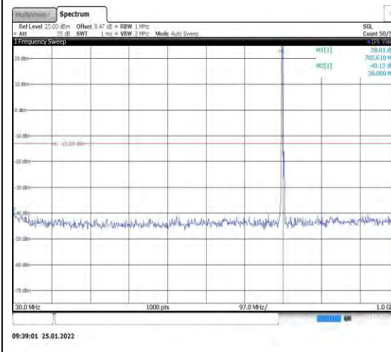
Band12-3MHz-QPSK-23095-1RB#0-Range 1:30~1000MHz
