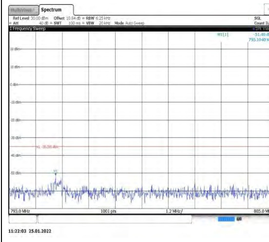
Band13-10MHz-QPSK-23230-1RB#0-Rang e4:793~805MHz
