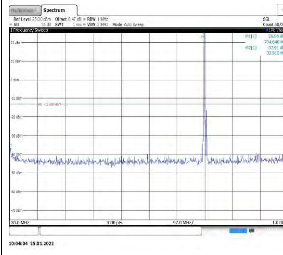
Band12-5MHz-QPSK-23095-1RB#0-Range 1:30~1000MHz
