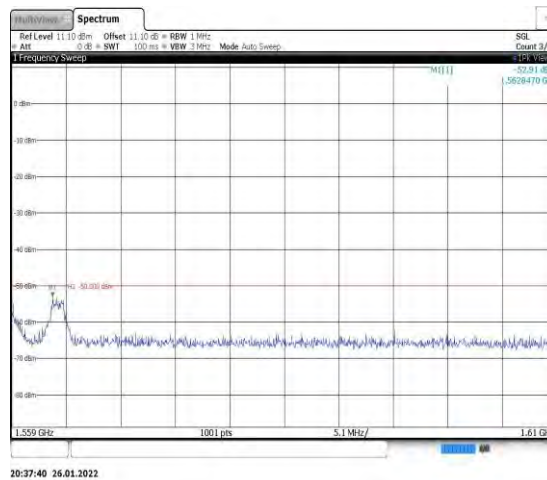
Band13-5MHz-QPSK-23205-1RB#0-Range5:1559~1610MHz
