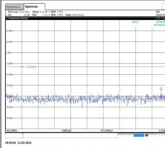
Band4-3MHz-QPSK-20385-1RB#0-Range1: 30~1000MHz
