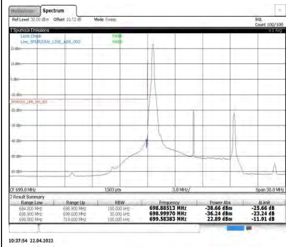
Band12-10MHz-16QAM-23060-1RB#0
