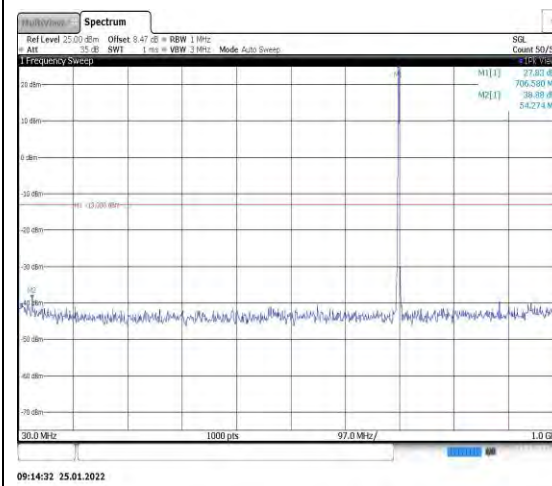
Band12-1.4MHz-QPSK-23095-1RB#0-Rang e1:30~1000MHz
