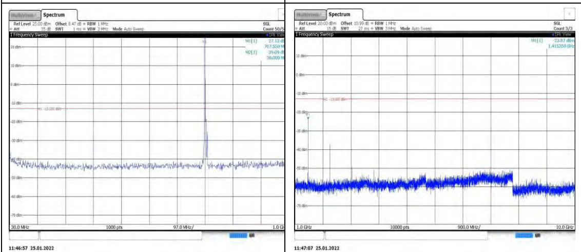
Band17-5MHz-QPSK-23790-1RB#0-Range 1:30~1000MHz
