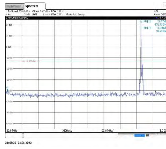
Band5-10MHz-QPSK-20525-1RB#0-Range 1:30~1000MHz
