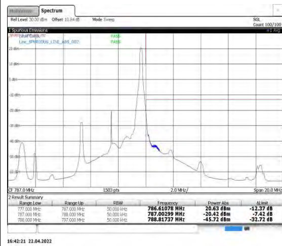
Band13-5MHz-QPSK-23255-1RB#24
