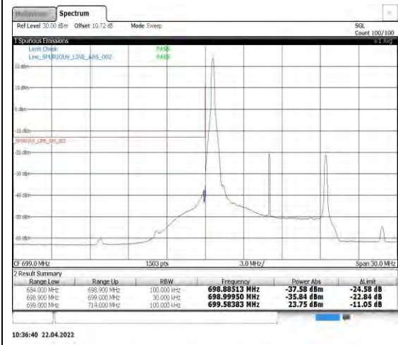
Band12-10MHz-QPSK-23060-1RB#0
