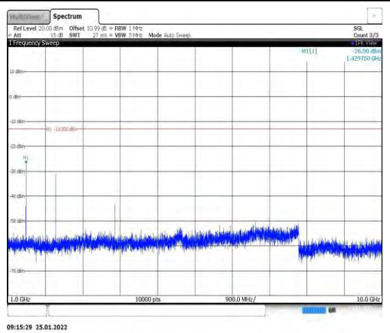
Band12-1.4MHz-QPSK-23173-1RB#0-Range2 :1000~10000MHz
