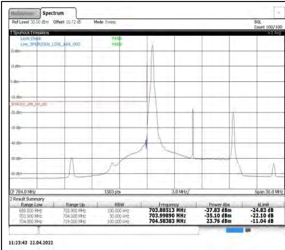
Band17-10MHz-16QAM-23780-1RB#0
