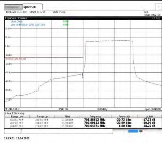
Band17-10MHz-QPSK-23780-50RB#0
