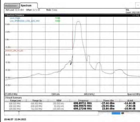
Band12-1.4MHz-QPSK-23017-1RB#0
