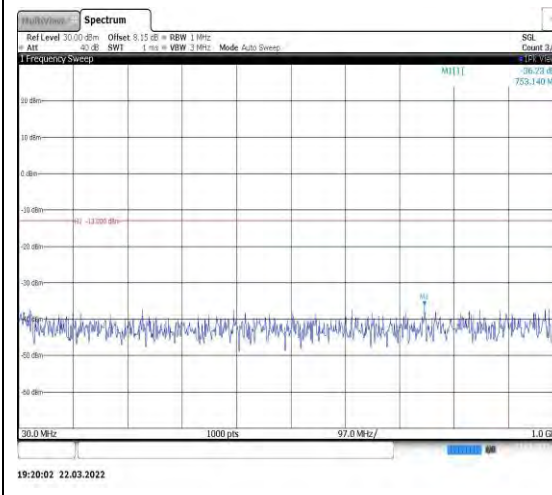
Band2-5MHz-QPSK-18900-1RB#0-Range1: 30~1000MHz
