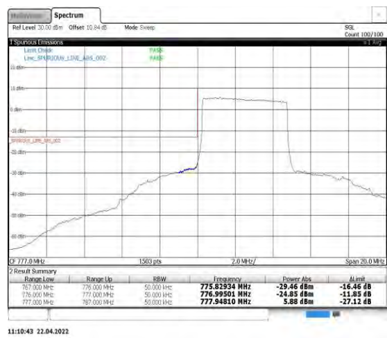
Band13-5MHz-16QAM-23205-25RB#0
