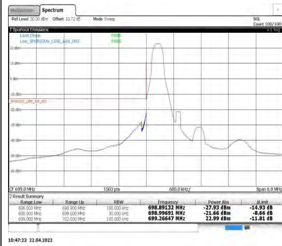
Band12-1.4MHz-16QAM-23017-1RB#0
