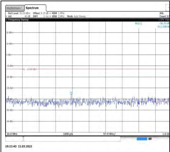
Band2-15MHz-QPSK-18675-1RB#0-Range 1:30~1000MHz
