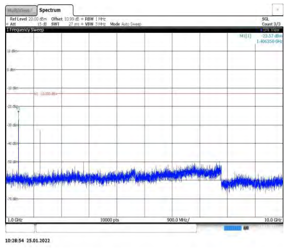
Band12-10MHz-QPSK-23095-1RB#0-Range2: 1000~10000MHz
