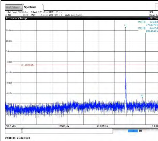
Band13-5MHz-QPSK-23205-1RB#0-Range 1:30~1000MHz
