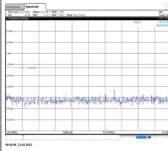
Band4-20MHz-QPSK-20175-1RB#0-Range 1:30~1000MHz
