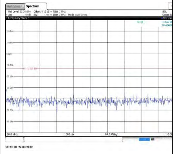
Band2-15MHz-QPSK-18900-1RB#0-Range 1:30~1000MHz
