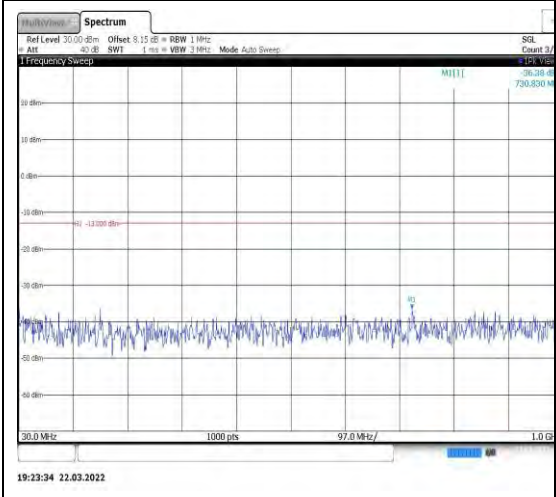
Band2-15MHz-QPSK-19125-1RB#0-Range 1:30~1000MHz
