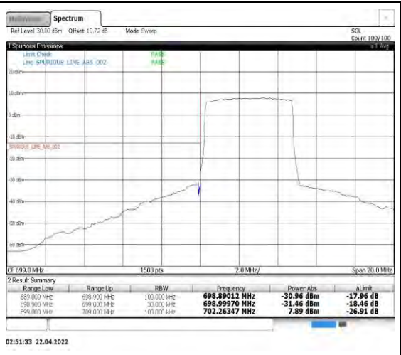
Band12-5MHz-16QAM-23035-25RB#0
