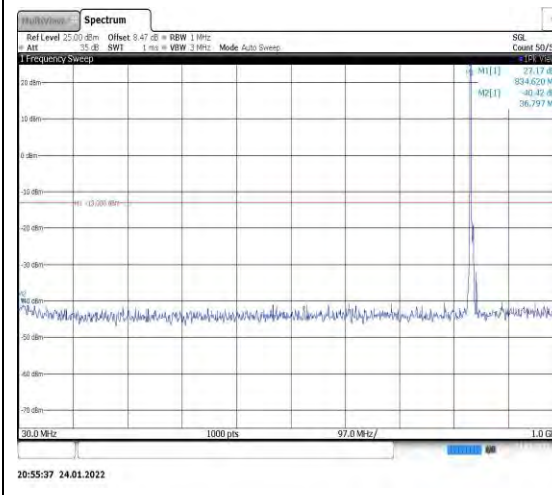
Band5-3MHz-QPSK-20525-1RB#0-Range1: 30~1000MHz
