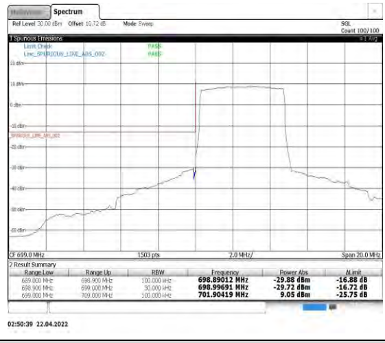
Band12-5MHz-QPSK-23035-25RB#0
