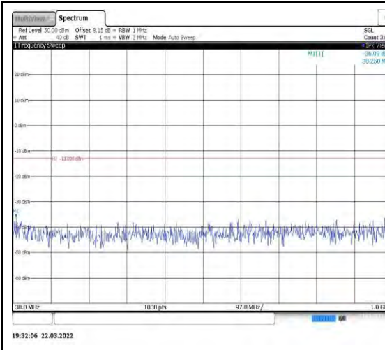
Band4-3MHz-QPSK-19965-1RB#0-Range1: 30~1000MHz
