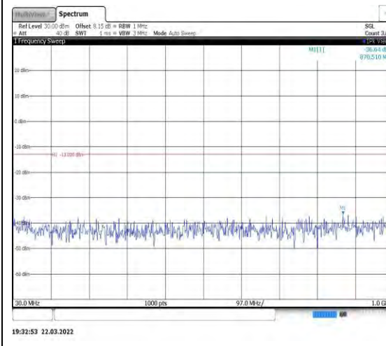
Band4-3MHz-QPSK-20175-1RB#0-Range1: 30~1000MHz
