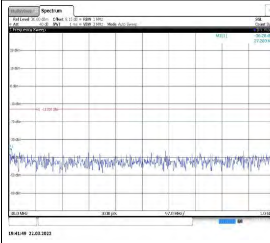
Band4-15MHz-QPSK-20325-1RB#0-Range 1:30~1000MHz
