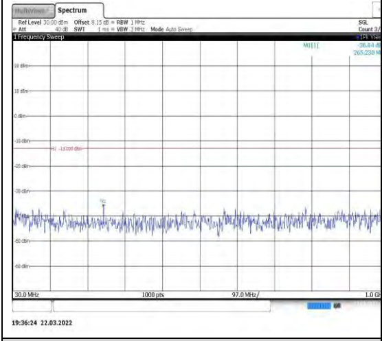
Band4-5MHz-QPSK-20375-1RB#0-Range1: 30~1000MHz
