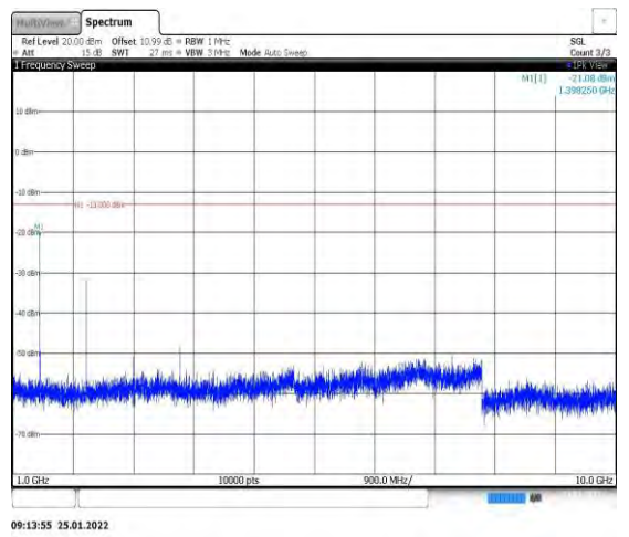
Band12-1.4MHz-QPSK-23017-1RB#0-Range2 :1000~10000MHz
