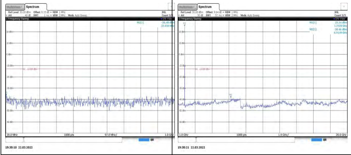
Band4-1.4MHz-QPSK-20175-1RB#0-Range 1:30~1000MHz
