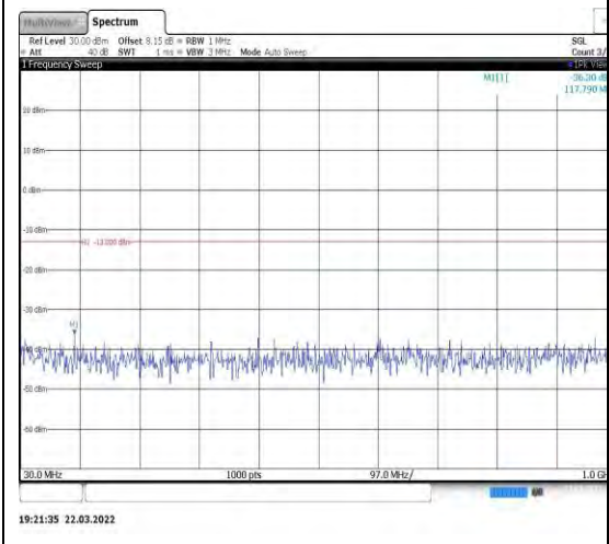
Band2-10MHz-QPSK-18900-1RB#0-Range 1:30~1000MHz
