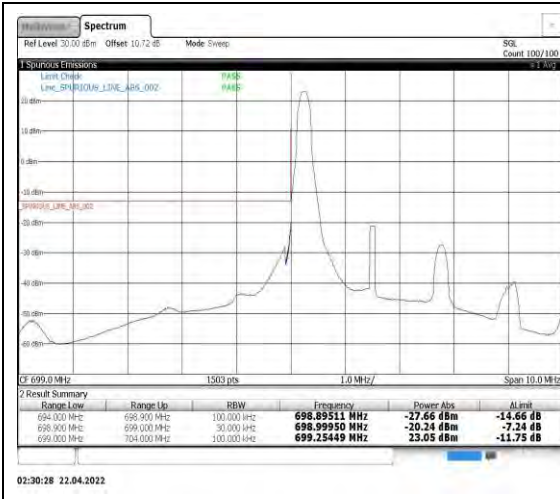
Band12-3MHz-16QAM-23025-1RB#0
