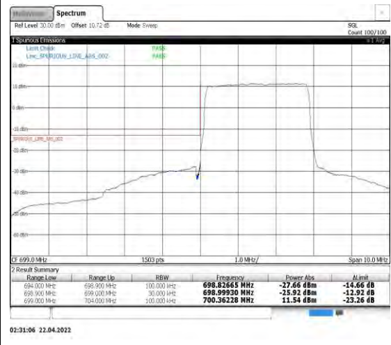
Band12-3MHz-QPSK-23025-15RB#0
