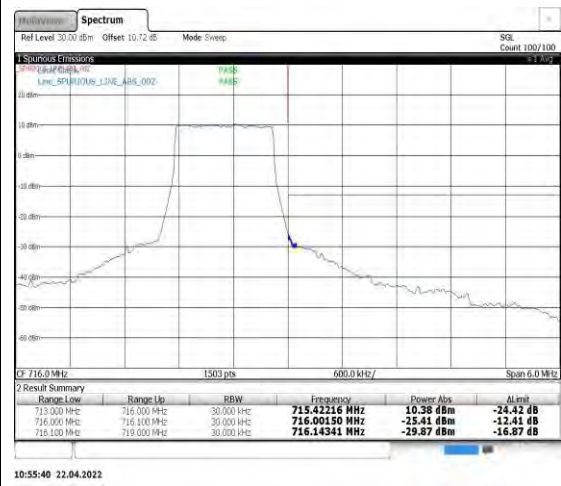
Band12-1.4MHz-QPSK-23173-6RB#0
