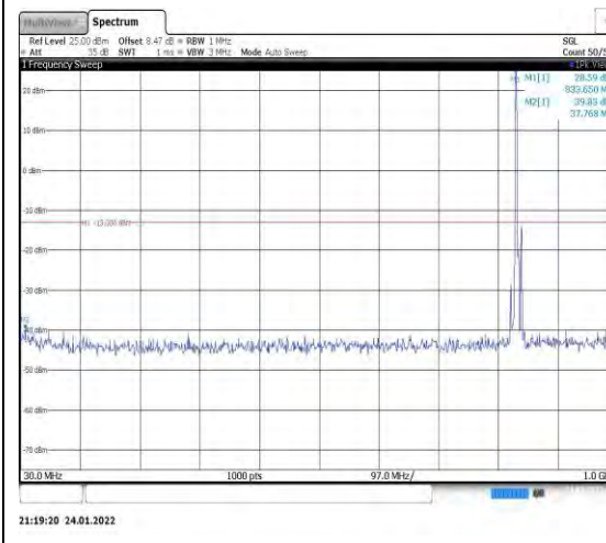
Band5-5MHz-QPSK-20525-1RB#0-Range1: 30~1000MHz
