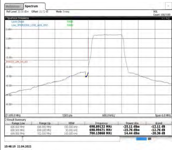
Band12-1.4MHz-16QAM-23017-6RB#0
