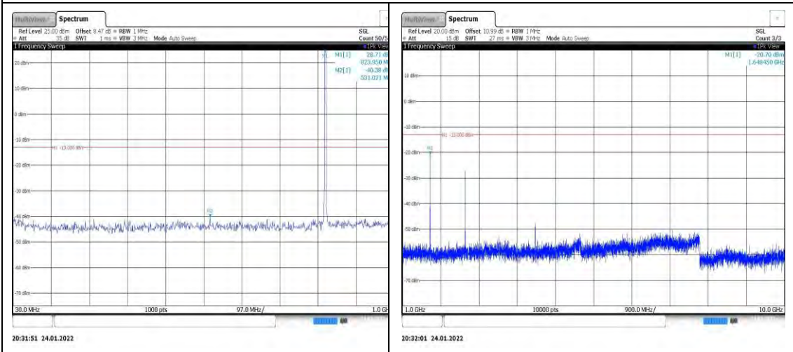
Band5-1.4MHz-QPSK-20407-1RB#0-Range 1:30~1000MHz
