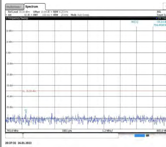
Band13-5MHz-QPSK-23205-1RB#0-Range 4:793~805MHz
