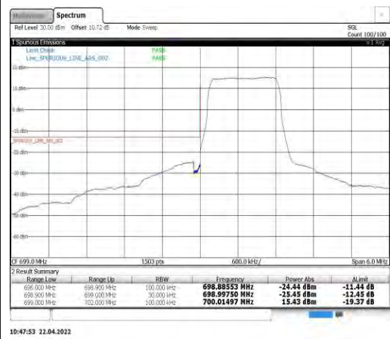
Band12-1.4MHz-QPSK-23017-6RB#0
