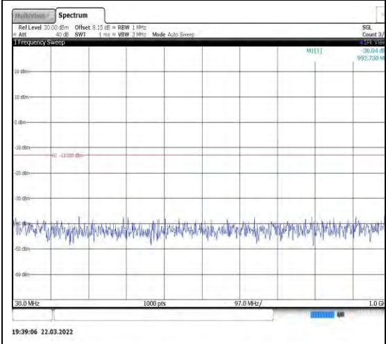
Band4-10MHz-QPSK-20350-1RB#0-Range 1:30~1000MHz
