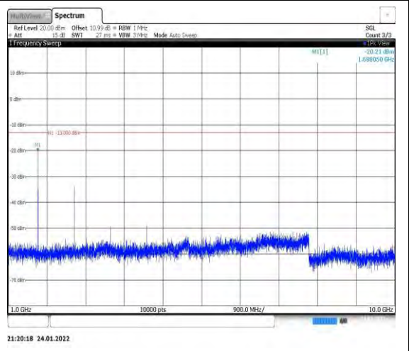
Band5-5MHz-QPSK-20625-1RB#0-Range2:10 00~10000MHz
