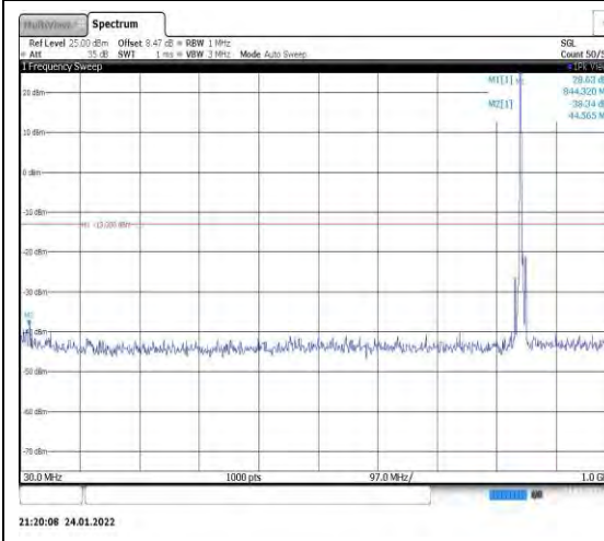
Band5-5MHz-QPSK-20625-1RB#0-Range1: 30~1000MHz
