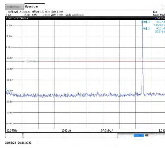
Band5-3MHz-QPSK-20635-1RB#0-Range1: 30~1000MHz
