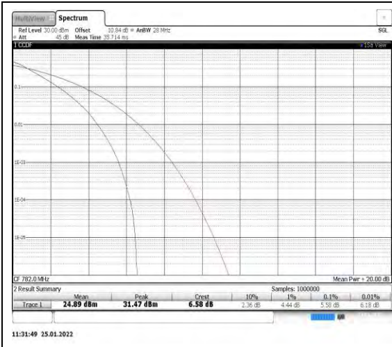
Band13-10MHz-QPSK-23230
