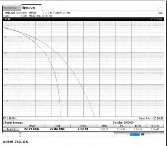
Band2-10MHz-16QAM-18900
