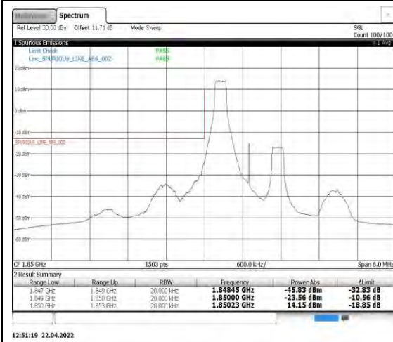
Band2-1.4MHz-16QAM-18607-1RB#0
