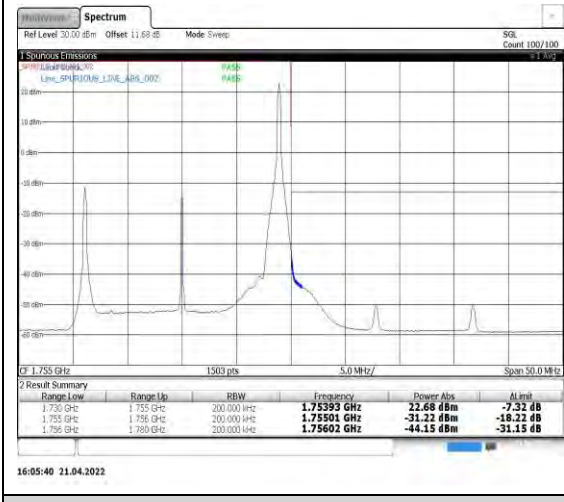
Band4-20MHz-16QAM-20300-1RB#99
