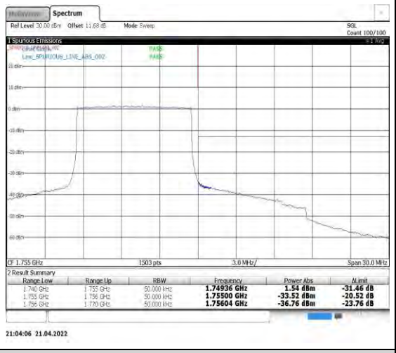
Band4-10MHz-QPSK-20350-50RB#0
