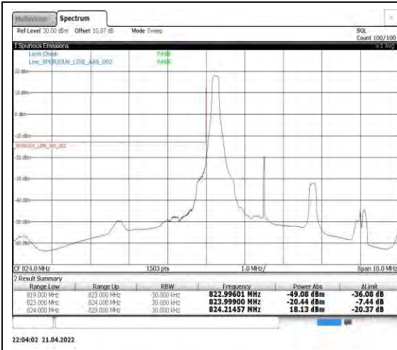
Band5-3MHz-16QAM-20415-1RB#0
