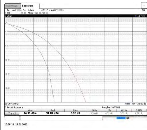
Band12-10MHz-QPSK-23095
