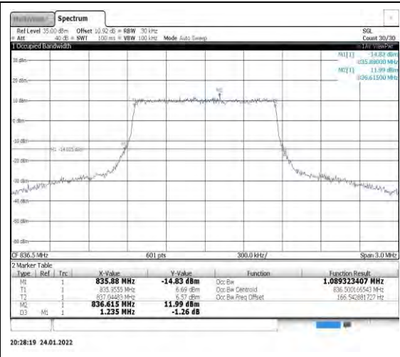
Band5-1.4MHz-16QAM-20525-6RB#0
