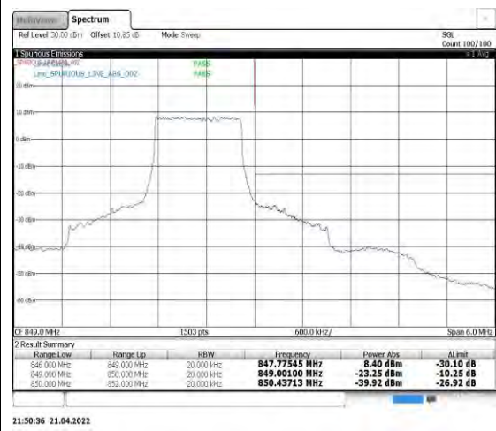
Band5-1.4MHz-QPSK-20643-6RB#0
