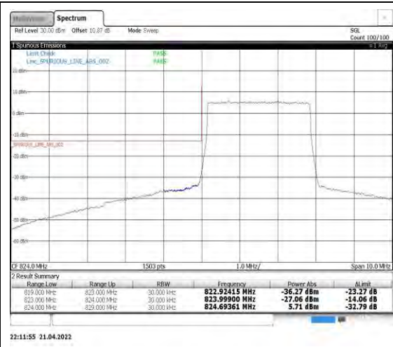
Band5-3MHz-16QAM-20415-15RB#0
