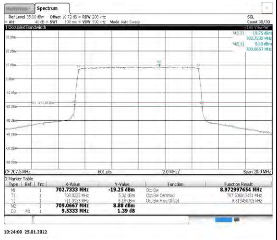
Band12-10MHz-16QAM-23095-50RB#0
