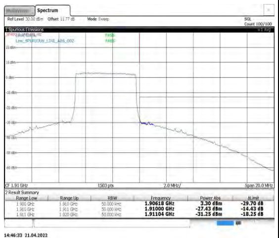
Band2-5MHz-16QAM-19175-25RB#0
