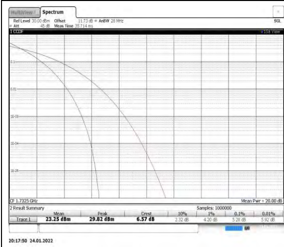
Band4-20MHz-QPSK-20175
