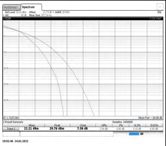
Band4-5MHz-16QAM-20175
