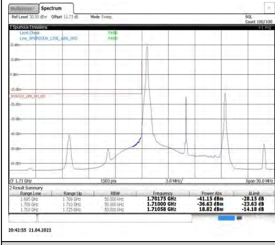
Band4-10MHz-16QAM-20000-1RB#0
