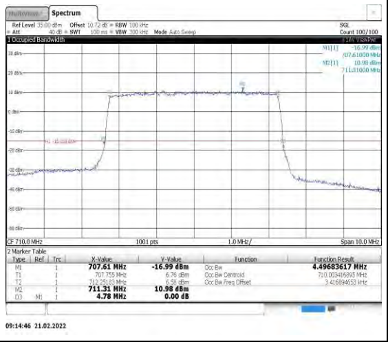
Band17-5MHz-16QAM-23790-25RB#0
