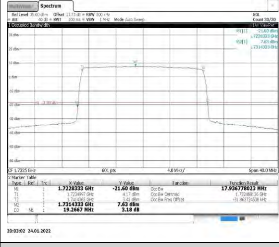
Band4-20MHz-16QAM-20175-100RB#0
