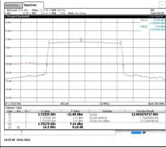
Band4-15MHz-16QAM-20175-75RB#0
