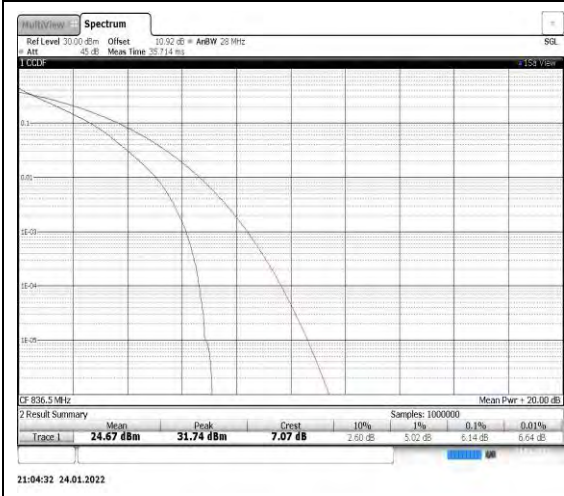
Band5-3MHz-QPSK-20525
