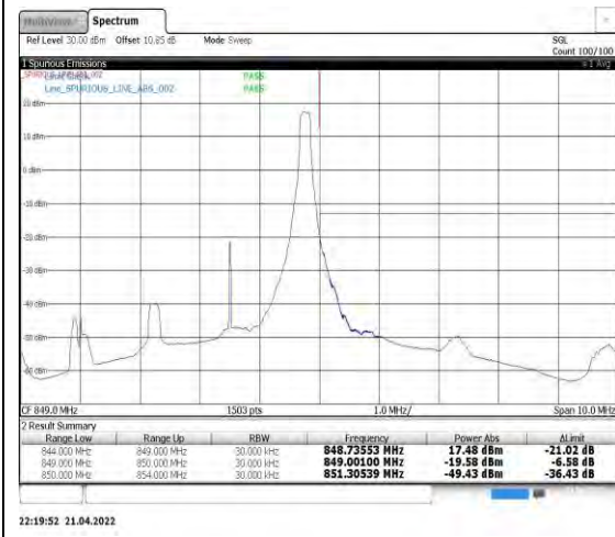
Band5-3MHz-16QAM-20635-1RB#14
