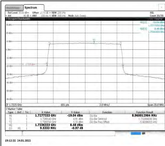
Band4-10MHz-QPSK-20175-50RB#0
