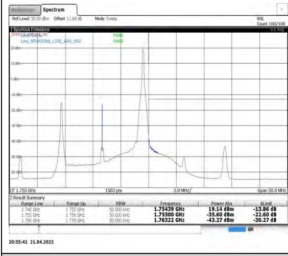
Band4-10MHz-QPSK-20350-1RB#49
