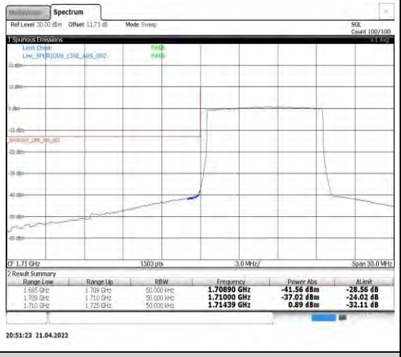
Band4-10MHz-16QAM-20000-50RB#0
