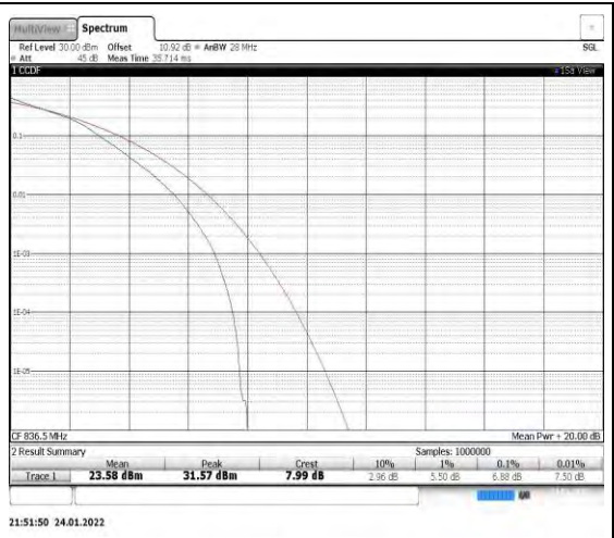
Band5-10MHz-16QAM-20525
