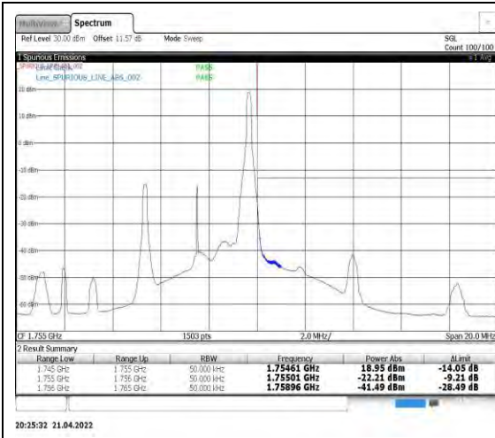
Band4-5MHz-QPSK-20375-1RB#24
