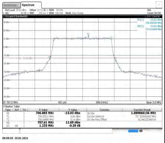
Band12-1.4MHz-16QAM-23095-6RB#0
