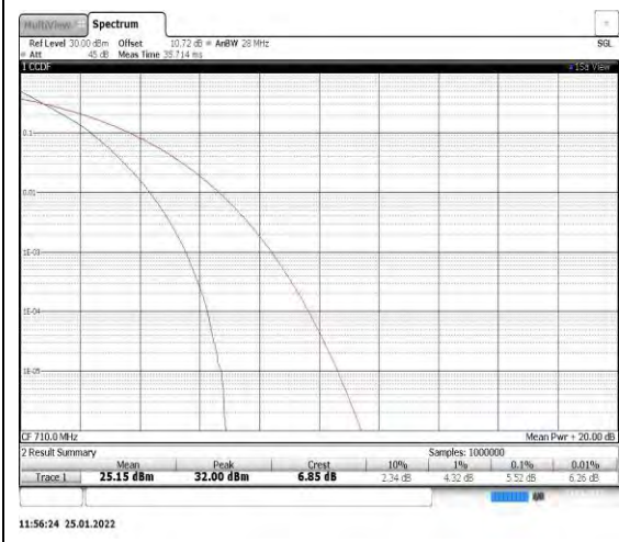
Band17-5MHz-QPSK-23790
