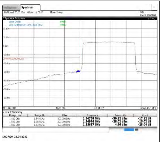
Band2-15MHz-16QAM-18675-75RB#0
