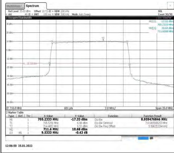
Band17-10MHz-QPSK-23790-50RB#0
