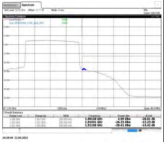
Band2-15MHz-16QAM-19125-75RB#0
