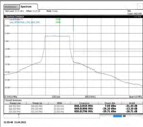
Band5-1.4MHz-16QAM-20643-6RB#0
