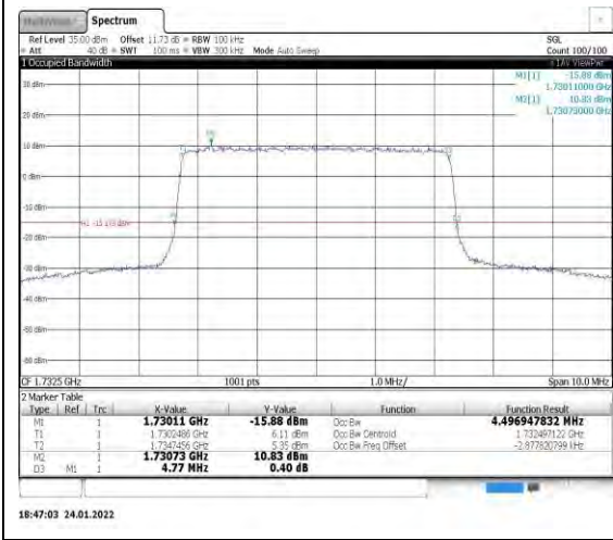
Band4-5MHz-QPSK-20175-25RB#0
