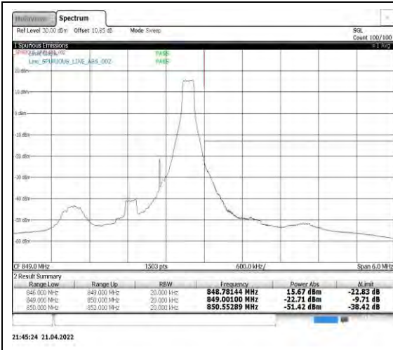
Band5-1.4MHz-16QAM-20643-1RB#5
