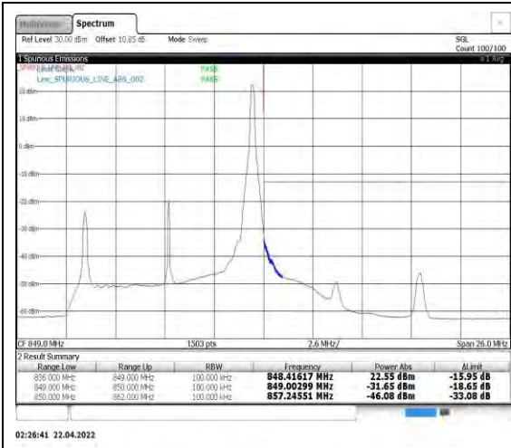
Band5-10MHz-16QAM-20600-1RB#49
