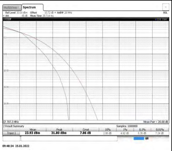
Band12-3MHz-16QAM-23095
