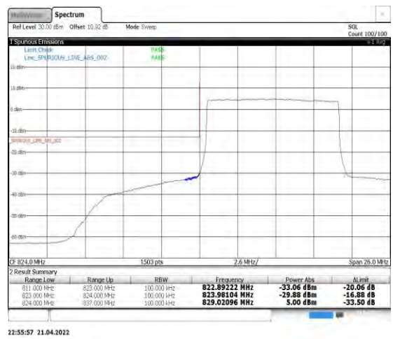
Band5-10MHz-16QAM-20450-50RB#0
