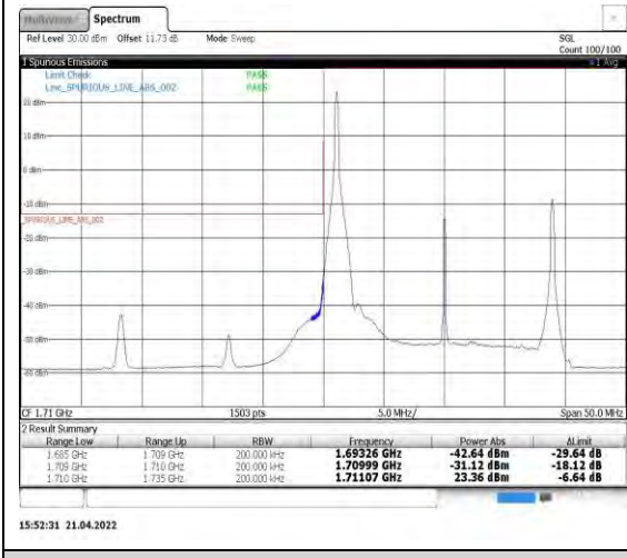
Band4-20MHz-16QAM-20050-1RB#0
