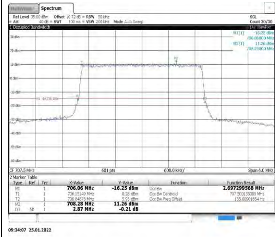
Band12-3MHz-QPSK-23095-15RB#0
