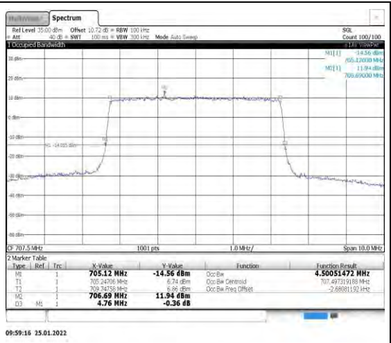
Band12-5MHz-16QAM-23095-25RB#0
