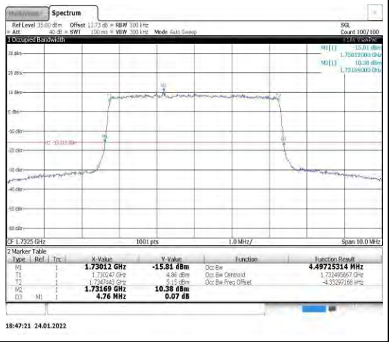
Band4-5MHz-16QAM-20175-25RB#0
