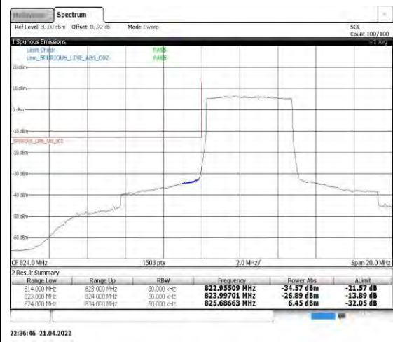
Band5-5MHz-QPSK-20425-25RB#0
