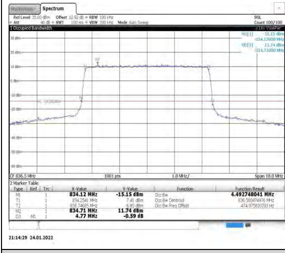
Band5-5MHz-QPSK-20525-25RB#0
