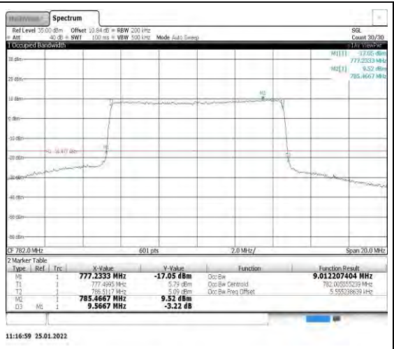
Band13-10MHz-16QAM-23230-50RB#0
