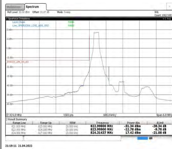
Band5-1.4MHz-QPSK-20407-1RB#0
