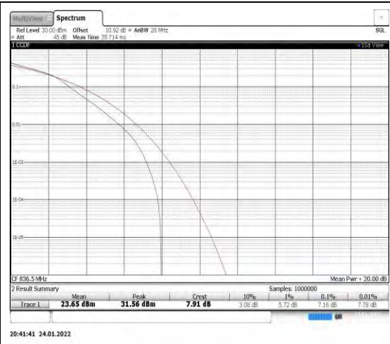
Band5-1.4MHz-16QAM-20525
