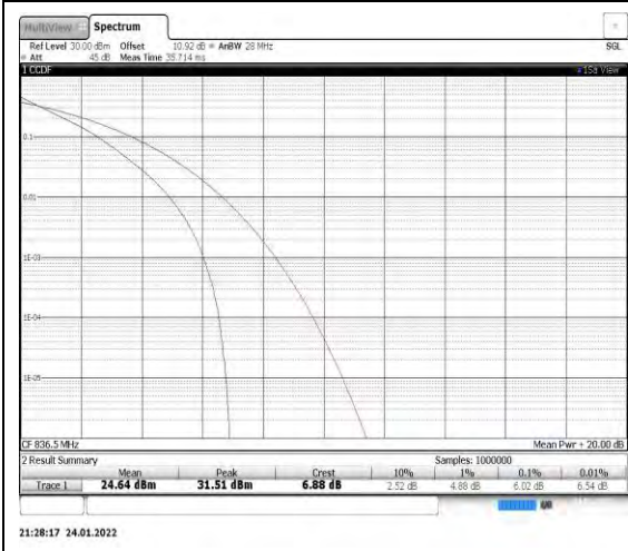
Band5-5MHz-QPSK-20525
