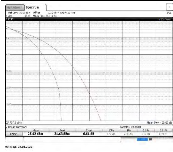
Band12-1.4MHz-QPSK-23095
