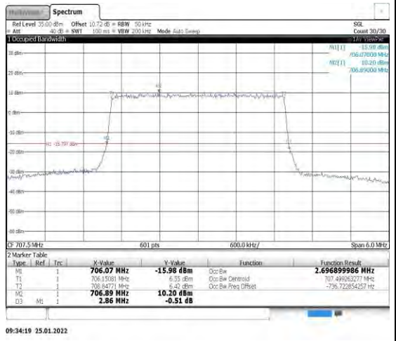
Band12-3MHz-16QAM-23095-15RB#0
