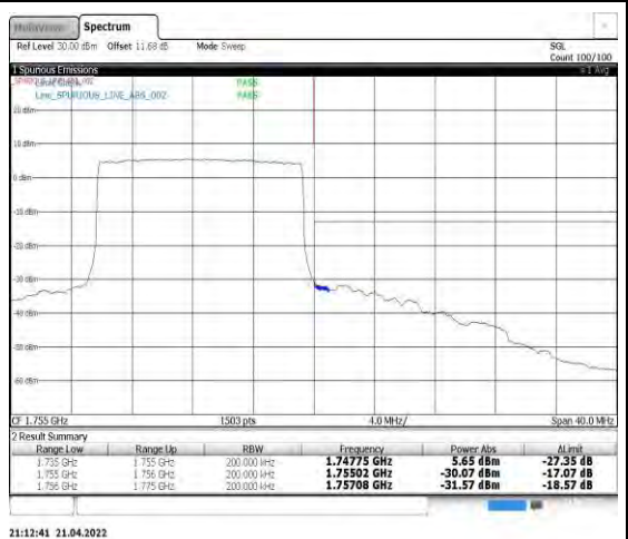
Band4-15MHz-QPSK-20325-75RB#0
