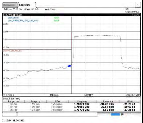
Band4-15MHz-QPSK-20025-75RB#0
