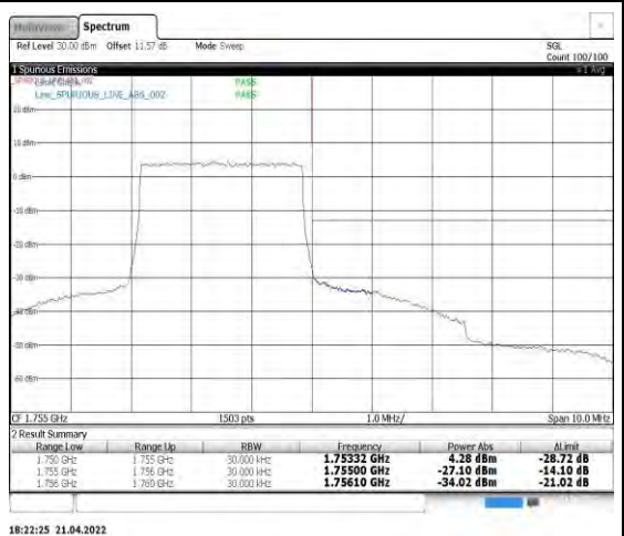
Band4-3MHz-QPSK-20385-15RB#0
