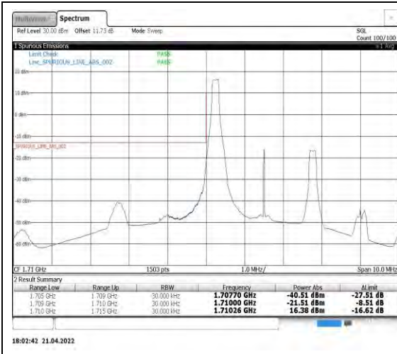
Band4-3MHz-16QAM-19965-1RB#0
