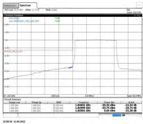
Band2-10MHz-16QAM-18650-50RB#0
