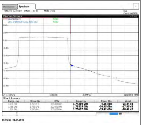
Band4-20MHz-QPSK-20300-100RB#0
