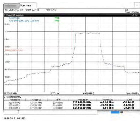
Band5-1.4MHz-QPSK-20407-6RB#0
