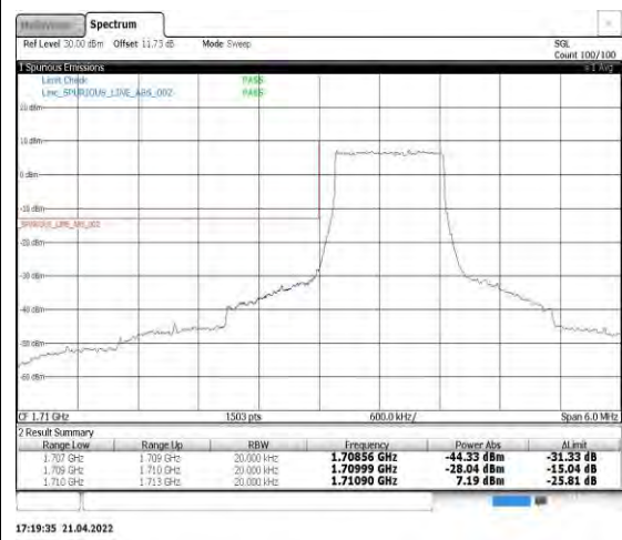
Band4-1.4MHz-QPSK-19957-6RB#0
