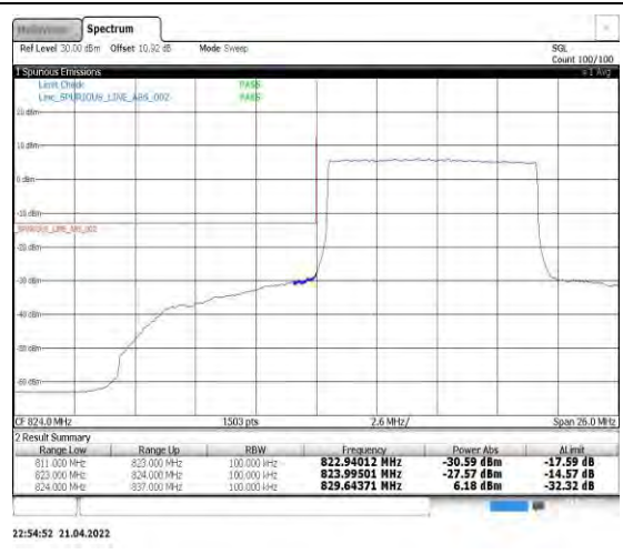
Band5-10MHz-QPSK-20450-50RB#0
