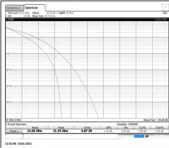
Band5-10MHz-QPSK-20525
