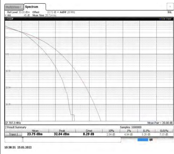
Band12-10MHz-16QAM-23095
