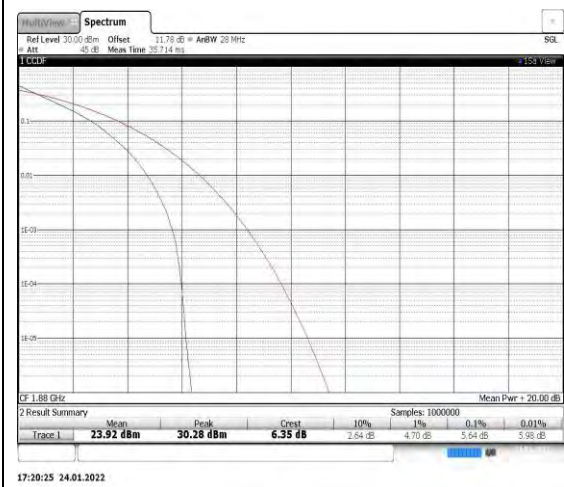
Band2-15MHz-QPSK-18900
