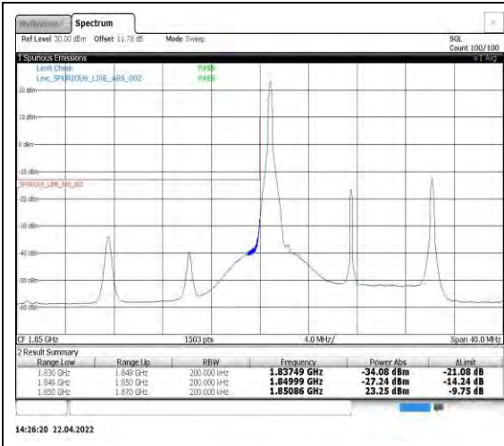
Band2-15MHz-16QAM-18675-1RB#0
