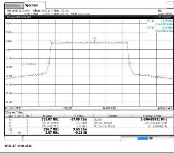
Band5-3MHz-16QAM-20525-15RB#0
