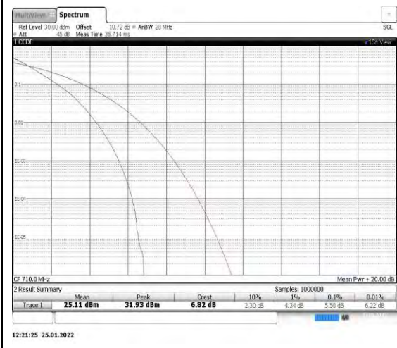
Band17-10MHz-QPSK-23790
