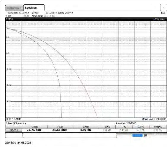
Band5-1.4MHz-QPSK-20525
