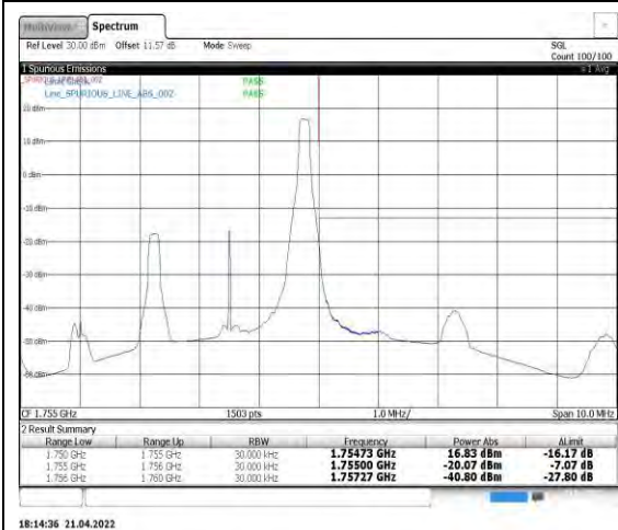
Band4-3MHz-QPSK-20385-1RB#14
