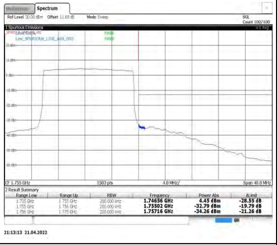
Band4-15MHz-16QAM-20325-75RB#0
