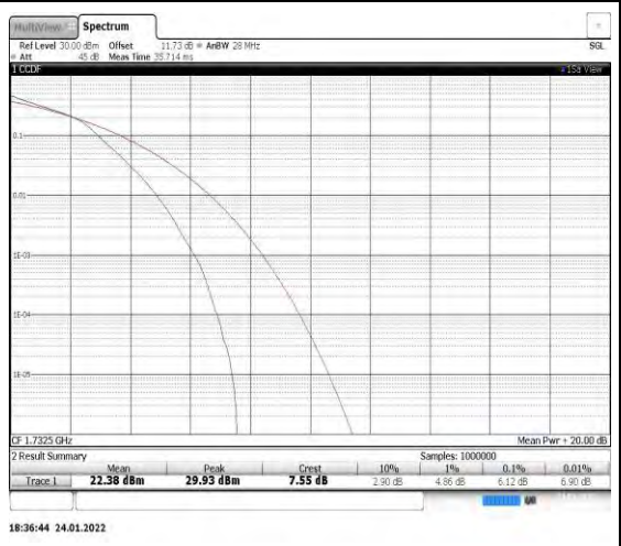
Band4-3MHz-16QAM-20175
