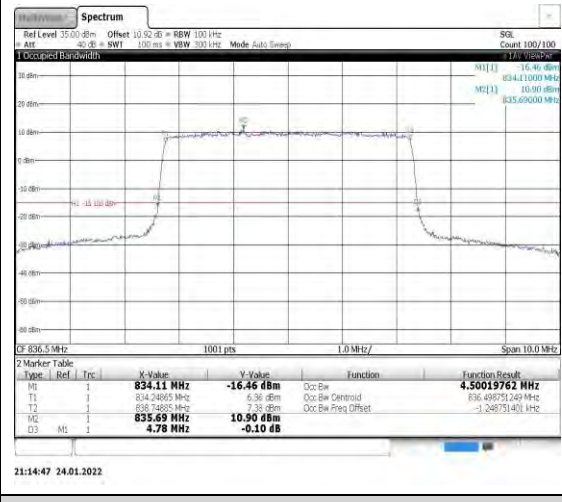
Band5-5MHz-16QAM-20525-25RB#0
