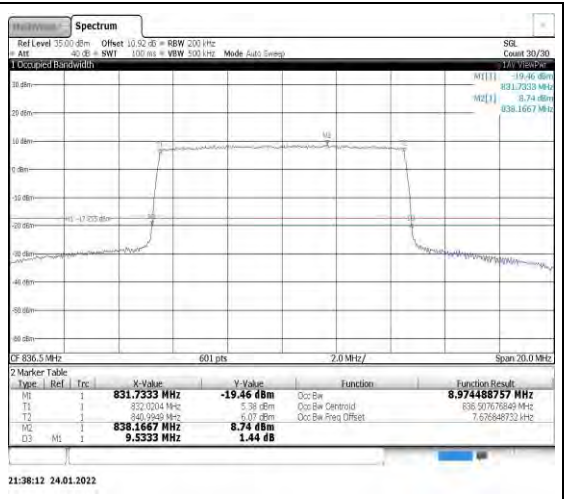
Band5-10MHz-16QAM-20525-50RB#0
