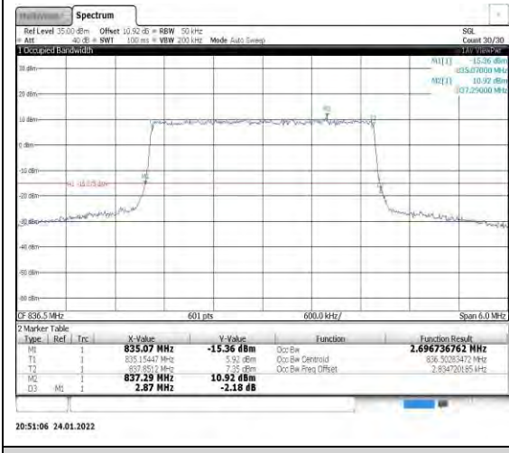
Band5-3MHz-QPSK-20525-15RB#0
