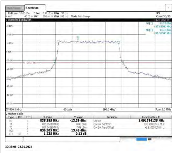
Band5-1.4MHz-QPSK-20525-6RB#0
