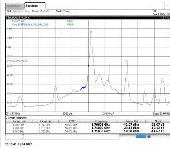
Band4-5MHz-16QAM-19975-1RB#0
