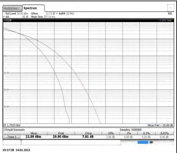
Band4-10MHz-16QAM-20175
