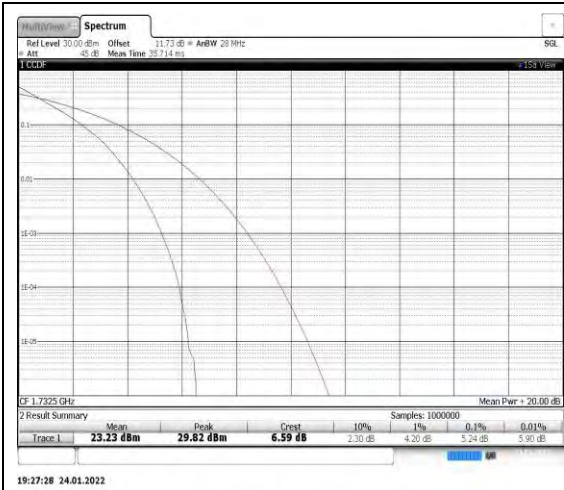
Band4-10MHz-QPSK-20175
