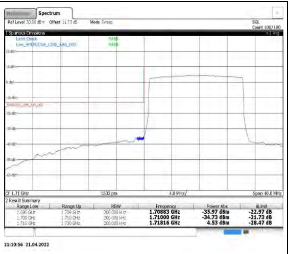
Band4-15MHz-16QAM-20025-75RB#0
