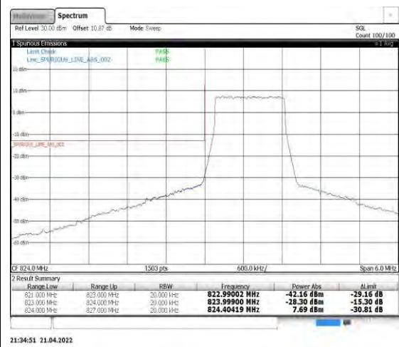
Band5-1.4MHz-16QAM-20407-6RB#0
