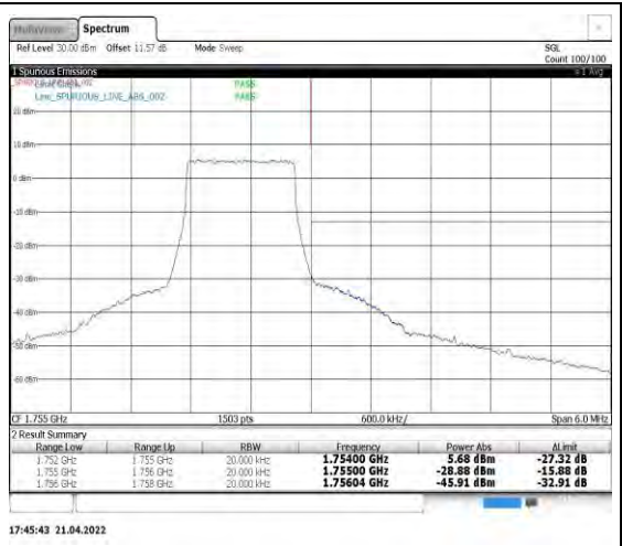
Band4-1.4MHz-16QAM-20393-6RB#0
