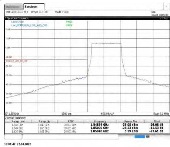
Band2-1.4MHz-16QAM-18607-6RB#0
