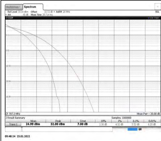
Band12-3MHz-QPSK-23095
