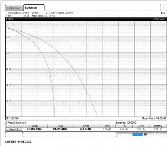
Band2-10MHz-QPSK-18900
