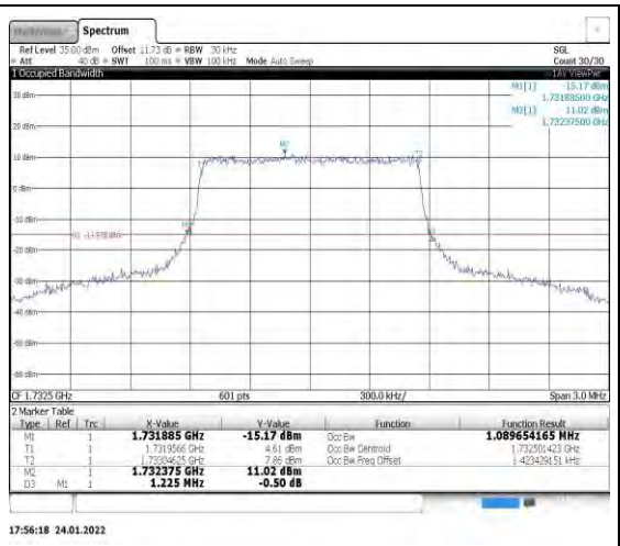
Band4-1.4MHz-16QAM-20175-6RB#0
