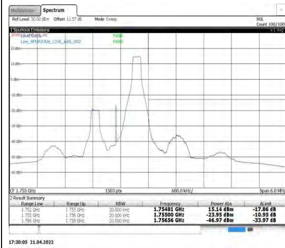
Band4-1.4MHz-QPSK-20393-1RB#5
