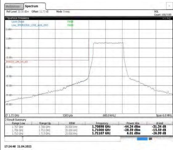
Band4-1.4MHz-16QAM-19957-6RB#0
