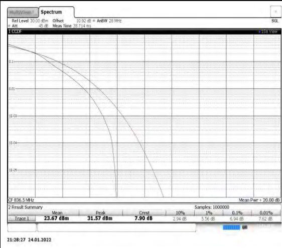
Band5-5MHz-16QAM-20525
