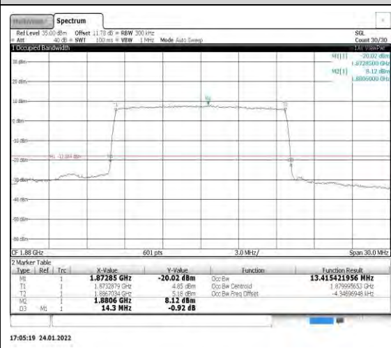
Band2-15MHz-16QAM-18900-75RB#0
