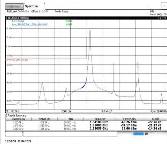
Band2-10MHz-16QAM-18650-1RB#0
