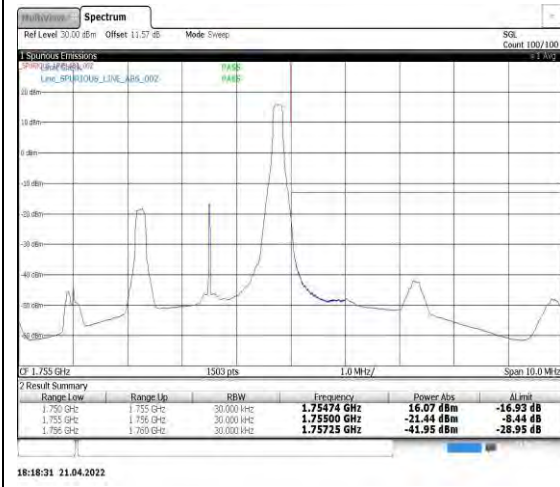
Band4-3MHz-16QAM-20385-1RB#14
