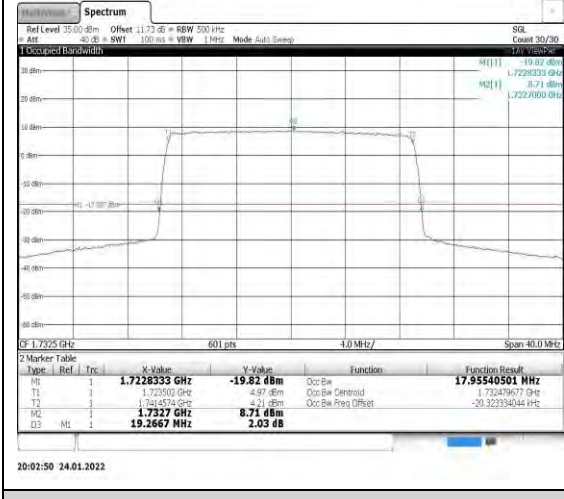
Band4-20MHz-QPSK-20175-100RB#0
