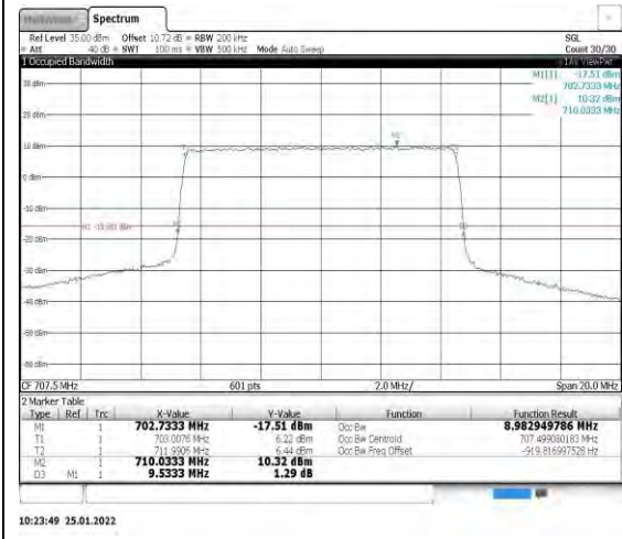
Band12-10MHz-QPSK-23095-50RB#0
