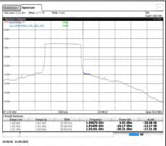
Band2-5MHz-QPSK-19175-25RB#0
