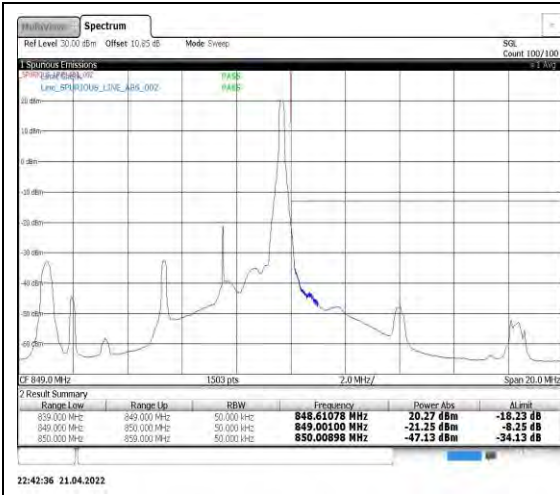
Band5-5MHz-QPSK-20625-1RB#24
