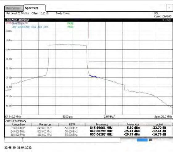
Band5-5MHz-QPSK-20625-25RB#0
