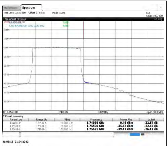
Band4-10MHz-16QAM-20350-50RB#0
