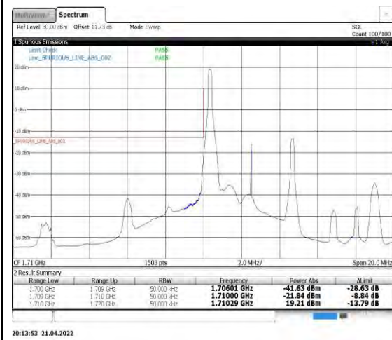
Band4-5MHz-QPSK-19975-1RB#0
