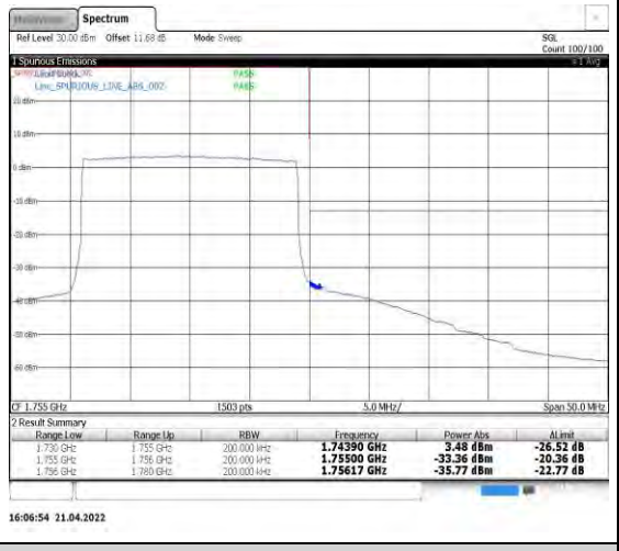
Band4-20MHz-16QAM-20300-100RB#0
