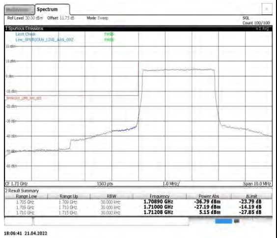
Band4-3MHz-QPSK-19965-15RB#0
