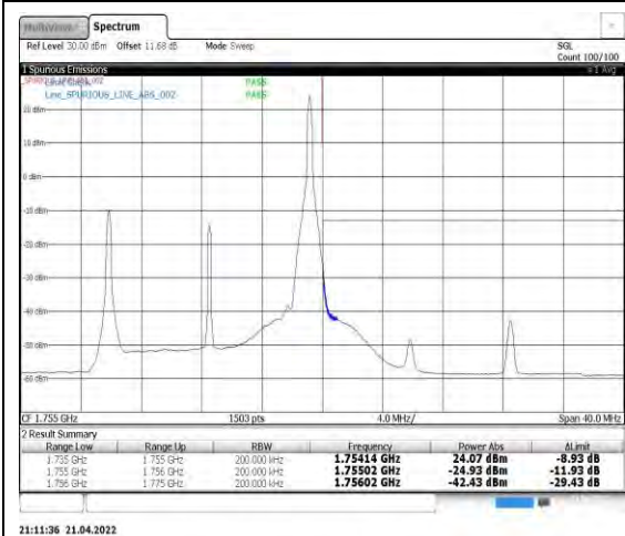
Band4-15MHz-QPSK-20325-1RB#74
