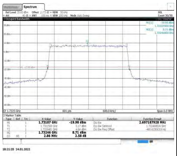
Band4-3MHz-16QAM-20175-15RB#0
