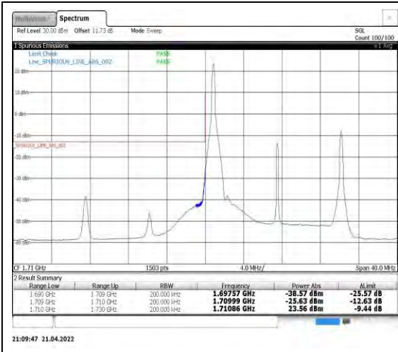
Band4-15MHz-16QAM-20025-1RB#0
