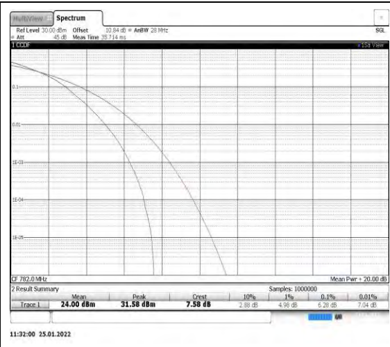
Band13-10MHz-16QAM-23230
