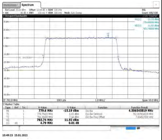
Band13-5MHz-16QAM-23230-25RB#0
