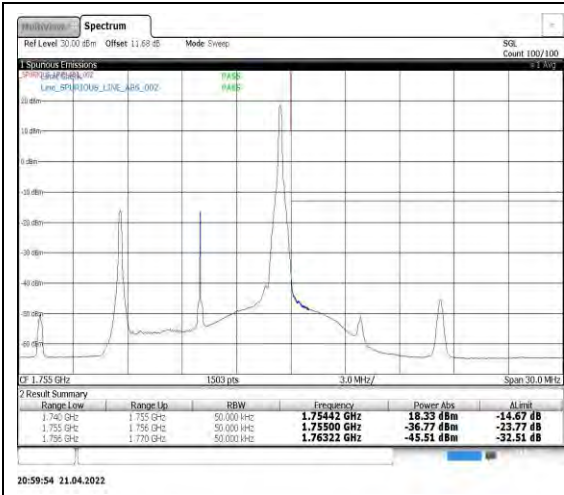
Band4-10MHz-16QAM-20350-1RB#49
