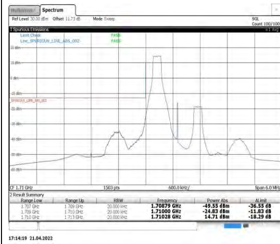
Band4-1.4MHz-16QAM-19957-1RB#0
