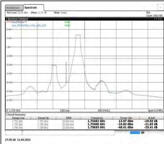
Band4-1.4MHz-16QAM-20393-1RB#5
