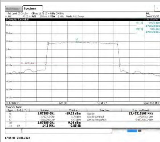
Band2-15MHz-QPSK-18900-75RB#0
