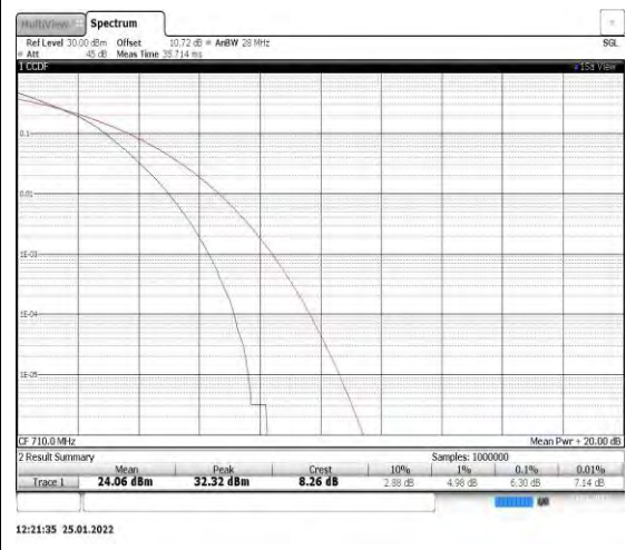
Band17-10MHz-16QAM-23790
