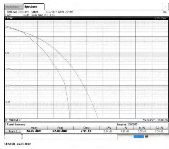
Band17-5MHz-16QAM-23790
