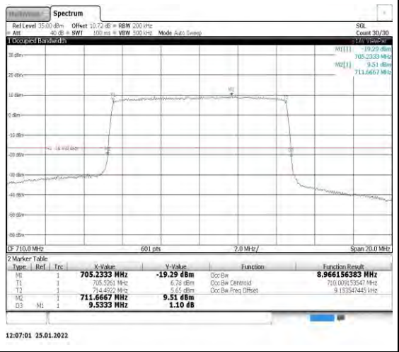
Band17-10MHz-16QAM-23790-50RB#0
