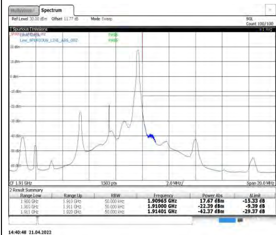
Band2-5MHz-16QAM-19175-1RB#24
