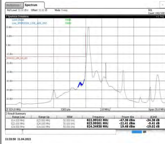
Band5-5MHz-16QAM-20425-1RB#0
