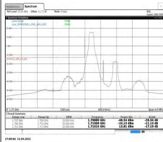
Band4-1.4MHz-QPSK-19957-1RB#0
