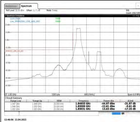
Band2-1.4MHz-QPSK-18607-1RB#0
