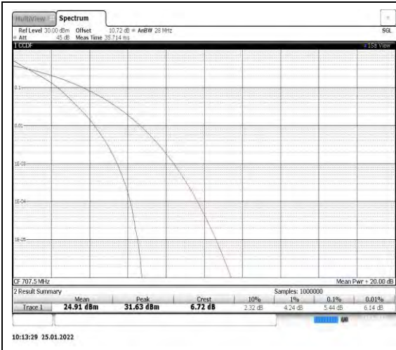
Band12-5MHz-QPSK-23095
