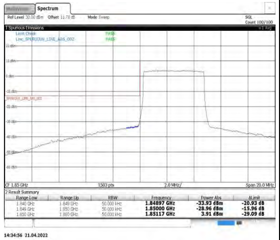
Band2-5MHz-16QAM-18625-25RB#0
