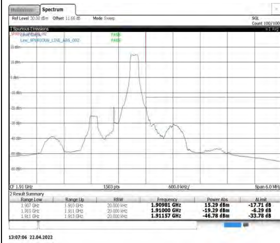
Band2-1.4MHz-QPSK-19193-1RB#5
