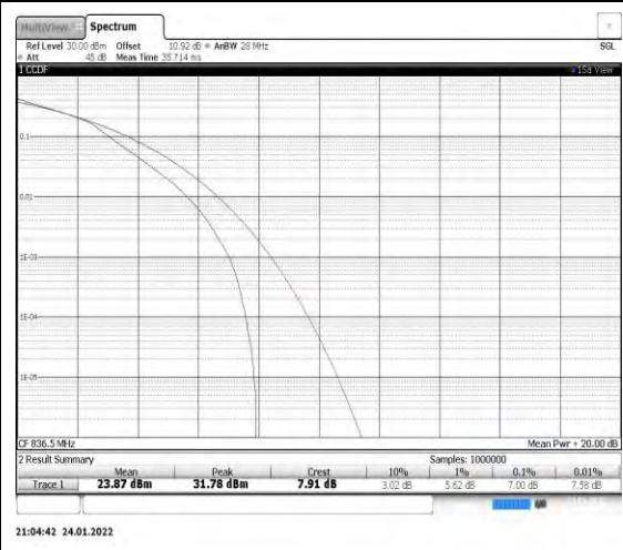
Band5-3MHz-16QAM-20525
