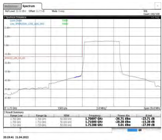
Band4-5MHz-QPSK-19975-25RB#0
