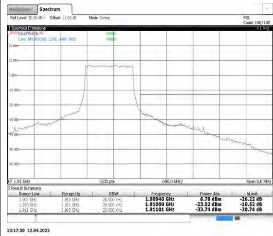
Band2-1.4MHz-QPSK-19193-6RB#0
