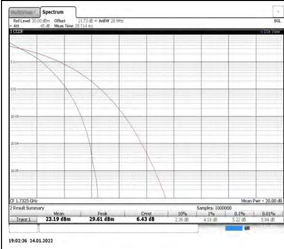
Band4-5MHz-QPSK-20175
