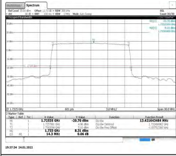
Band4-15MHz-QPSK-20175-75RB#0
