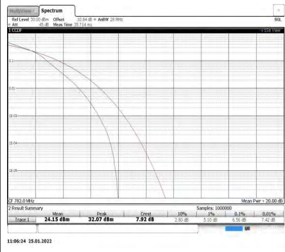
Band13-5MHz-16QAM-23230
