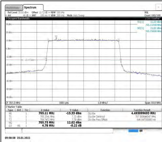
Band12-5MHz-QPSK-23095-25RB#0
