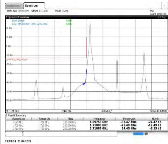
Band4-15MHz-QPSK-20025-1RB#0
