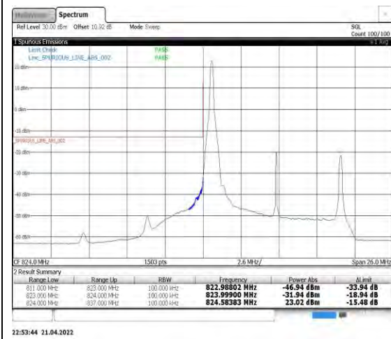
Band5-10MHz-16QAM-20450-1RB#0
