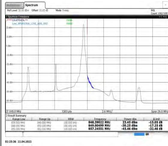
Band5-10MHz-QPSK-20600-1RB#49
