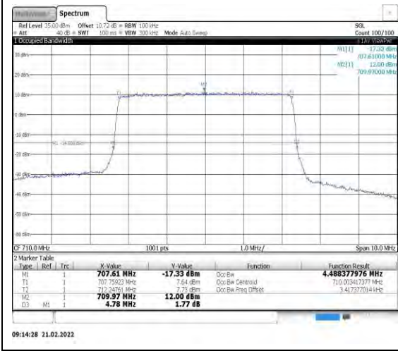
Band17-5MHz-QPSK-23790-25RB#0
