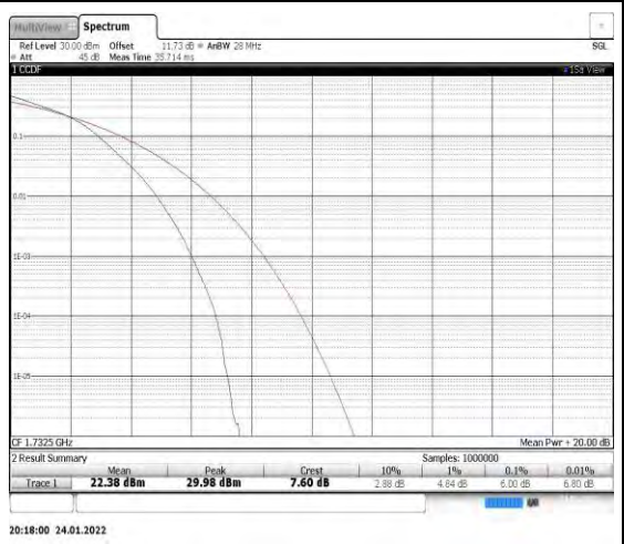
Band4-20MHz-16QAM-20175
