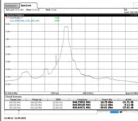
Band5-1.4MHz-QPSK-20643-1RB#5
