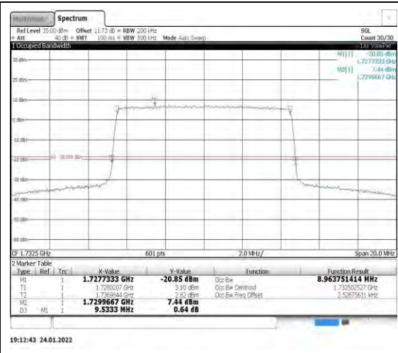
Band4-10MHz-16QAM-20175-50RB#0
