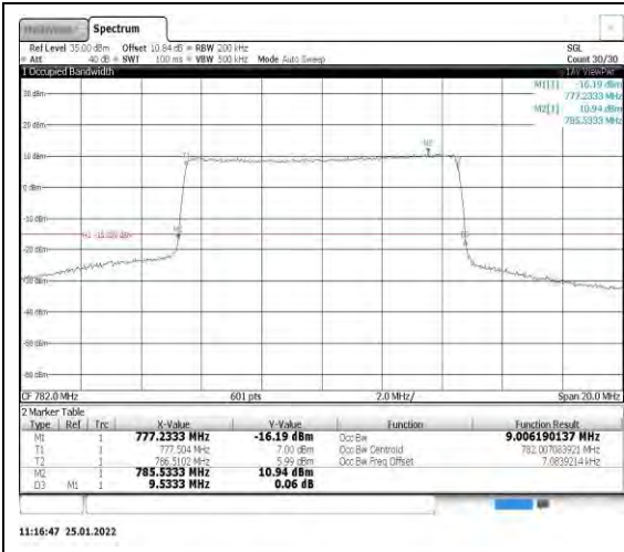
Band13-10MHz-QPSK-23230-50RB#0
