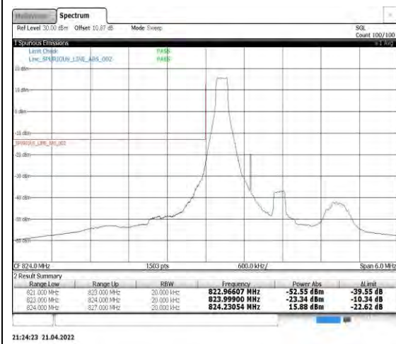
Band5-1.4MHz-16QAM-20407-1RB#0
