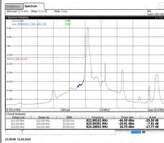
Band5-5MHz-QPSK-20425-1RB#0
