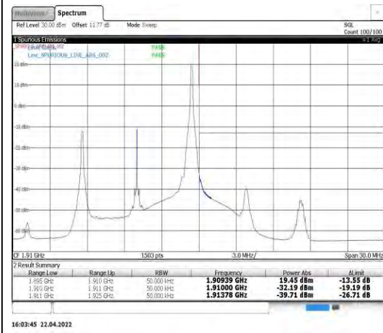
Band2-10MHz-QPSK-19150-1RB#49
