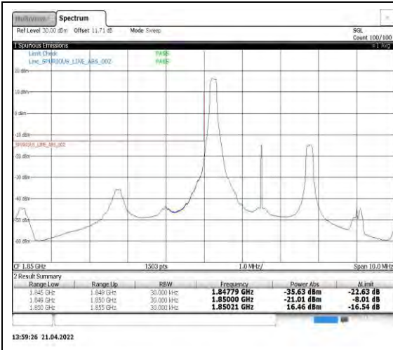
Band2-3MHz-16QAM-18615-1RB#0
