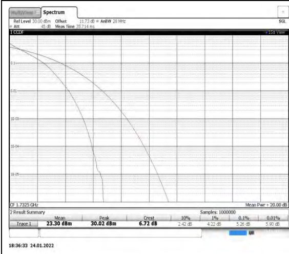
Band4-3MHz-QPSK-20175
