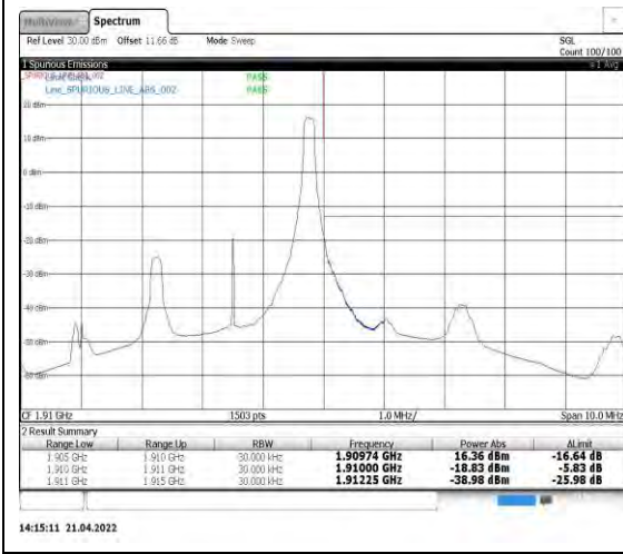
Band2-3MHz-16QAM-19185-1RB#14
