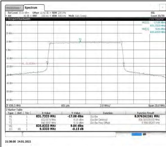
Band5-10MHz-QPSK-20525-50RB#0
