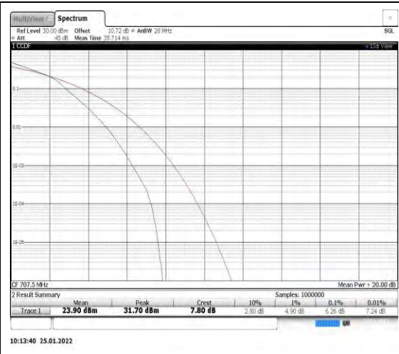
Band12-5MHz-16QAM-23095
