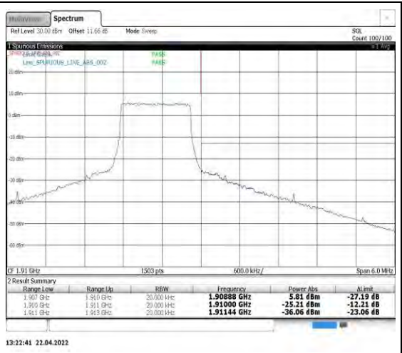
Band2-1.4MHz-16QAM-19193-6RB#0
