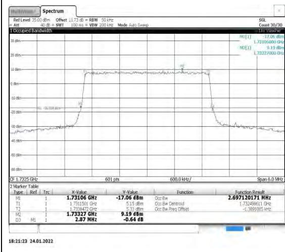
Band4-3MHz-QPSK-20175-15RB#0
