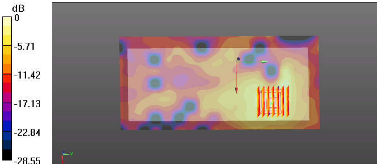
0 dB = 0.0362 W/kg
