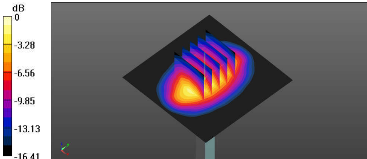
0 dB = 12.2 W/kg
