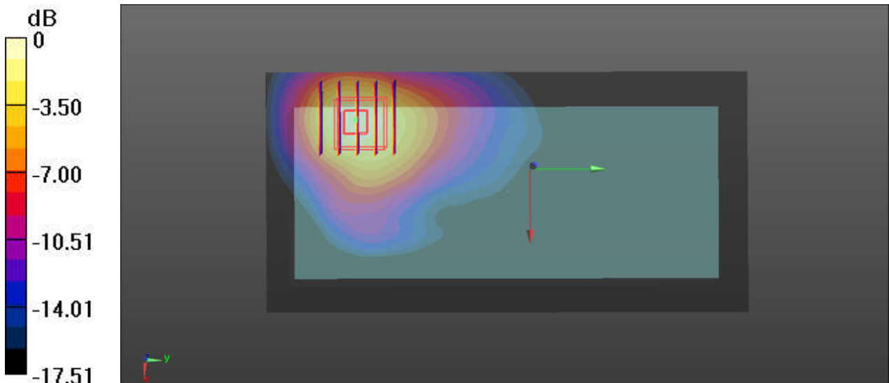
0 dB = 1.68 W/kg
