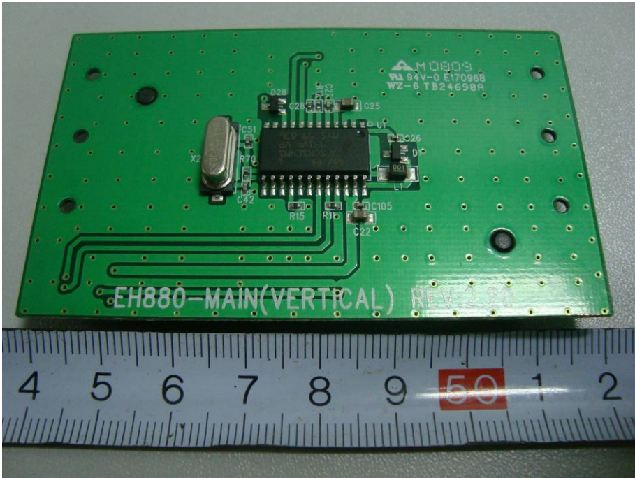
EUT – Main Board (IC Card Reader) Top Components View (eH880-DP-CF)
