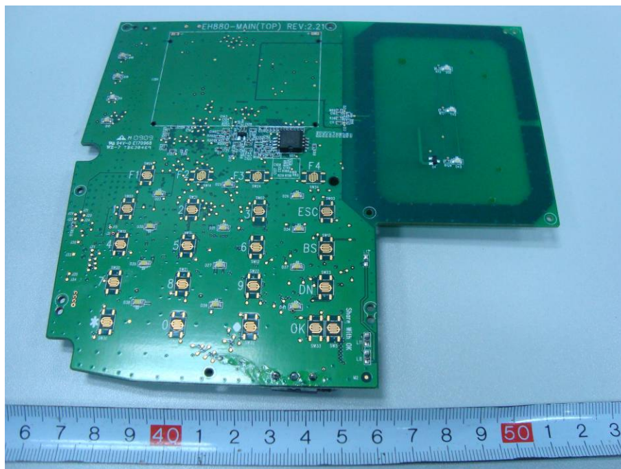
EUT – Main Board (Wireless Card Reader) Bottom Components View 2 (eH880-DP-CF)
