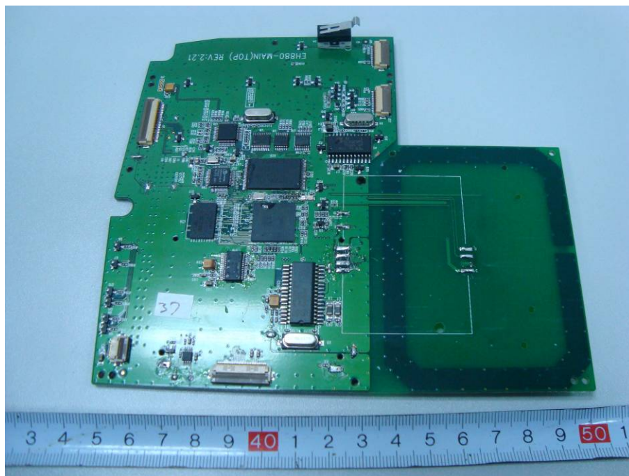
EUT – Main Board (Wireless Card Reader) Top Components Uncovered View (eH880-DP-CF)
