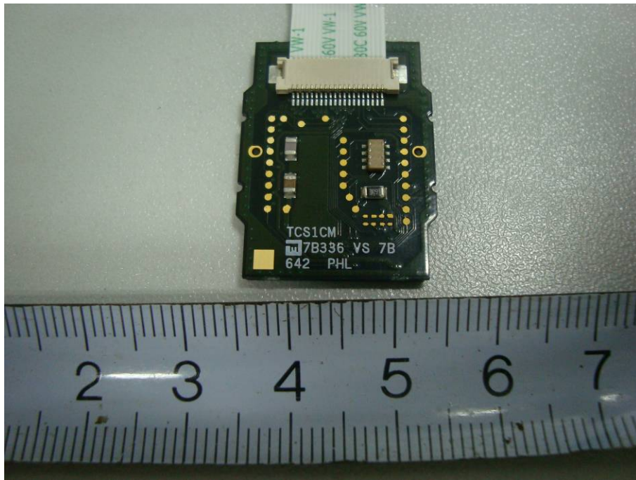
EUT – Fingerprint Board Bottom View (eH880-DP-CF)
