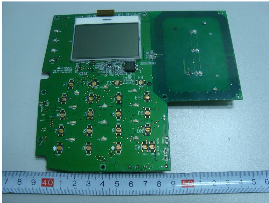
EUT – Main Board (Wireless Card Reader) Bottom Components View 1 (eH880-DP-CF)
