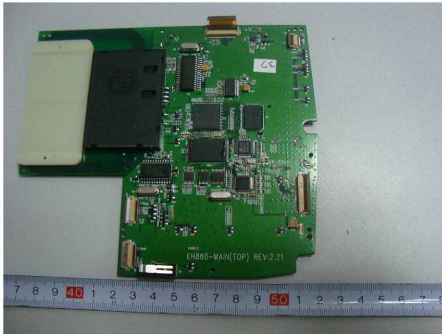
EUT – Main Board (Wireless Card Reader) Top Components View (eH880-DP-CF)
