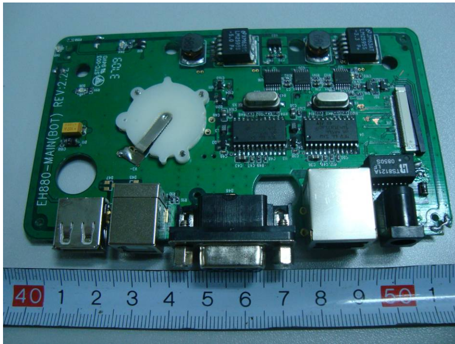
EUT – Main Board (Control and Data I/O) Top Components View (eH880-DP-CF)
