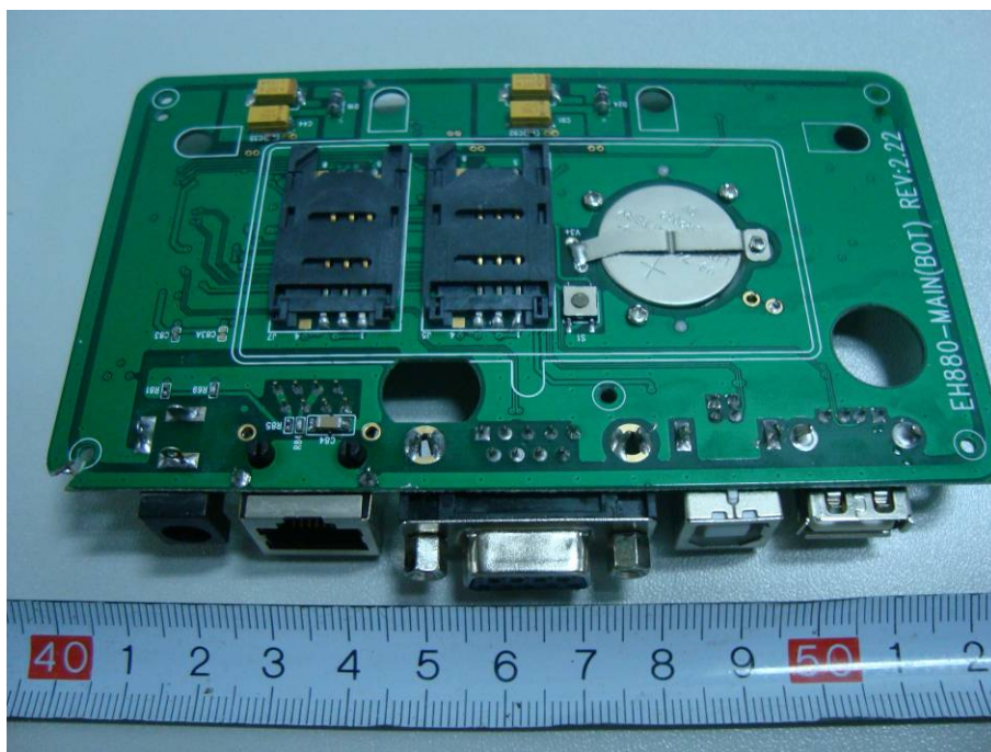
EUT – Main Board (Control and Data I/O) Bottom Components View (eH880-DP-CF)
