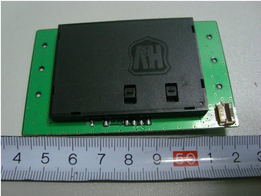
EUT – Main Board (IC Card Reader) Bottom Components View (eH880-DP-CF)
