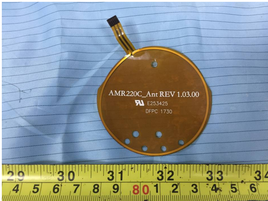
EUT – RFID Antenna Top View
