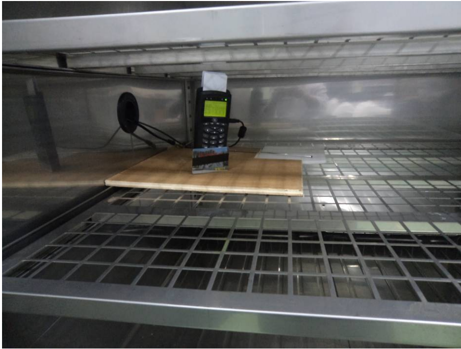
Frequency Stability Testing View (PC-Linked)
