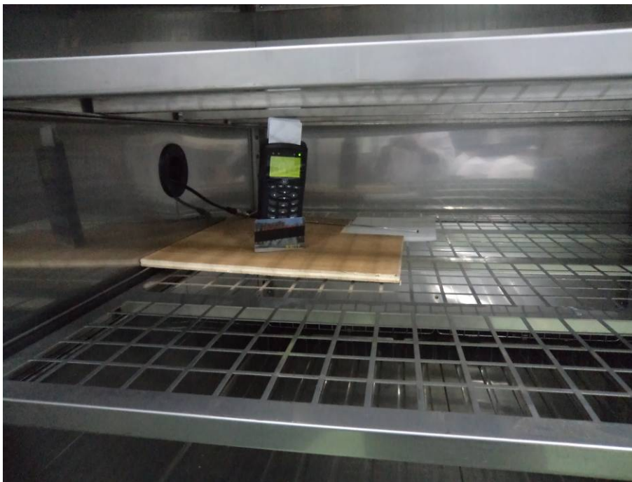
Frequency Stability Testing View (Stand-alone)
