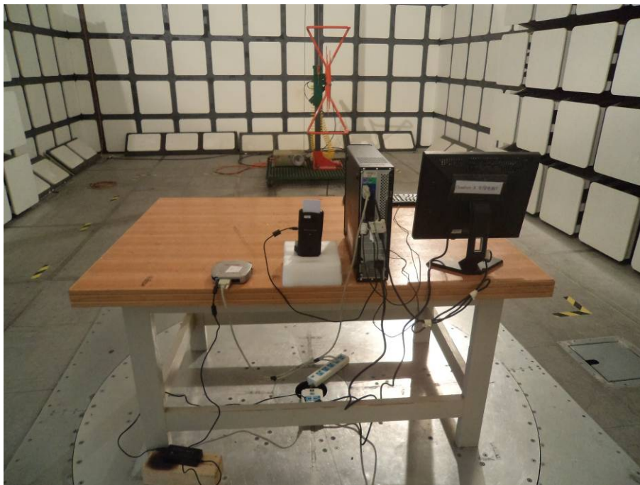
Radiated Emissions – Rear View (Above 30 MHz) (PC-Linked)
