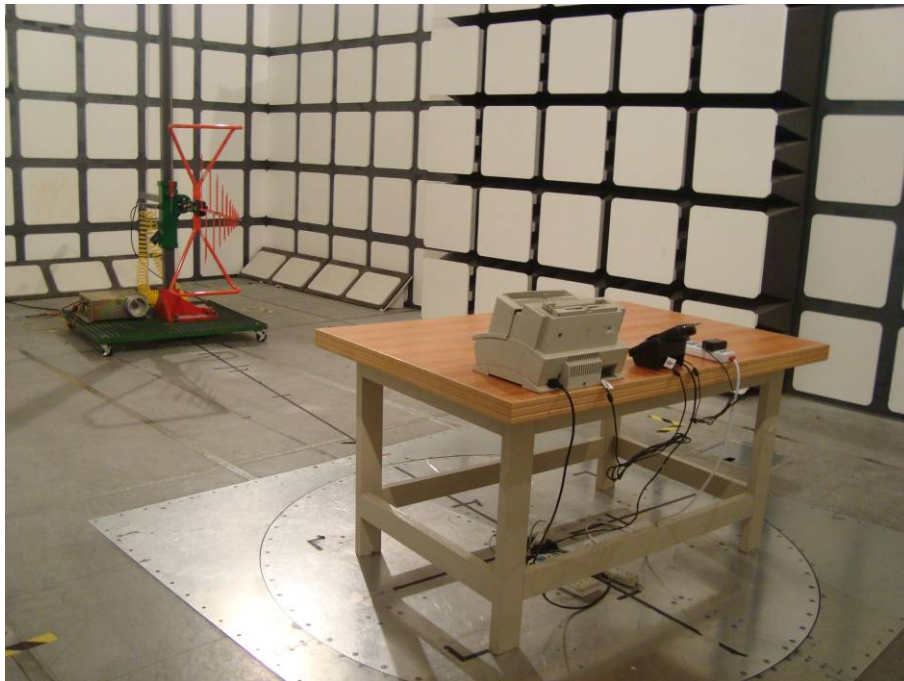
Above 30MHz: Radiated Emissions - Rear View
