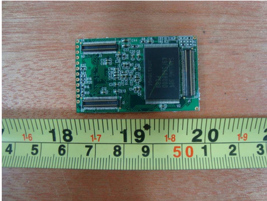
EUT – Handheld CPU Board Bottom View
