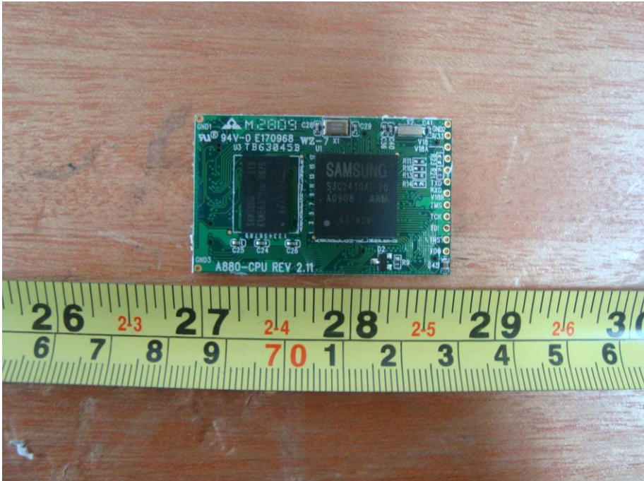
EUT – Handheld CPU Board Top View
