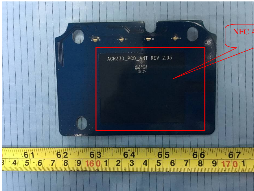
EUT –NFC Antenna Top View
