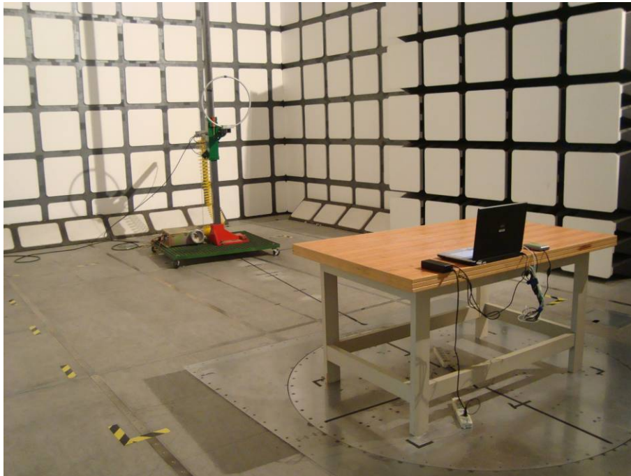
Below 30MHz: Radiated Emissions - Rear View
