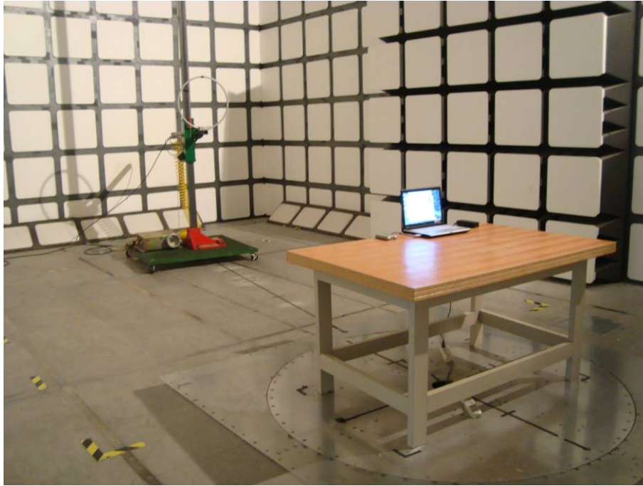
Below 30MHz: Radiated Emissions - Front View
