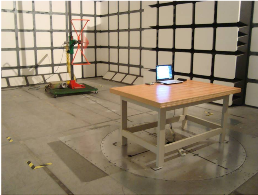
Above 30MHz: Radiated Emissions - Front View
