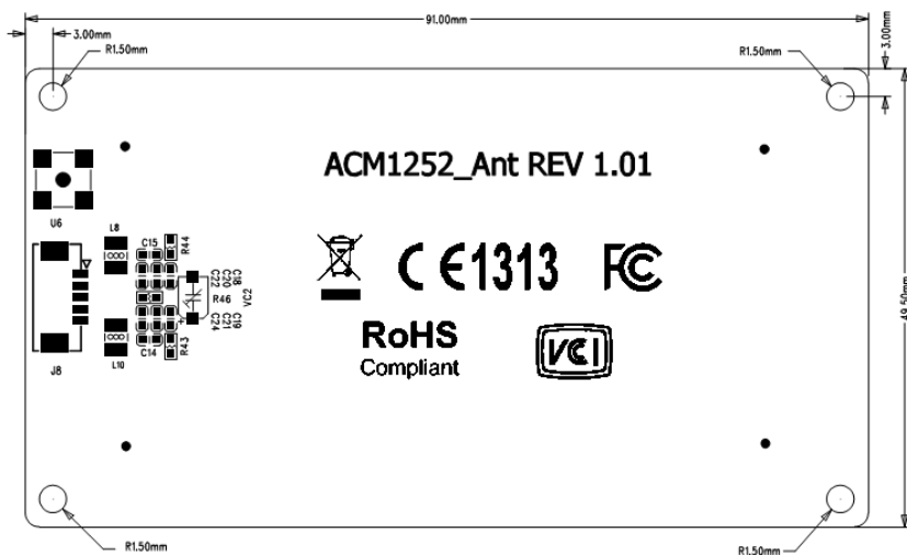
Antenna Board:
