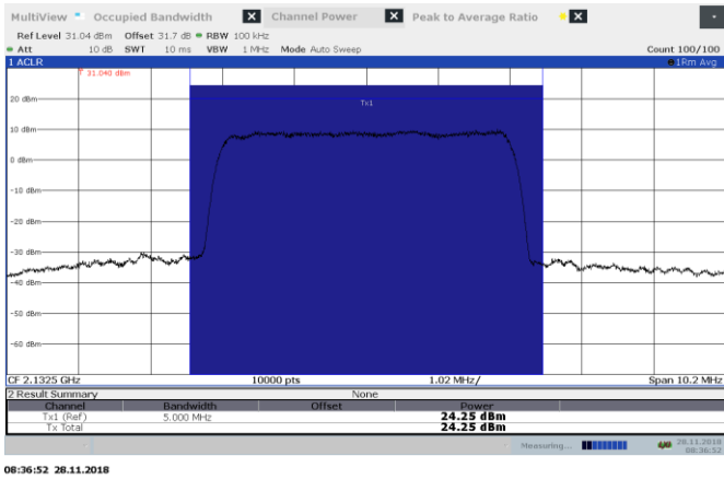
Figure 8.4-7: AWGN AGC +3dB 2132.5 MHz output DL
