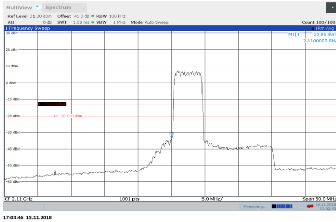
Figure 8.5-15: AWGN 2112.5 MHz AGC - 0.5dB Out-of-block DL
