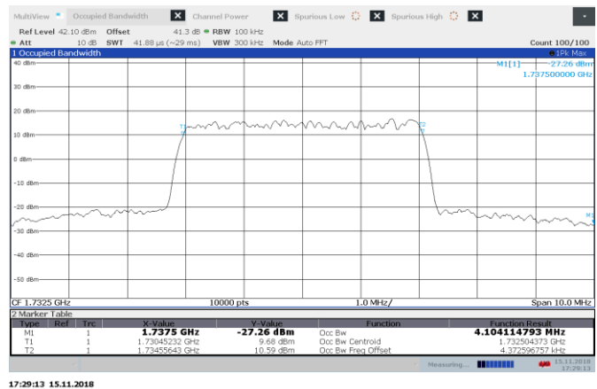
Figure 8.3-4: AWGN AGC +3 dB 1732.5 MHz output 99% BW UL
