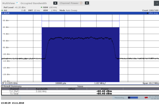
Figure 8.4-5: AWGN AGC—0.5 dB 2132.5 MHz input DL
