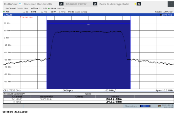
Figure 8.4-2: AWGN AGC—0.5 dB 1732.5 MHz output UL
