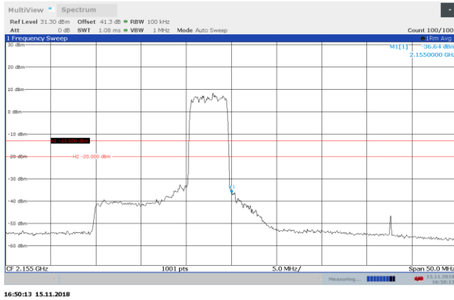
Figure 8.5-13: AWGN 2152.5 MHz AGC - 0.5dB Out-of-block DL
