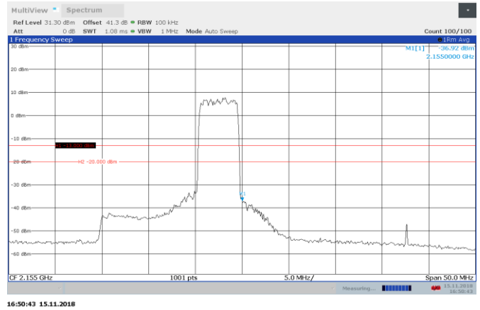
Figure 8.5-14: AWGN 2152.5 MHz AGC+ 3dB Out-of-block DL
