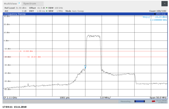
Figure 8.5-16: AWGN 2112.5 MHz AGC + 3dB Out-of-block DL
