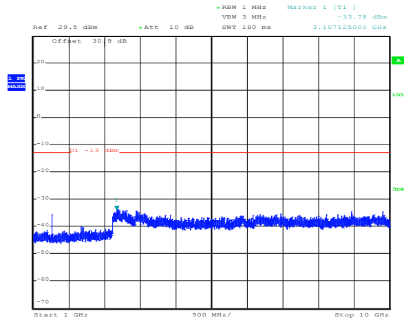
Figure 8.6-2: 1-10 GHz 728 MHz
