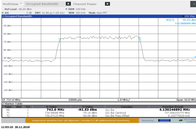
Figure 8.3-3: AGC +3 dB 737 MHz input 99% BW DL
