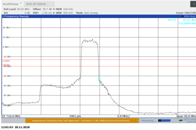
Figure 8.5-13: 713.5 MHz AGC - 0.5dB Out-of-block UL
