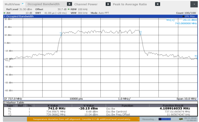
Figure 8.3-2: AGC-0.5 dB 737 MHz output 99% BW DL
