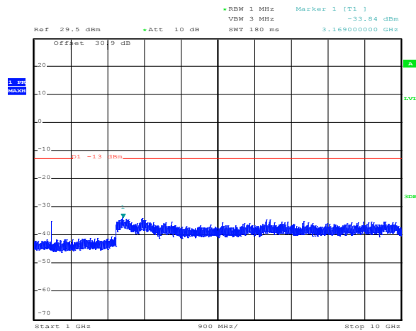
Figure 8.6-10: 1-10 GHz 707 MHz
