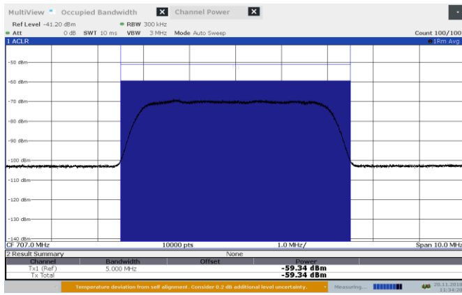
Figure 8.4-5: AGC -0.5 dB 707 MHz Input UL
