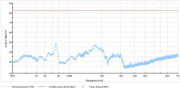
Figure 8.7-1: 30 MHz to 1 GHz UL
