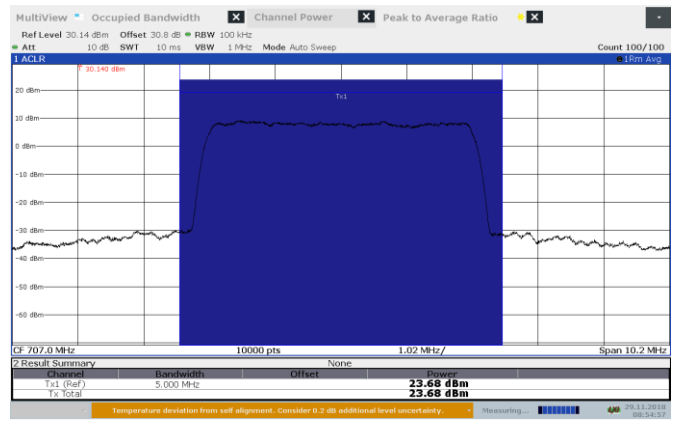
Figure 8.4-6: AGC -0.5 dB 707 MHz Output UL
