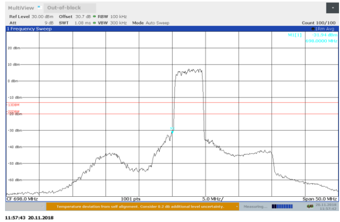
Figure 8.5-16: 700.5 MHz AGC + 3 dB Out-of-block UL
