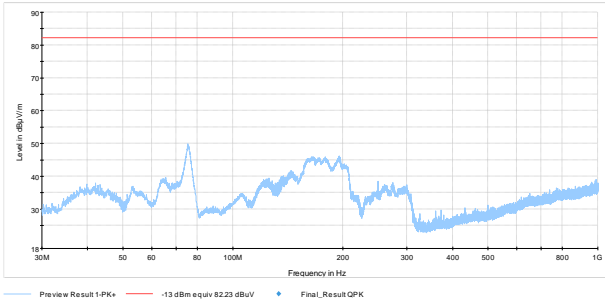
Figure 8.7-3: 30 MHz to 1 GHz DL
