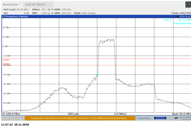
Figure 8.5-15: 700.5 MHz AGC - 0.5dB Out-of-block UL
