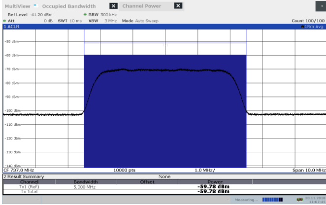
Figure 8.4-1: AGC -0.5 dB 737 MHz Input DL
