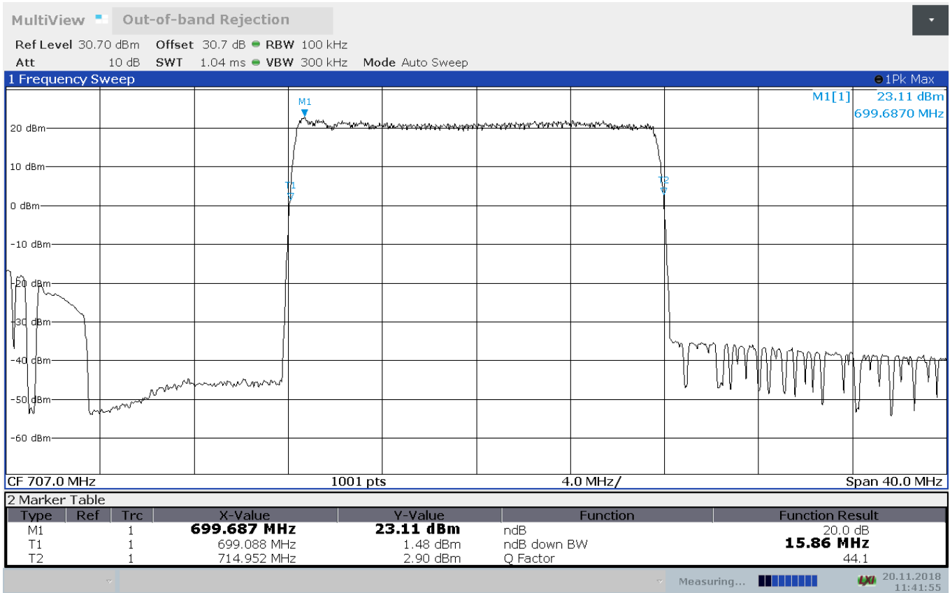
Figure 8.2-2: Passband Uplink
