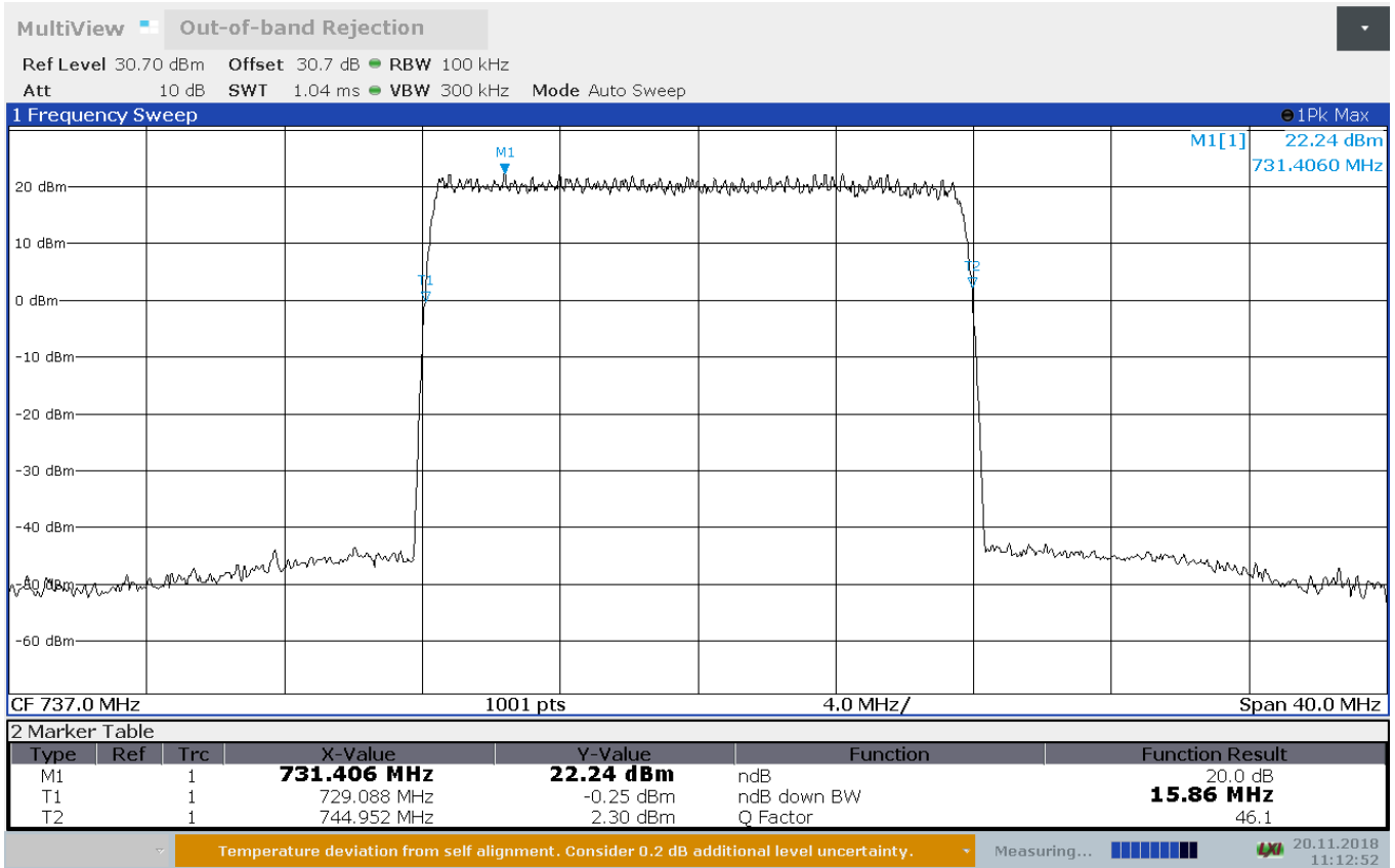
Figure 8.2-1: Passband Downlink
