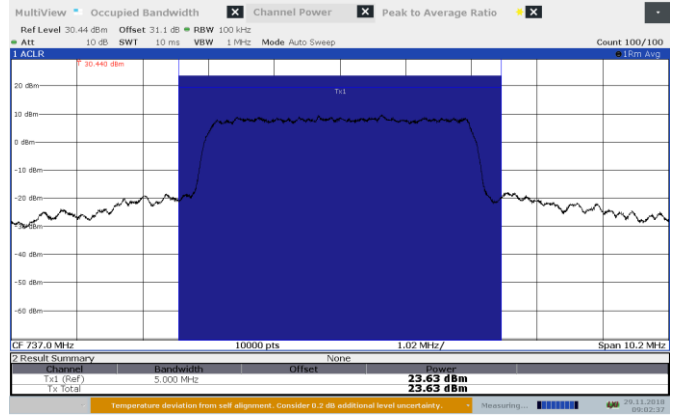
Figure 8.4-2: AGC -0.5 dB 737 MHz Output DL
