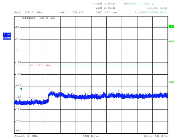
Figure 8.6-6: 1-10 GHz 746 MHz
