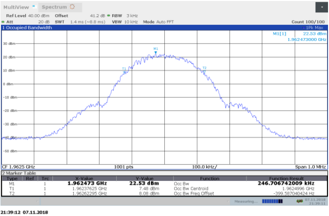
Figure 8.3-10: MSK AGC-0.5 dB 1962.5 MHz output 99% BW DL
