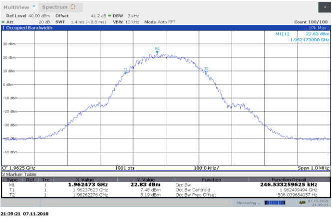
Figure 8.3-12: MSK AGC+3 dB 1962.5 MHz output 99% BW DL
