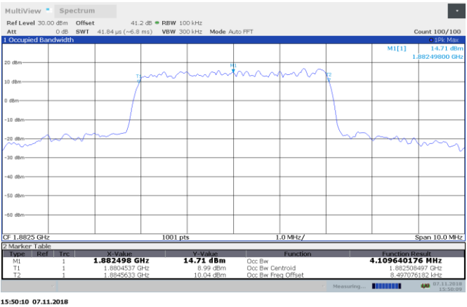
Figure 8.3-6: AWGN AGC -0.5 dB 1882.5 MHz output 99% BW UL
