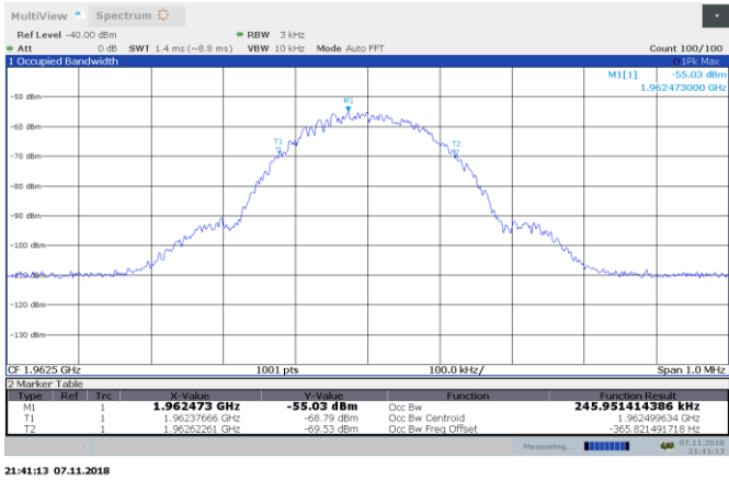
Figure 8.3-11: MSK AGC+3 dB 1962.5 MHz input 99% BW DL
