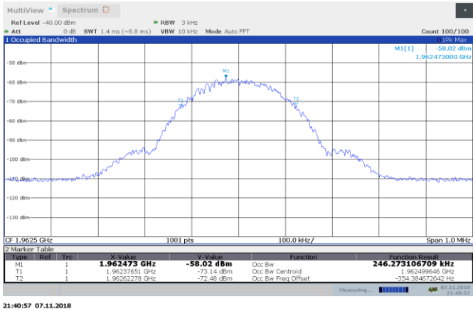
Figure 8.3-9: MSK AGC-0.5 dB 1962.5 MHz input 99% BW DL
