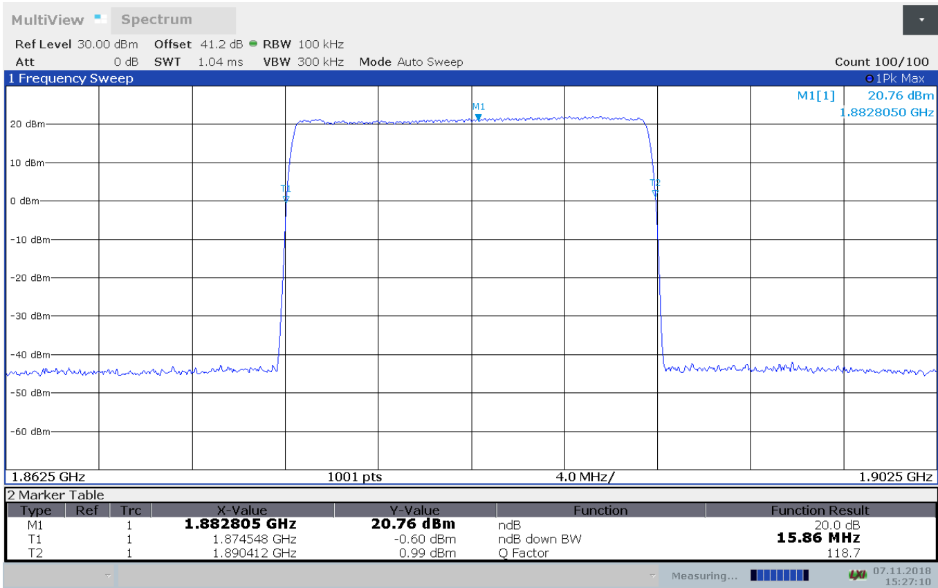
Figure 8.2-1: Passband Uplink
