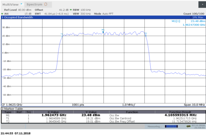
Figure 8.3-16: AWGN AGC +3 dB 1962.5 MHz output 99% BW DL
