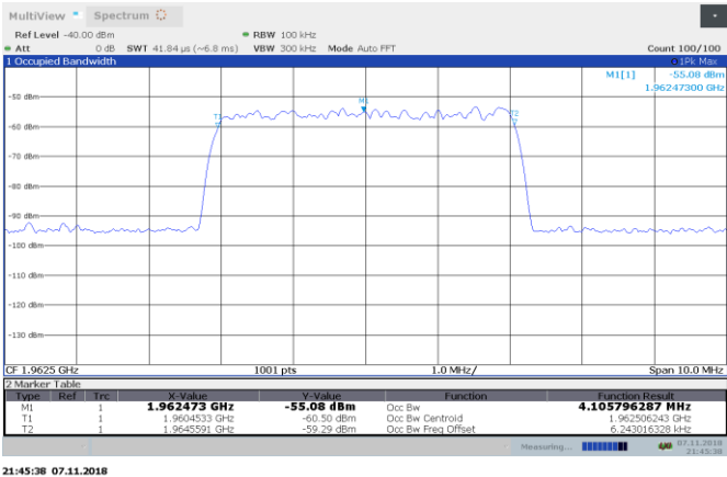
Figure 8.3-15: AWGN AGC +3 dB 1962.5 MHz input 99% BW DL
