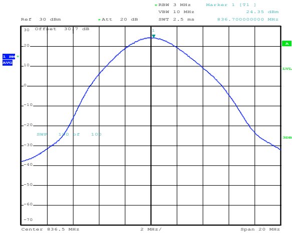
Figure 8.4-14: MSK AGC-0.5 dB UL 836.5 MHz output power peak
