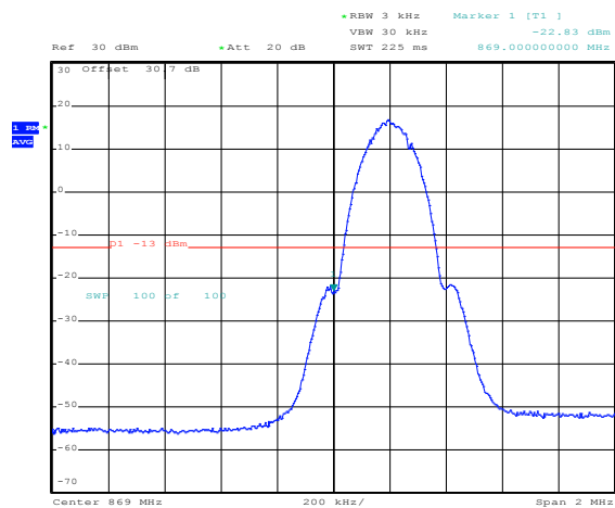
Figure 8.5-29: 2X MSK 869.2 and 869.4 MHz DL AGC Out-of-block
