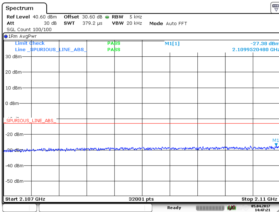
2 GSM signal on lower band edge AGC off
