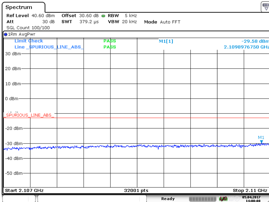
2 GSM signal on lower band edge AGC on
