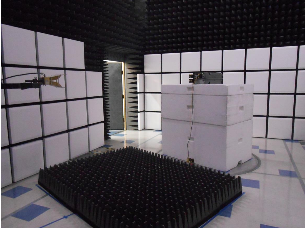
Radiated RF above 1 GHz
