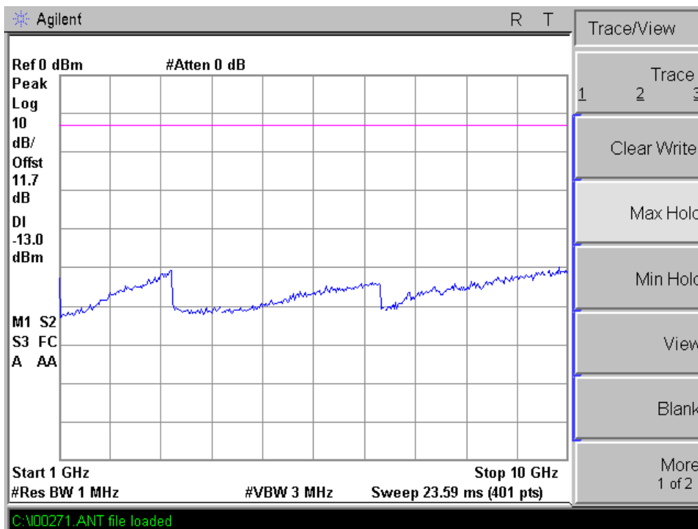
869MHz 1-10GHz
